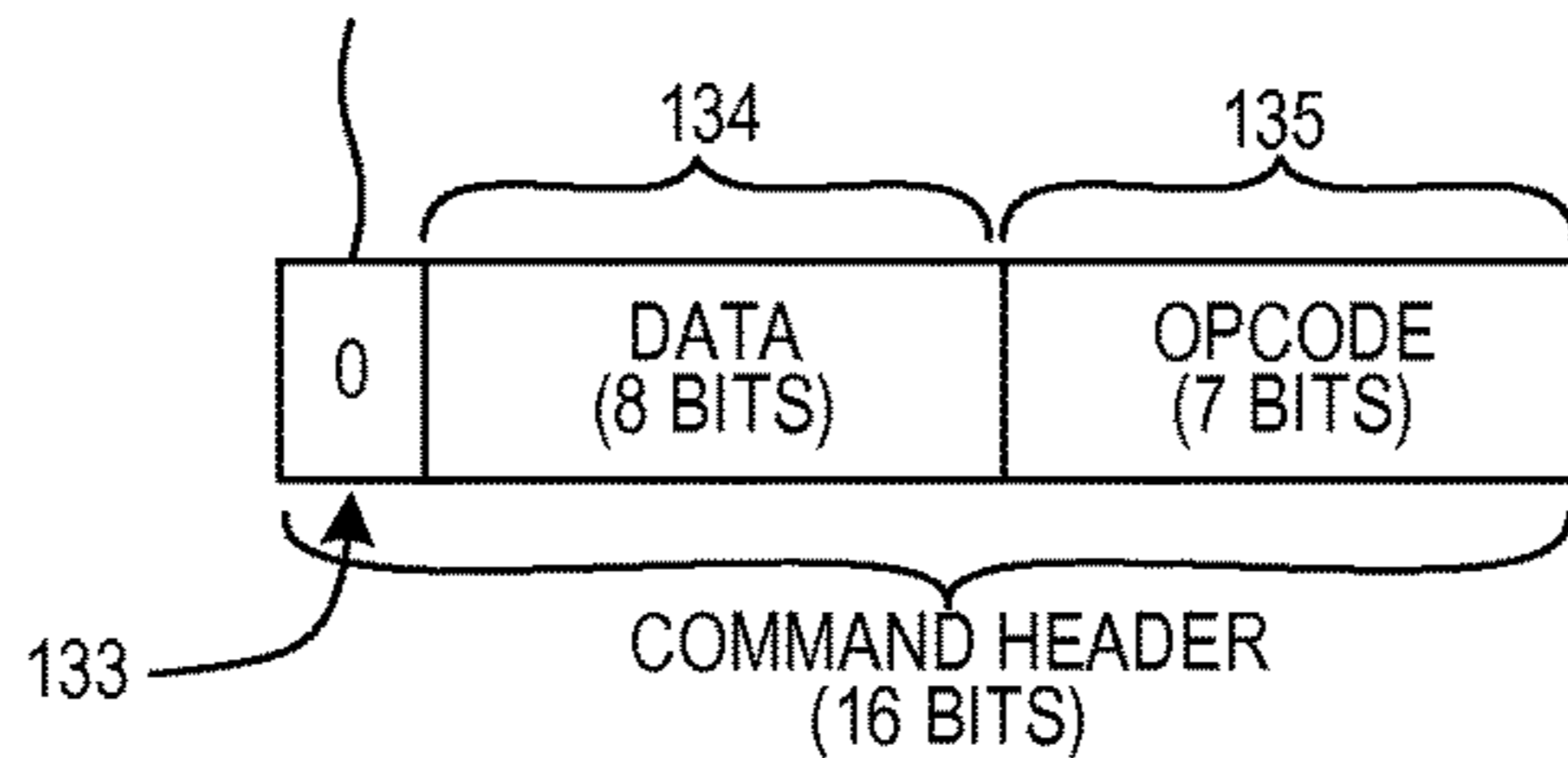
ONE COMMAND HEADER FIG. 13
