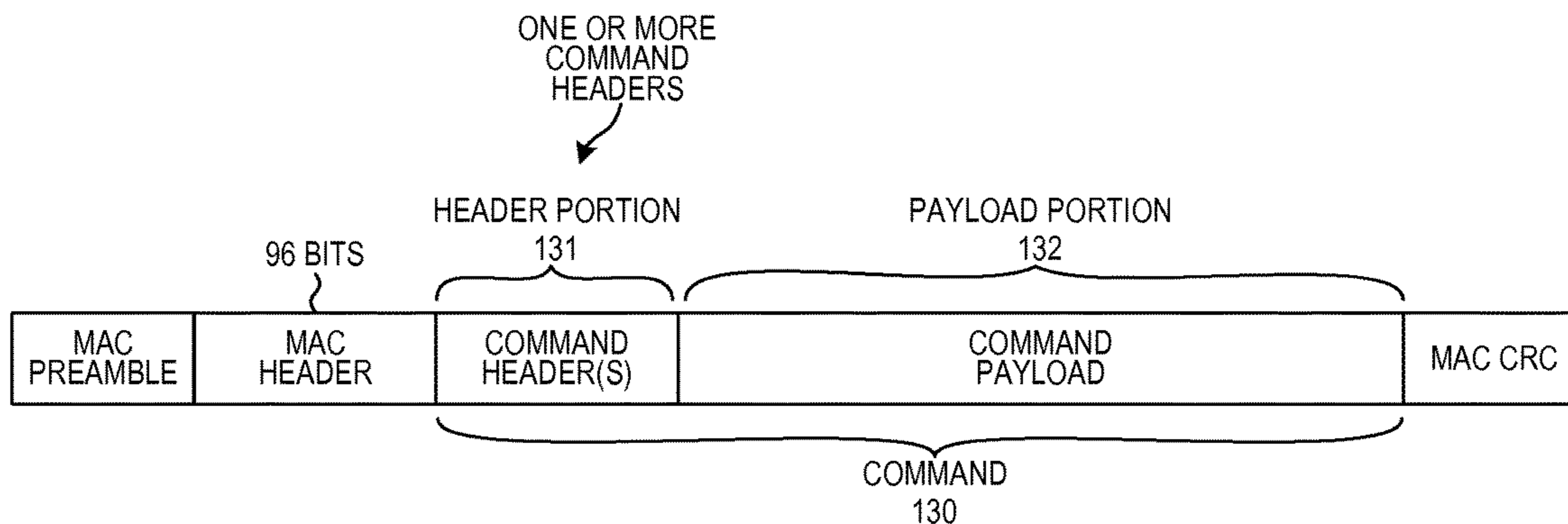
MAC FRAME (COMMAND MODE) FIG. 12
