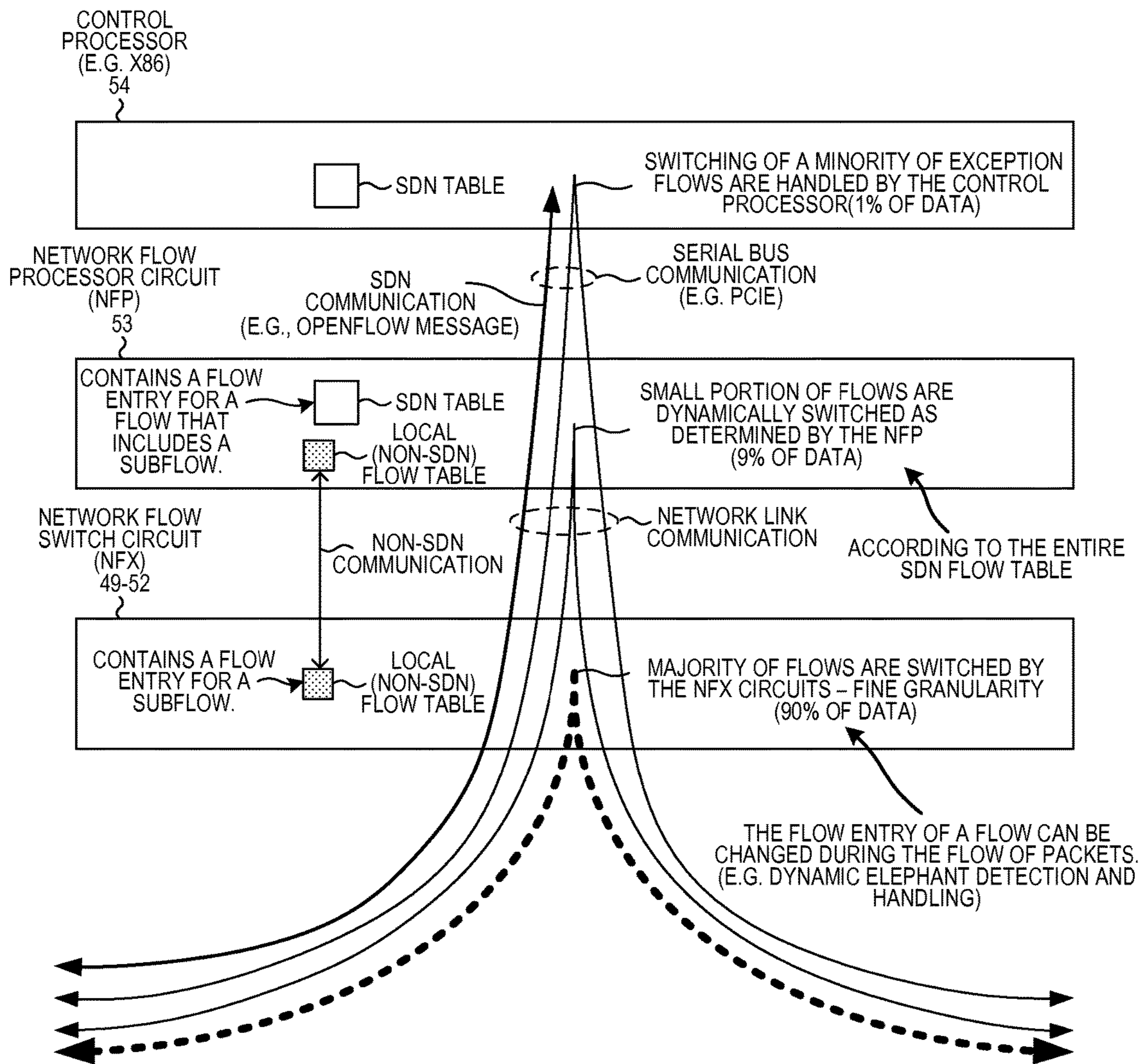
IMPROVED OPERATION WITH NFX ARCHITECTURE FIG. 16
