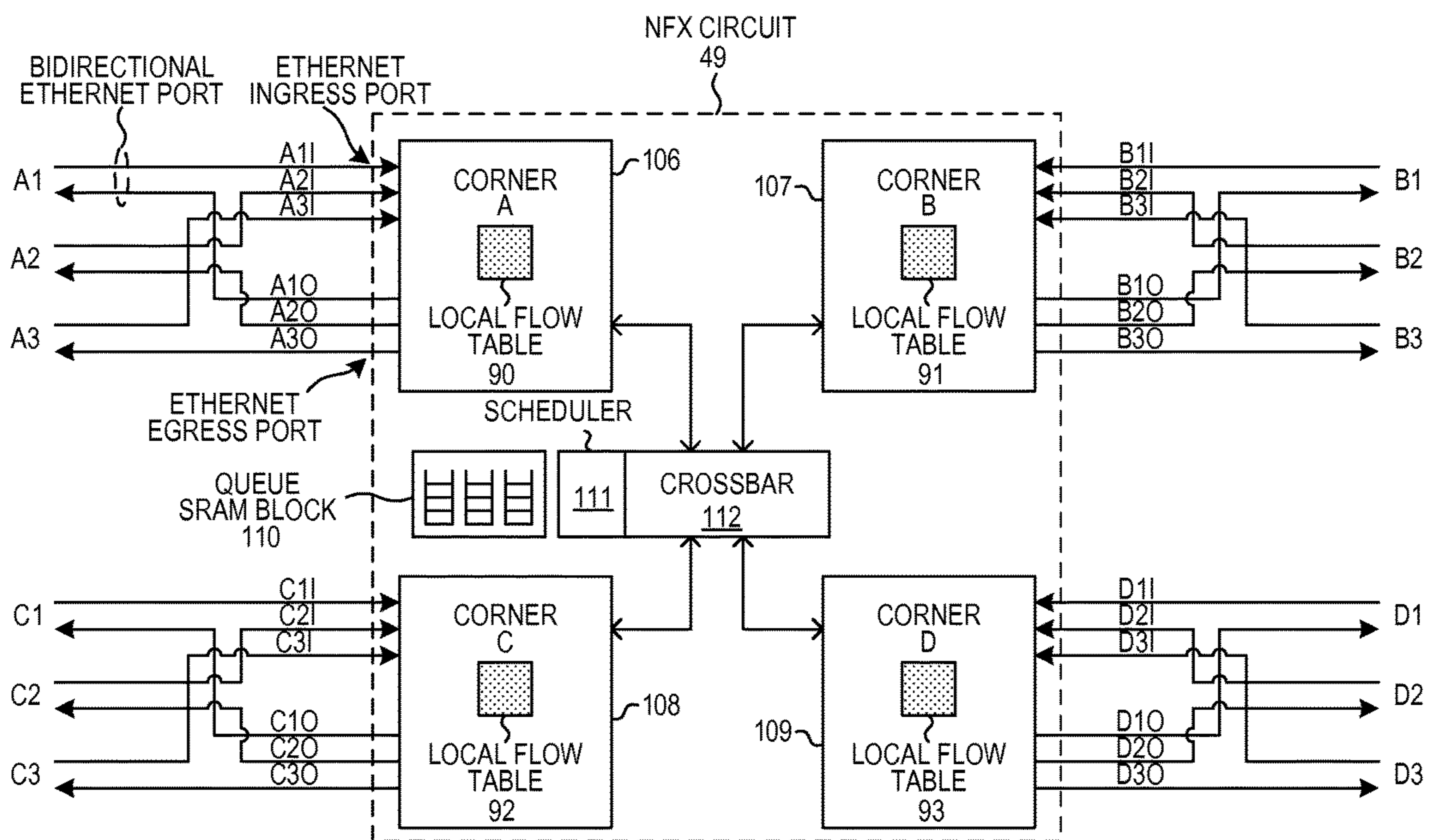
ONE NFX CIRCUIT
