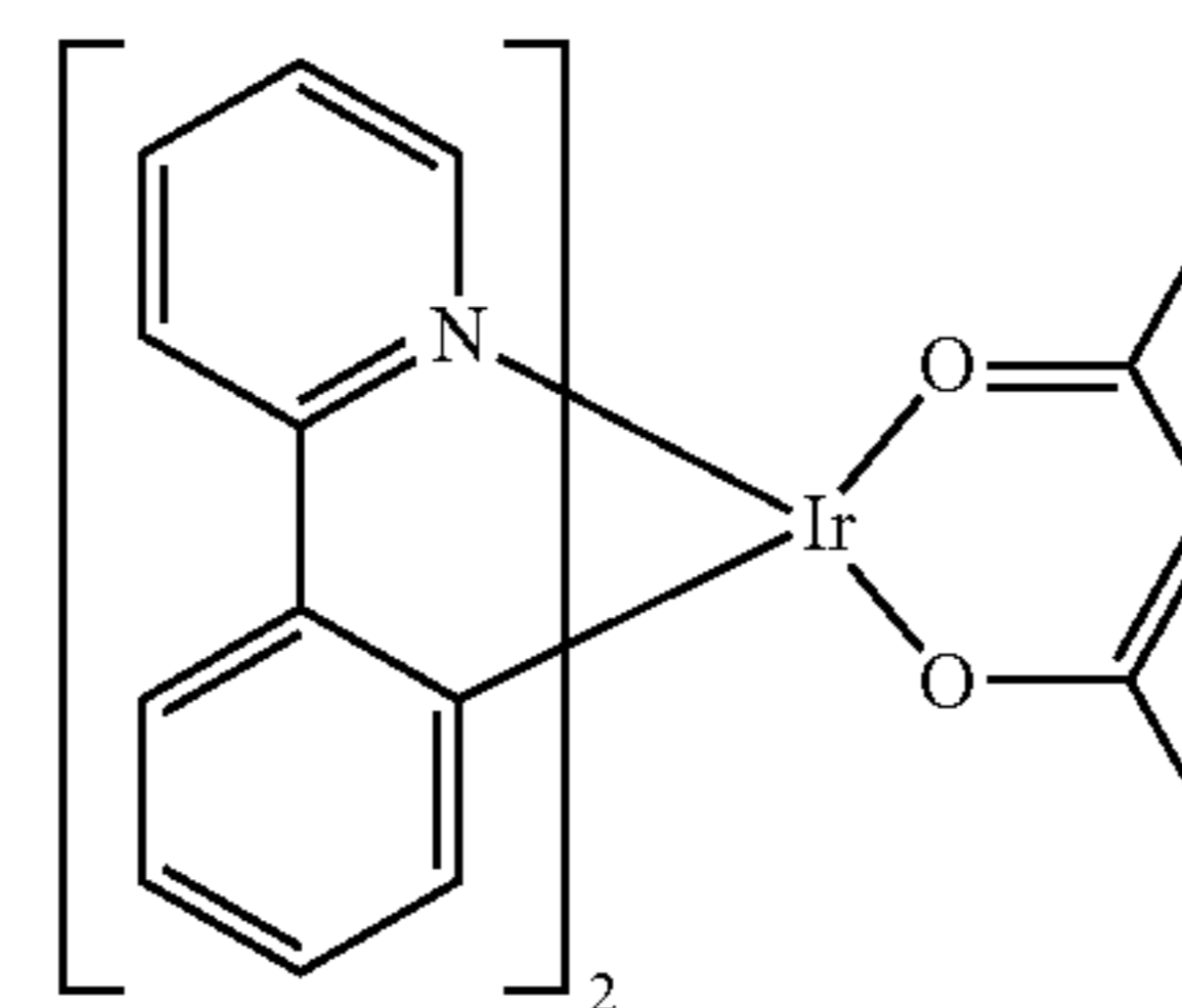
[[Ir(ppy) 2 (acac)]]
