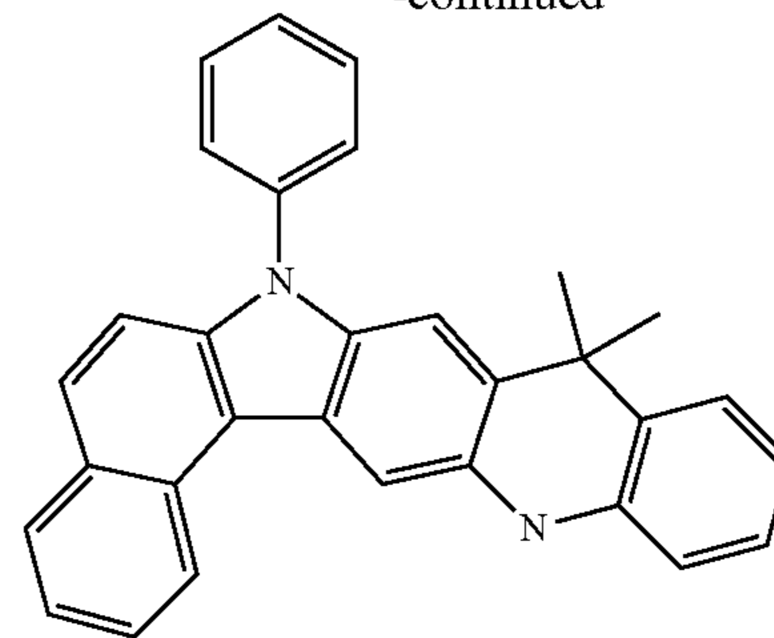
compound 5
