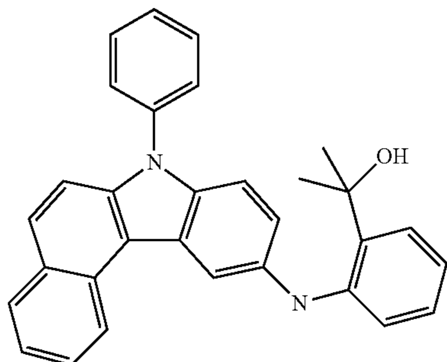
compound 4
