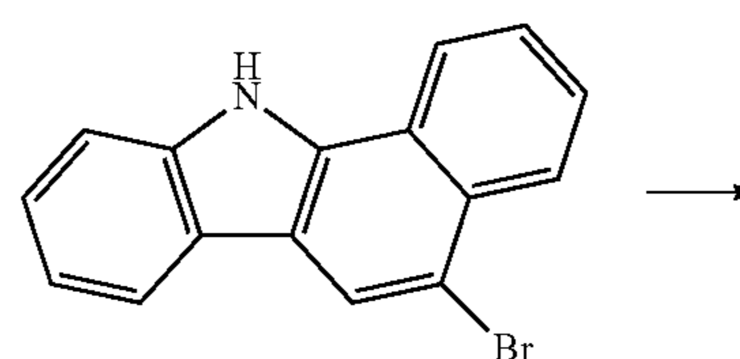
compound 1
