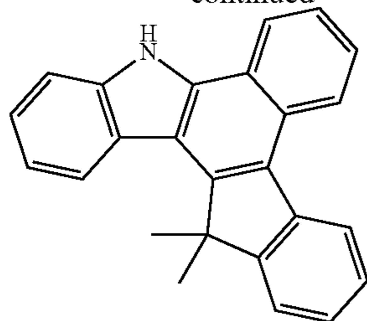
compound 3
