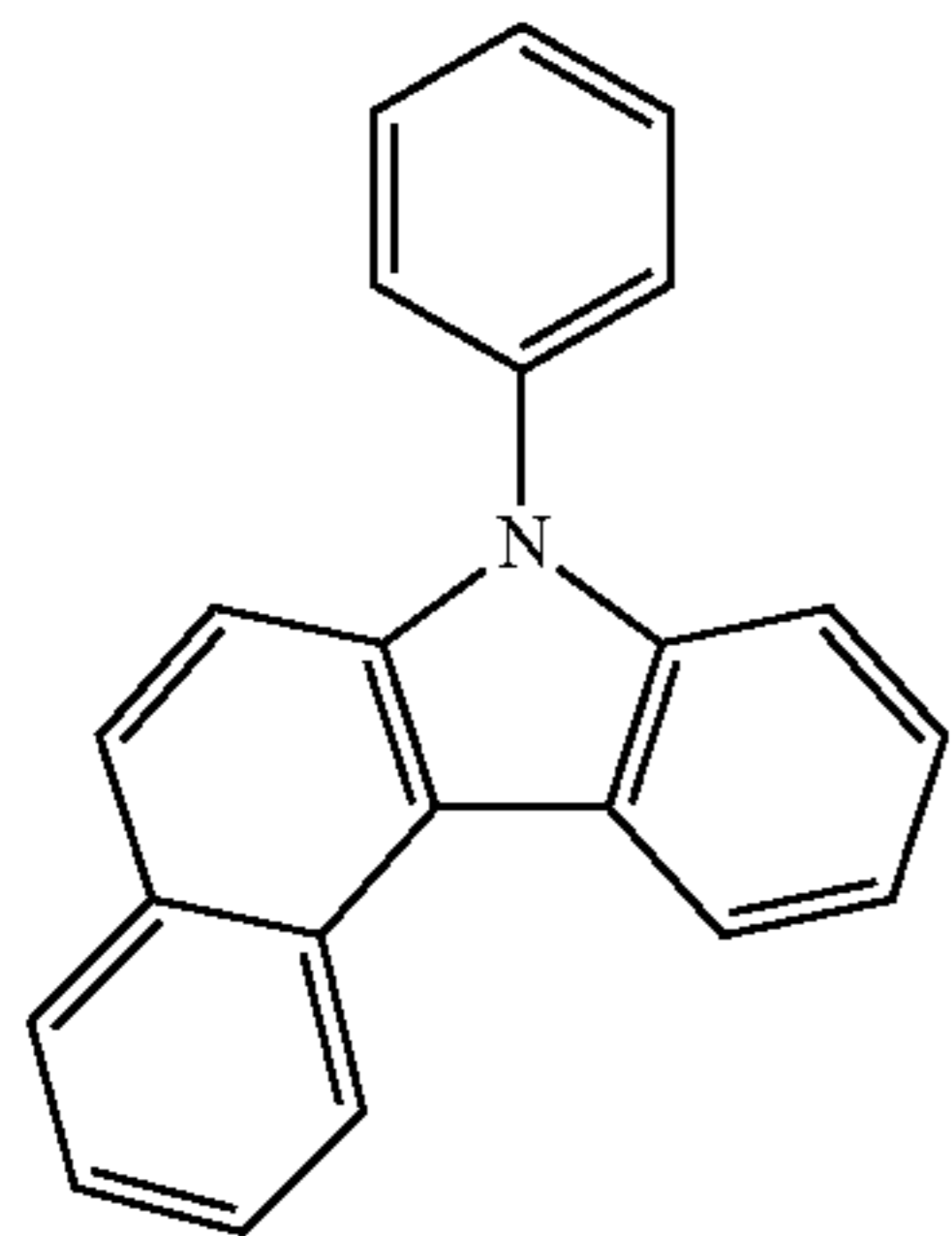
compound 1
