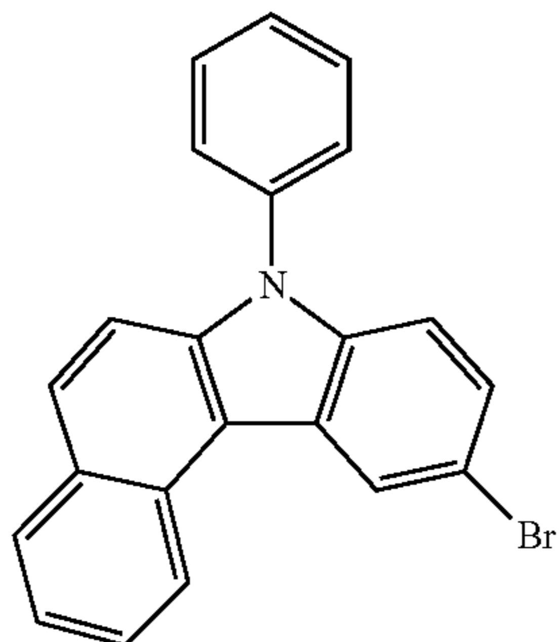
compound 2
