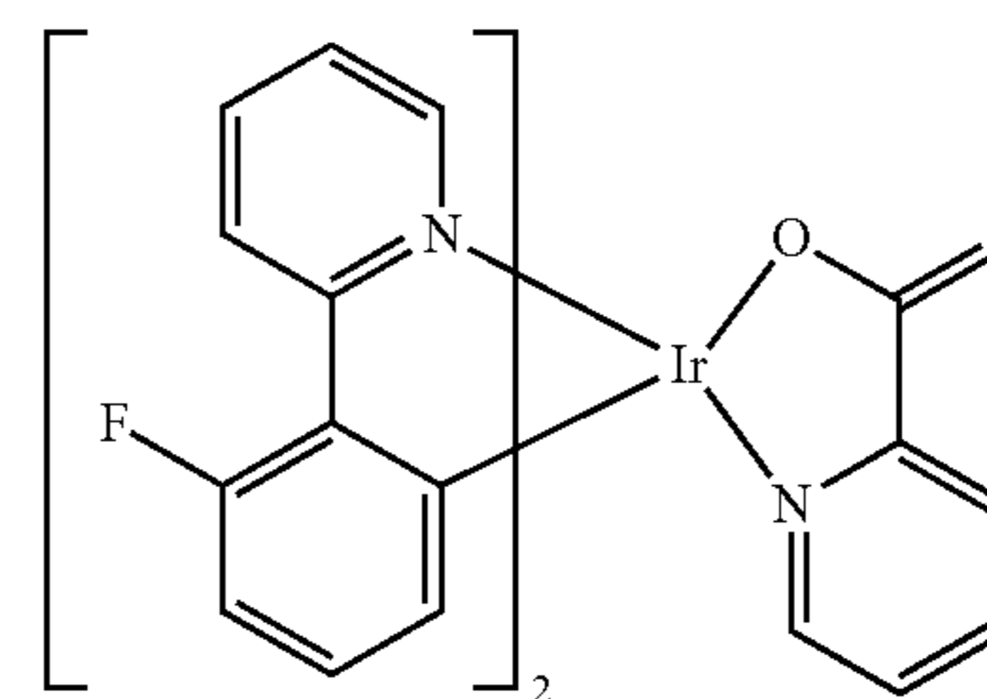
[F 2 Irpic]
