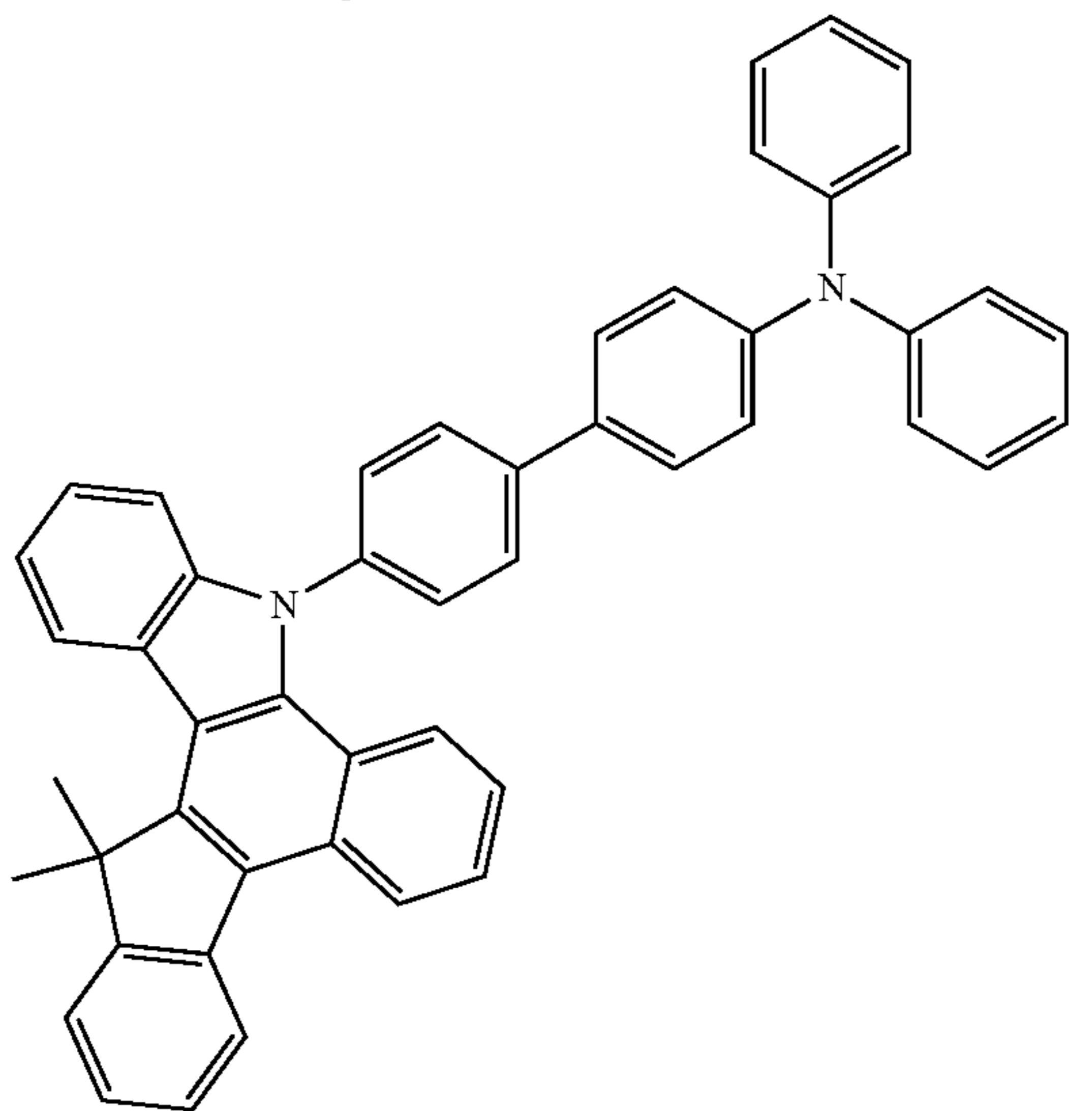
compound 3
