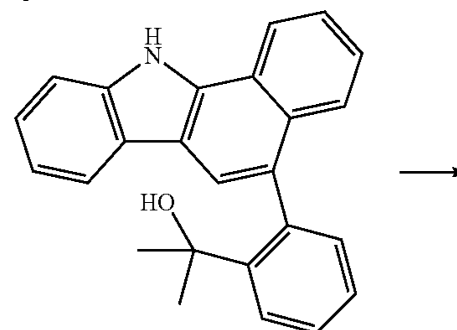
compound 2
