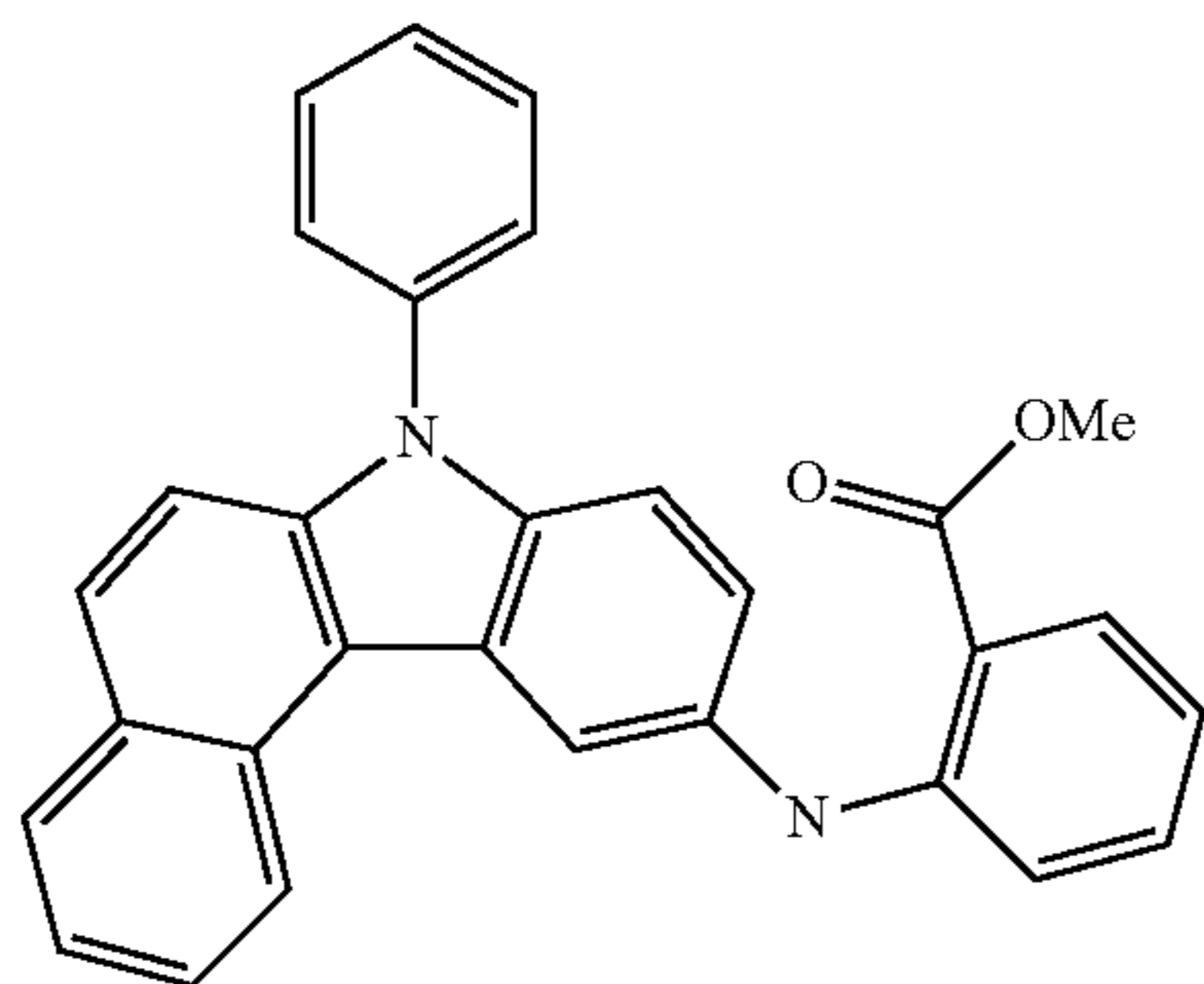
compound 3
