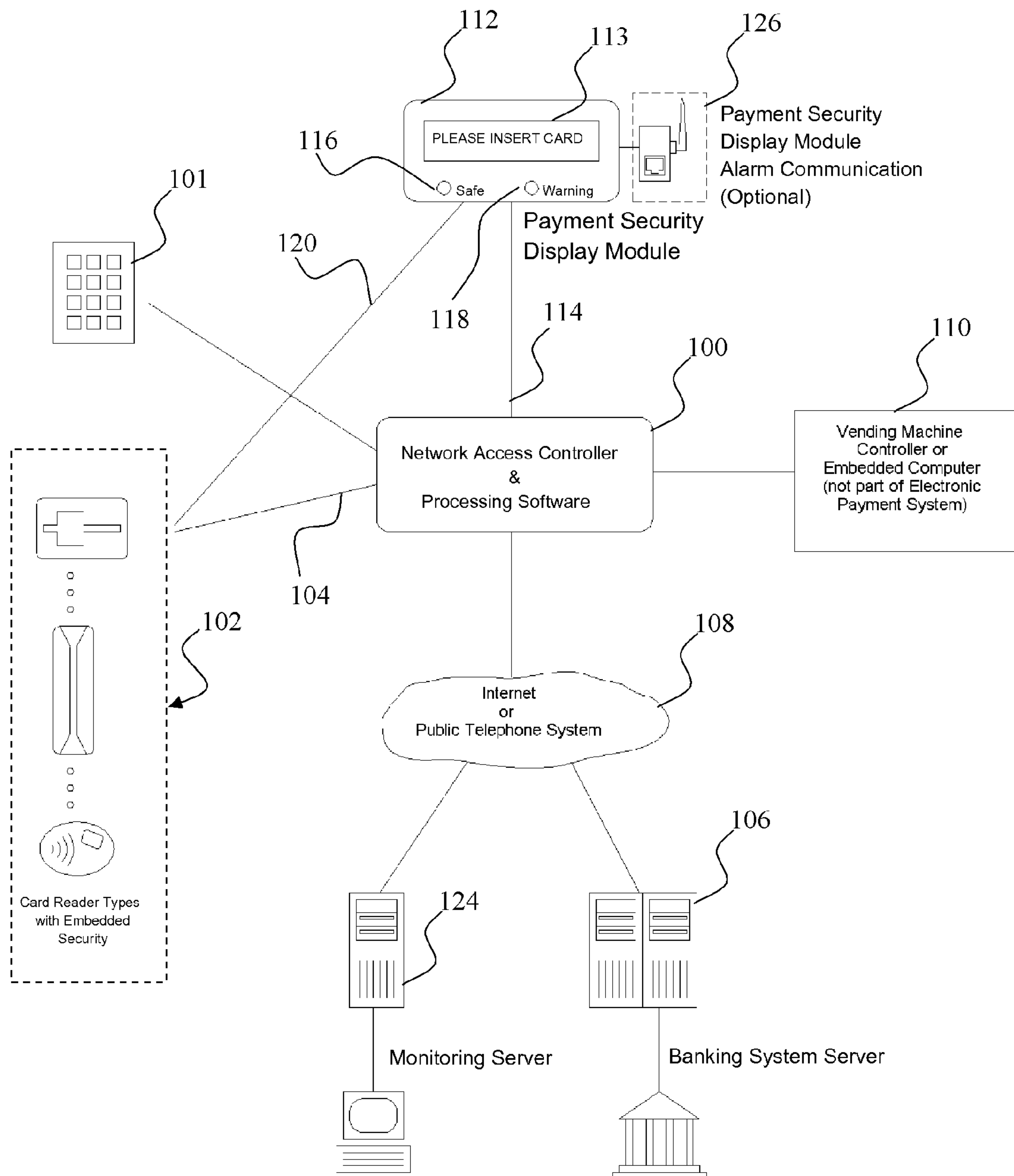
The Secure Electronic Payment System Block Diagram.
