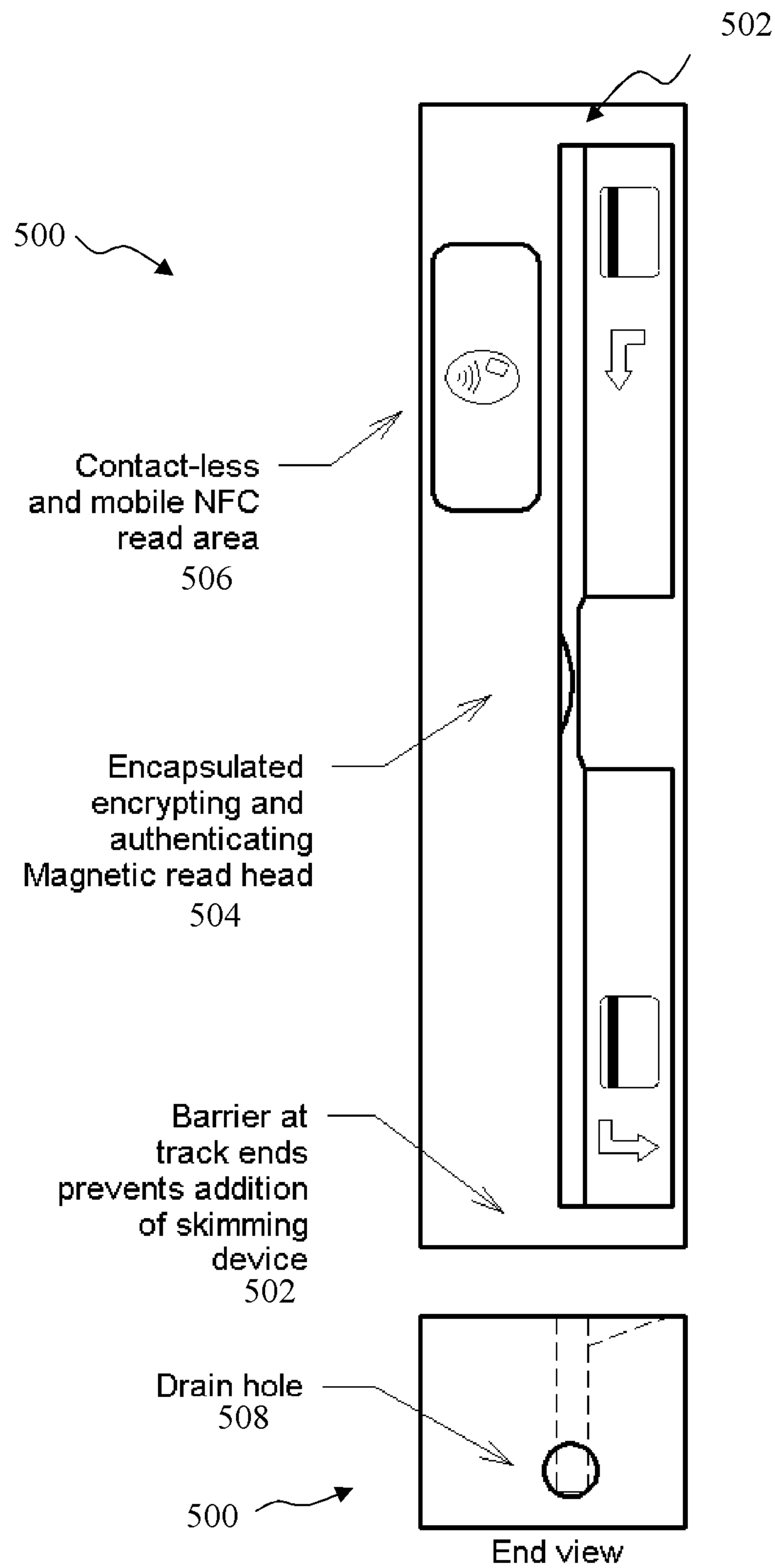
Secure Swipe Reader FIG. 12B
