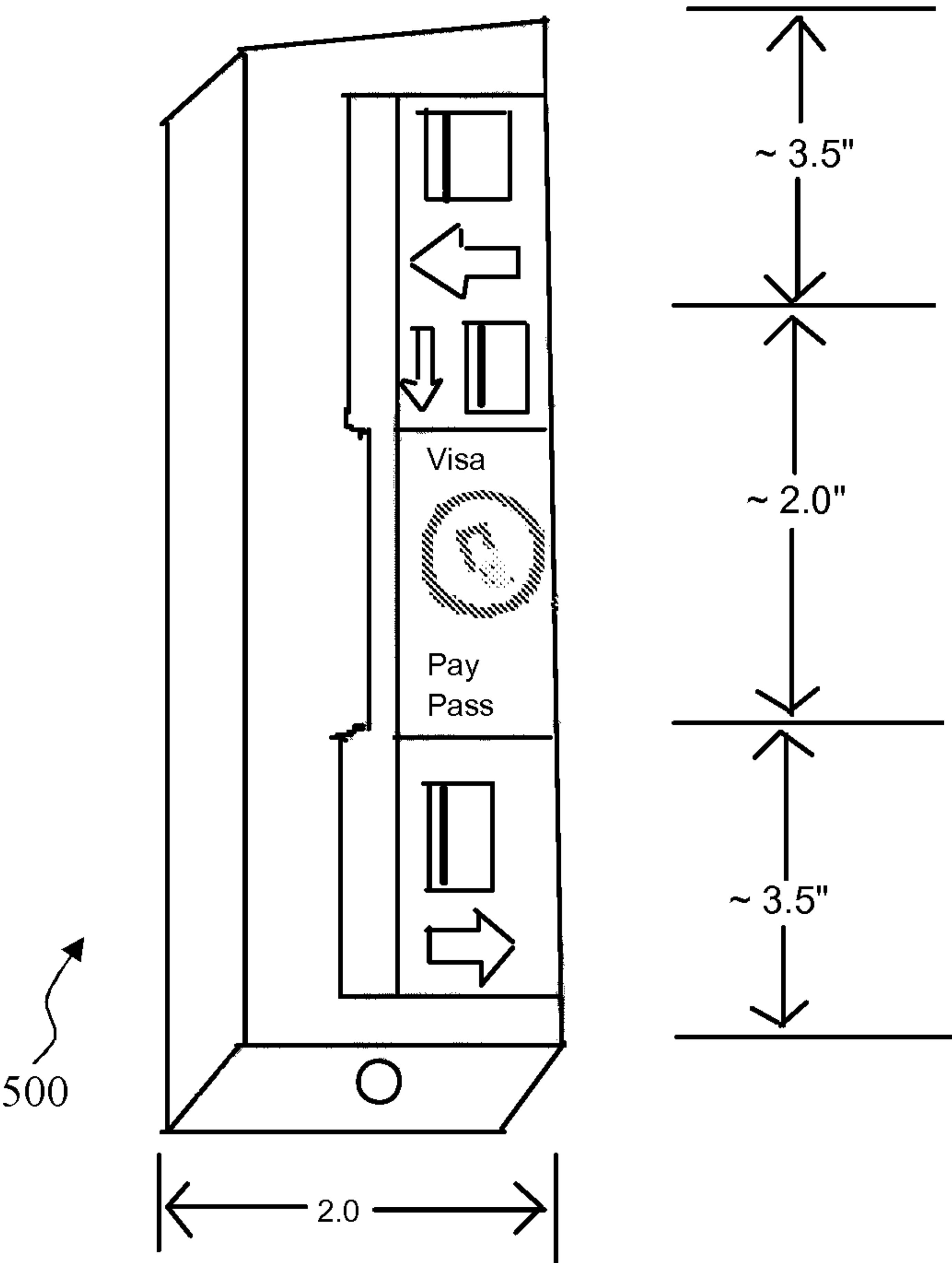
SKIMMING - RESISTANT SWIPE CARD READER
