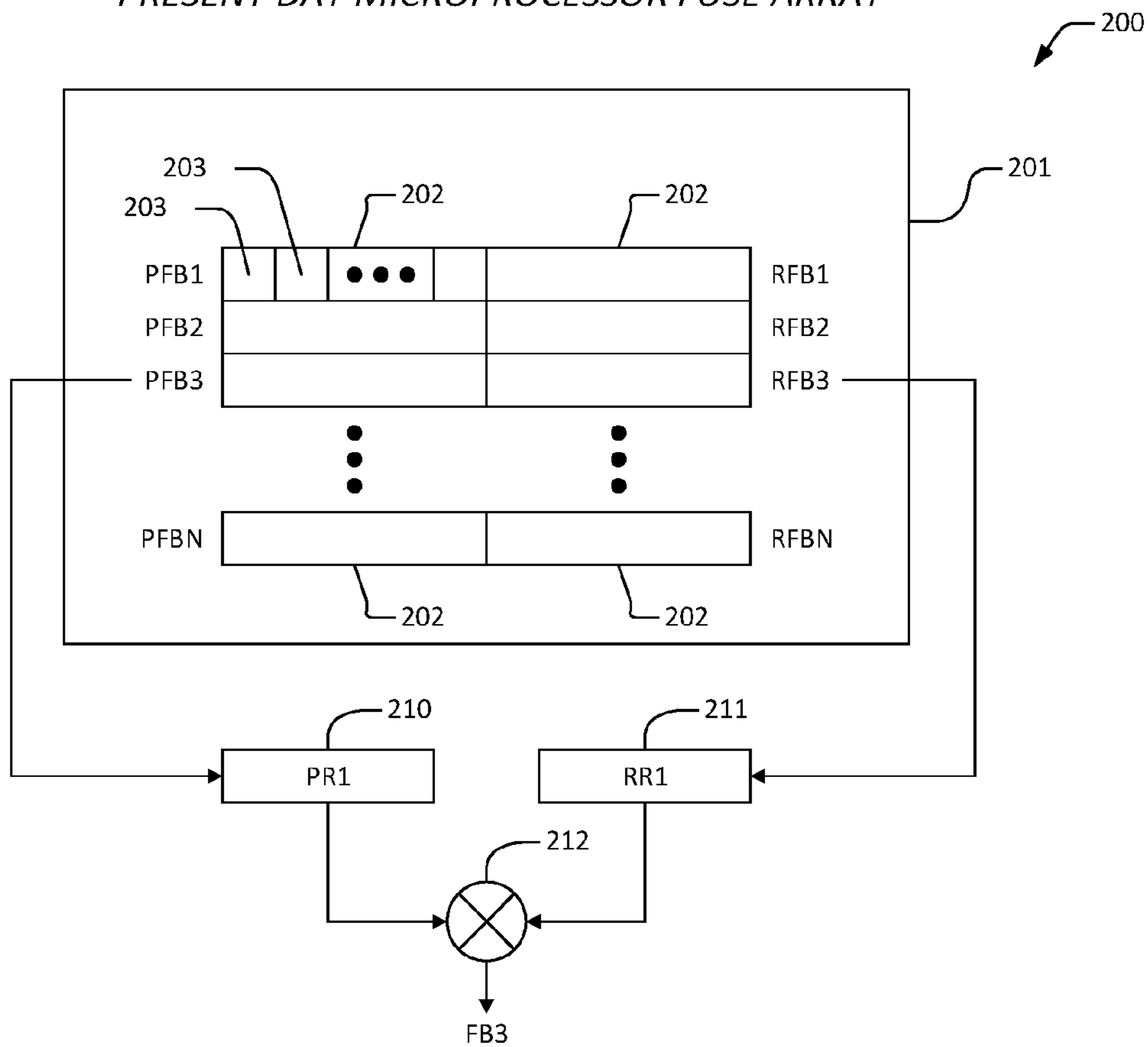
FIG. 2 (Prior Art)
