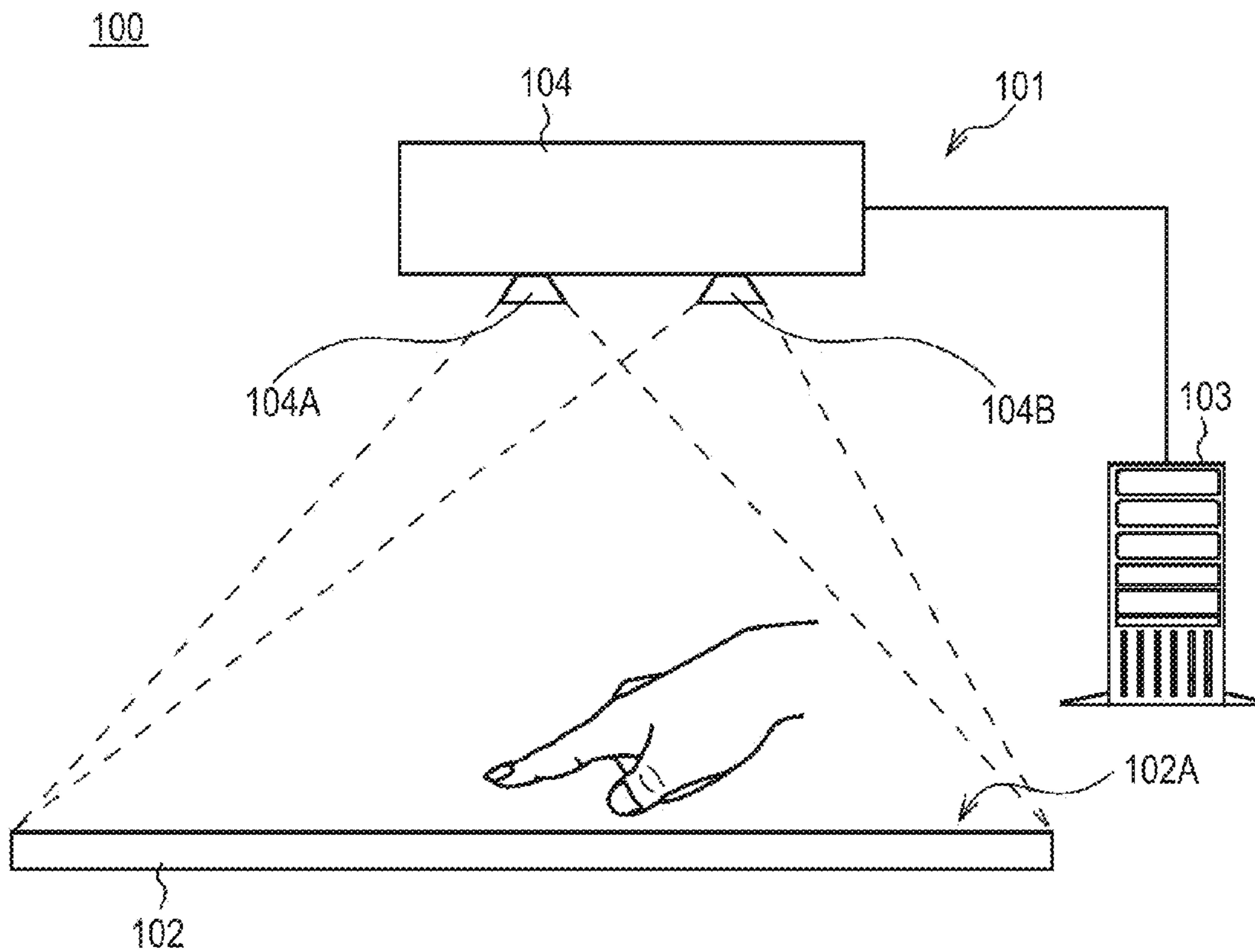
CONFIGURATION OF IMAGE PROJECTION SYSTEM
