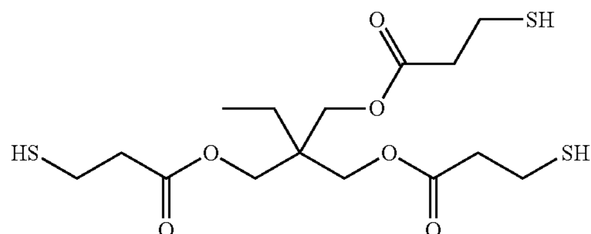
Chemical Formula 1-2
