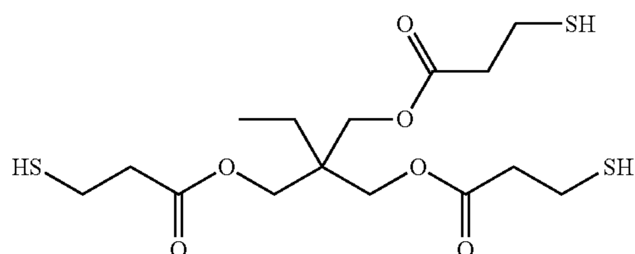
Chemical Formula 1-2
