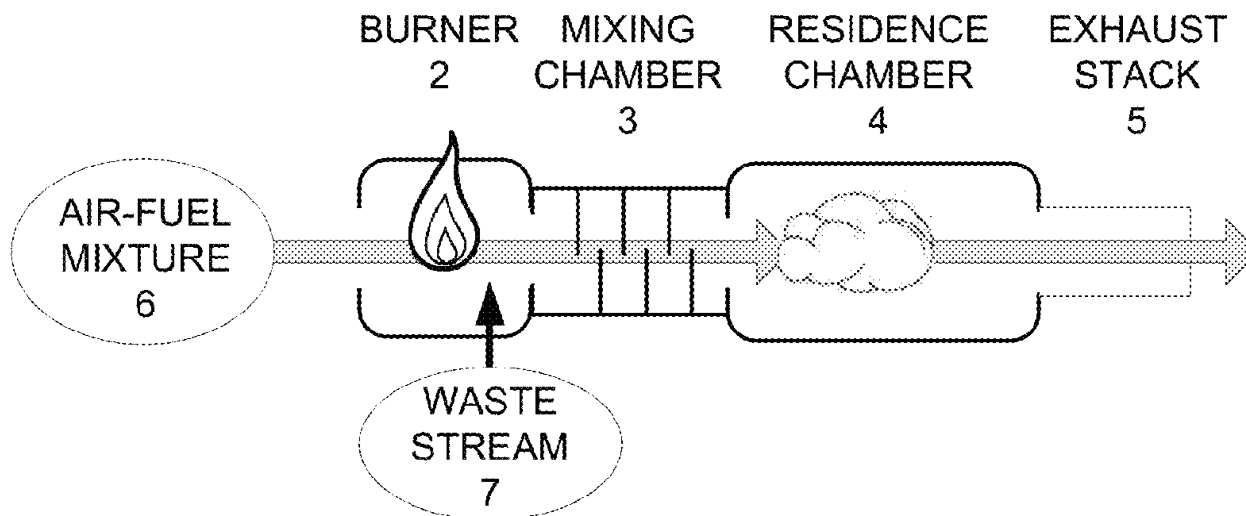
FIG. 1-1A PRIOR ART
