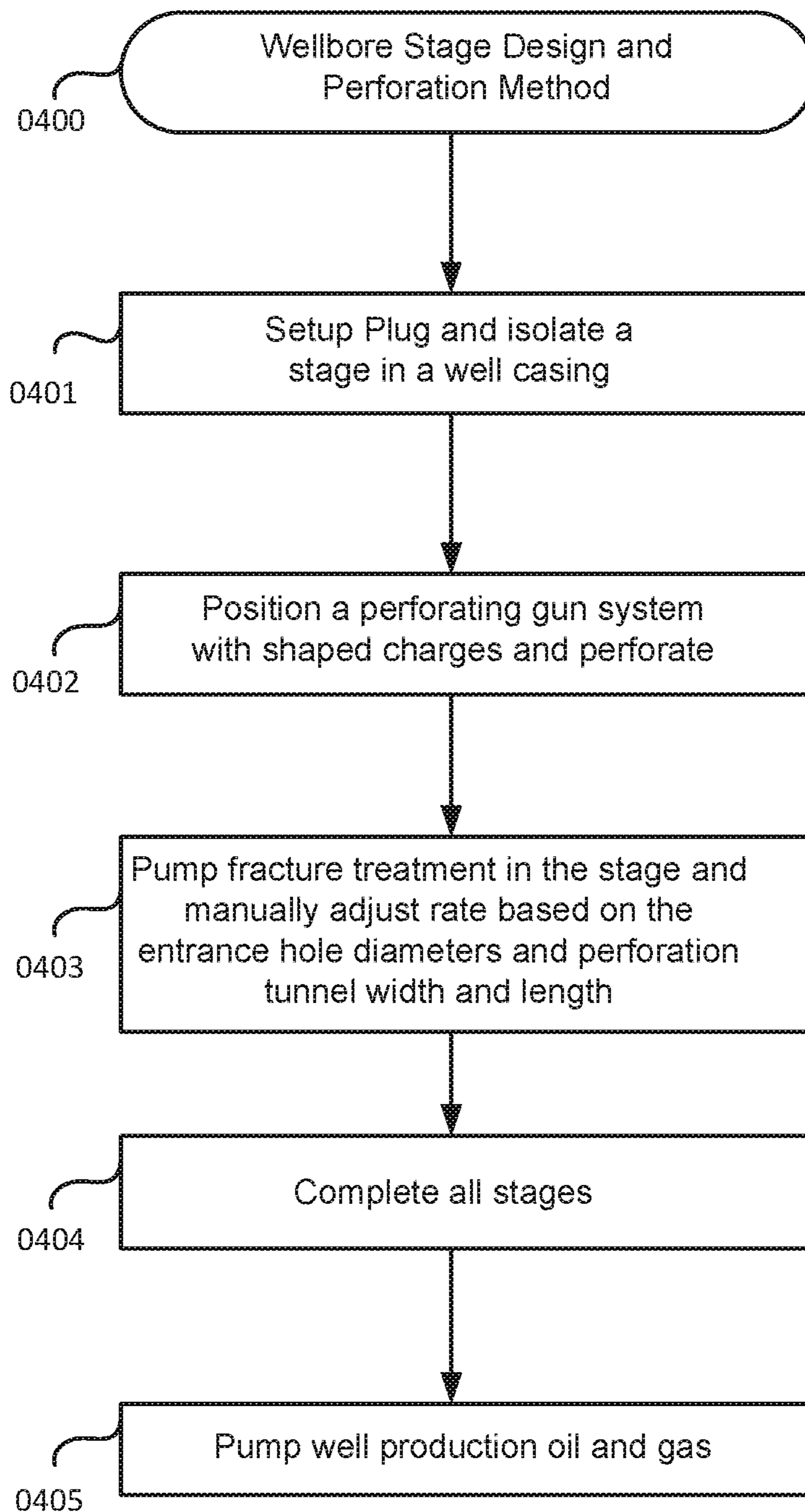
FIG.4 Prior Art
