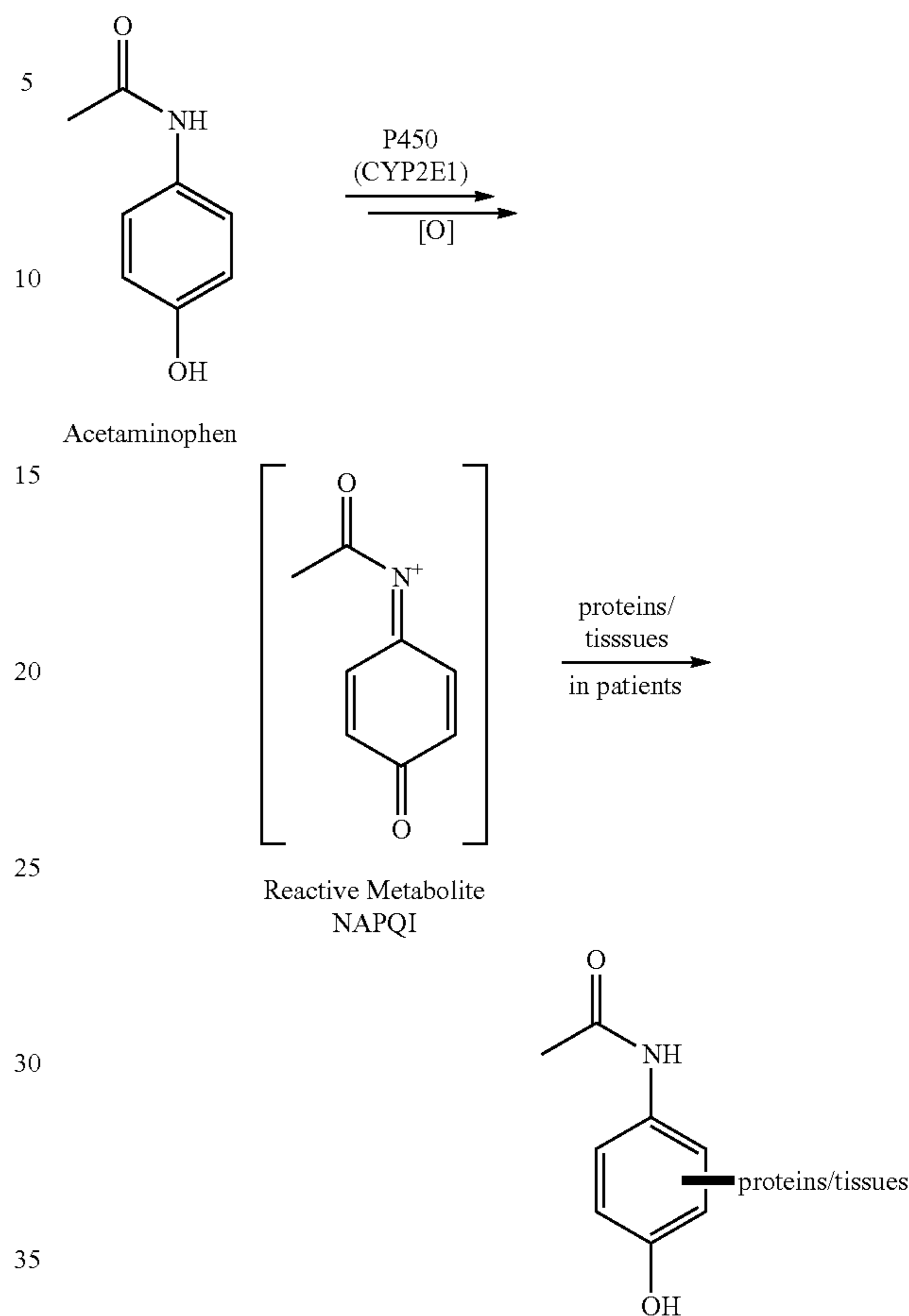
Scheme 10
