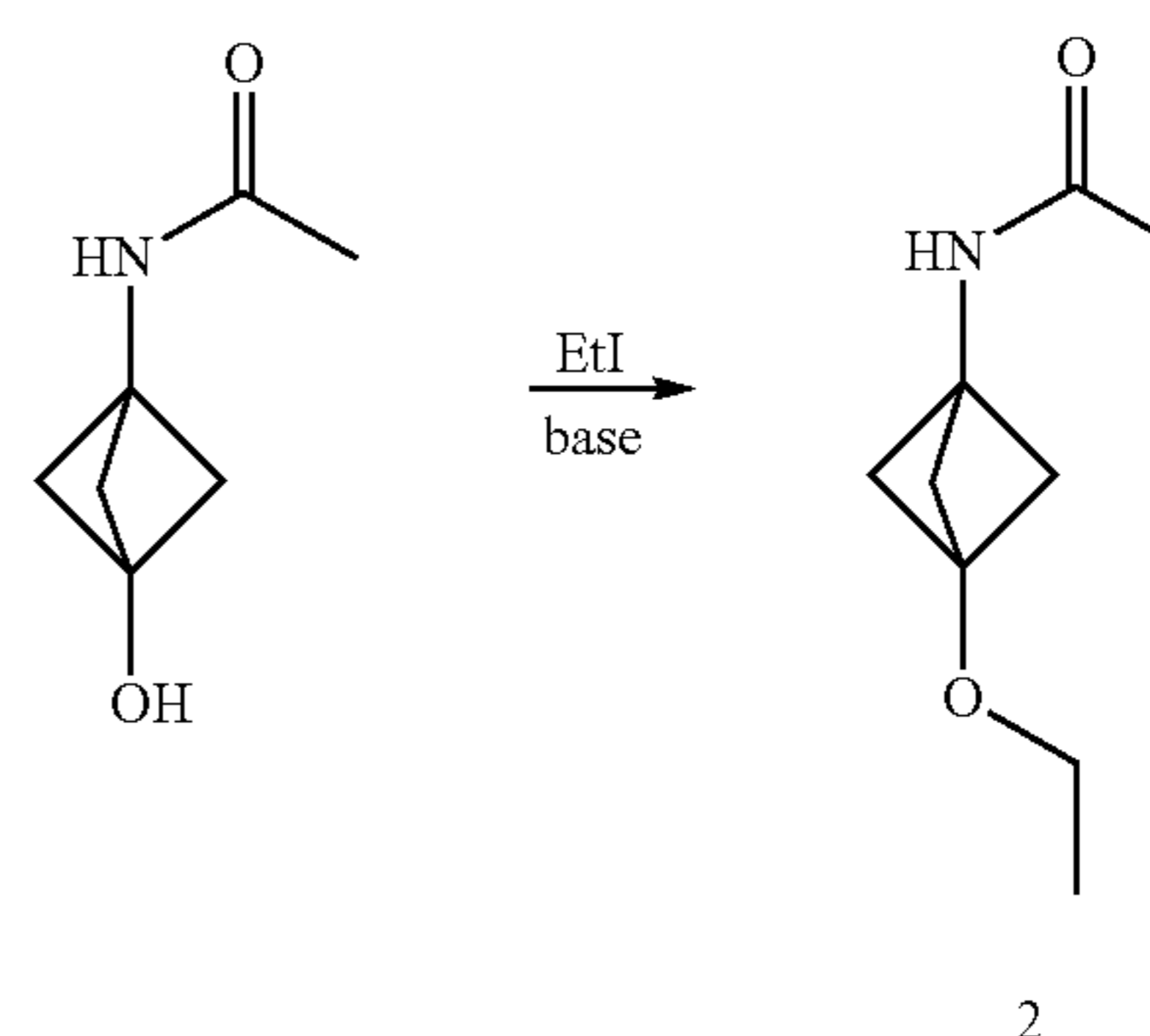
Scheme 5
