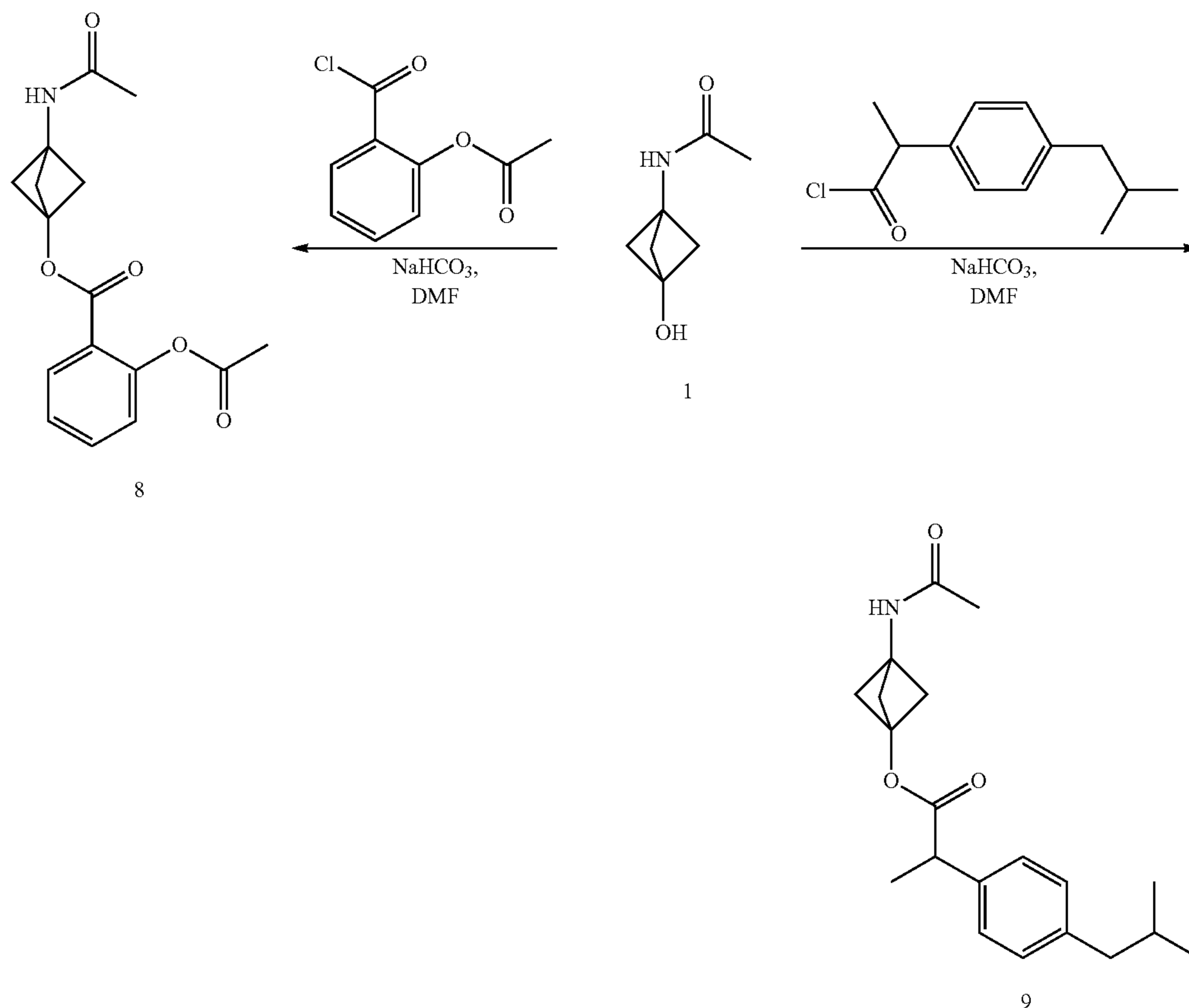
Scheme 9
