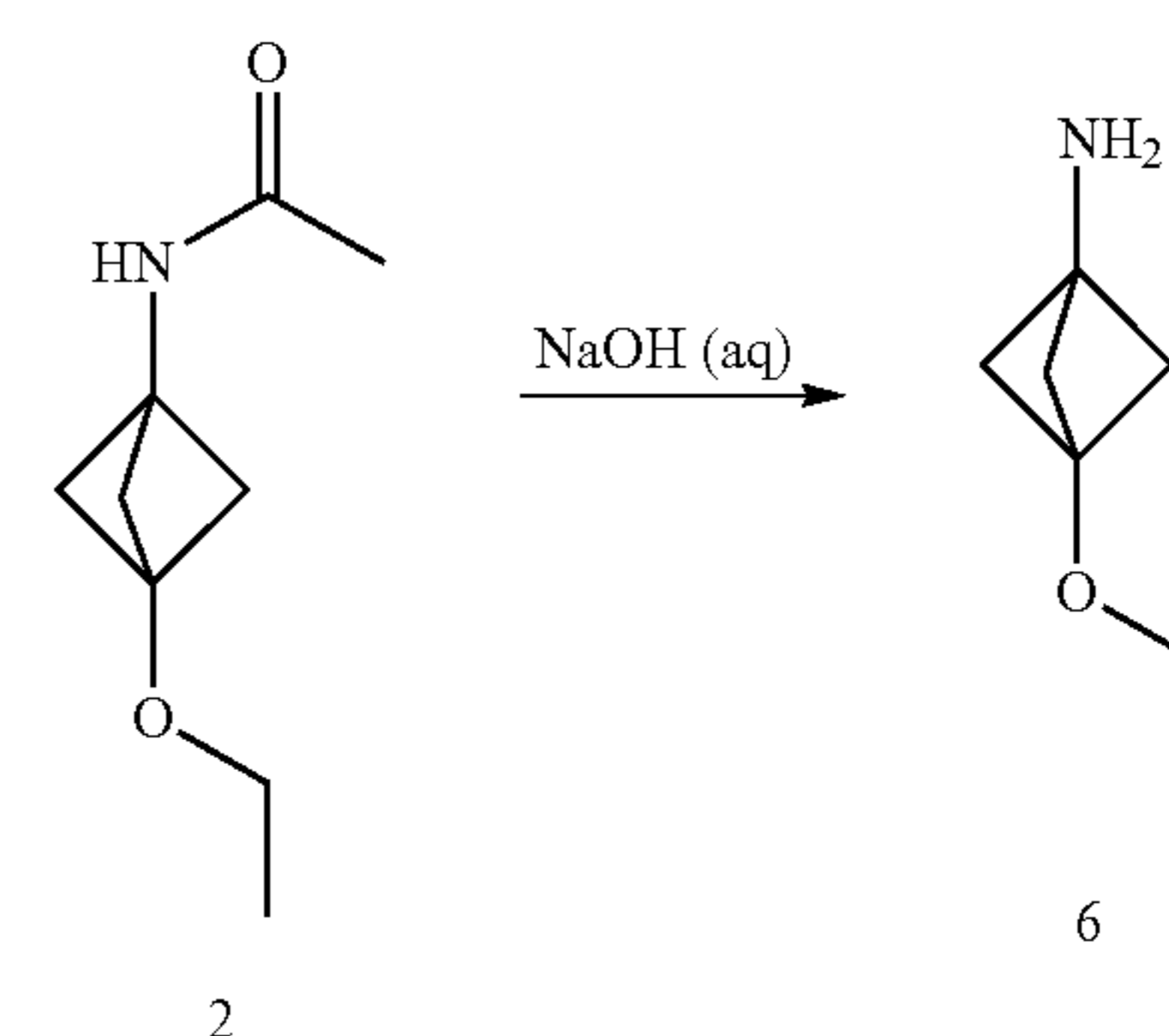
Scheme 6
