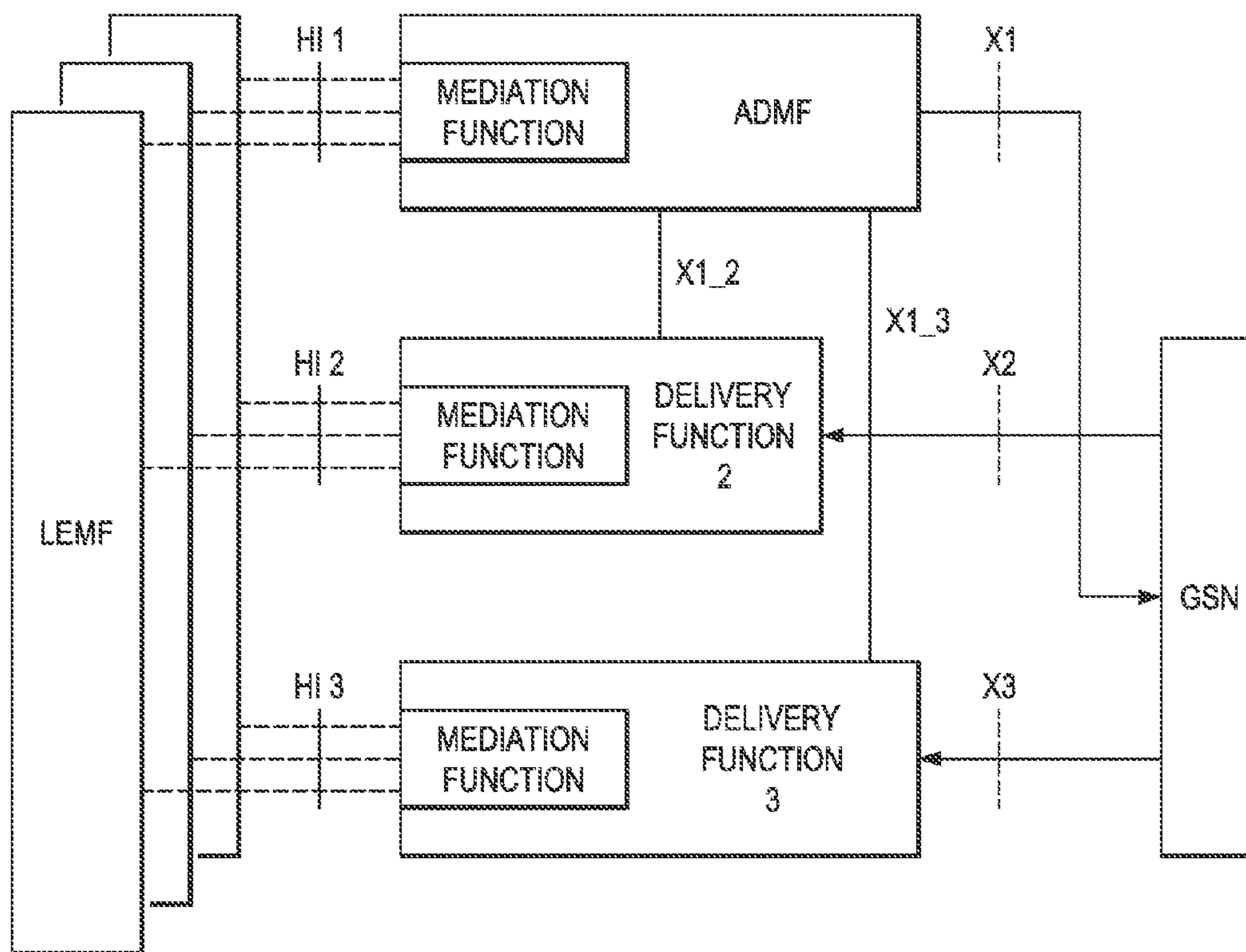
FIG. 16 (PRIOR ART)
