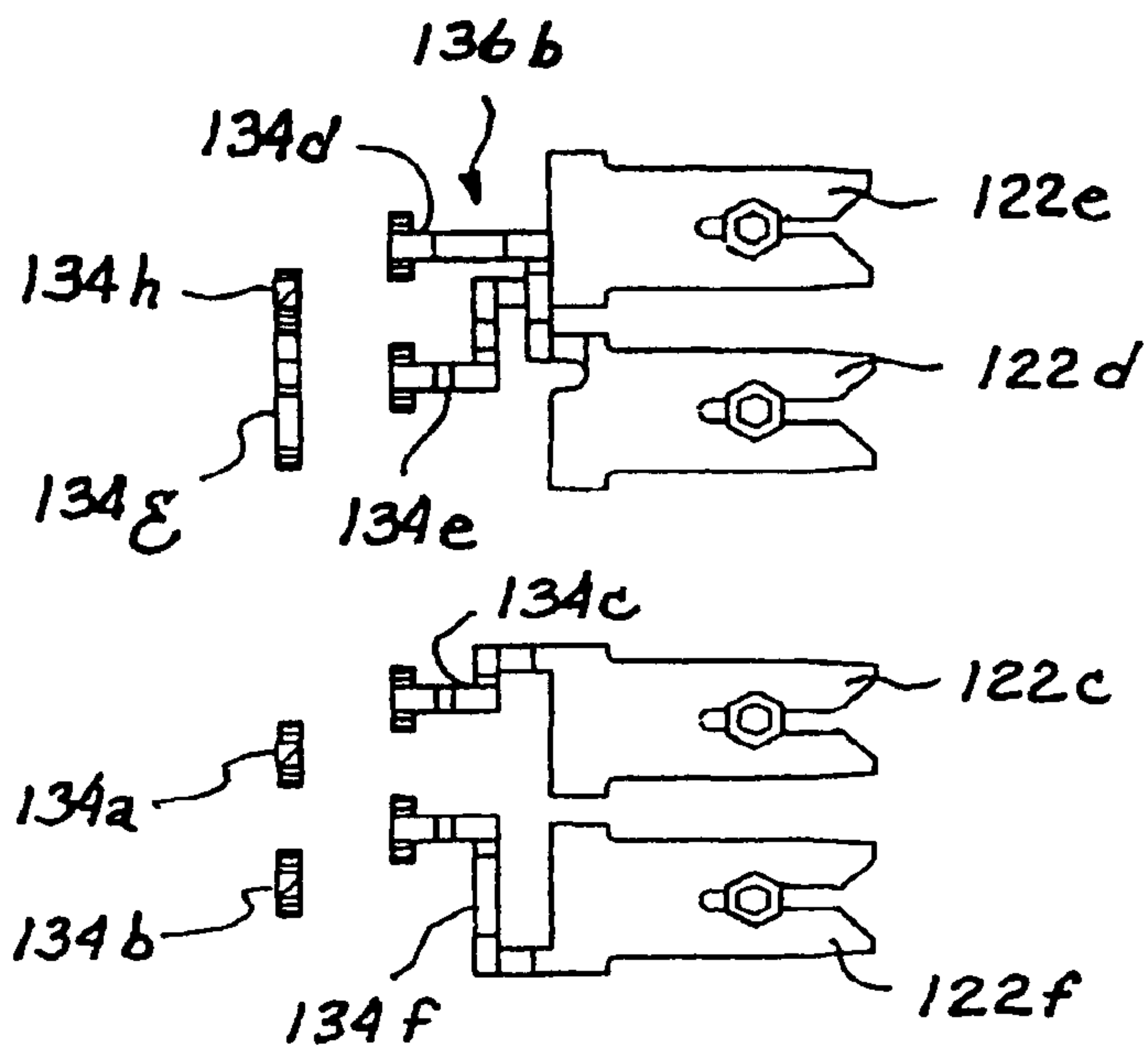
SECTION Q-Q
