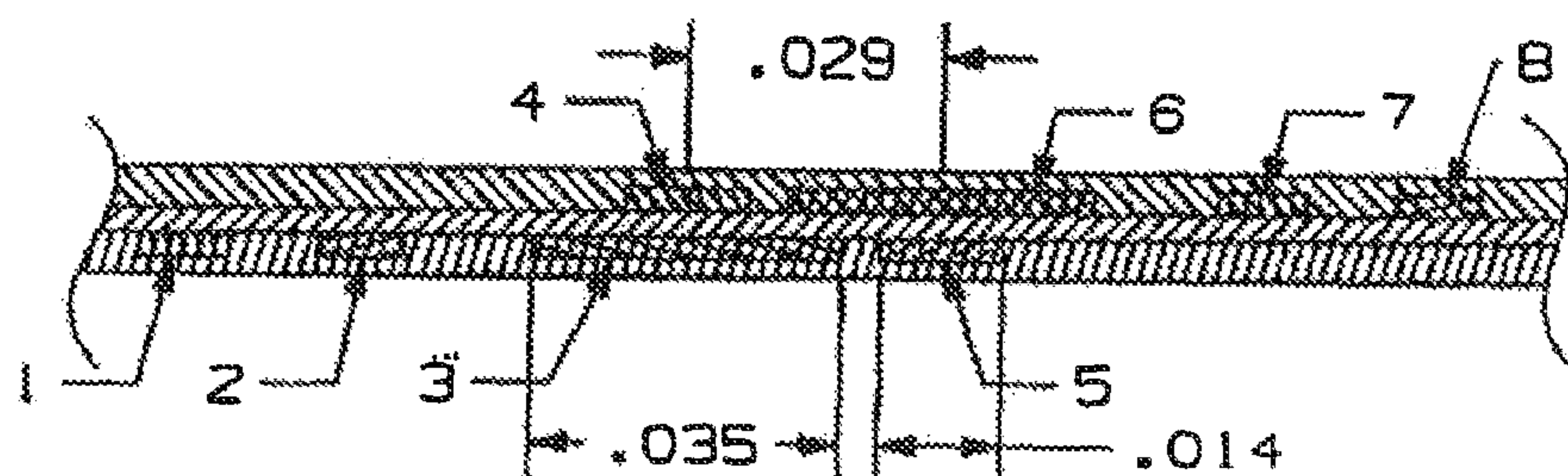
SECTION E-E
