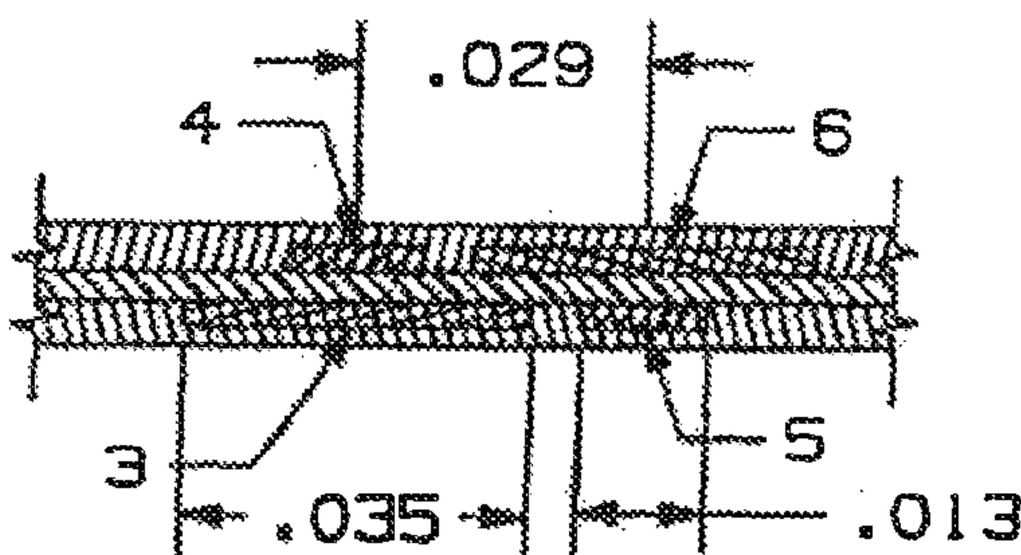
SECTION F-F
