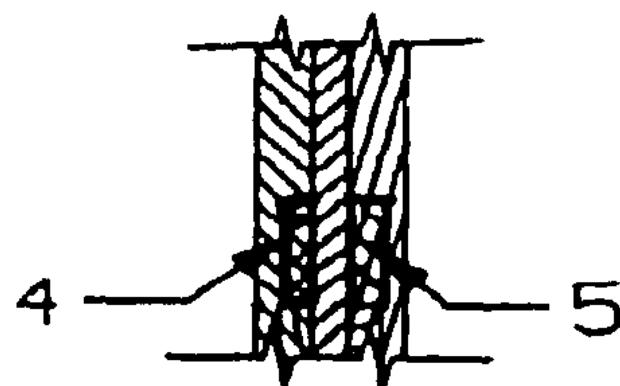
SECTION I-I
