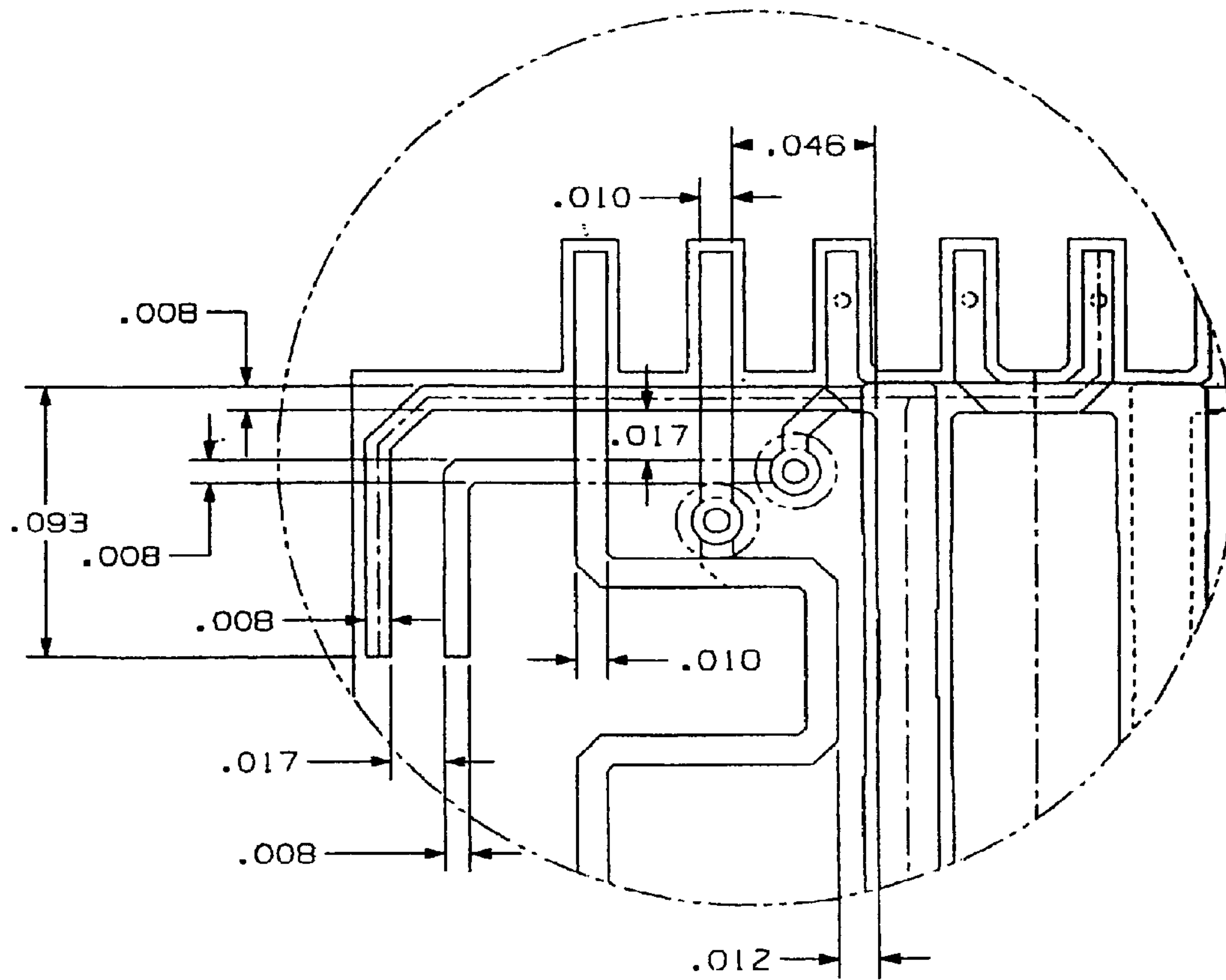
DETAIL M
