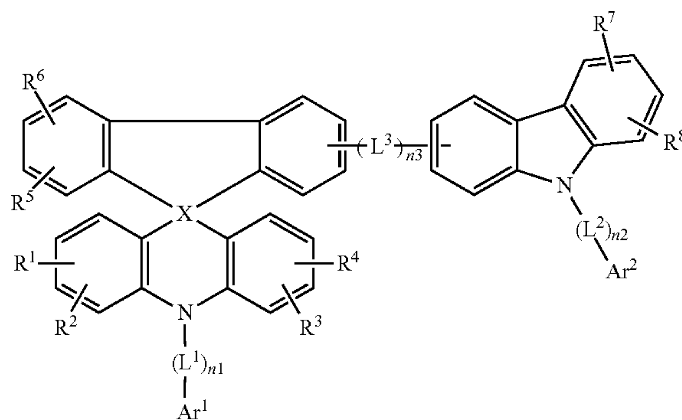
[Chemical Formula 2]
