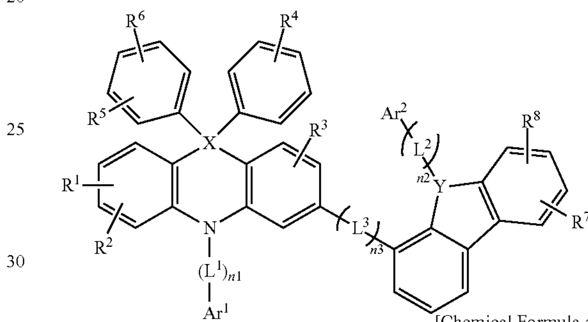
[Chemical Formula 4-1]
