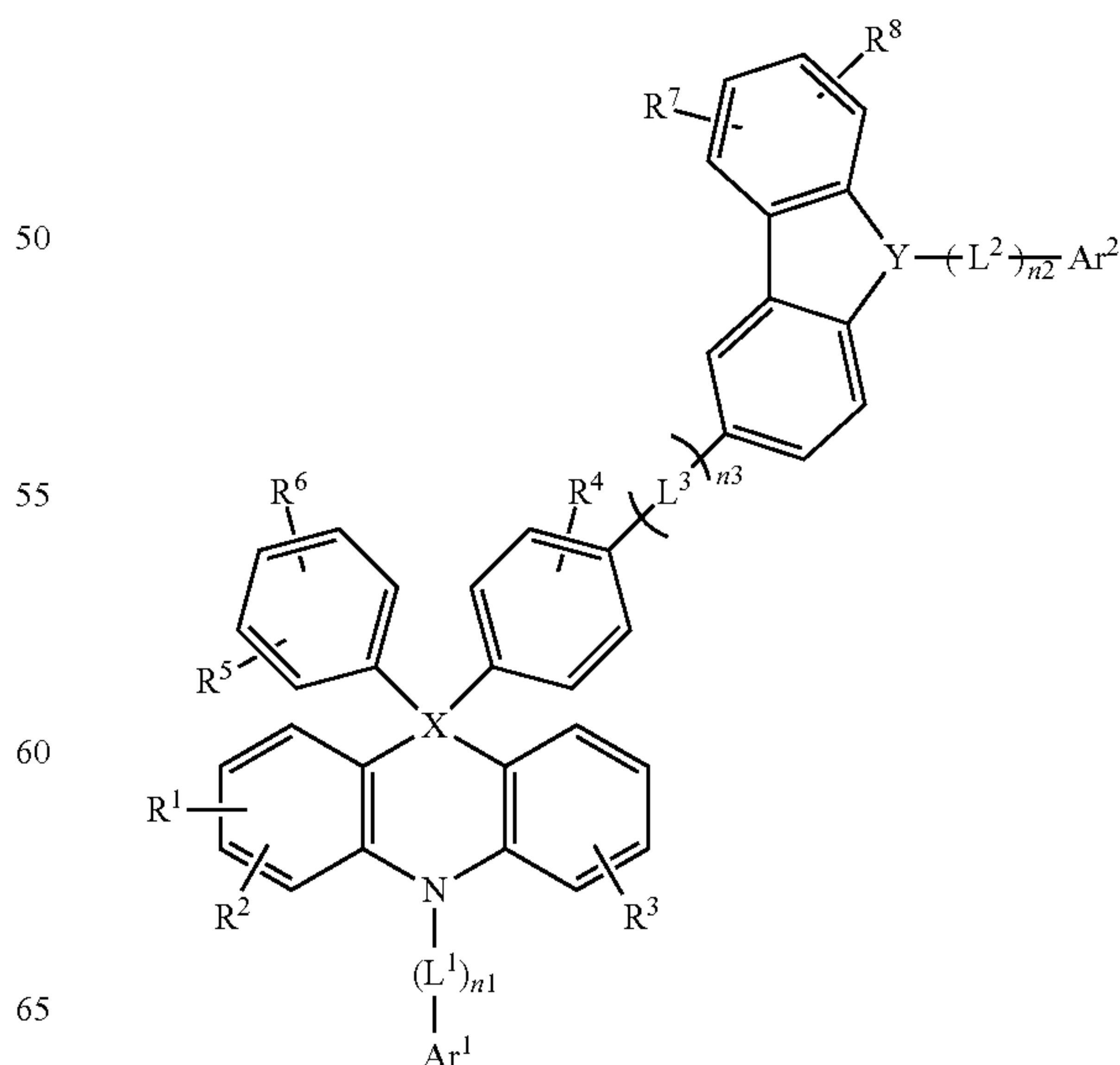
[Chemical Formula 1-4]
