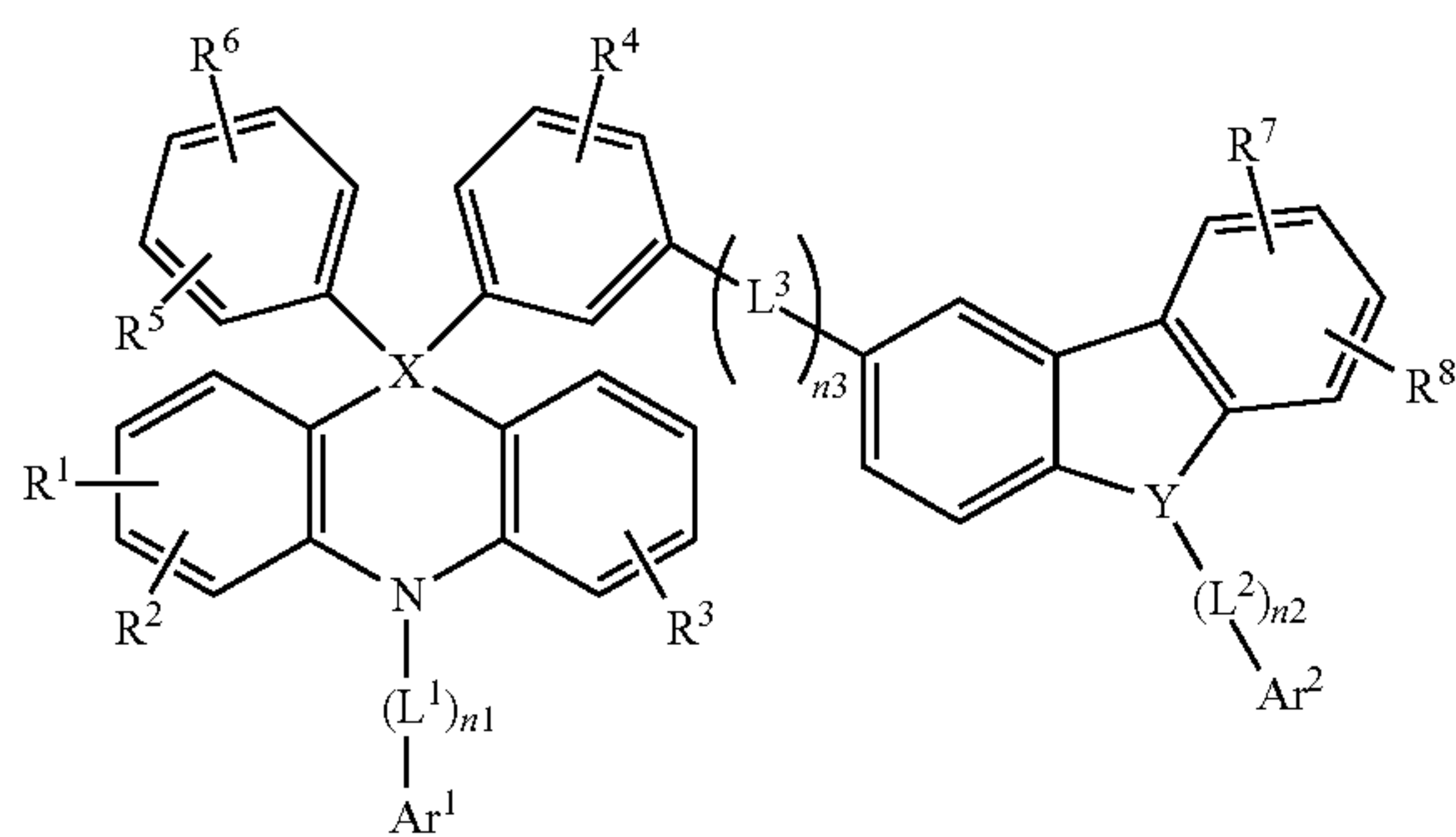
[Chemical Formula 1-1]
