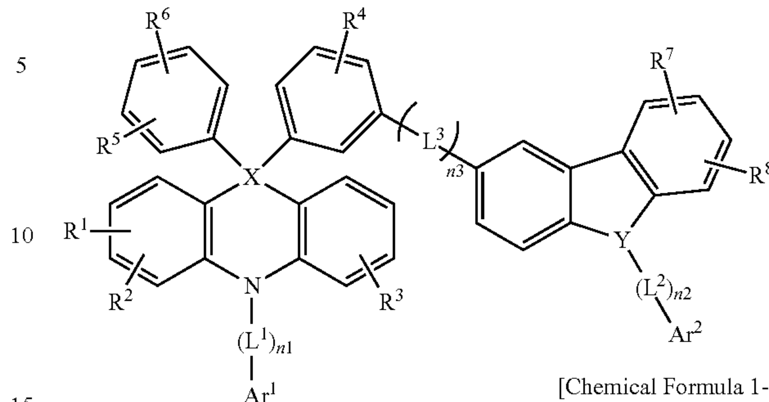
[Chemical Formula 1-1]
