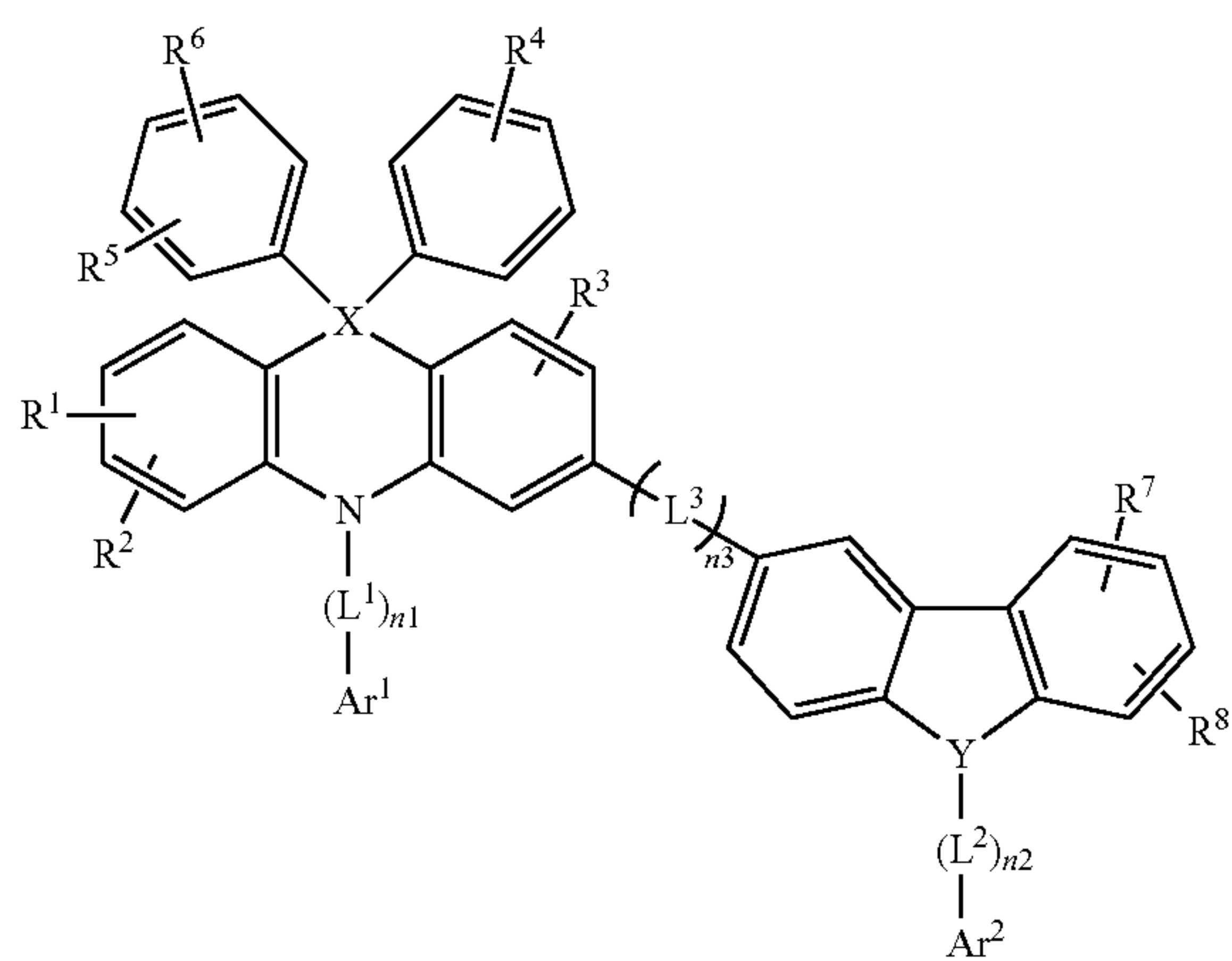
[Chemical Formula 3-1]
