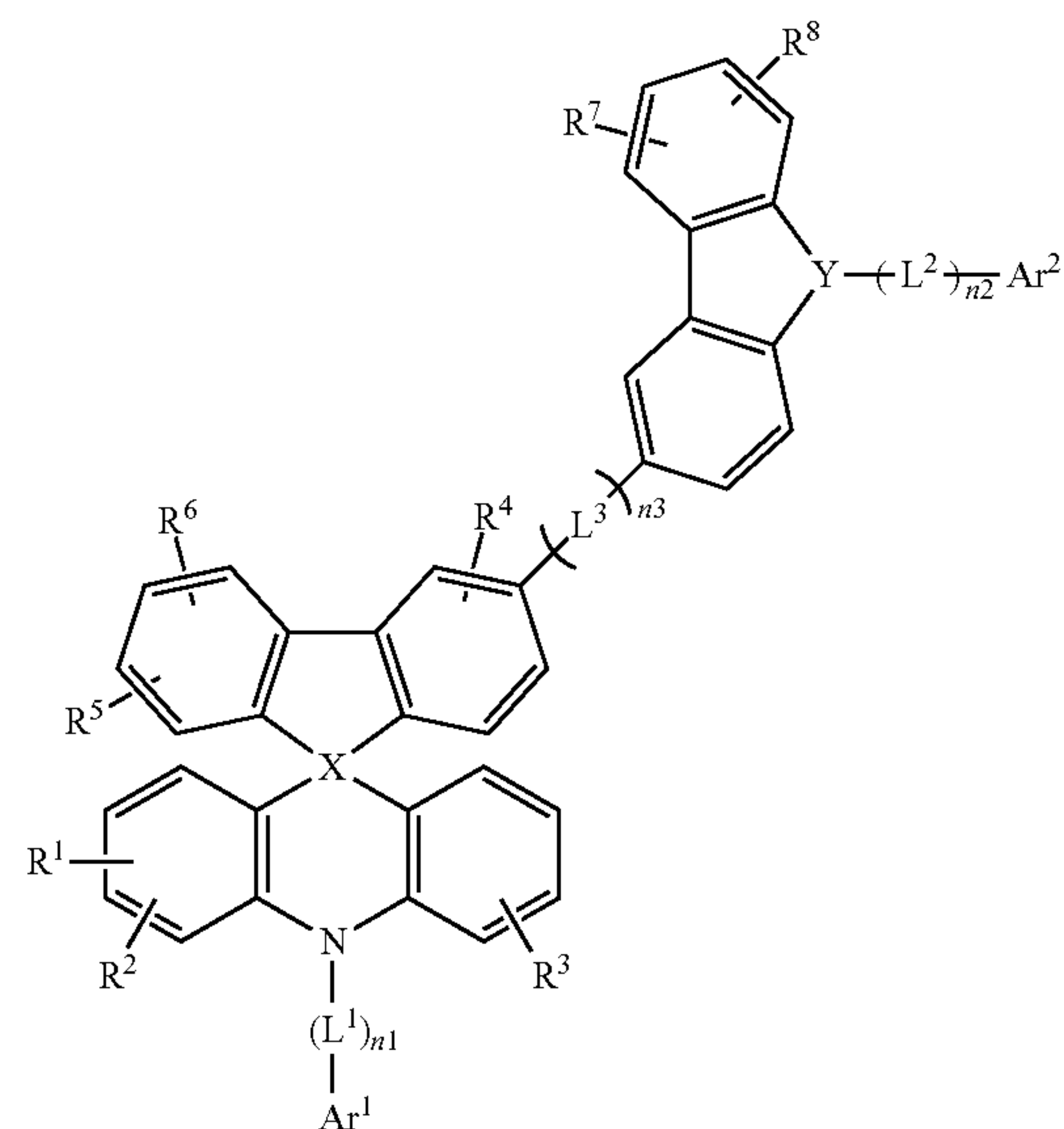
[Chemical Formula 2-4]
