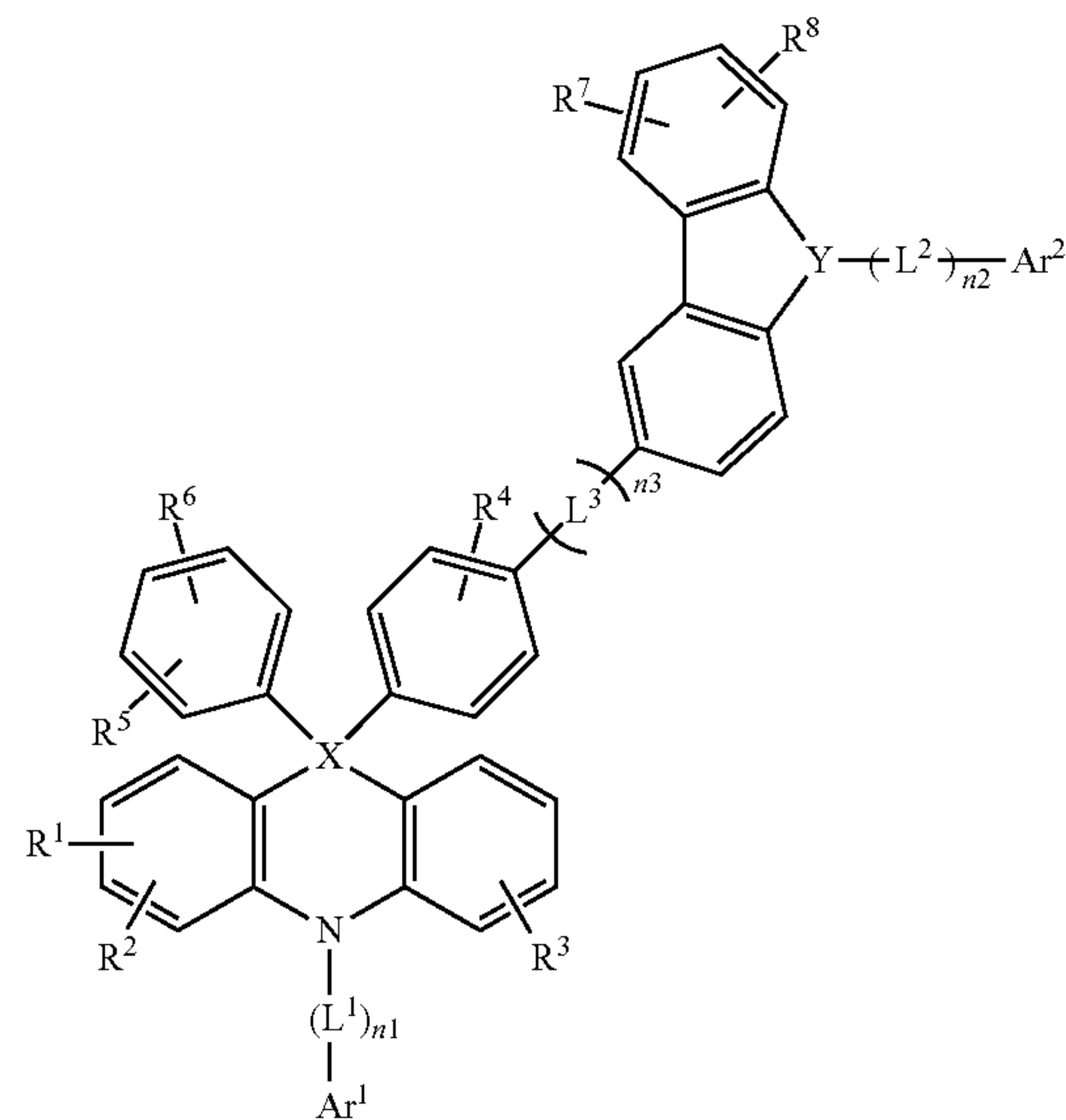
[Chemical Formula 1-4]
