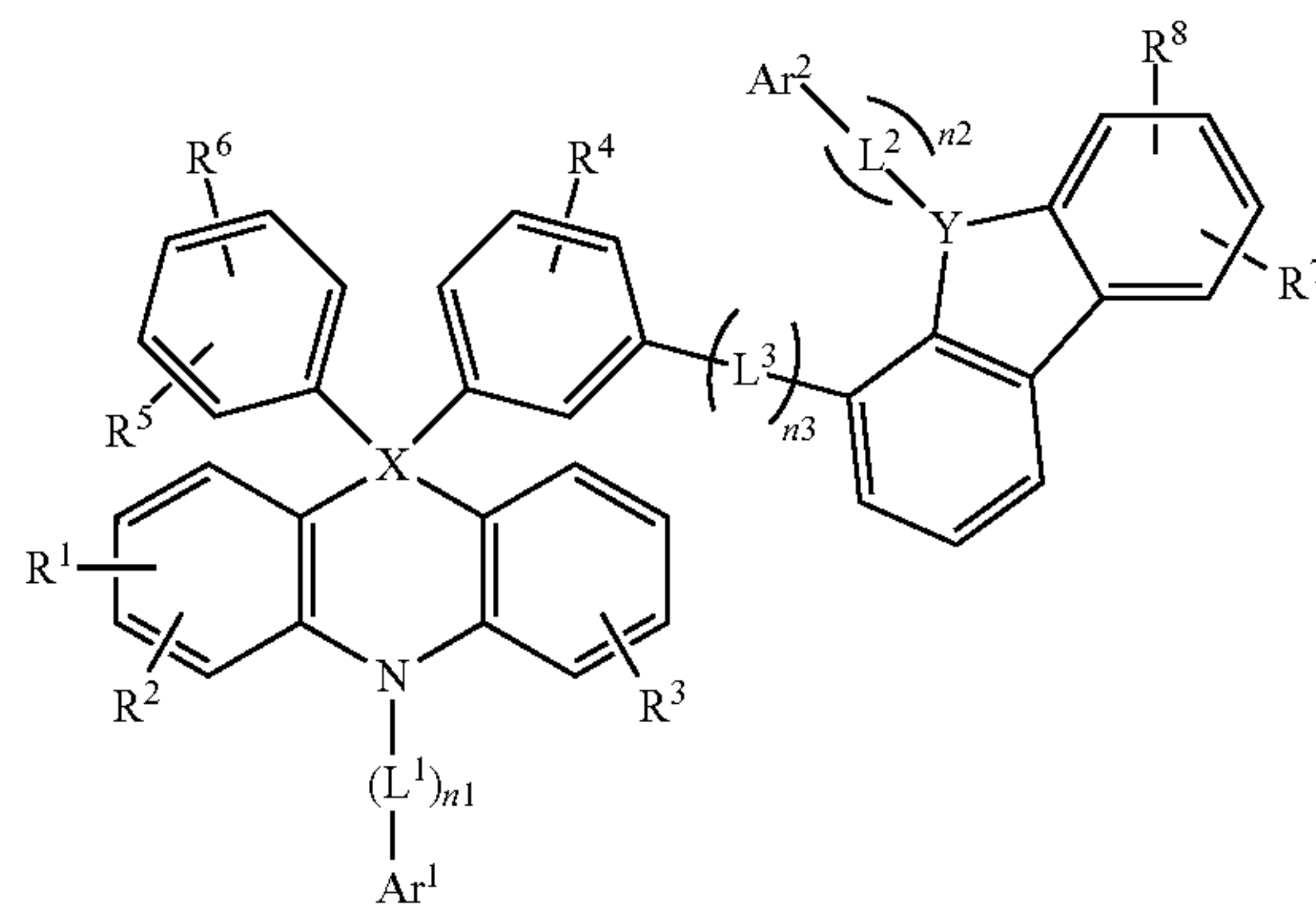
[Chemical Formula 1-3]
