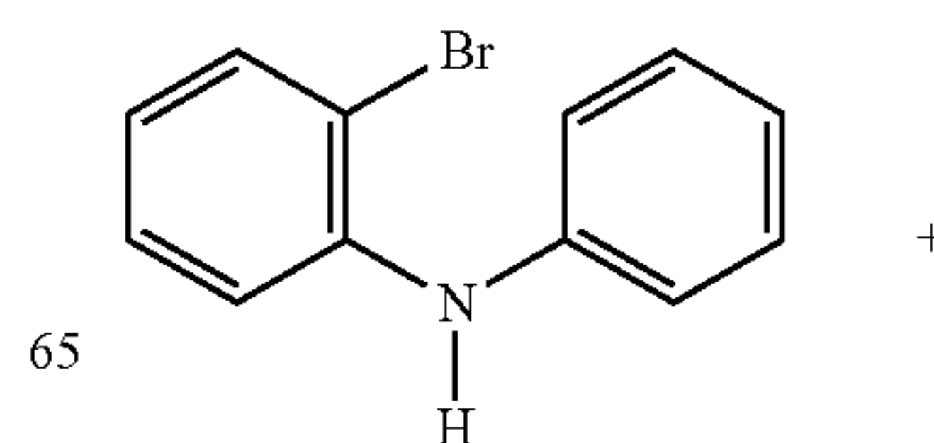
[Reaction Scheme 2]
