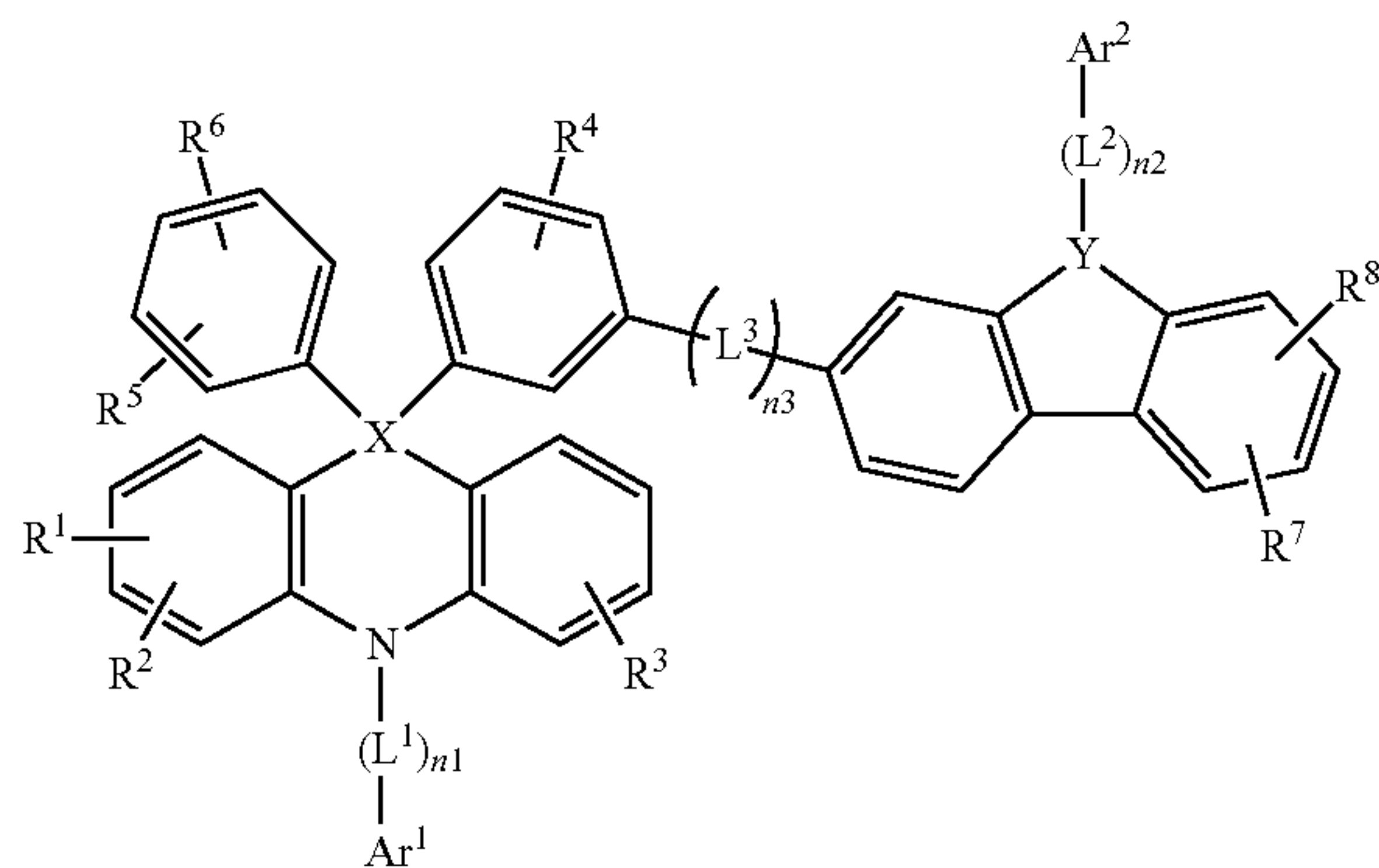
[Chemical Formula 1-2]
