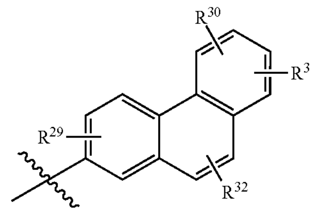
[Chemical Formula S-67]
