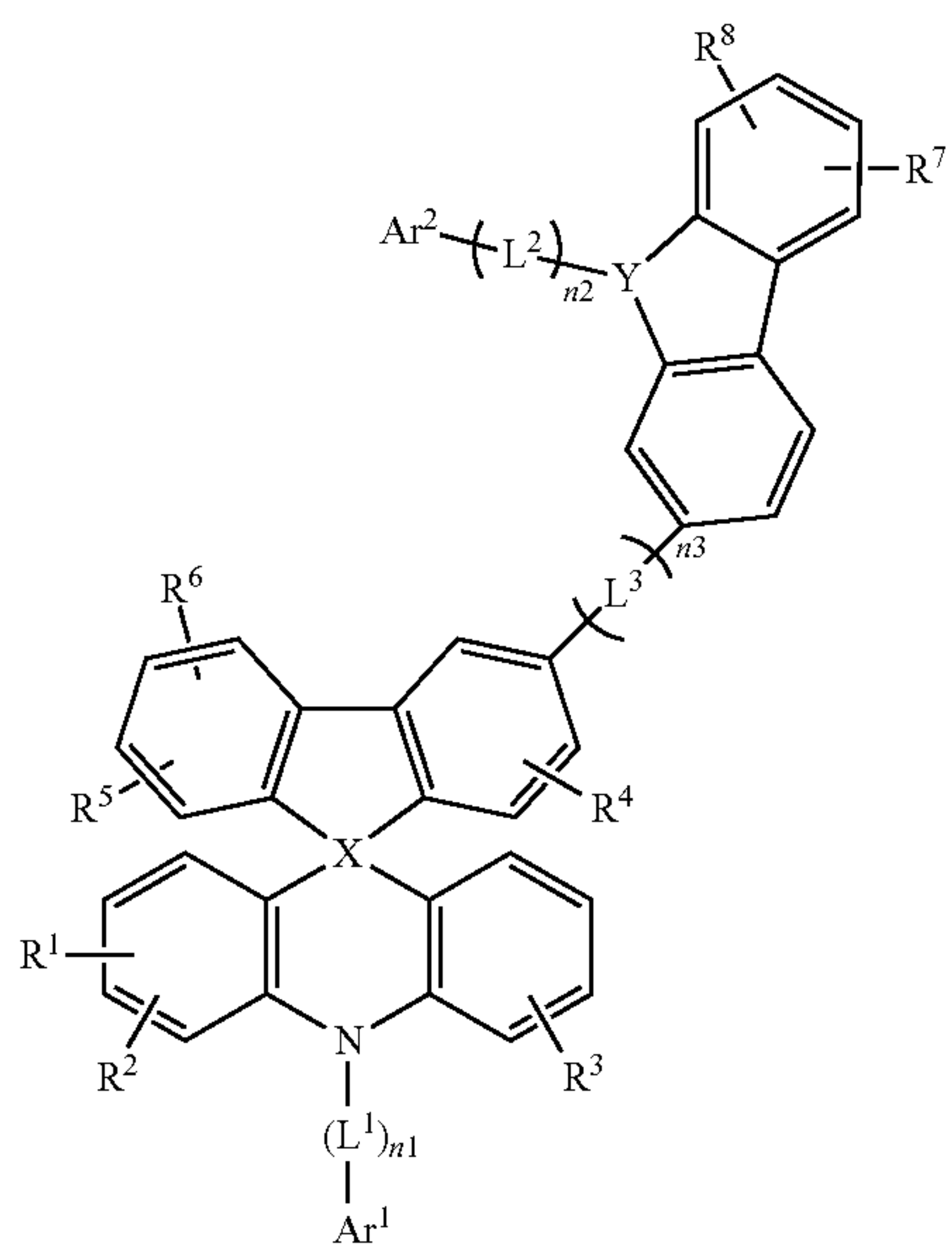
[Chemical Formula 2-5]
