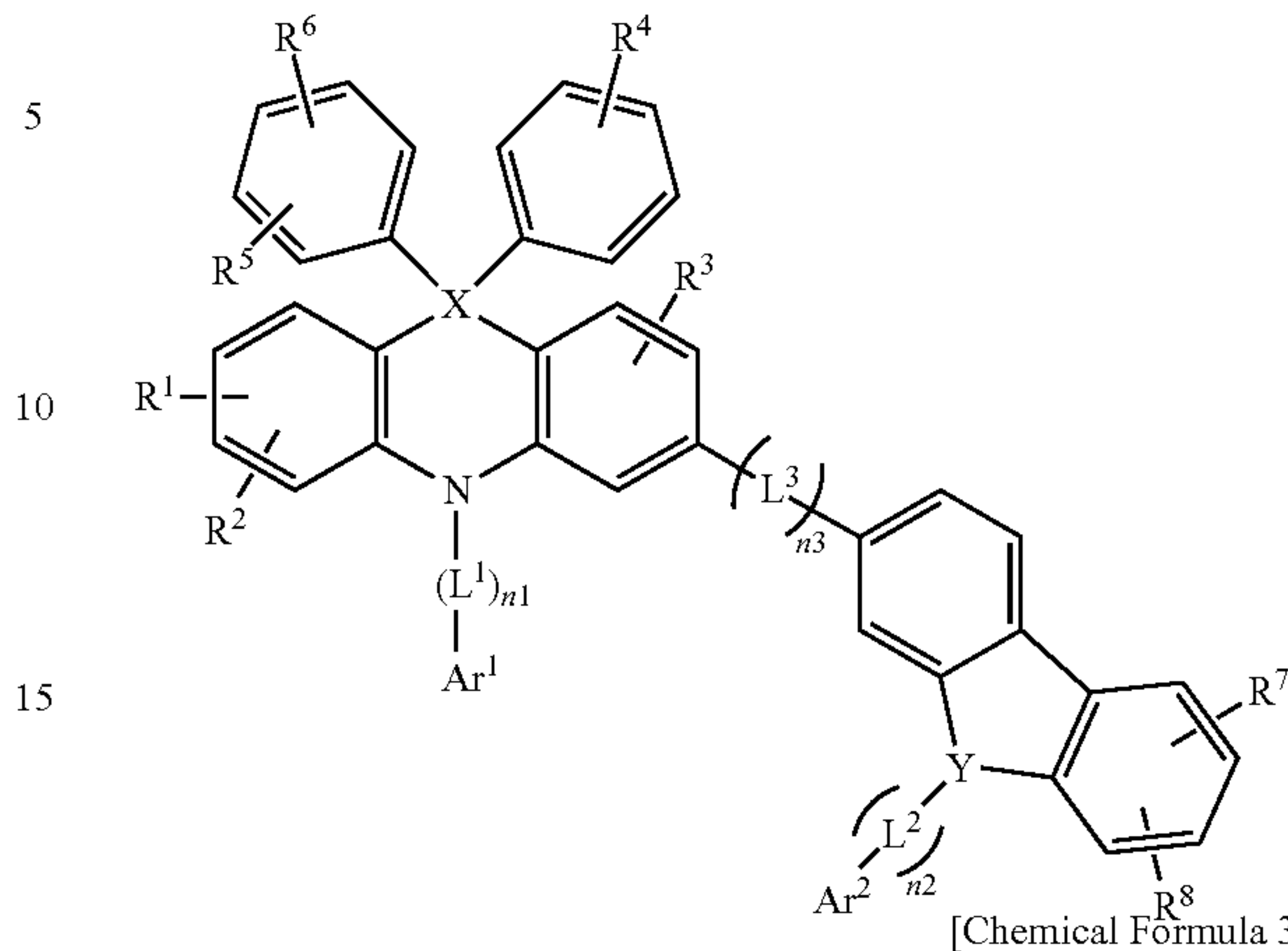
[Chemical Formula 3-2]
