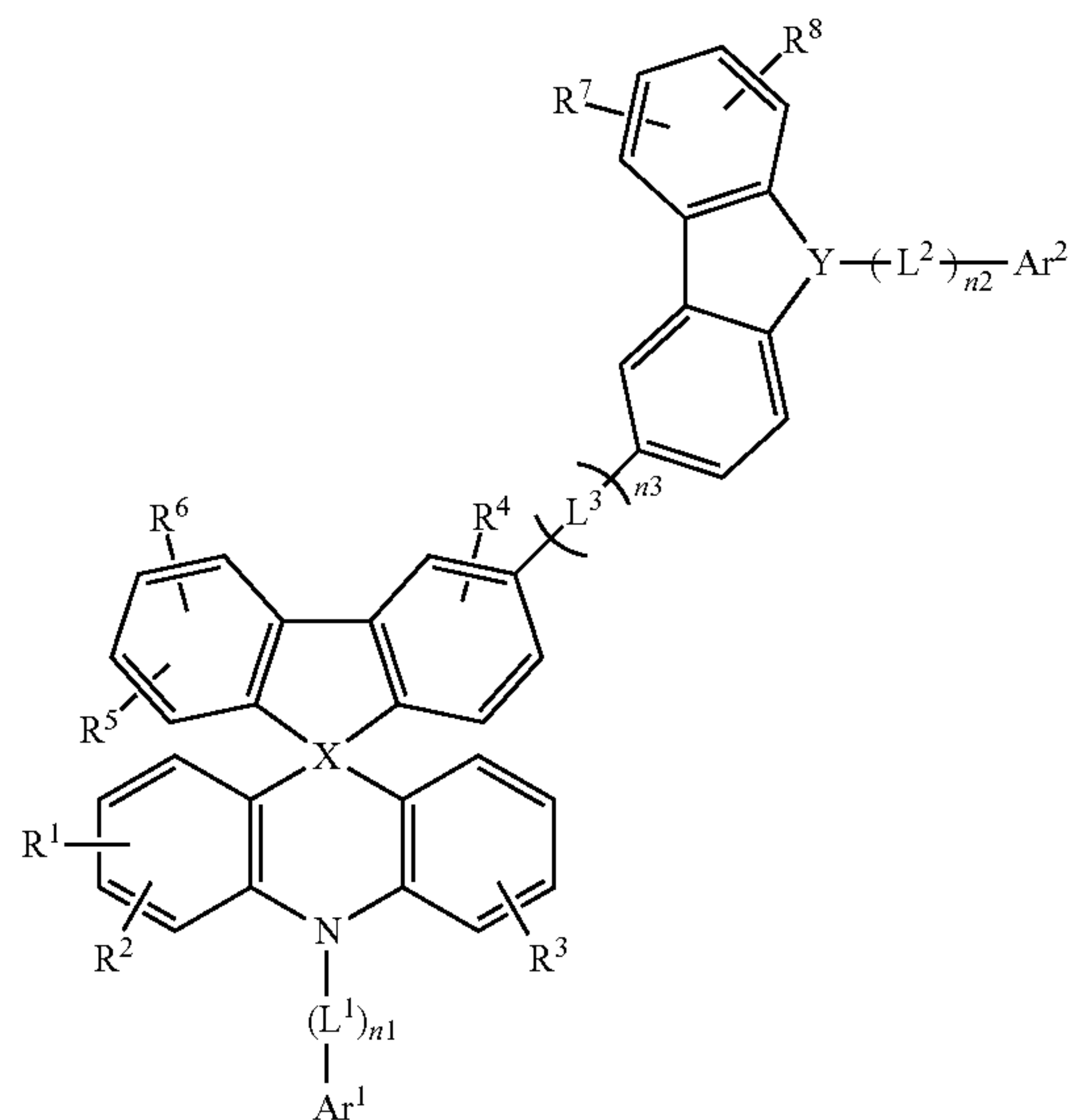
[Chemical Formula 2-4]
