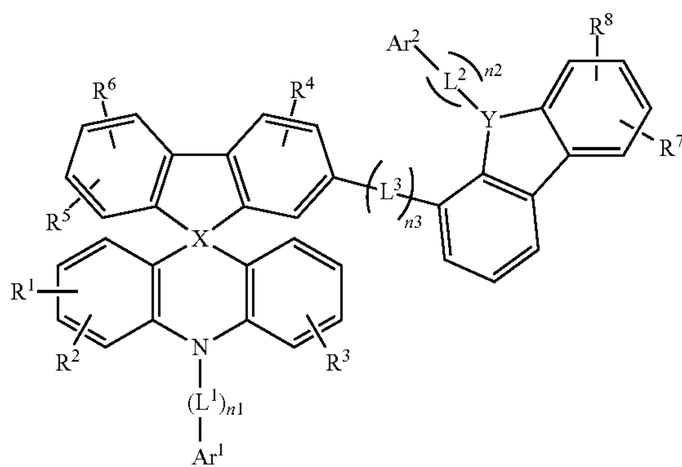
[Chemical Formula 2-3]
