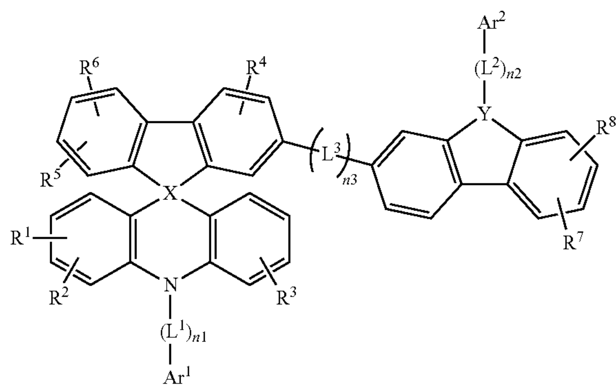
[Chemical Formula 2-2]
