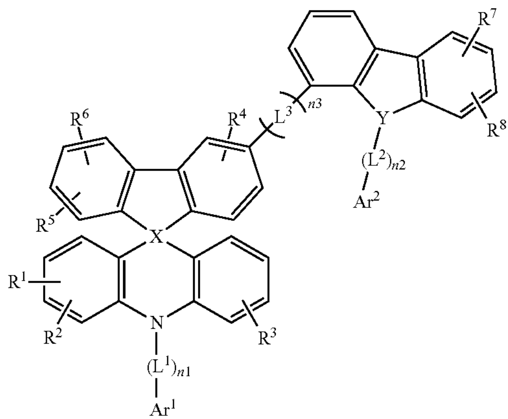
[Chemical Formula 2-6]
