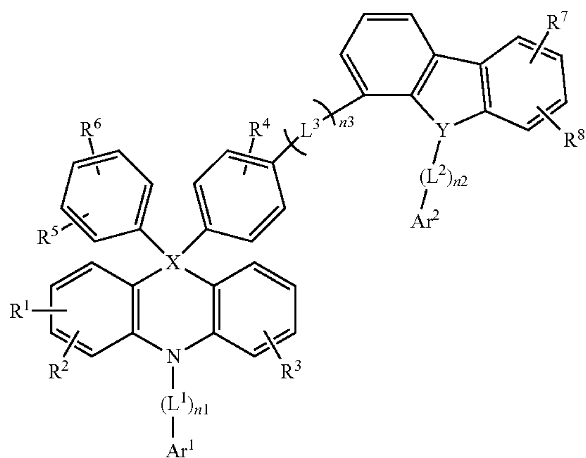
[Chemical Formula 1-6]
