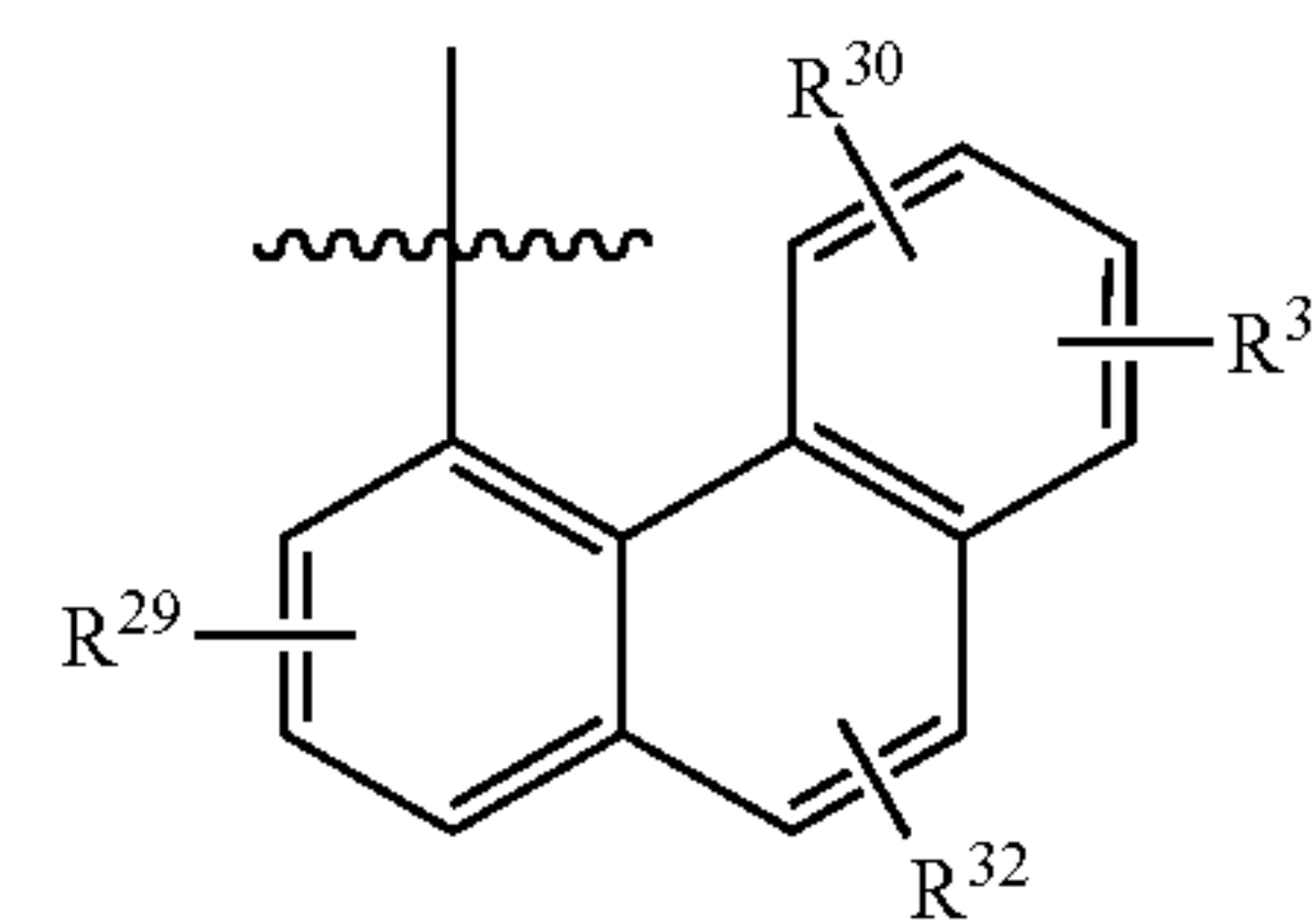
[Chemical Formula S-69]
