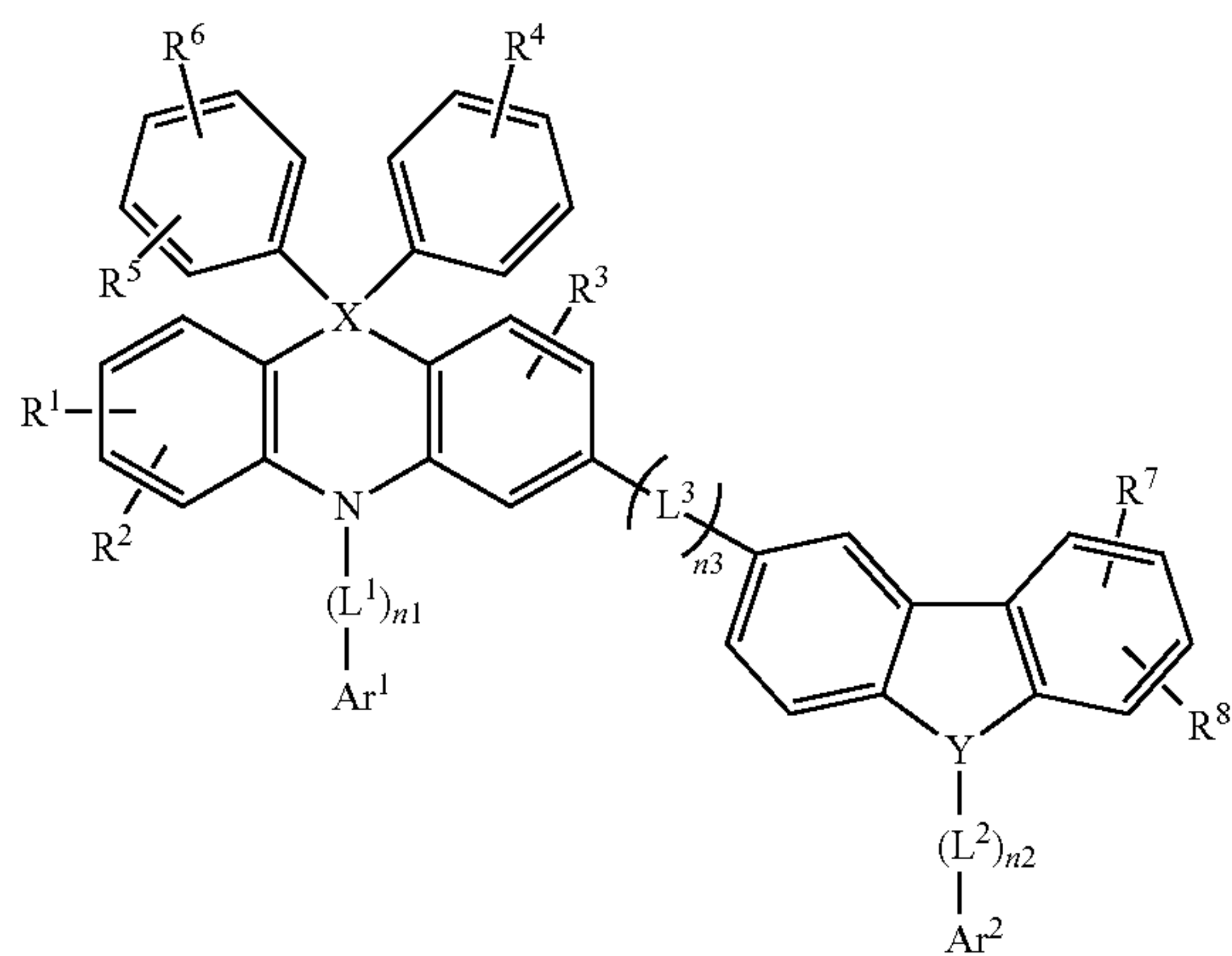
[Chemical Formula 3-1]
