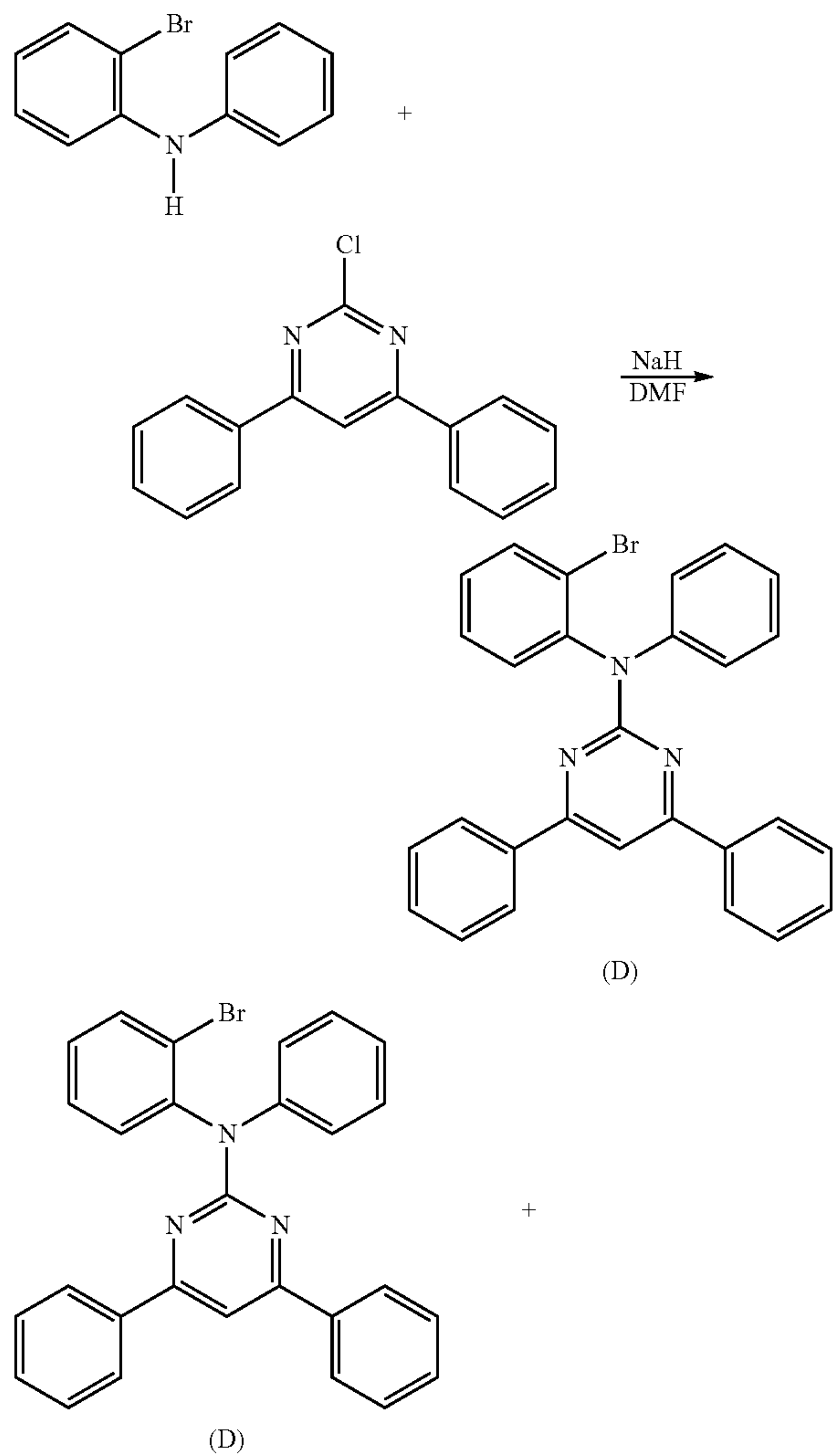
[Reaction Scheme 3]
