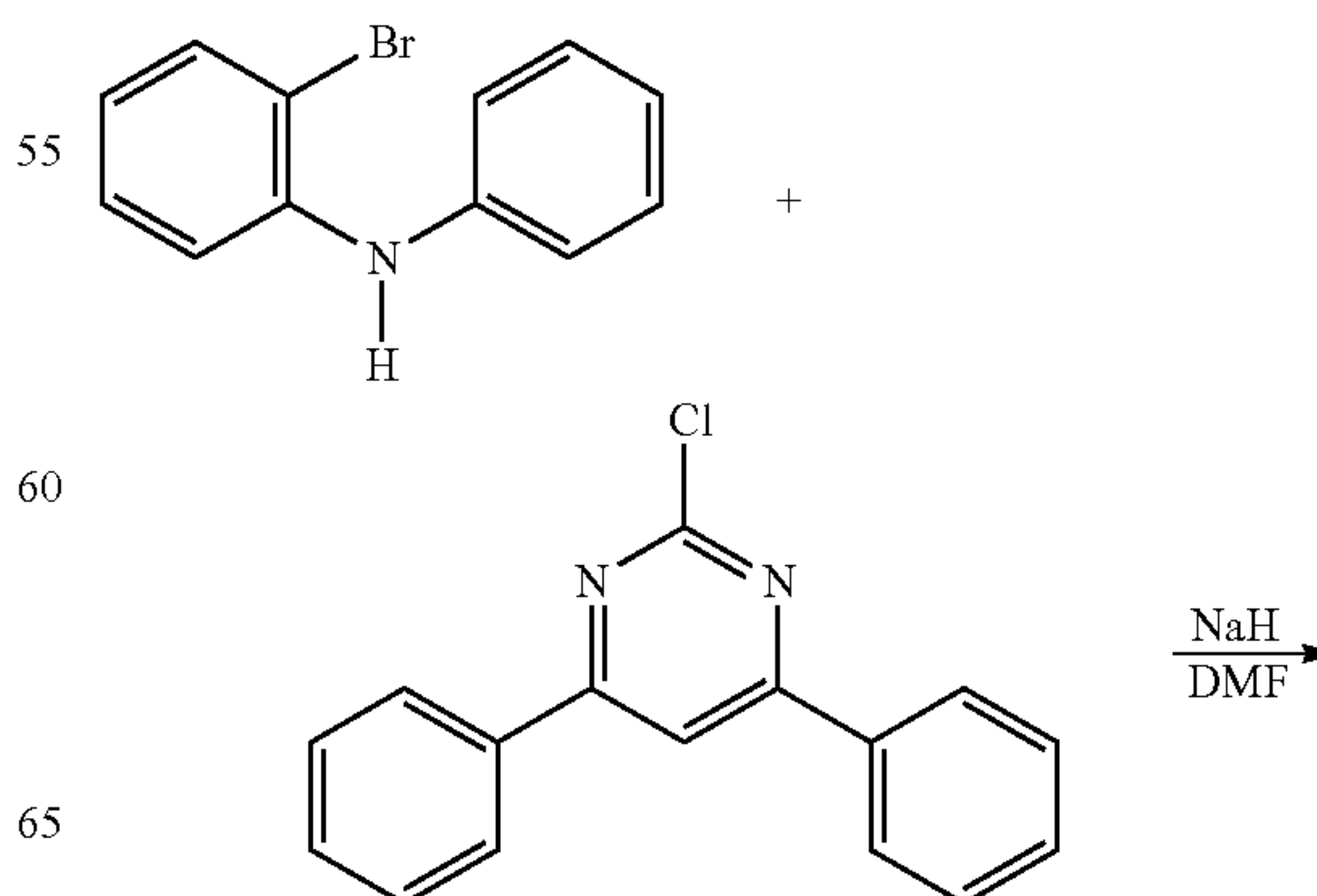
[Reaction Scheme 4]
