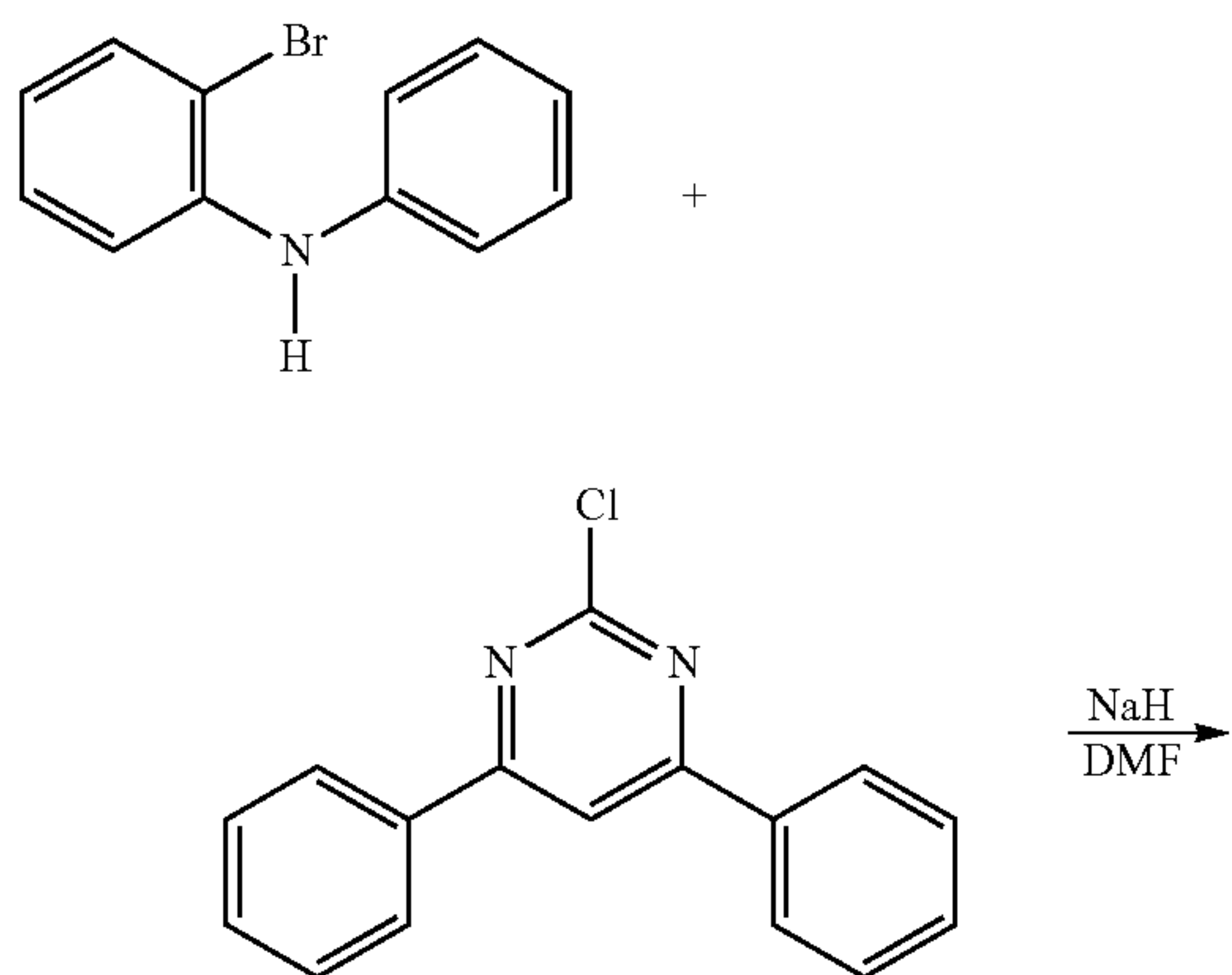
[Reaction Scheme 8]
