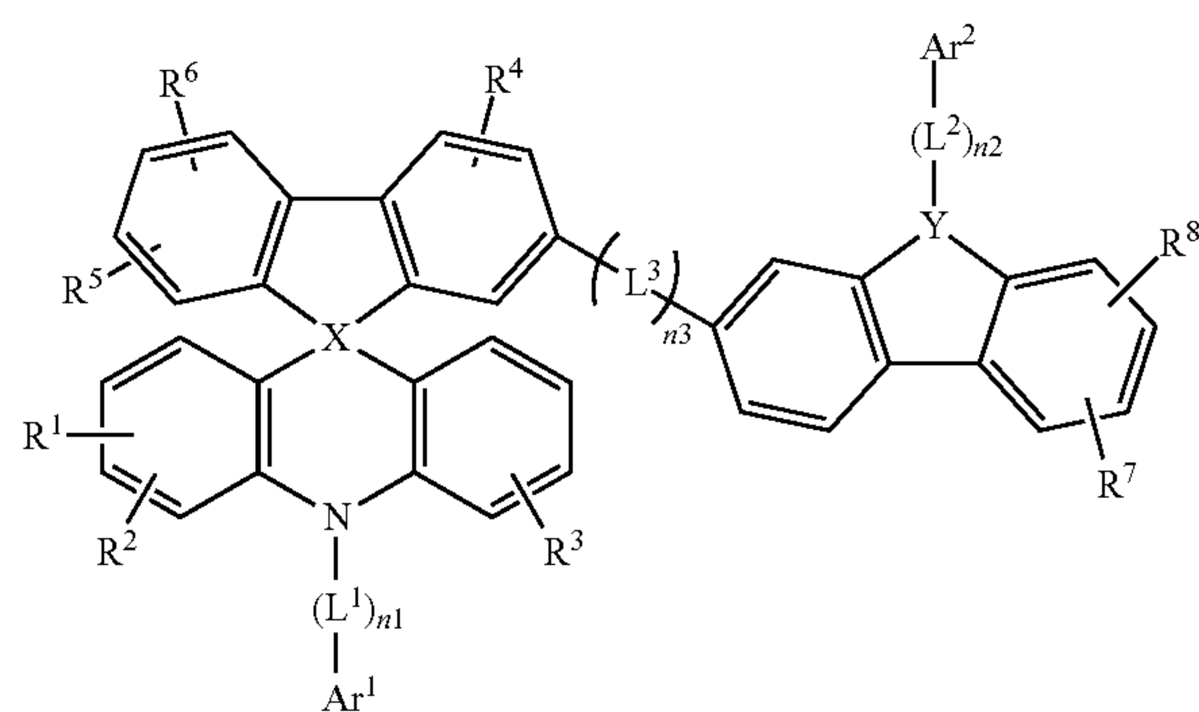
[Chemical Formula 2-2]
