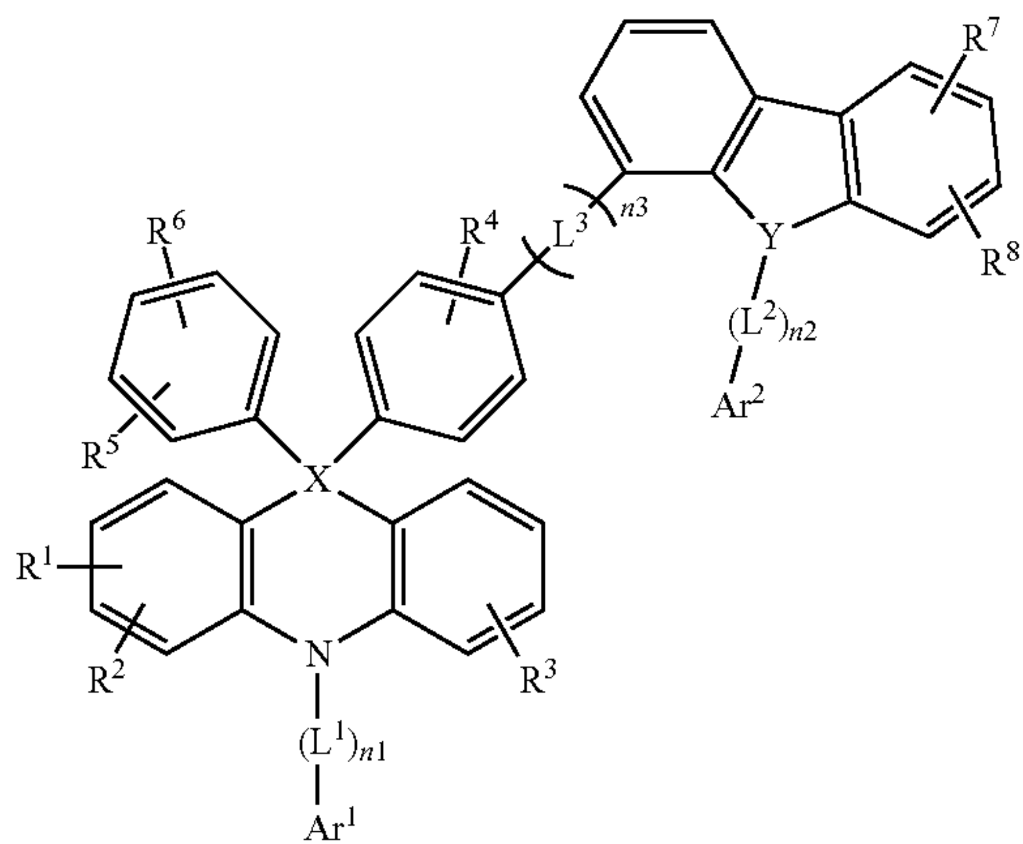
[Chemical Formula 1-6]
