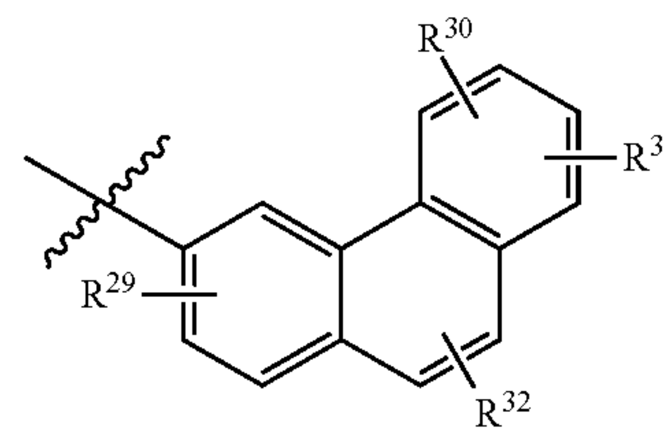
[Chemical Formula S-68]
