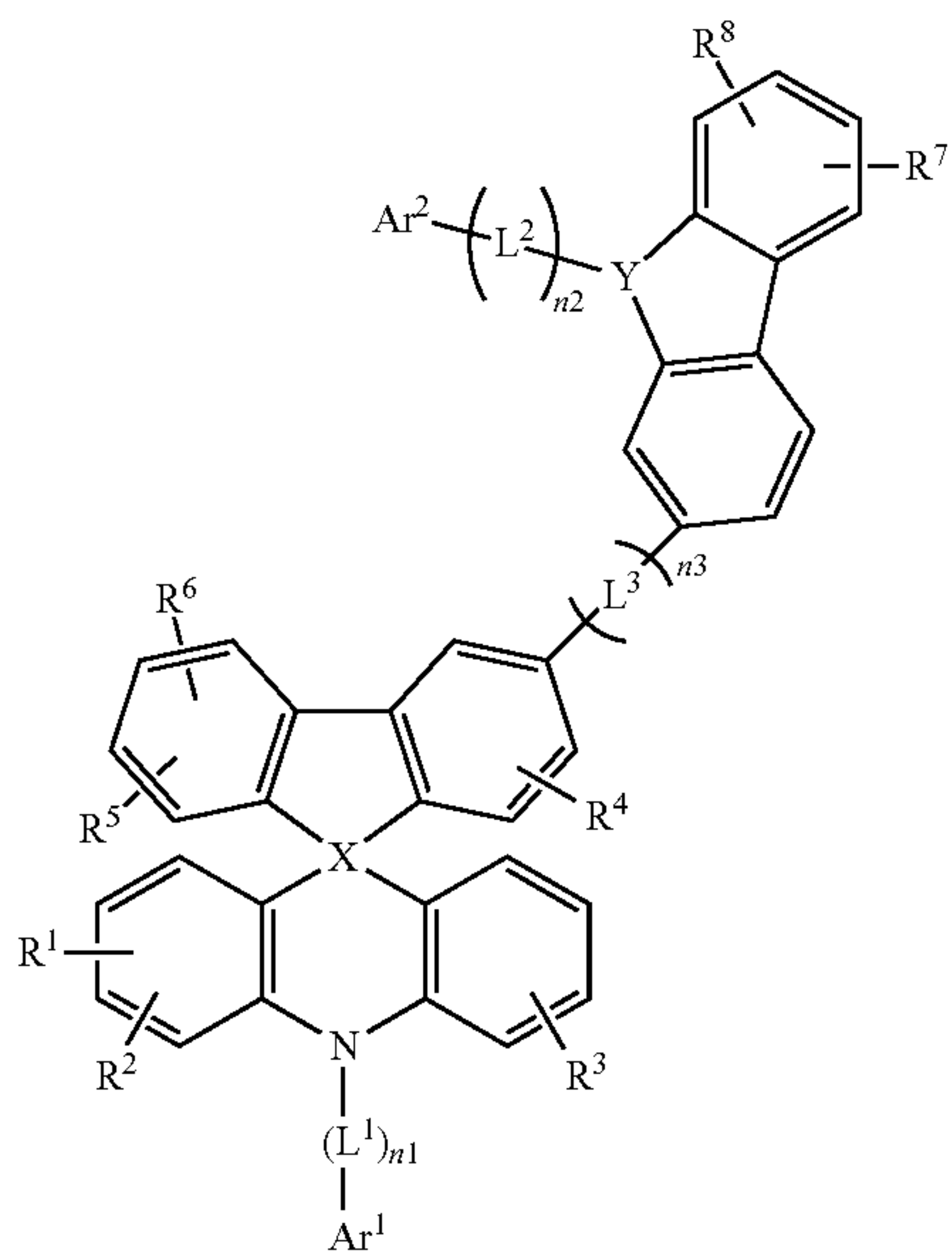
[Chemical Formula 2-5]
