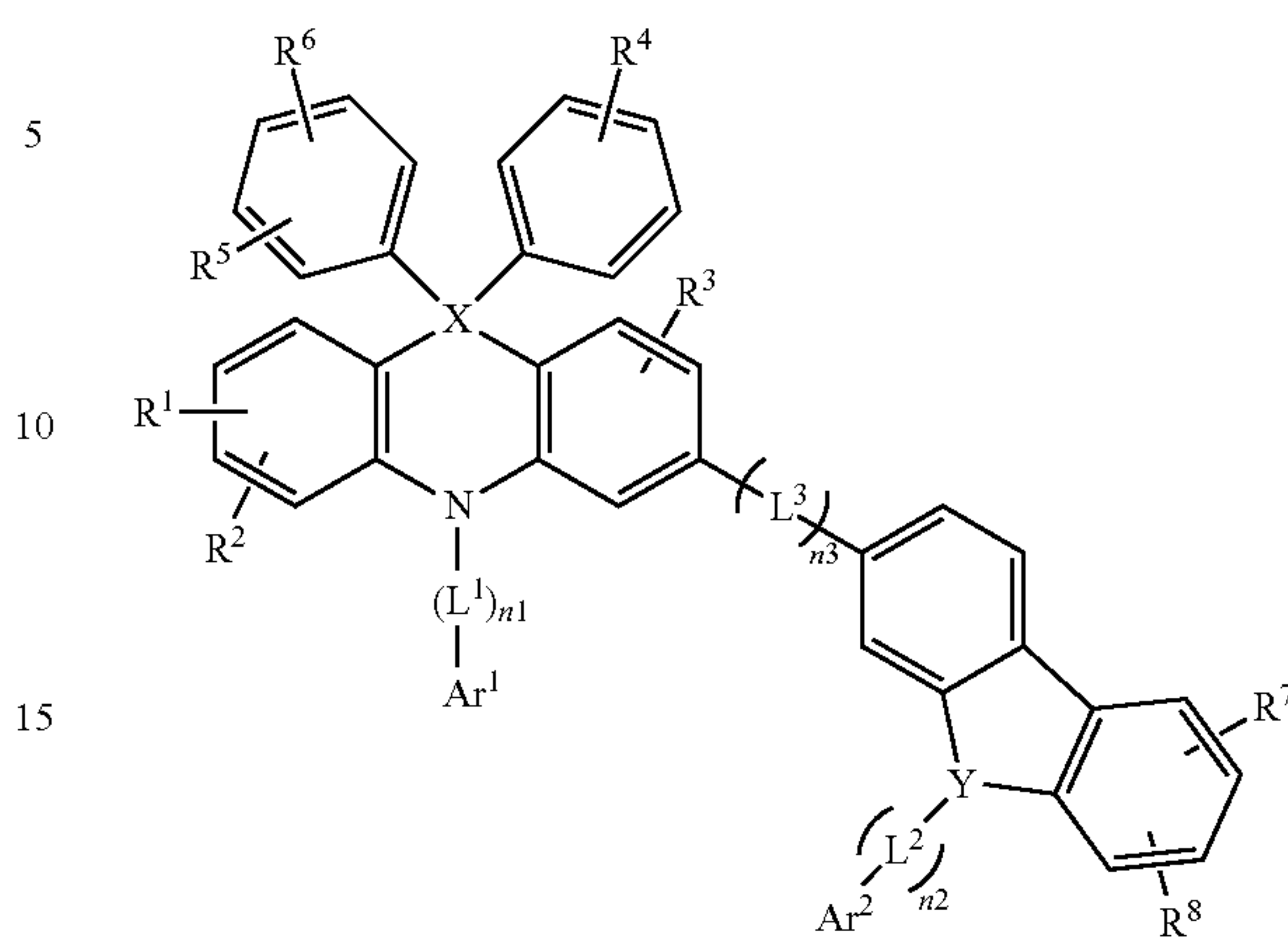
[Chemical Formula 3-3]
