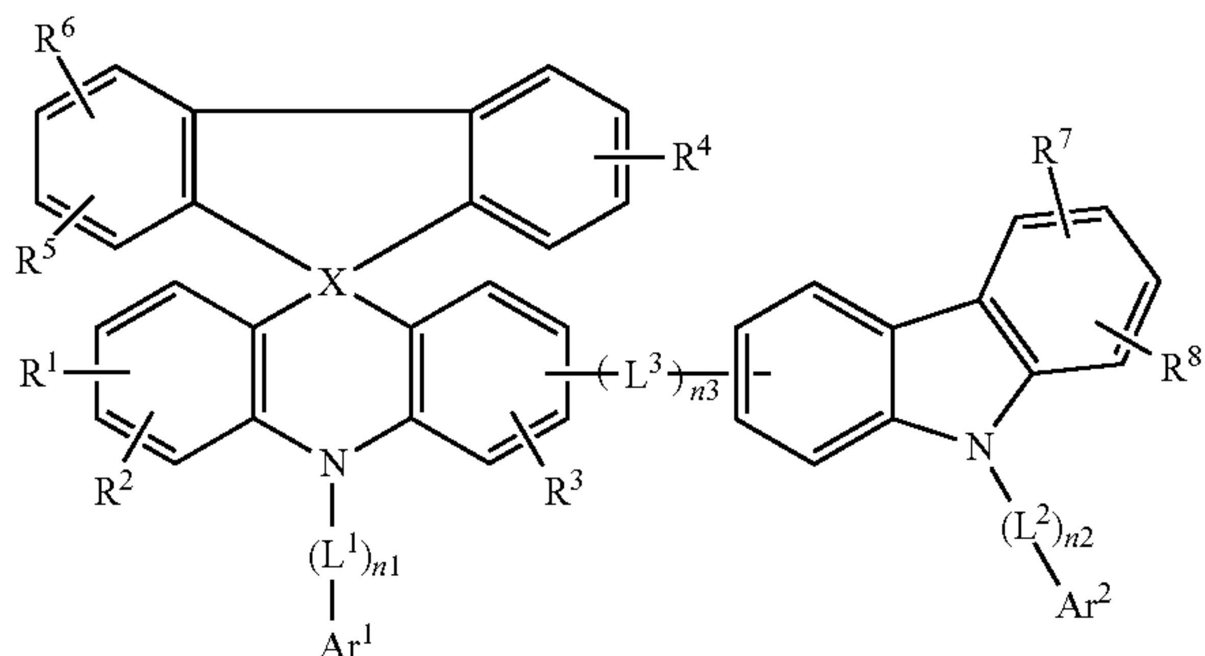
[Chemical Formula 4]
