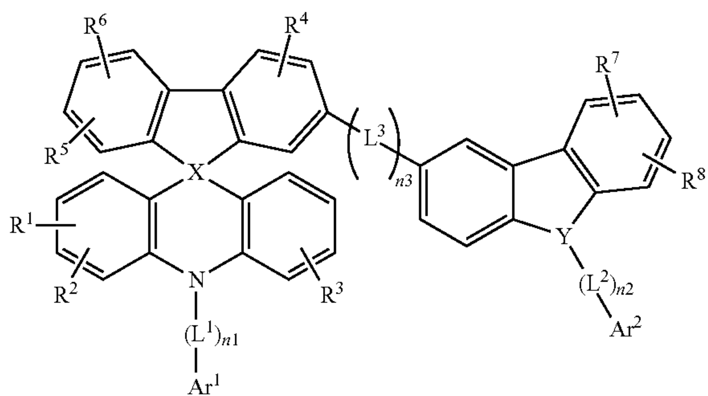
[Chemical Formula 2-1]
