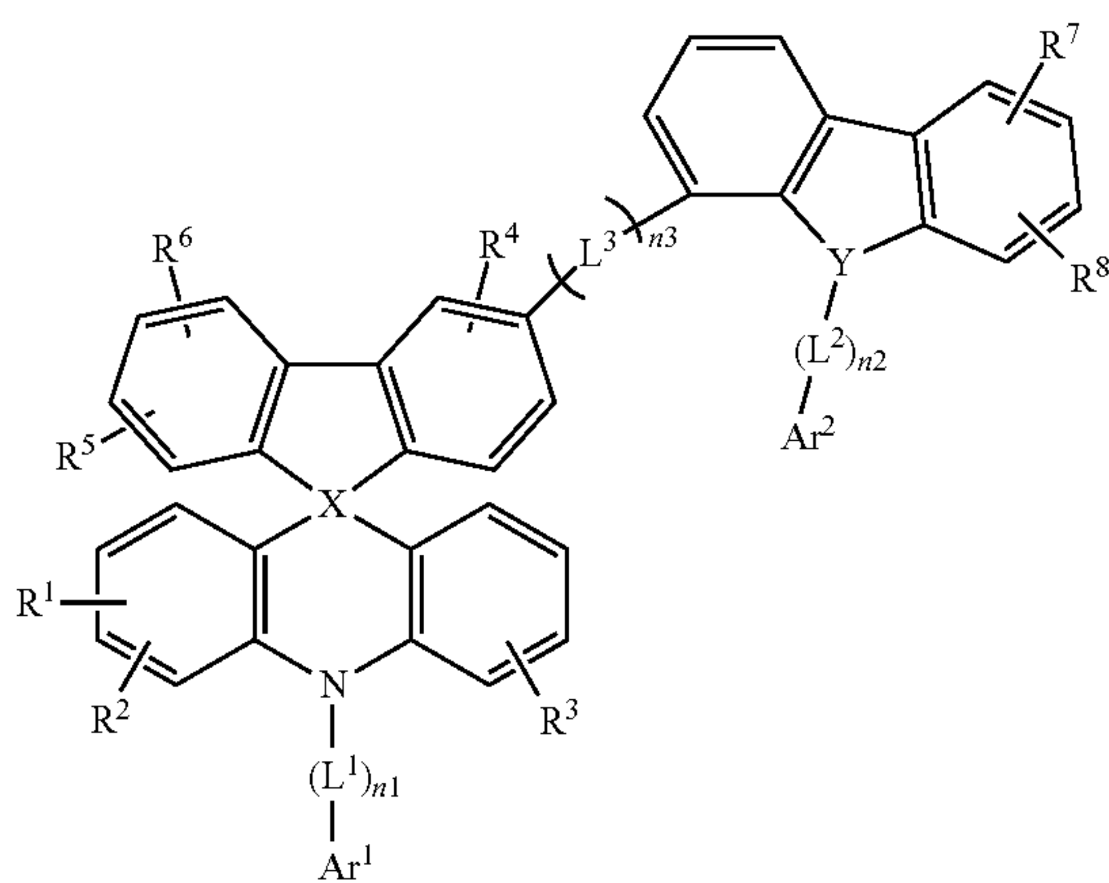
[Chemical Formula 2-6]
