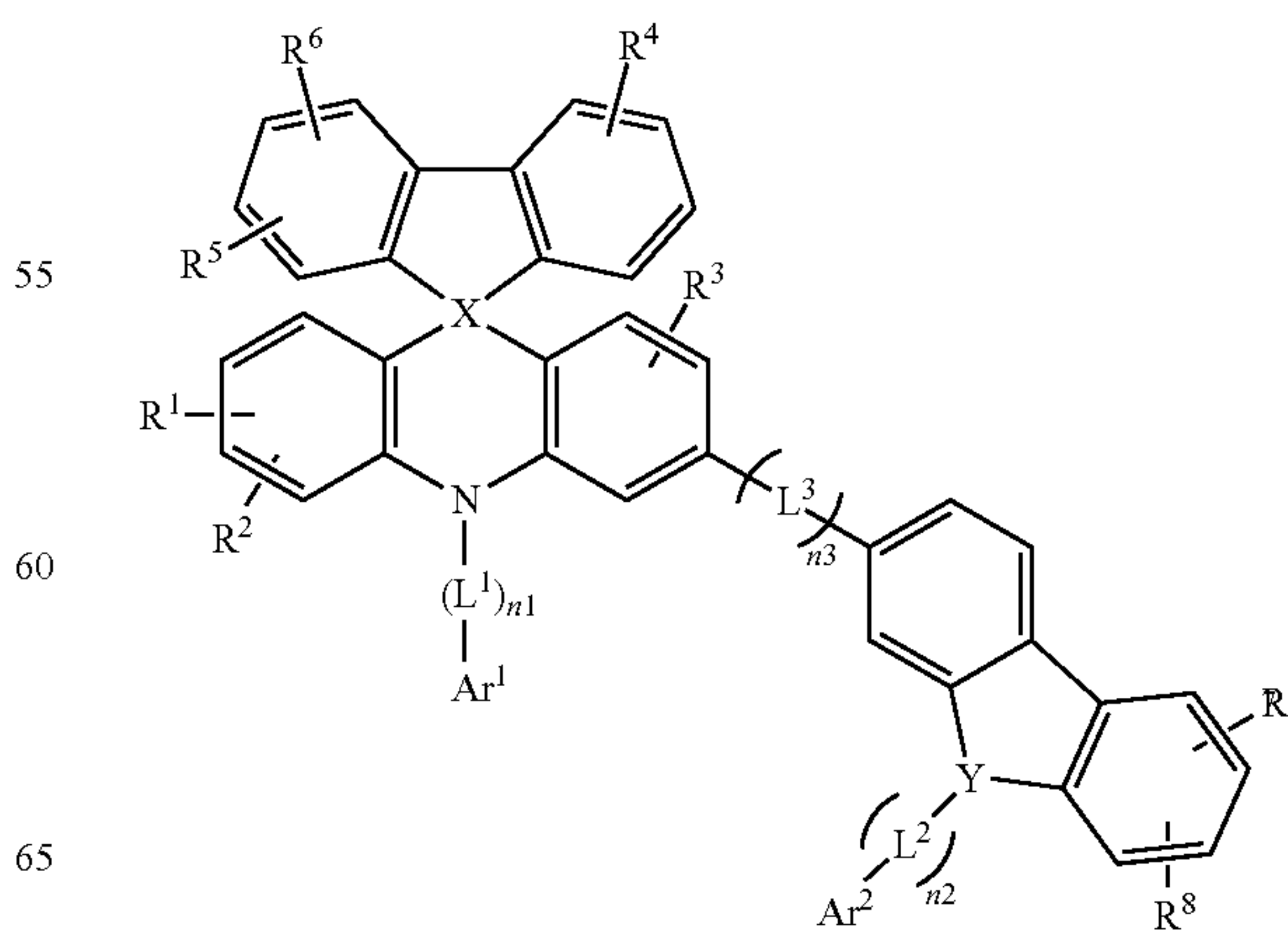
[Chemical Formula 4-2]
