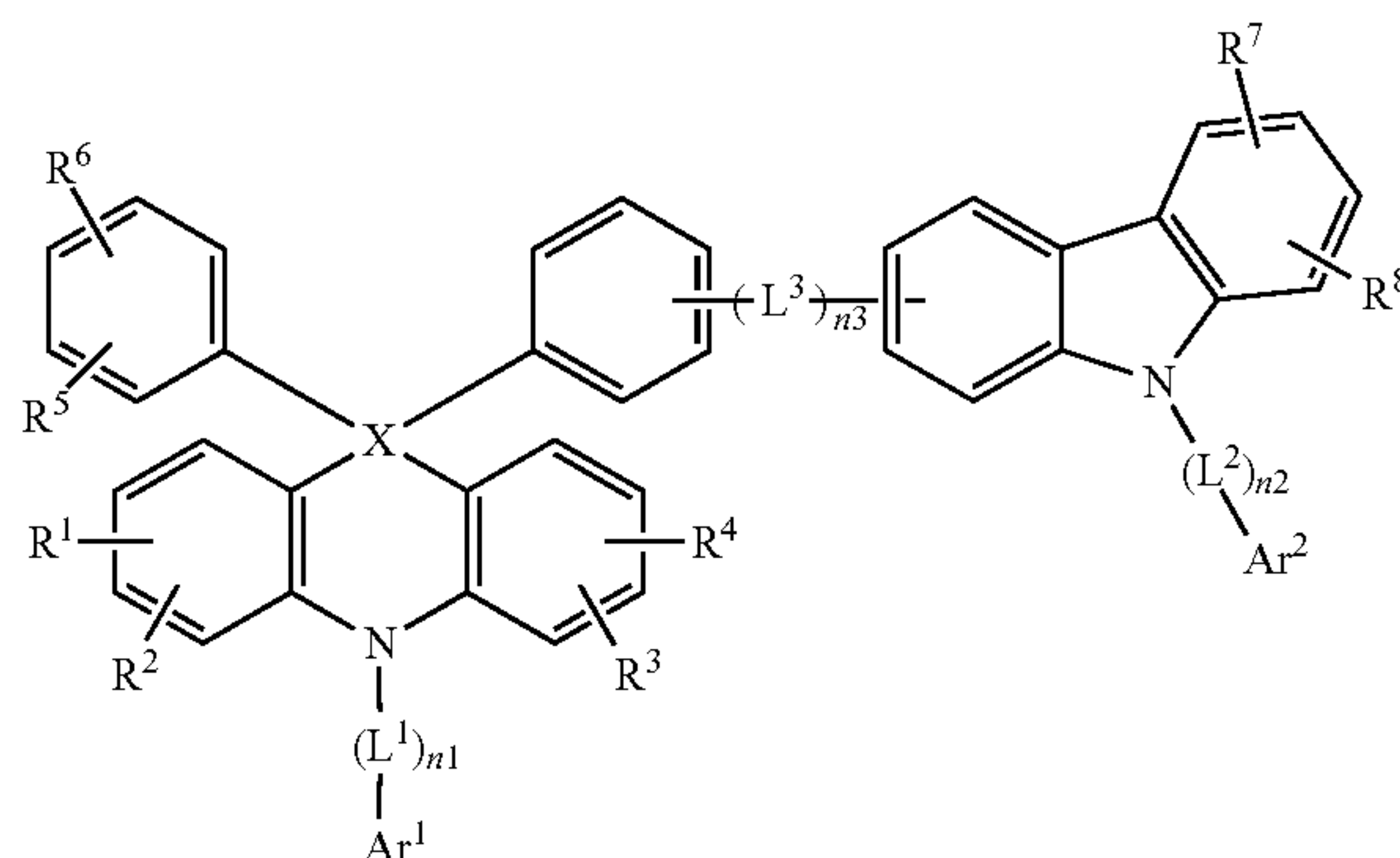
[Chemical Formula 2]
