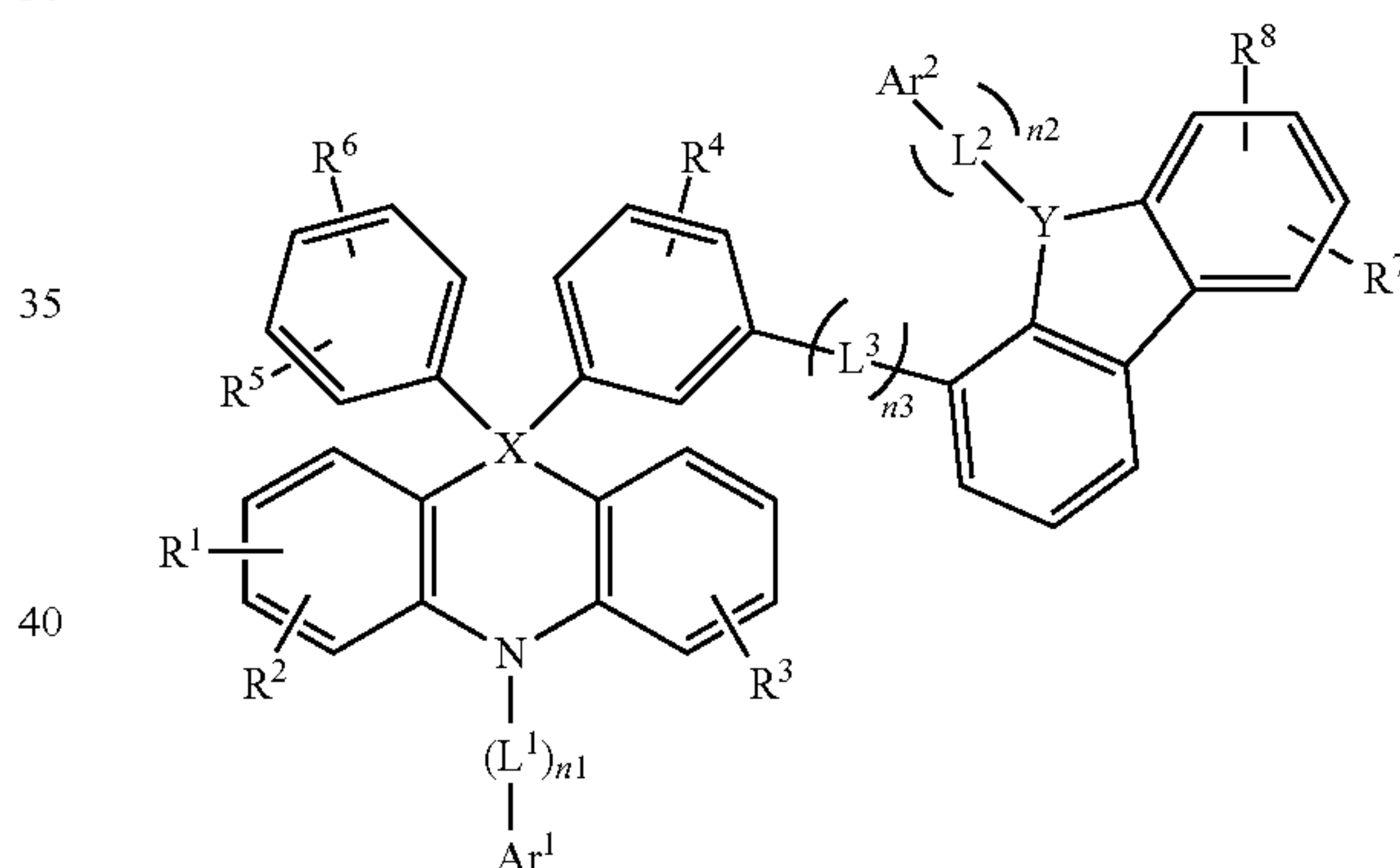
[Chemical Formula 1-4]
