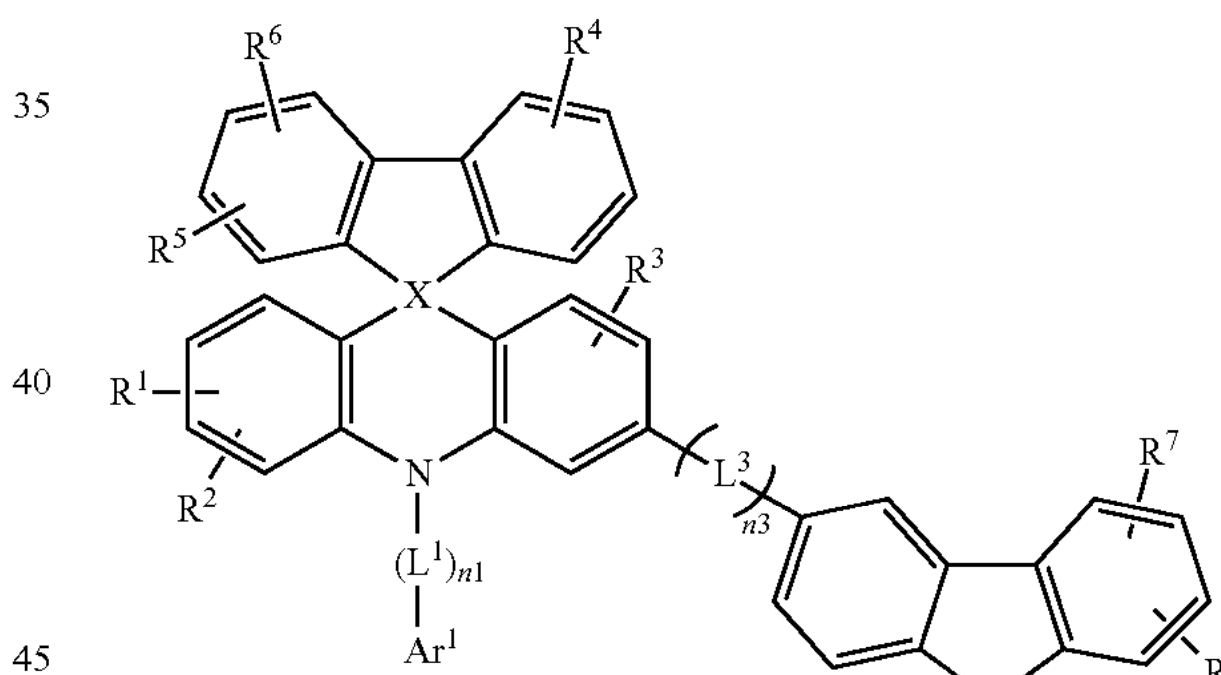
[Chemical Formula 4-1]
