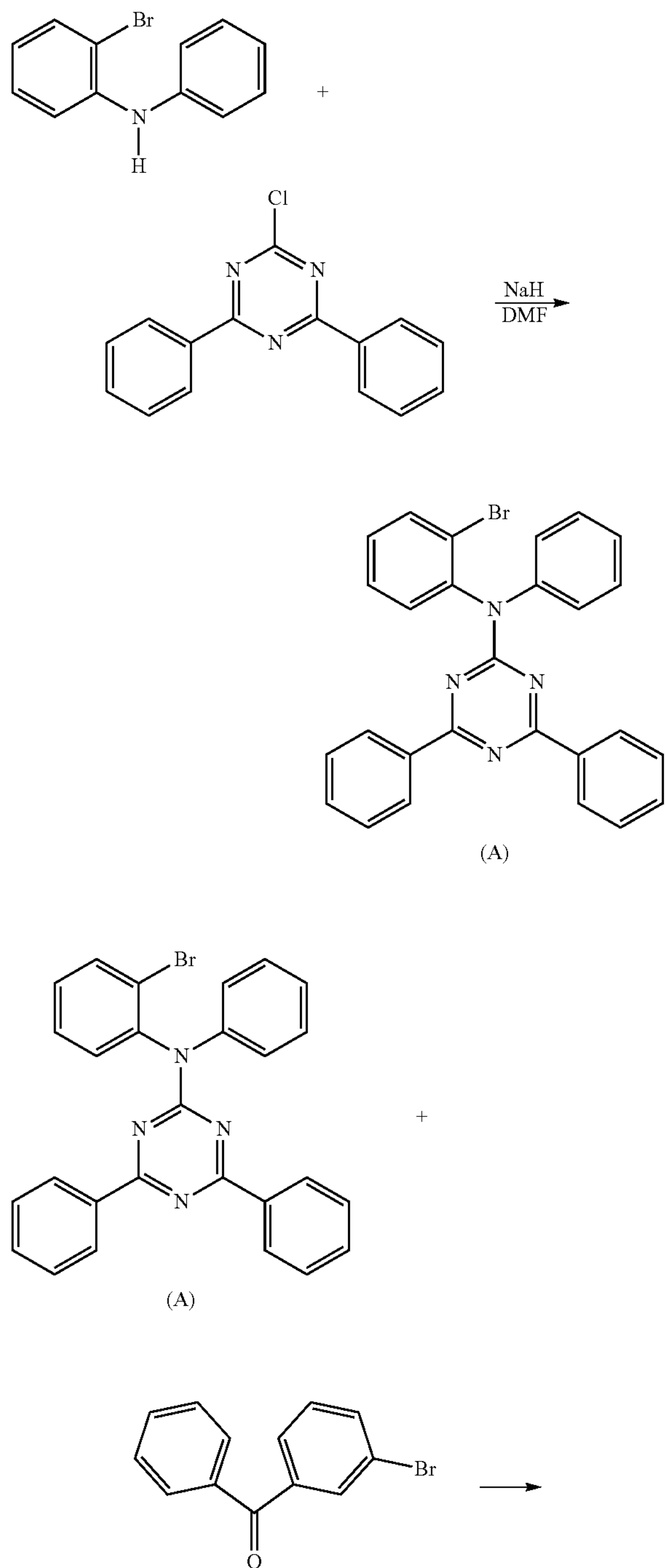
[Reaction Scheme 5]
