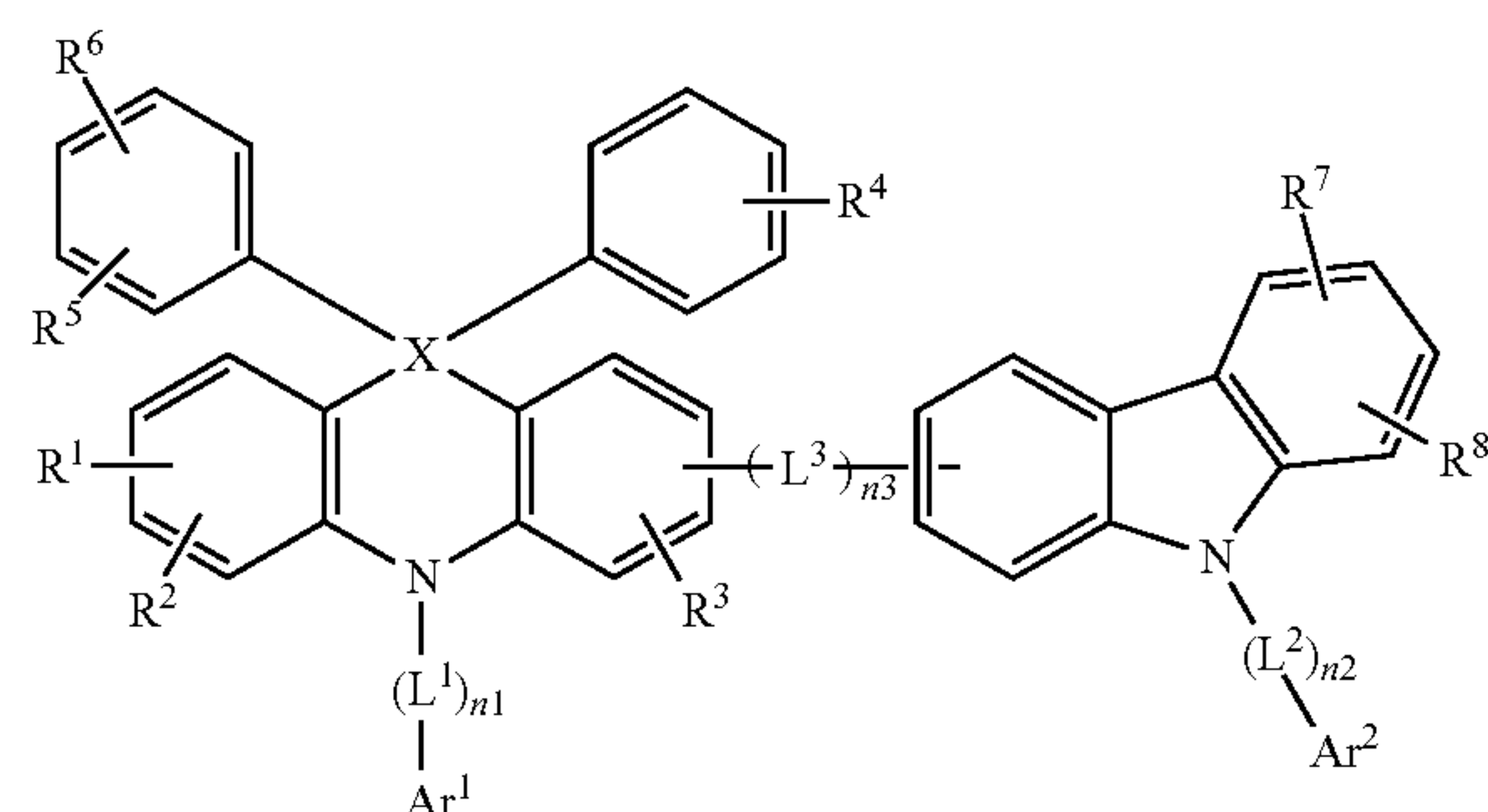
[Chemical Formula 3]
