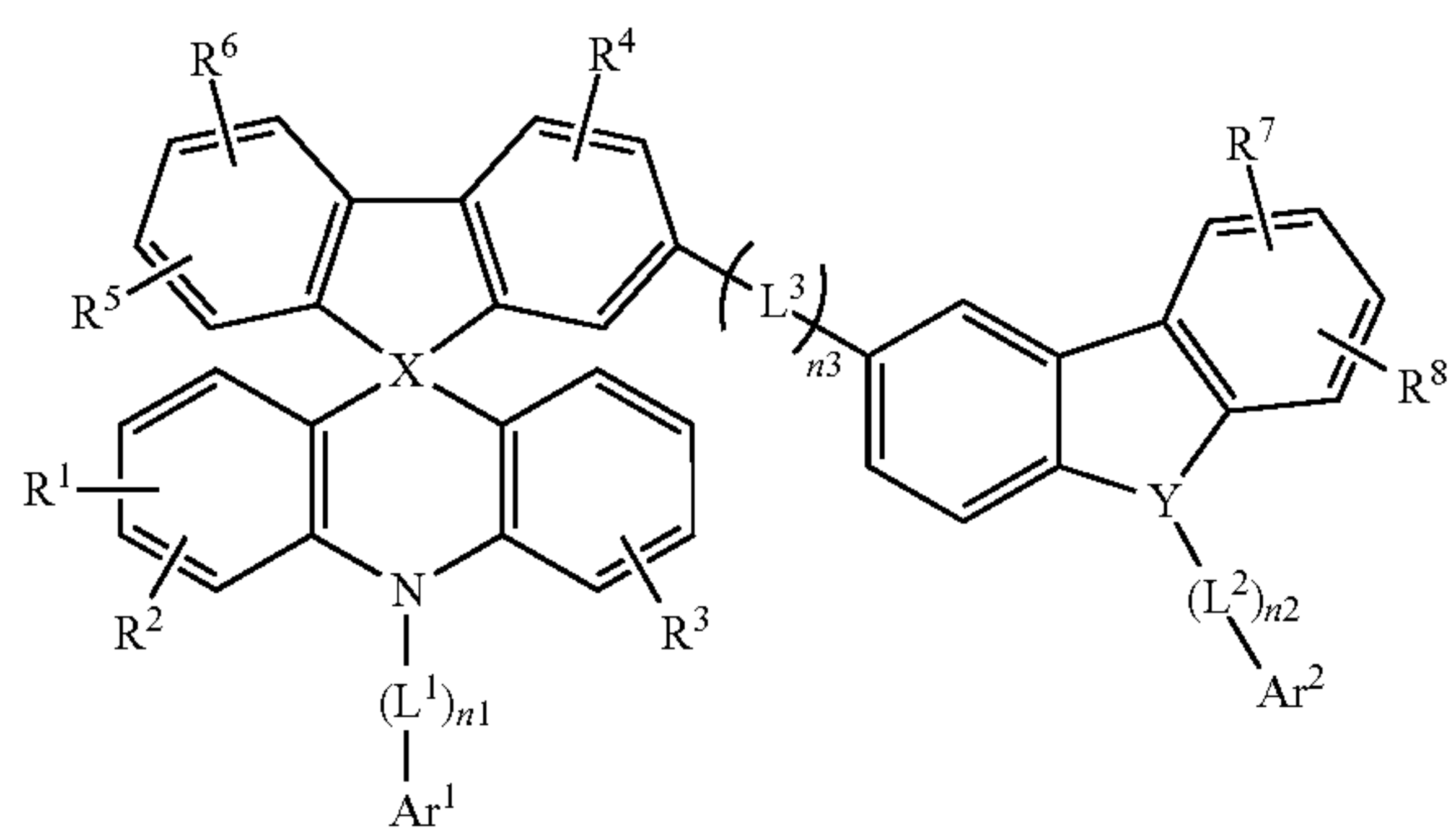
[Chemical Formula 2-1]
