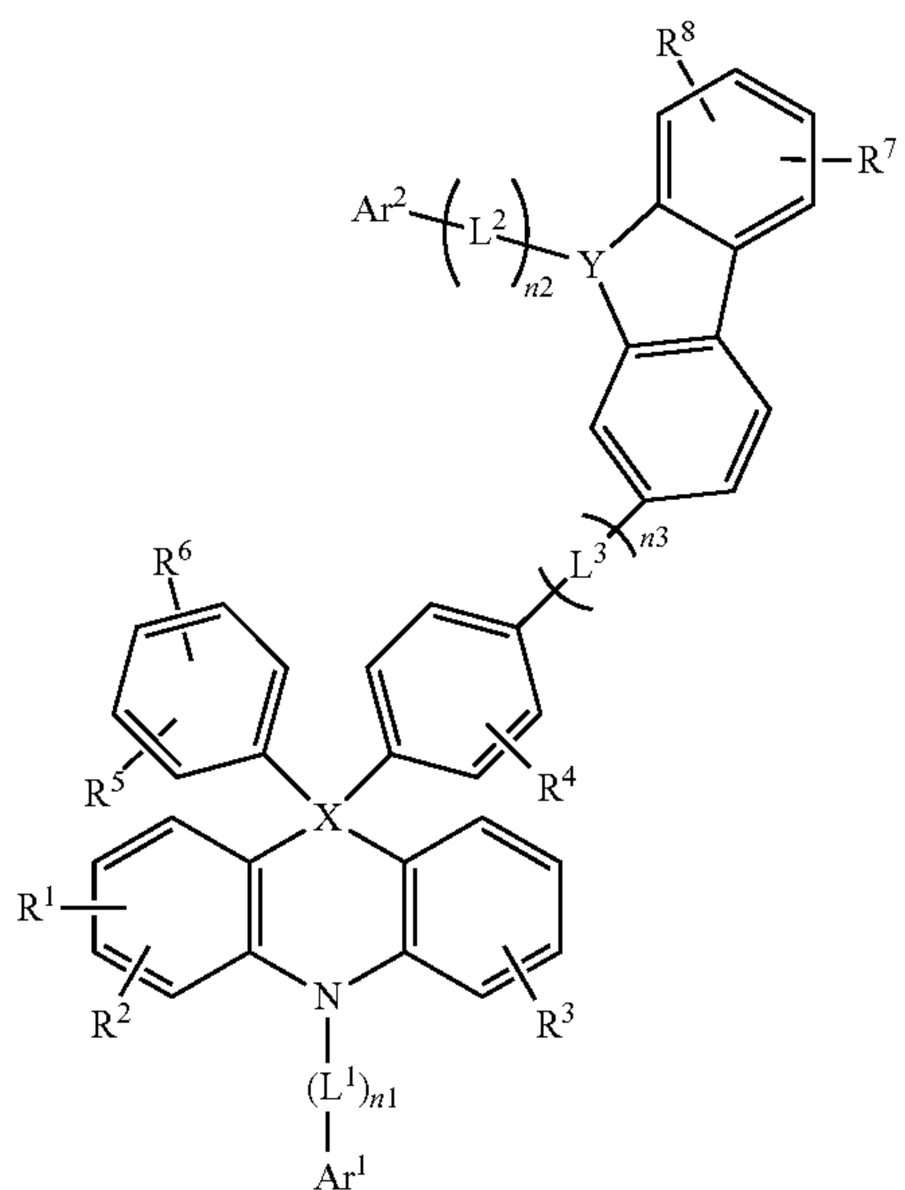
[Chemical Formula 1-5]
