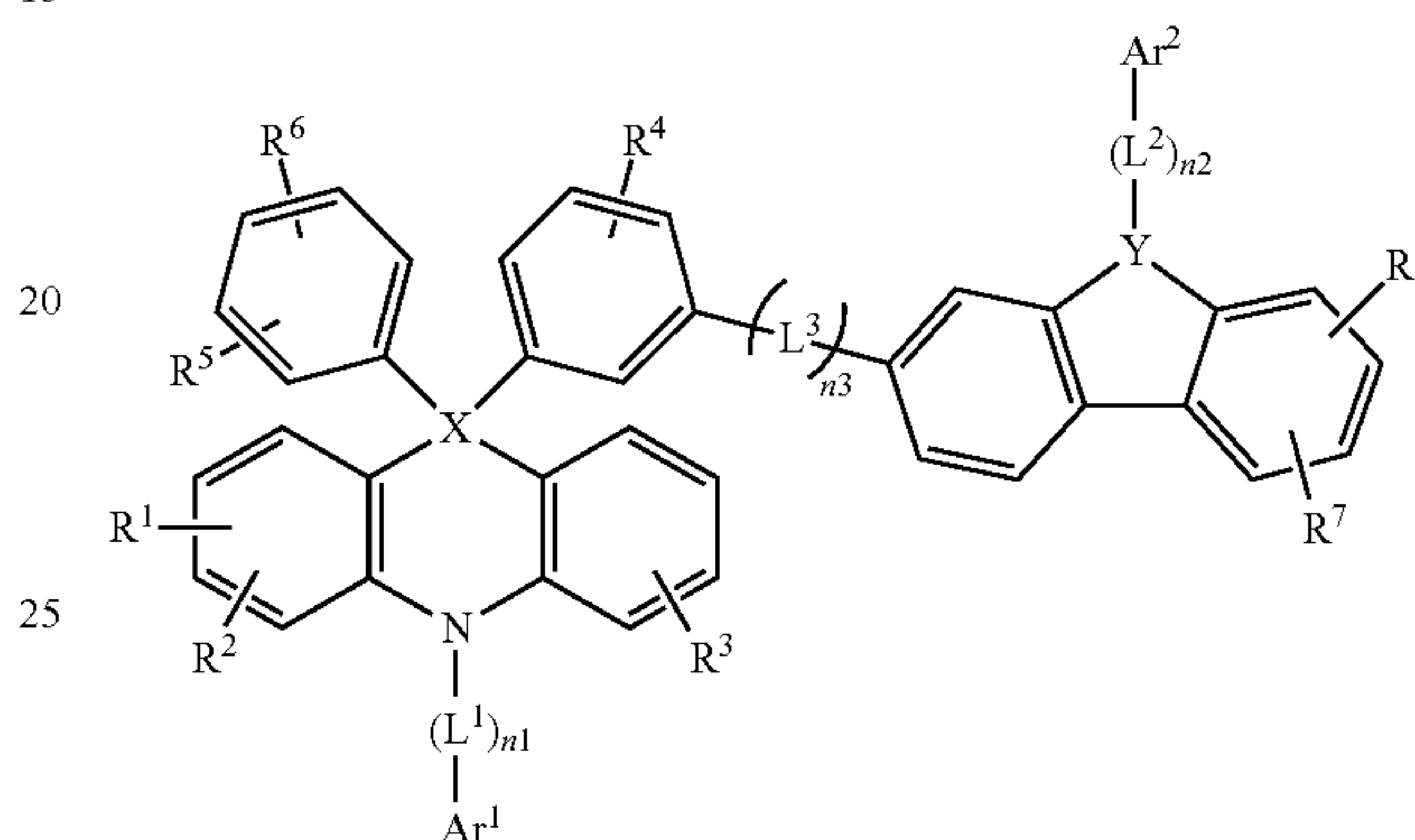
[Chemical Formula 1-3]
