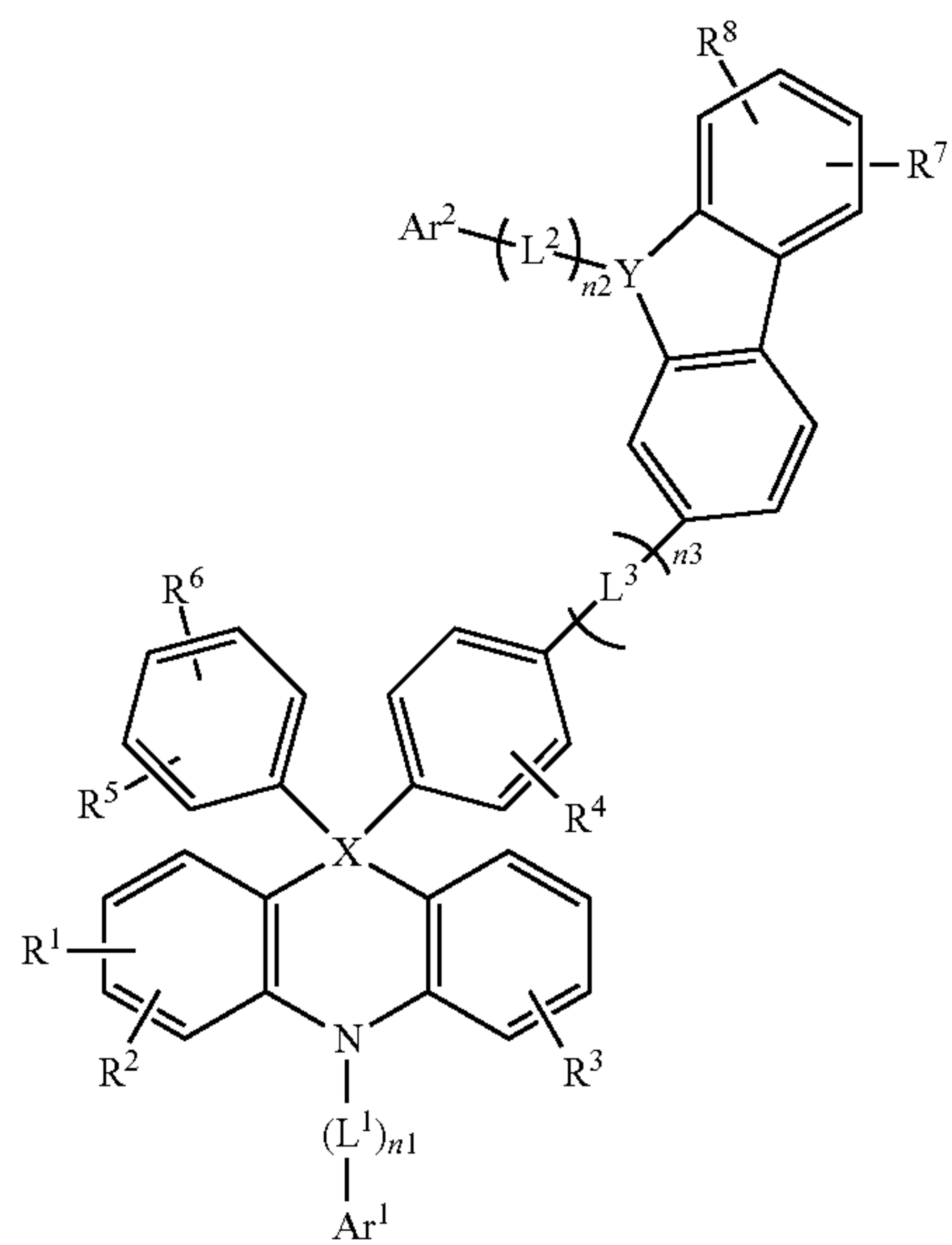
[Chemical Formula 1-5]
