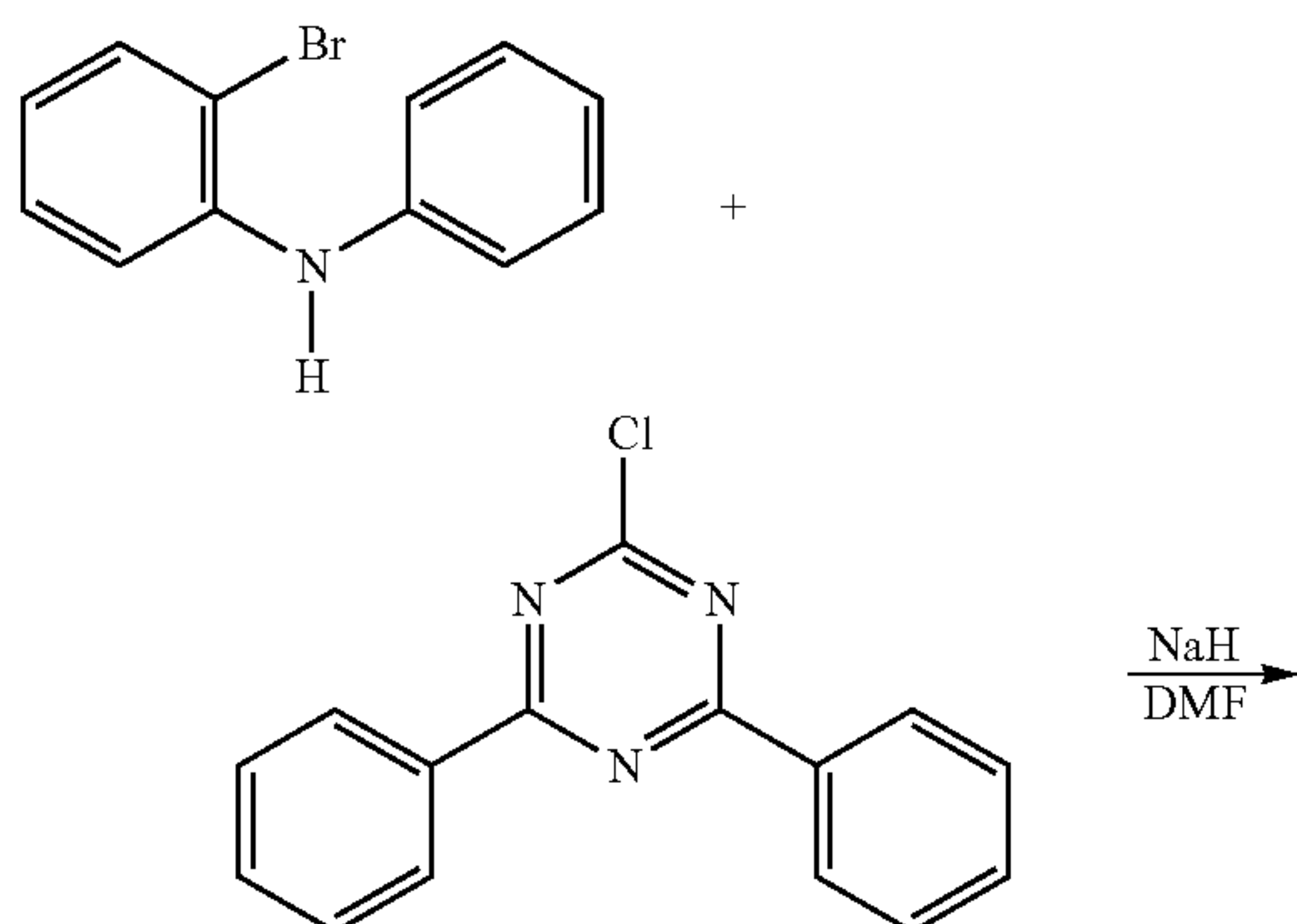
[Reaction Scheme 1]
