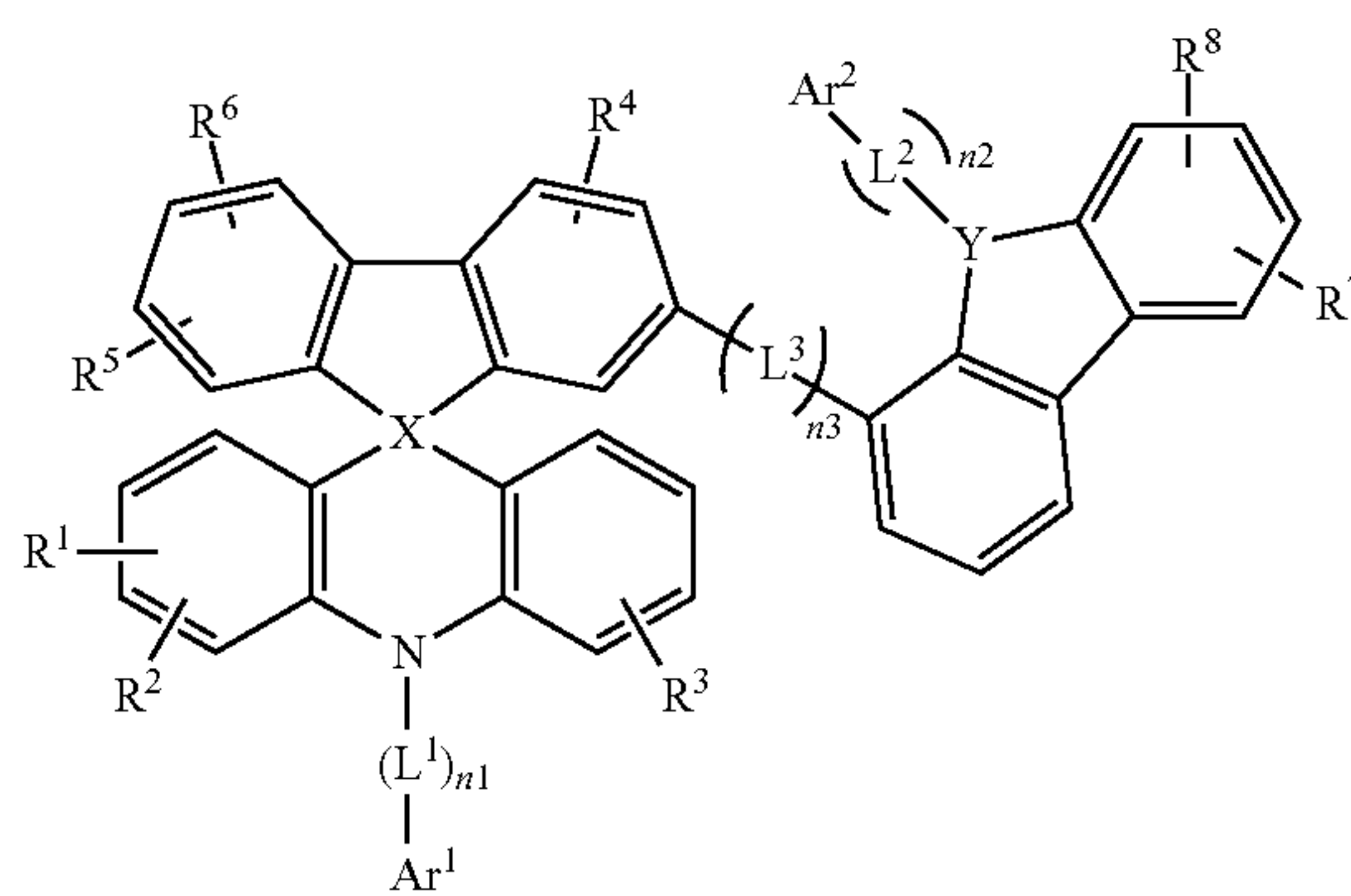
[Chemical Formula 2-3]
