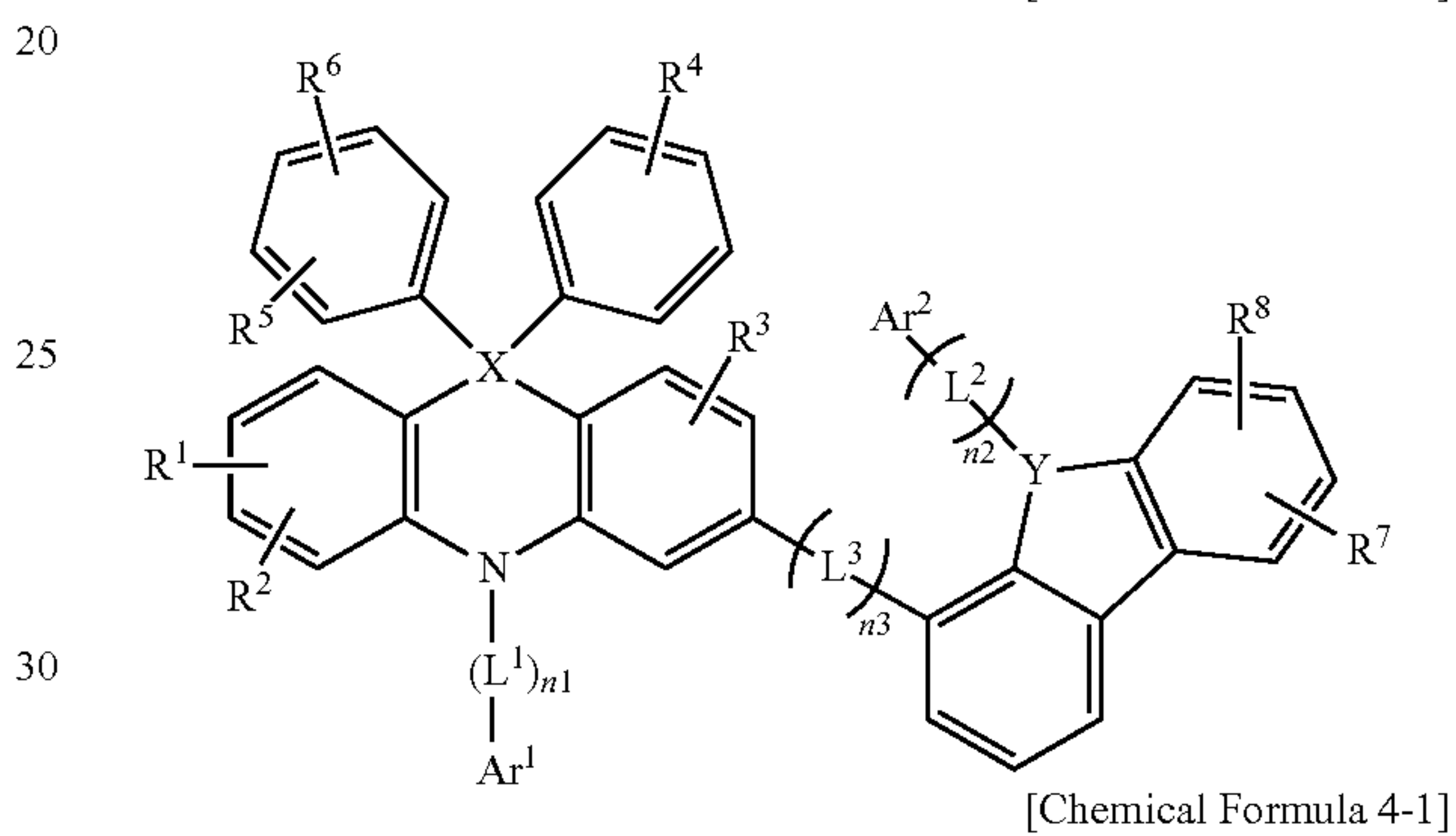
[Chemical Formula 2-6]
