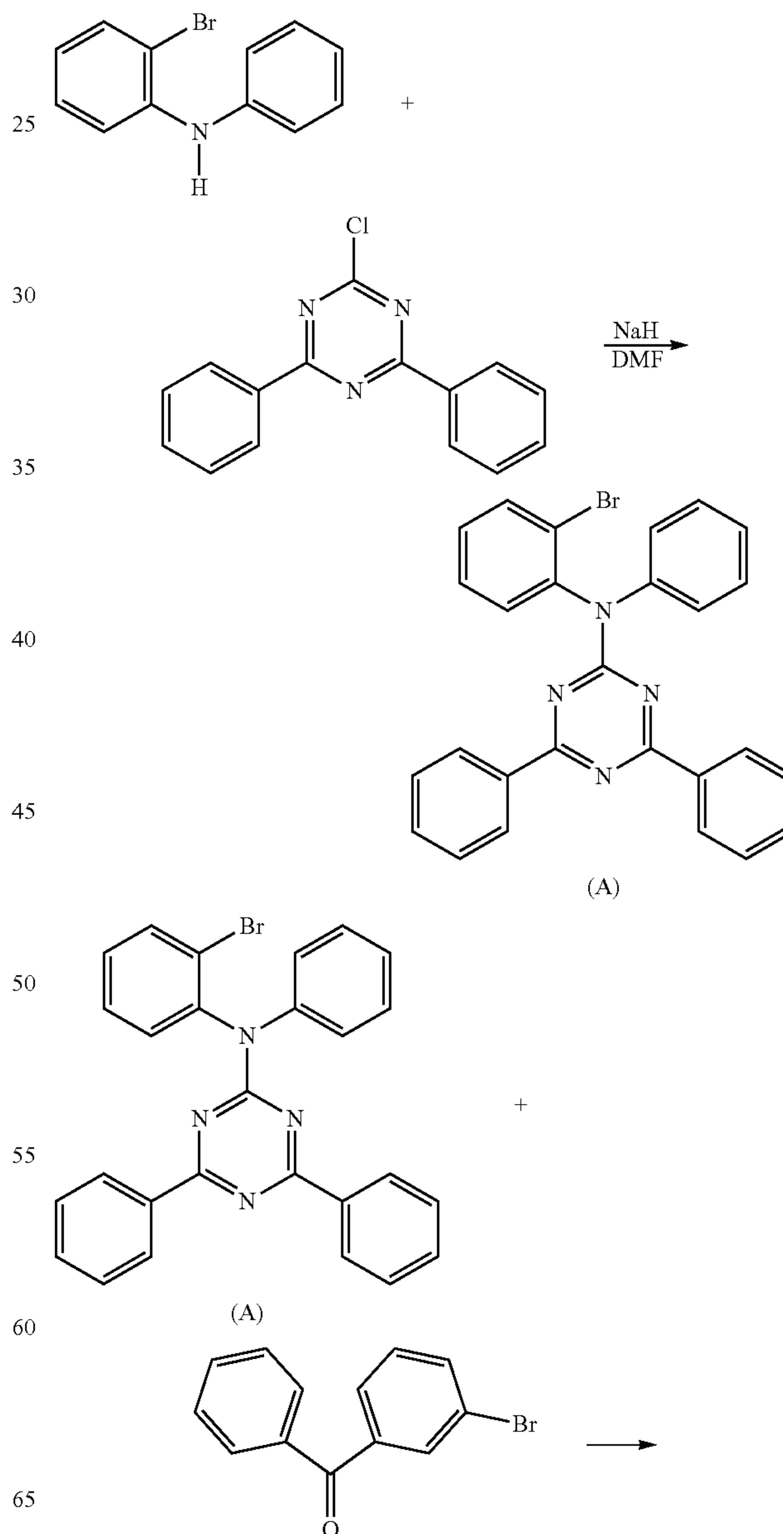
[Reaction Scheme 6]
