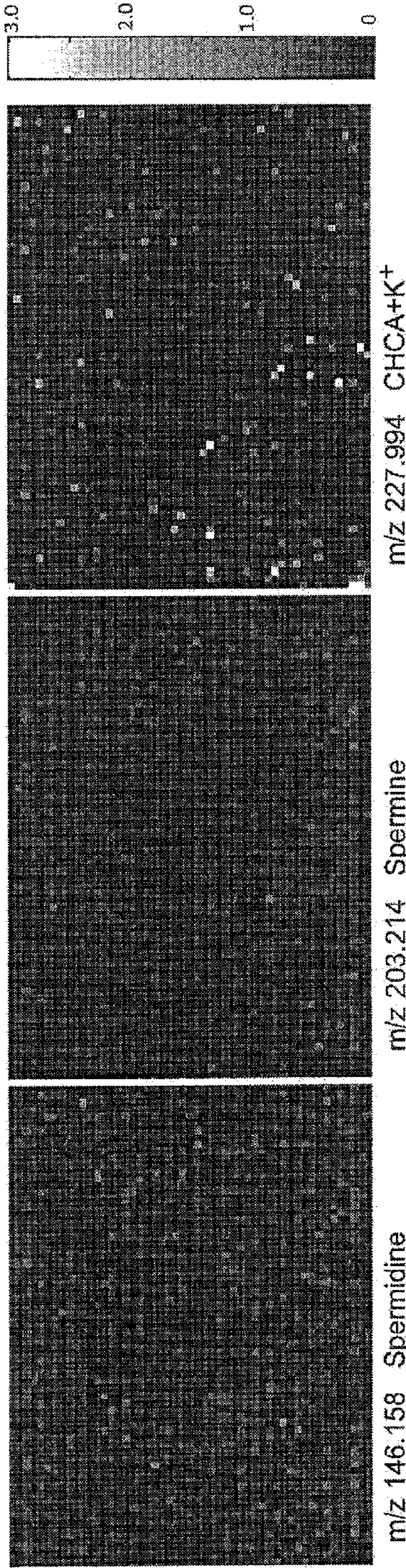
Fig. 12C MS IMAGING IMAGES
