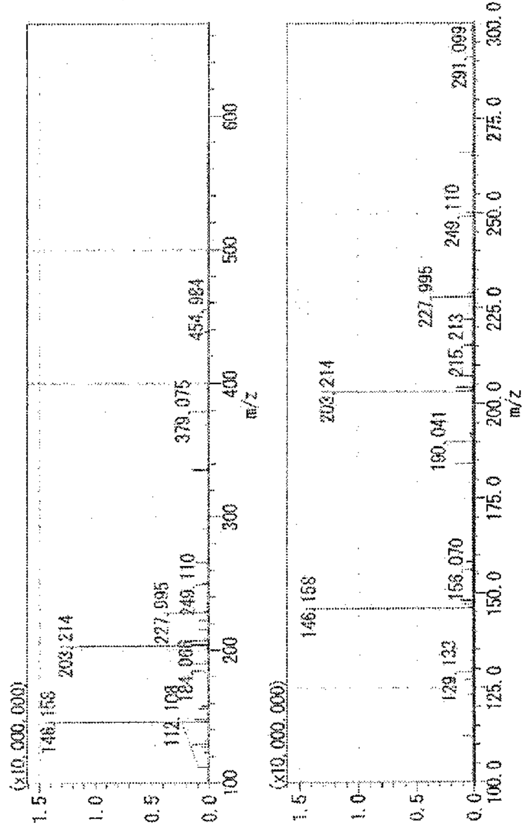
Fig. 15B MASS SPECTRUM
