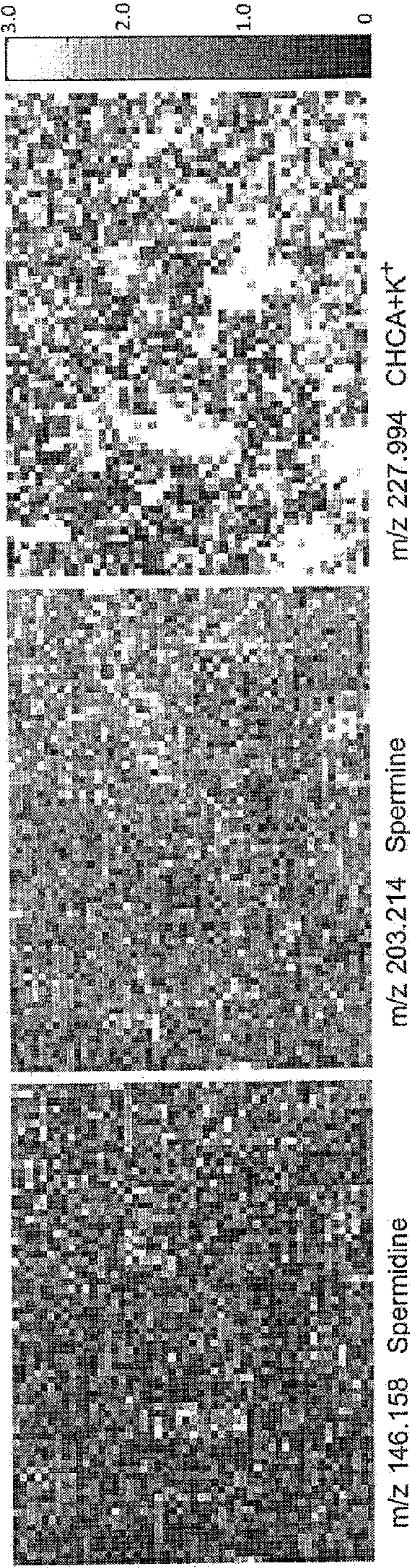
Fig. 14C MS IMAGING IMAGES
