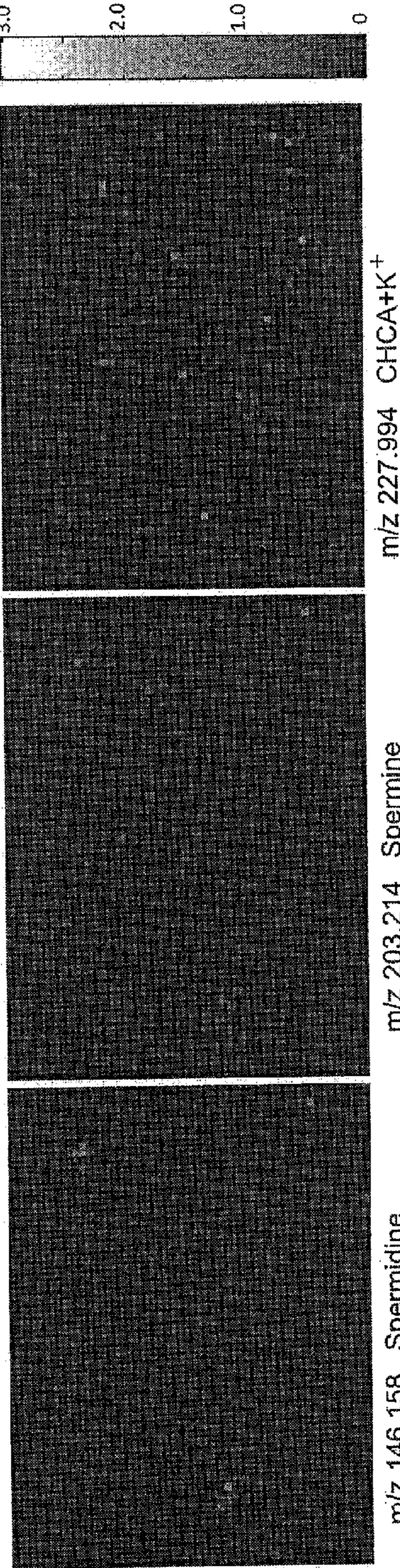
Fig. 13C MS IMAGING IMAGES
