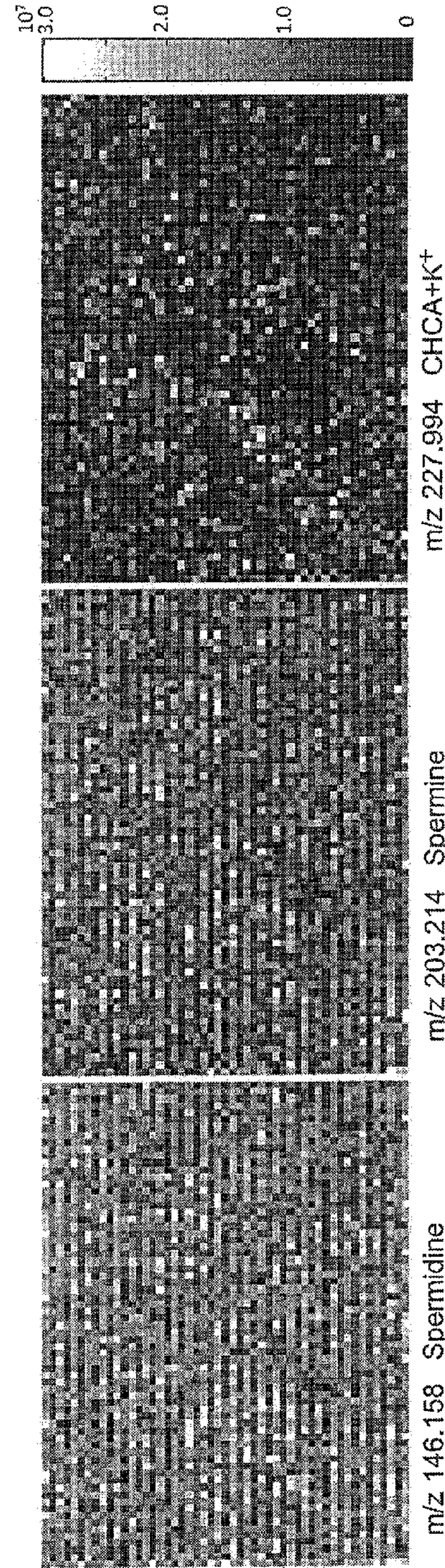
Fig. 15C MS IMAGING IMAGES
