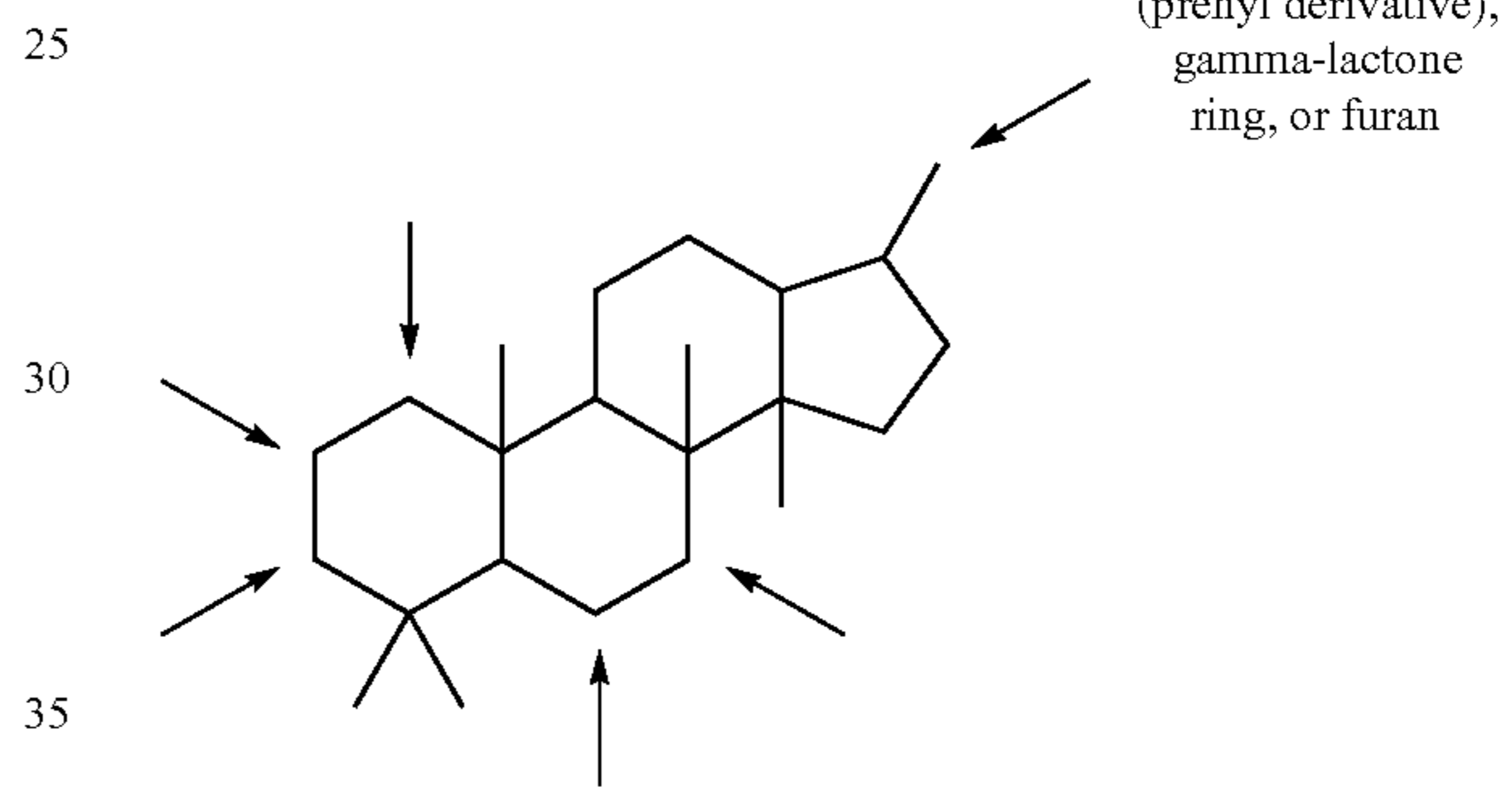
Cucurbitacin Core
