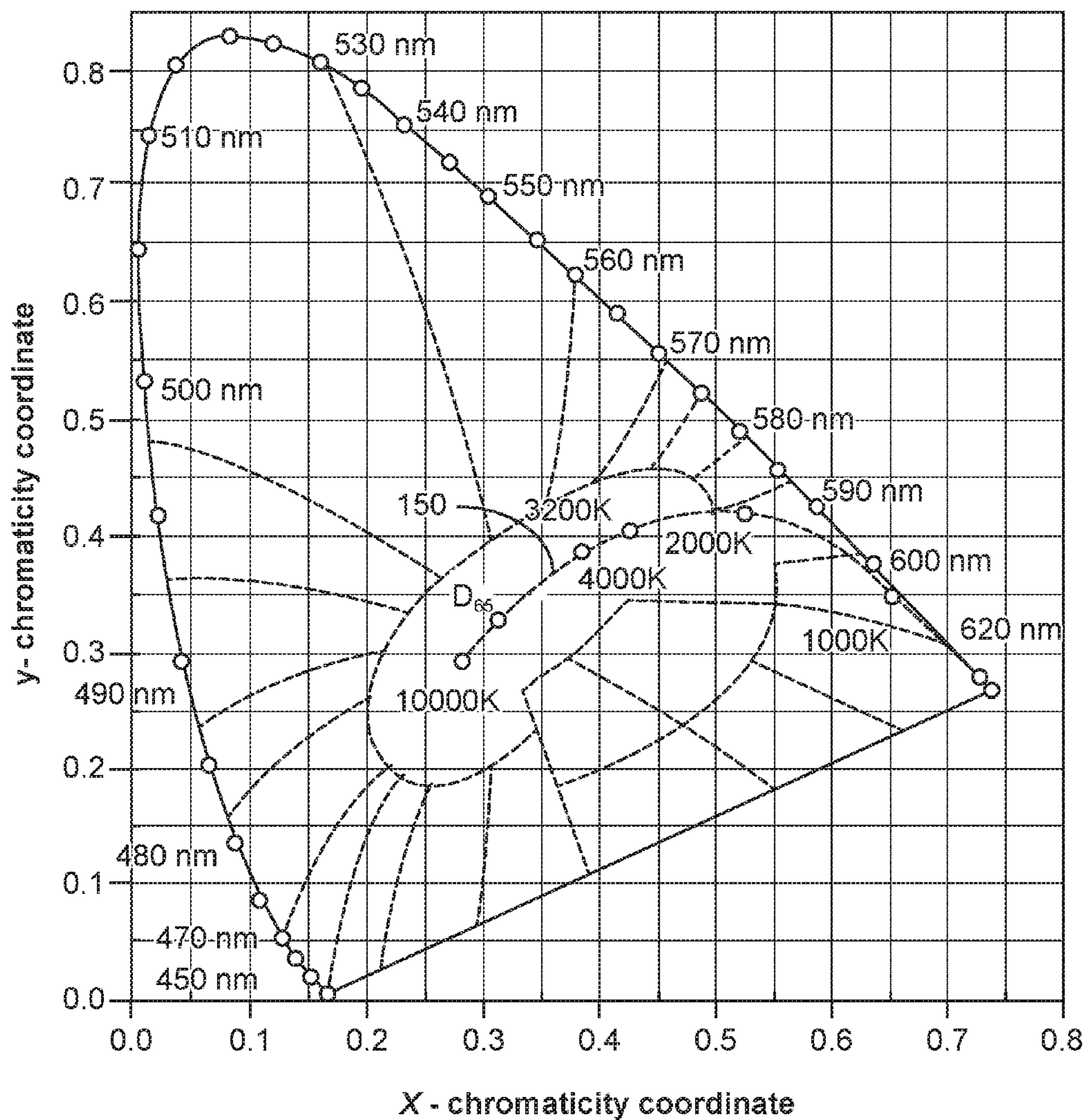
FIG. 3 PRIOR ART
