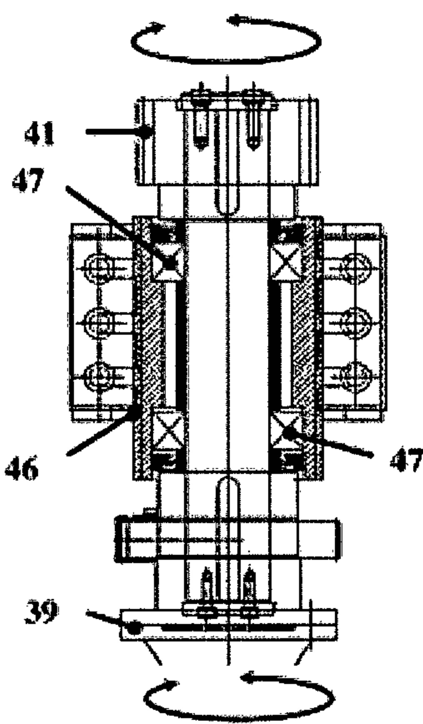
DETAIL B
