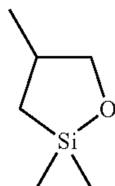
2,2,4-trimethyl-1-oxa-2-silacyclopentane
