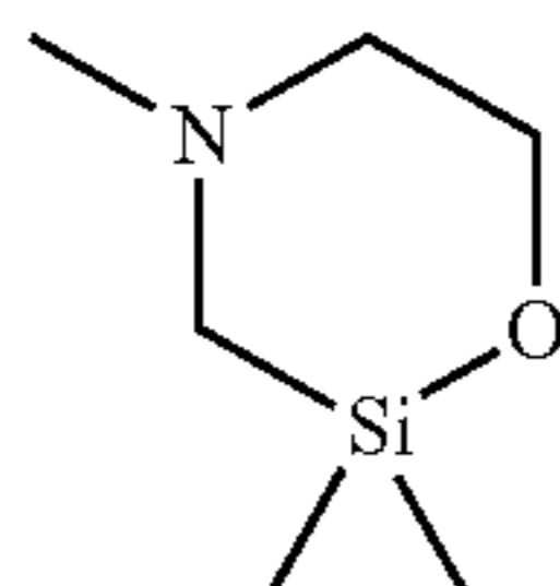
2,2,4-trimethyl-[1,4,2]oxazasilinane
