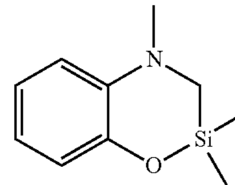
benzo-2,2,4-trimethyl-1-oxa-4-aza-2-silacyclohexane
