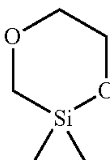
2,2-dimethyl-1,4-dioxo-2-silacyclohexane
