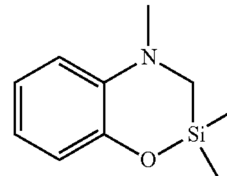
benzo-2,2,4-trimethyl-1-oxa-4-aza-2-silacyclohexane
