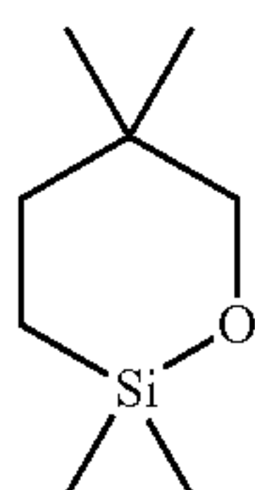
2,2,5,5-tetramethyl-1-oxa-2-silacyclohexane
