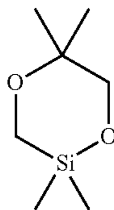
2,2,5,5-tetramethyl-1,4-dioxo-2,5-disilacyclohexane
