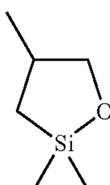
2,2,4-trimethyl-1-oxa-2-silacyclopentane
