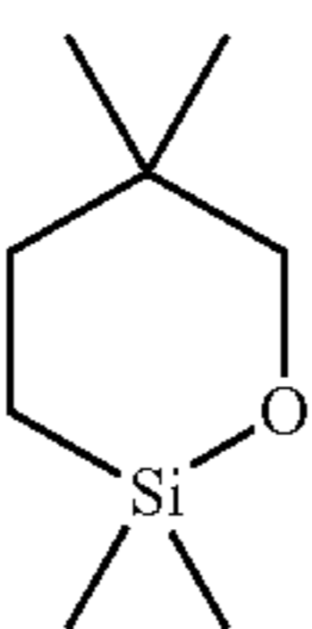
2,2,5,5-tetramethyl-1-oxa-2-silacyclohexane
