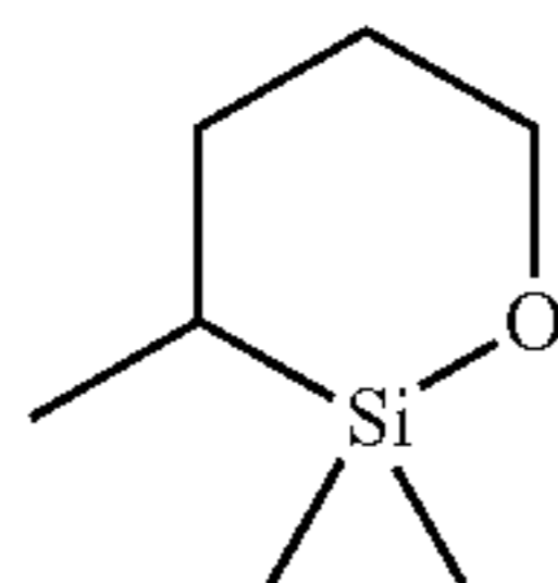
2,2,3-trimethyl-1-oxa-2-silacyclohexane
