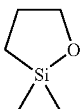
2,2-dimethyl-1-oxa-2-silacyclopentane
