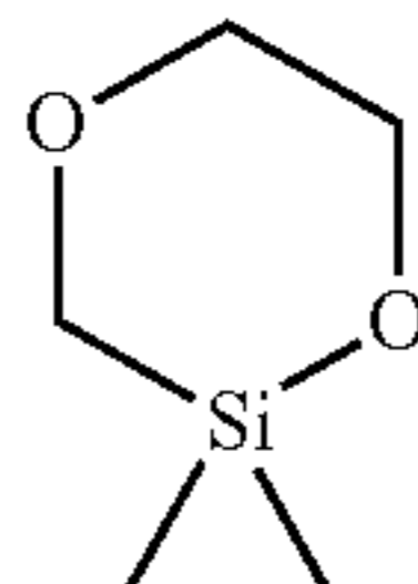
2,2-dimethyl-1,4-dioxo-2-silacyclohexane
