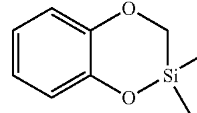
benzo-2,2-dimethyl-1,4-dioxo-2-silacyclohexane
