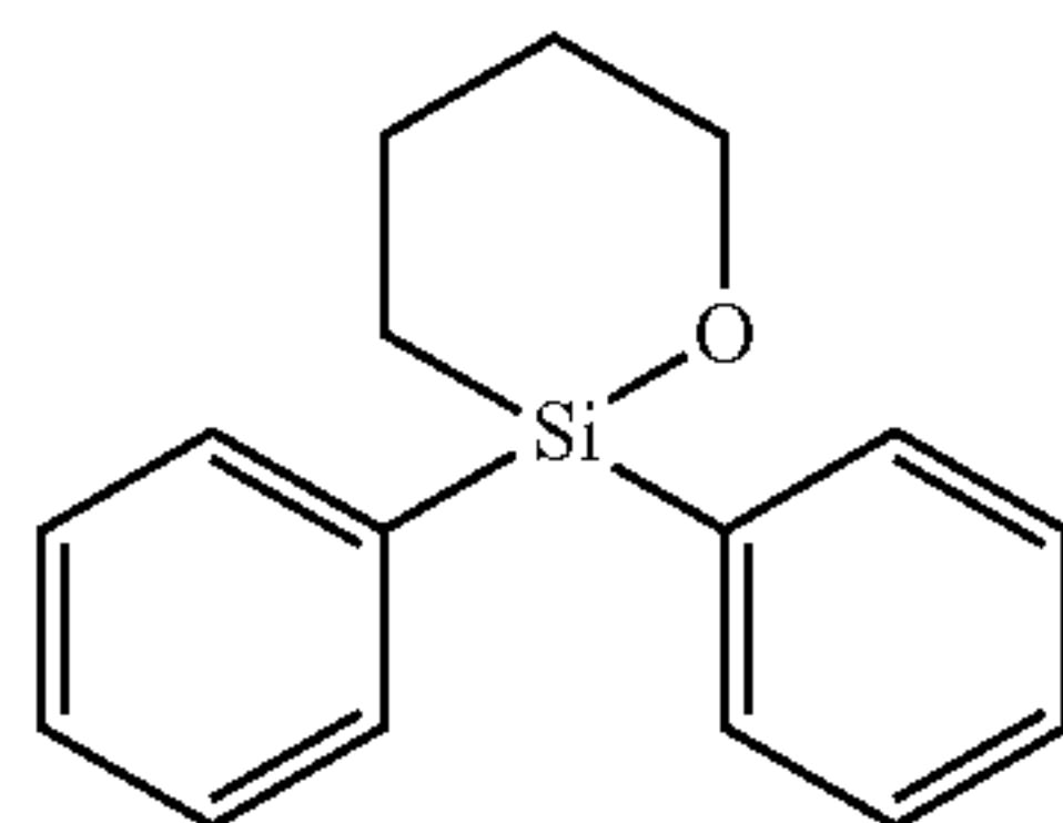
2,2-diphenyl-1-oxa-2-silacyclohexane
