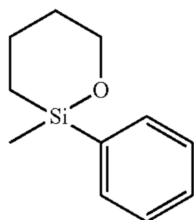
2-methyl-2-phenyl-1-oxa-2-silacyclohexane
