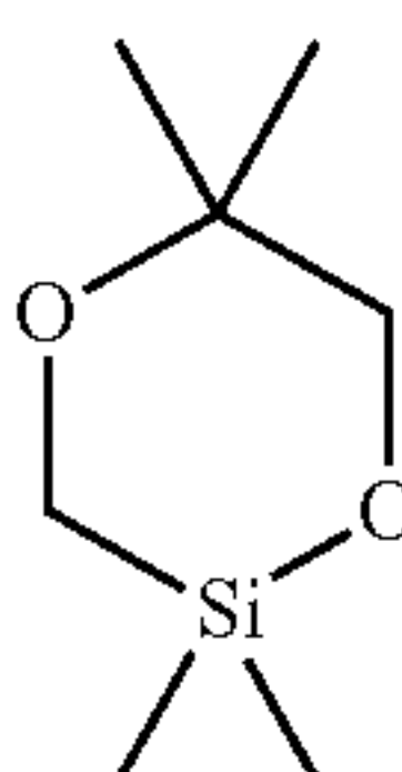
2,2,5,5-tetramethyl-1,4-dioxo-2,5-disilacyclohexane
