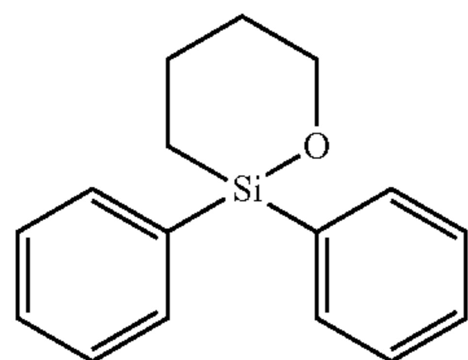
2,2-diphenyl-1-oxa-2-silacyclohexane
