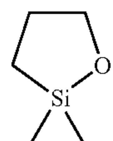
2,2-dimethyl-1-oxa-2-silacyclopentane
