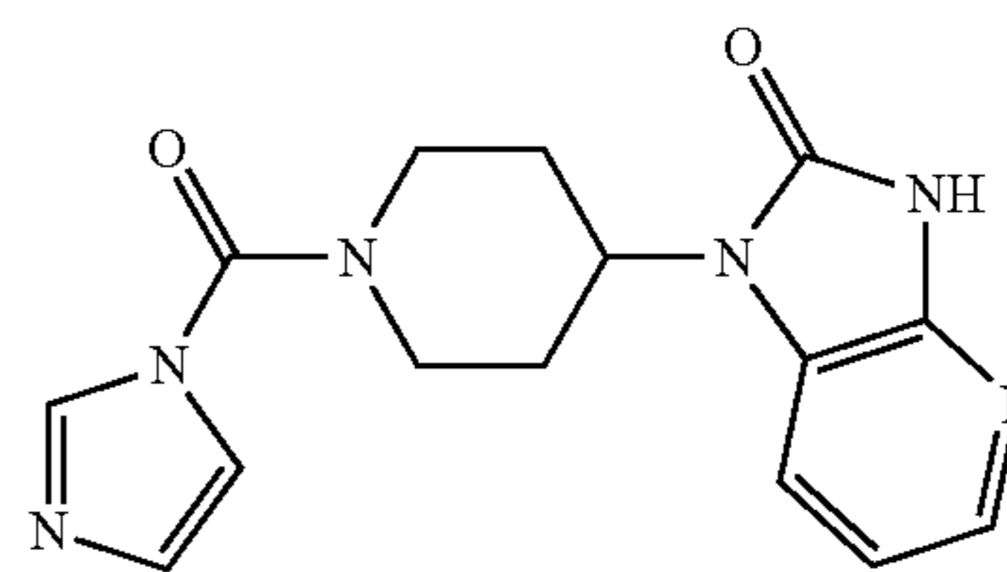
1-(1-(1H-imidazole-1-carbonyl)piperidin-4-yl)-1H-imidazo[4,5-b]pyridin-2(3H)-one
