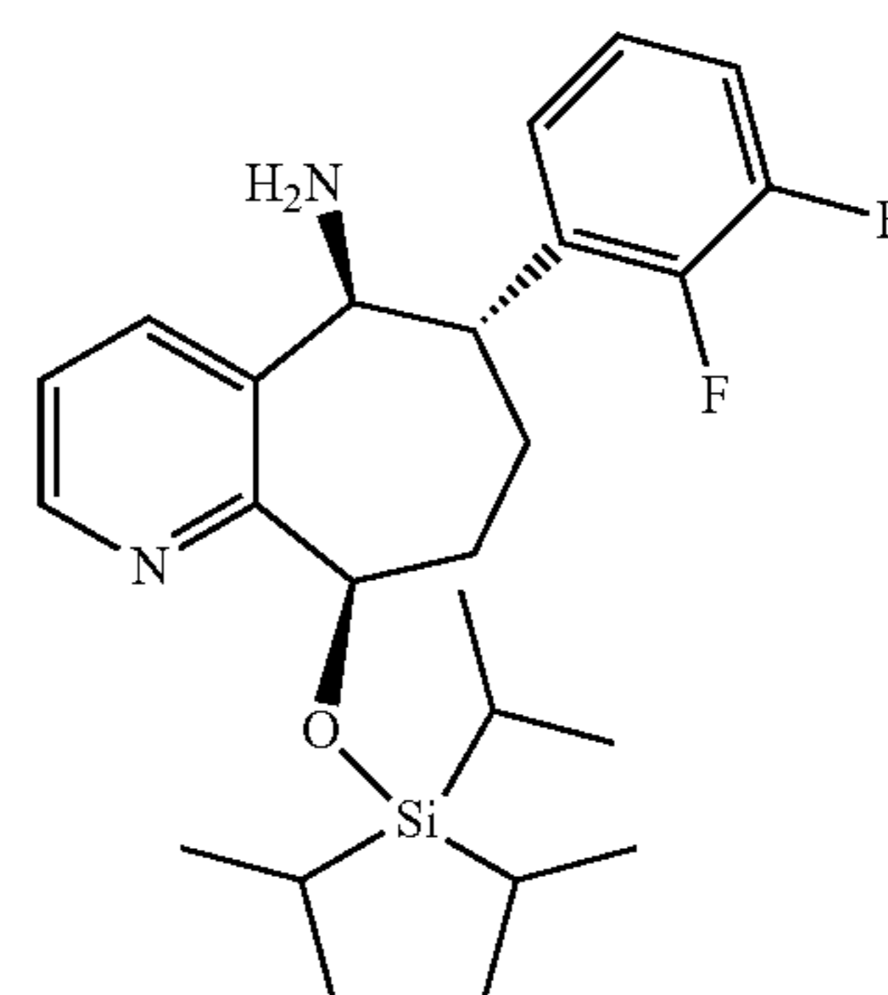
(6S,9R)-6-(2,3-difluorophenyl)-9-(triisopropylsilyloxy)-6,7,8,9-tetrahydro-5H-cyclohepta[b]pyridin-5-amine
