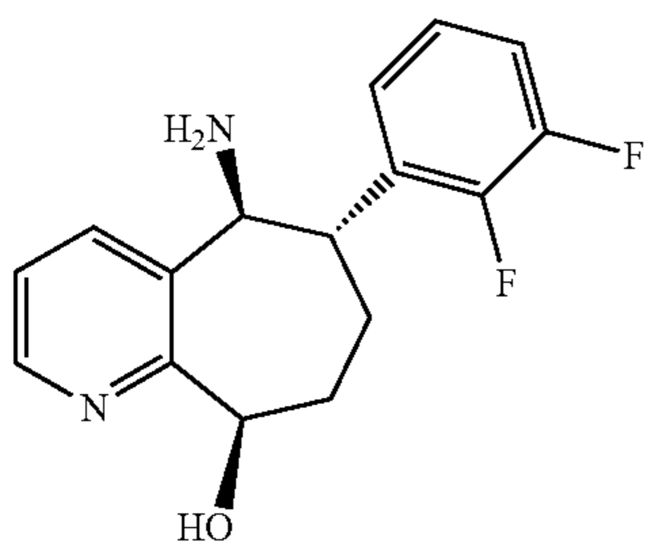
(6S,9R)-5-amino-6-(2,3-difluorophenyl)-6,7,8,9-tetrahydro-5H-cyclohepta[b]pyridin-9-ol
