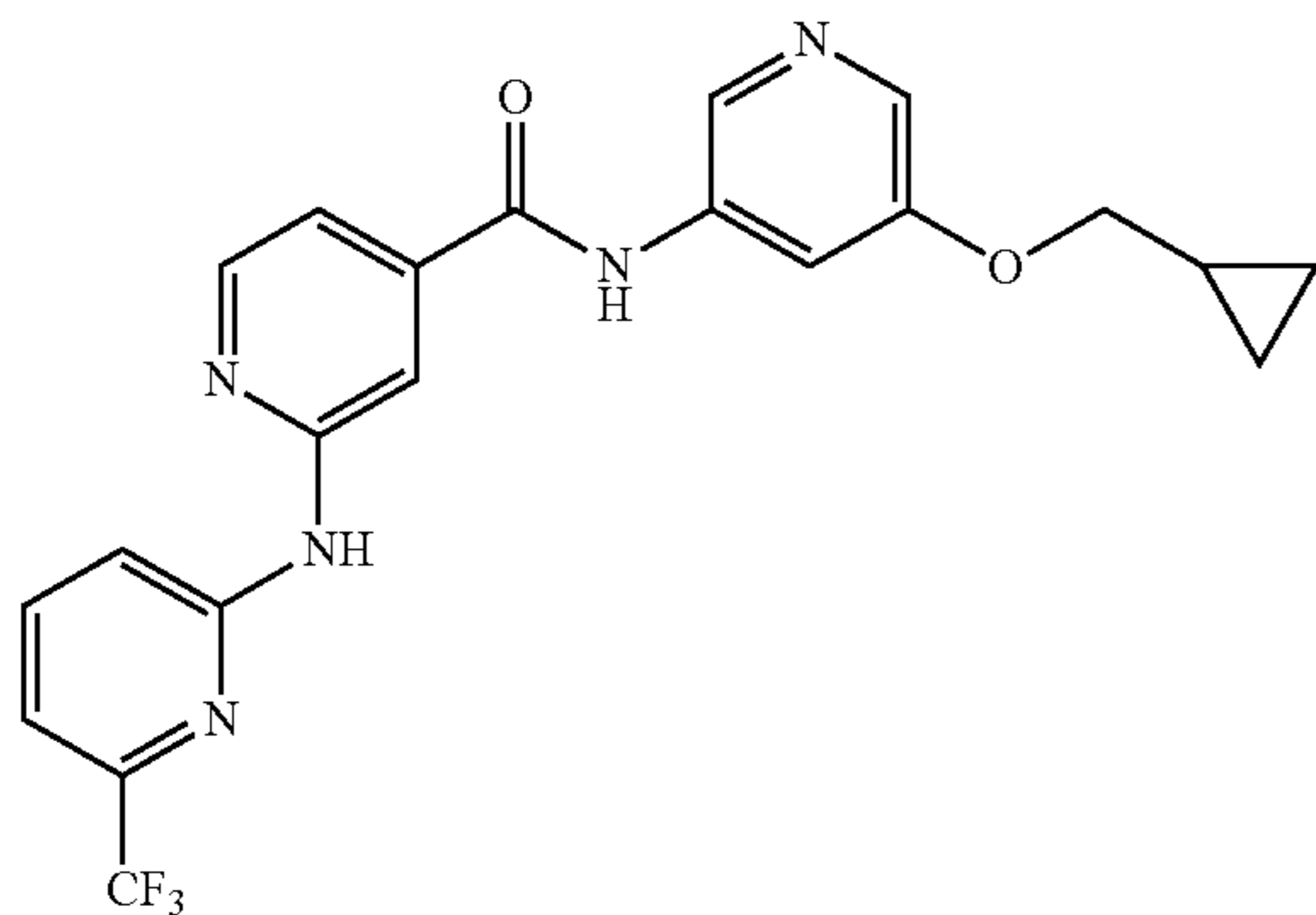
N-(5-(Cyclopropylmethoxy)pyridin-3-yl)-2-((6-(trifluoromethyl)pyridin-2-yl)amino)isonicotinamide
