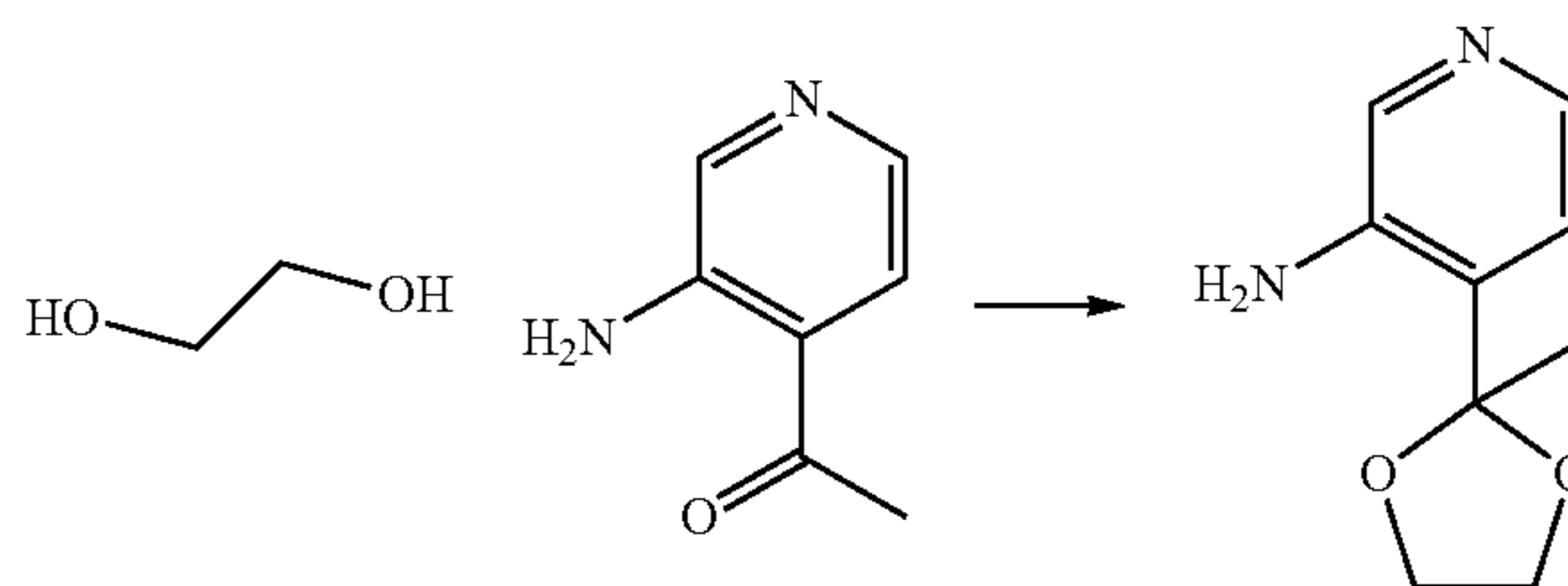
4-(2-Methyl-1,3-dioxolan-2-yl)pyridin-3-amine
