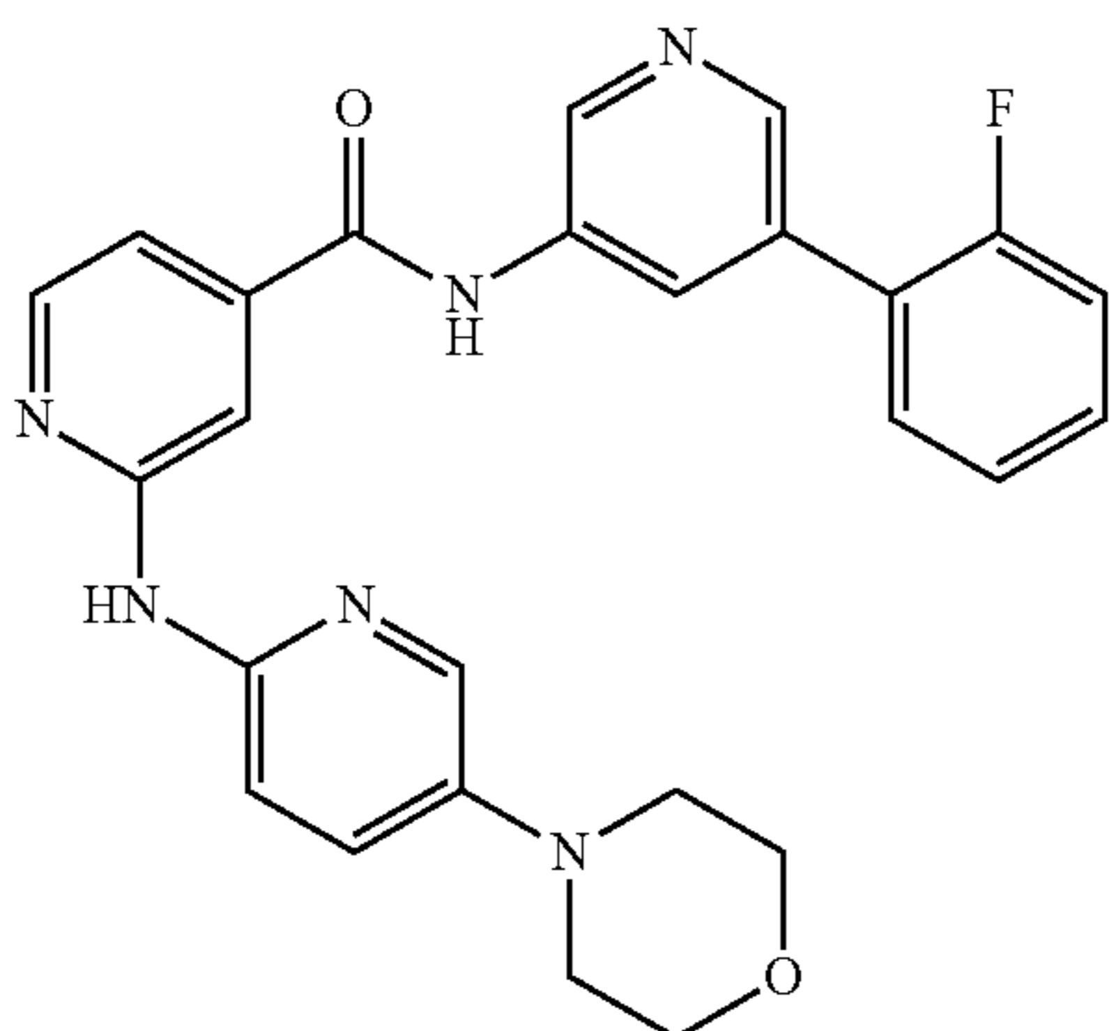
N-(5-(2-Fluorophenyl)pyridin-3-yl)-2-((5-morpholinopyridin-2-yl)amino)isonicotinamide
