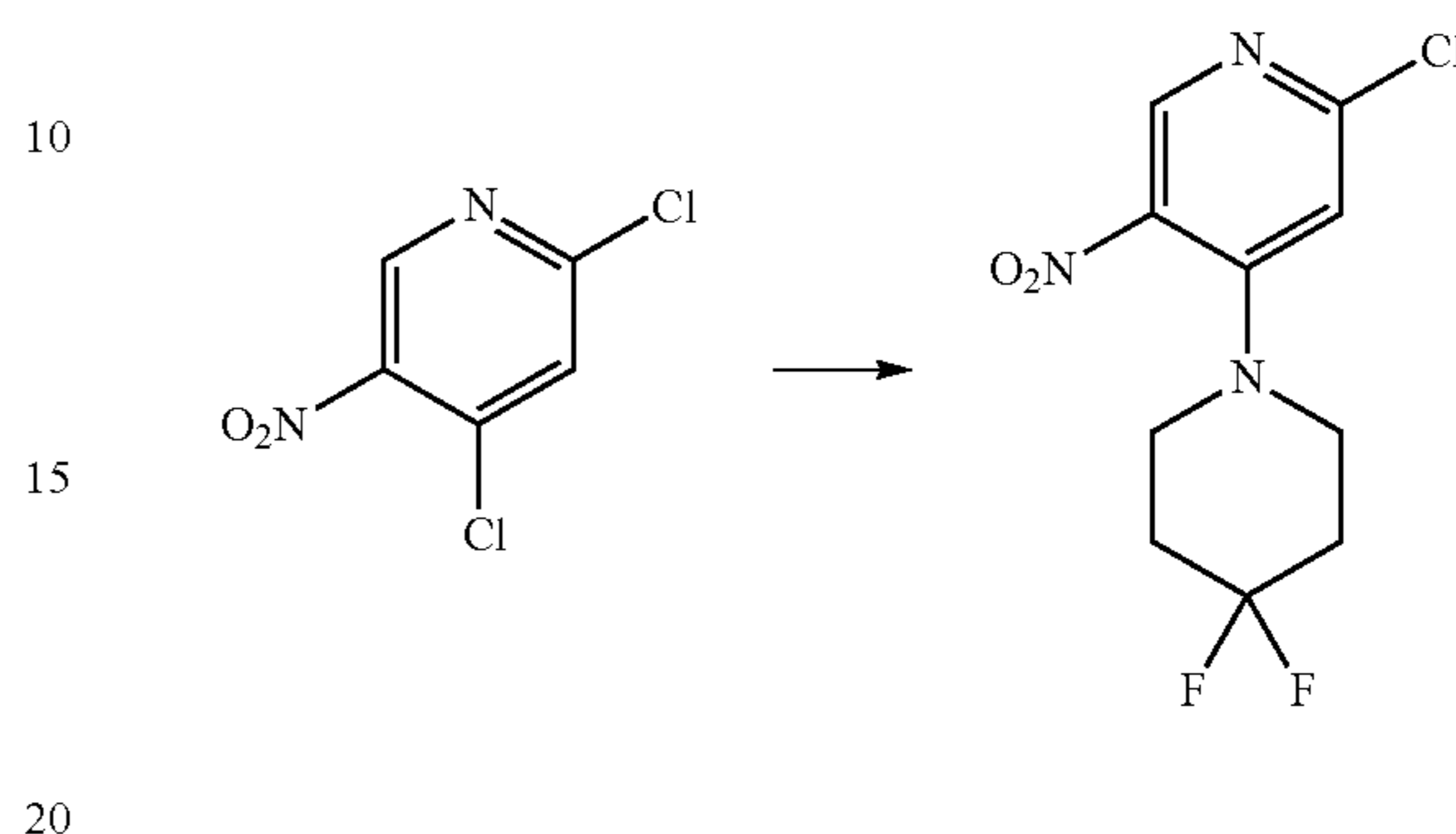
2-Chloro-4-(4,4-difluoropiperidin-1-yl)-5-nitropyridine
