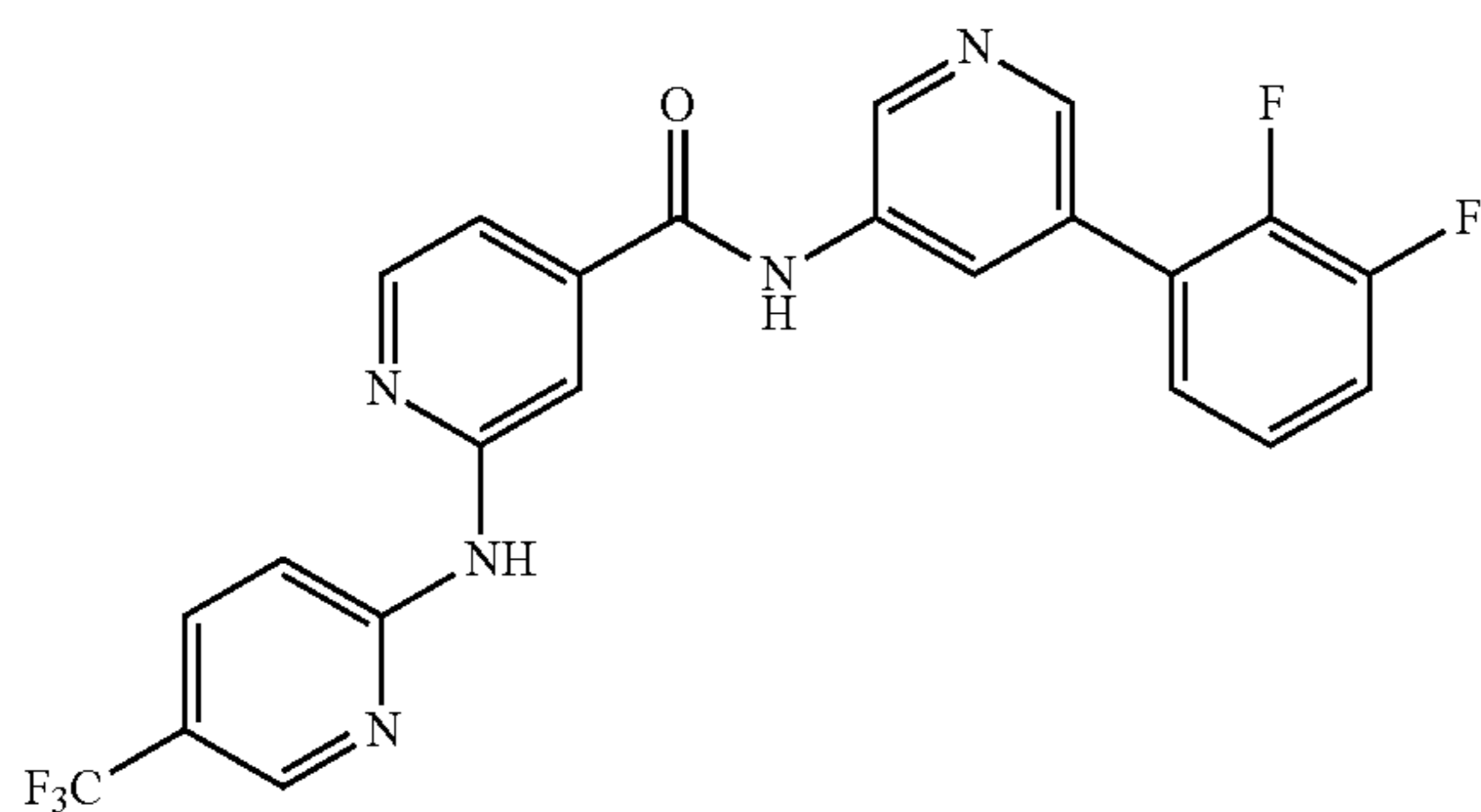
N-(5-(2,3-Difluorophenyl)pyridin-3-yl)-2-((5-(trifluoromethyl)pyridin-2-yl)amino)isonicotinamide
