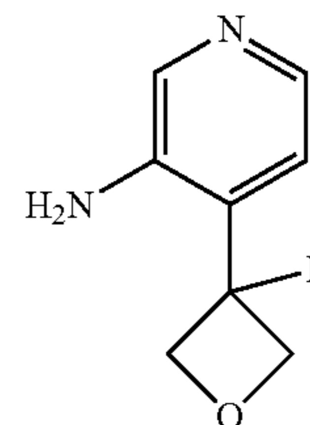
4-(3-Fluorooxetan-3-yl)pyridin-3-amine
