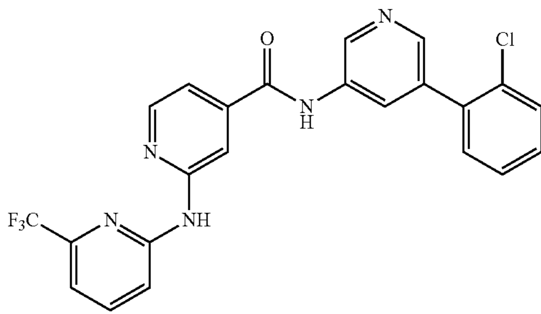
N-(5-(2-Chlorophenyl)pyridin-3-yl)-2-((6-(trifluoromethyl)pyridin-2-yl)amino)isonicotinamide
