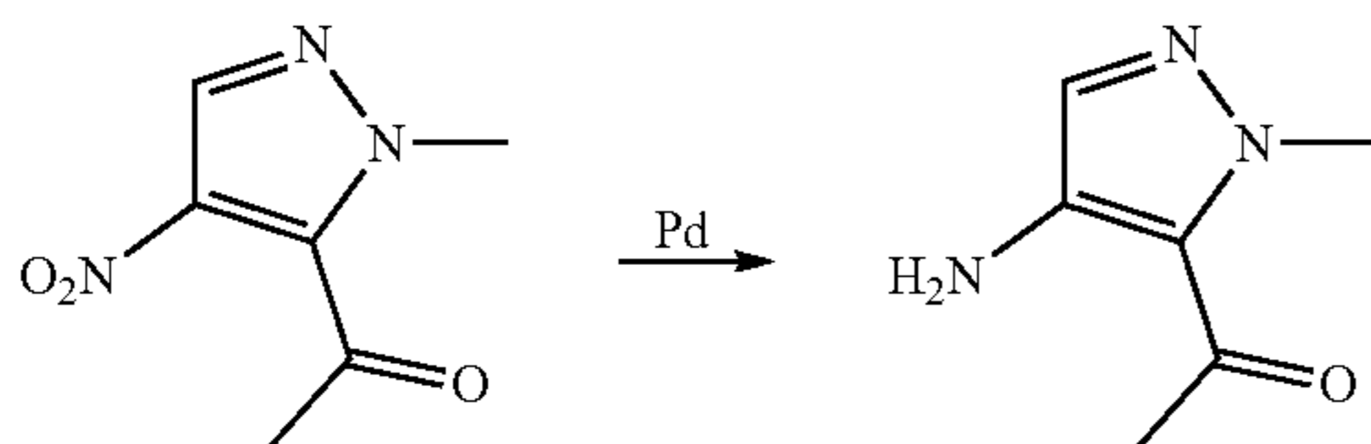
1-(4-Amino-1-methyl-1H-pyrazol-5-yl)ethanone
