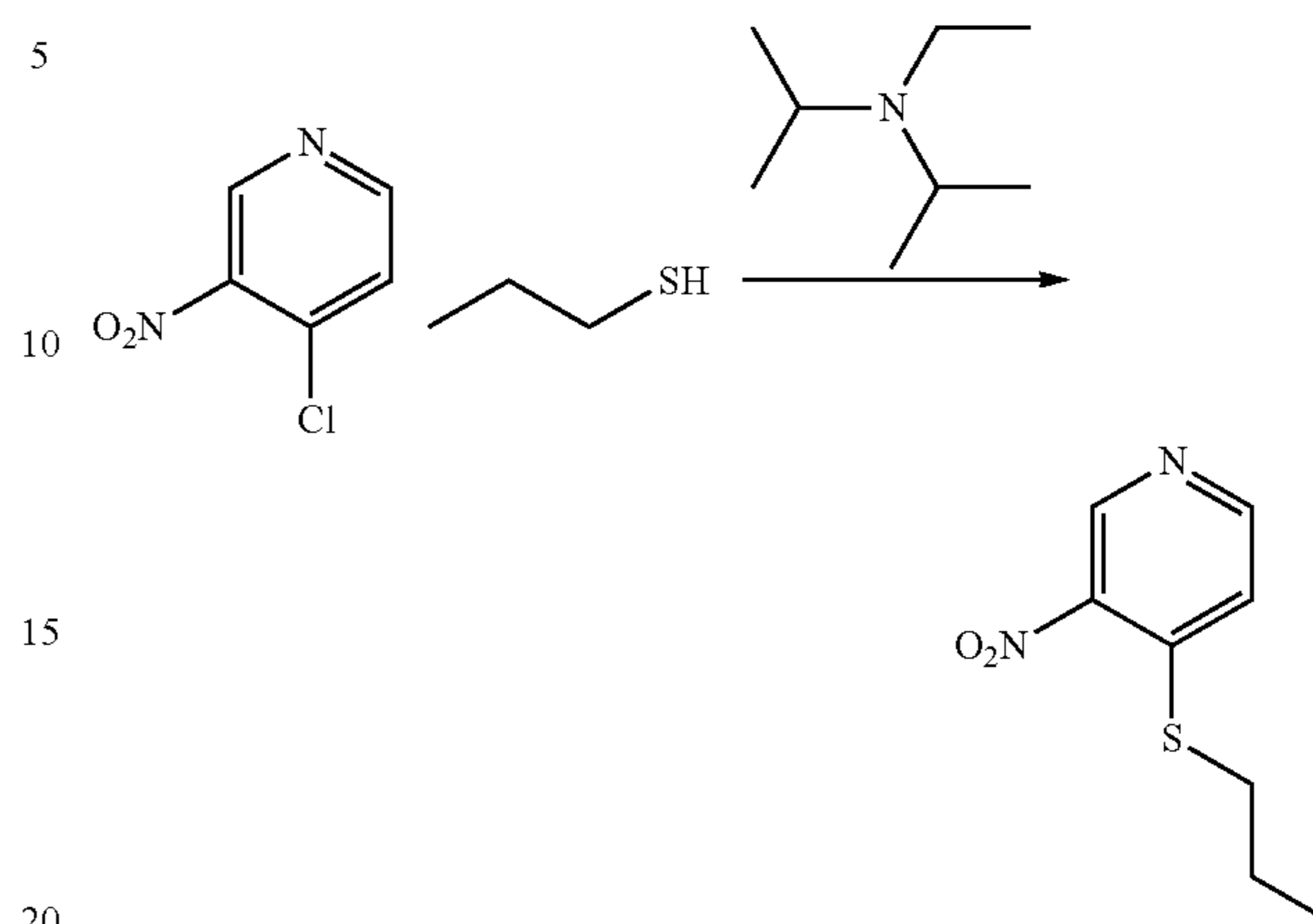
3-Nitro-4-(propylthio)pyridine
