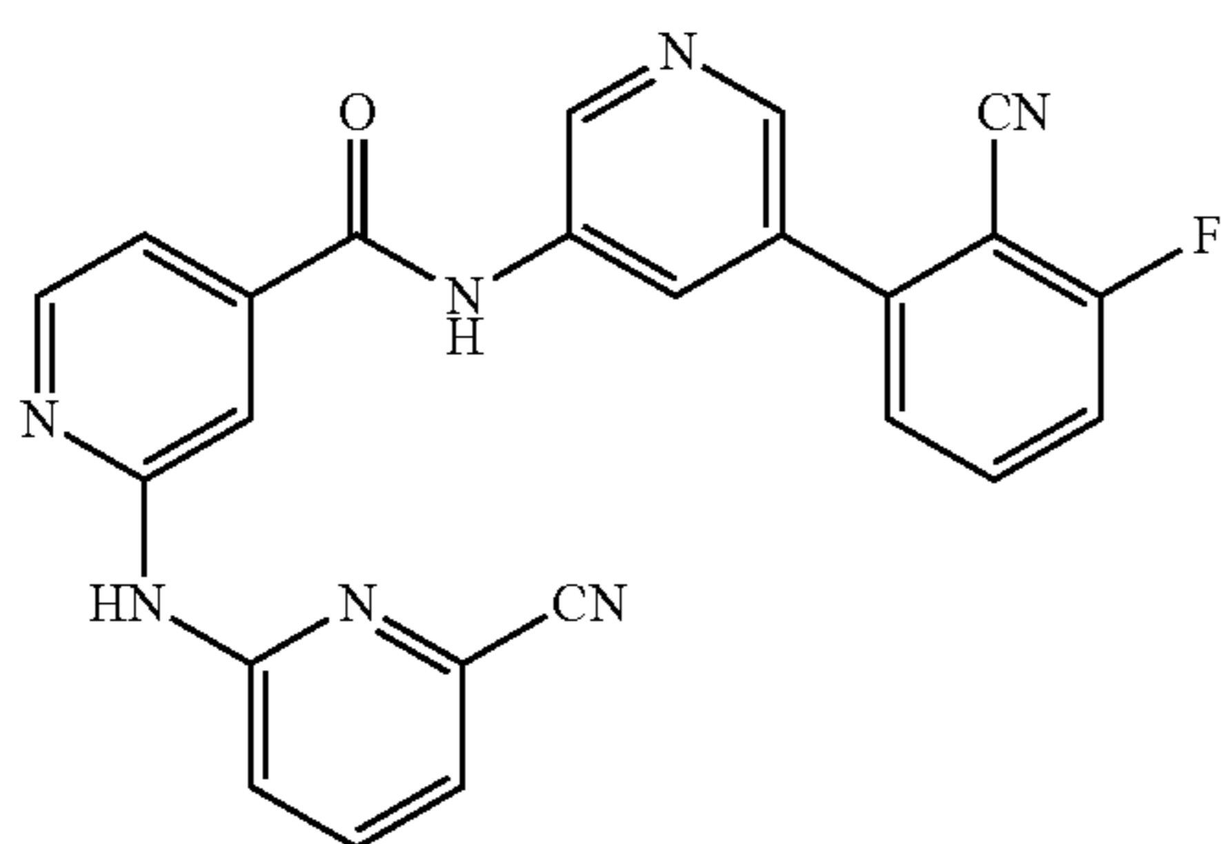
N-(5-(2-Cyano-3-fluorophenyl)pyridin-3-yl)-2-((6-cyanopyridin-2-yl)amino)isonicotinamide
