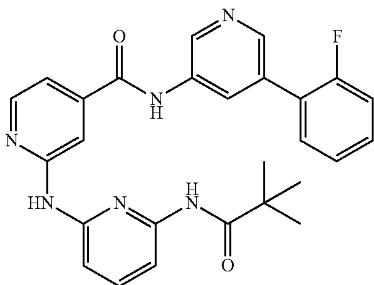
N-(5-(2-Fluorophenyl)pyridin-3-yl)-2-((6-pivalamidopyridin-2-yl)amino)isonicotinamide
