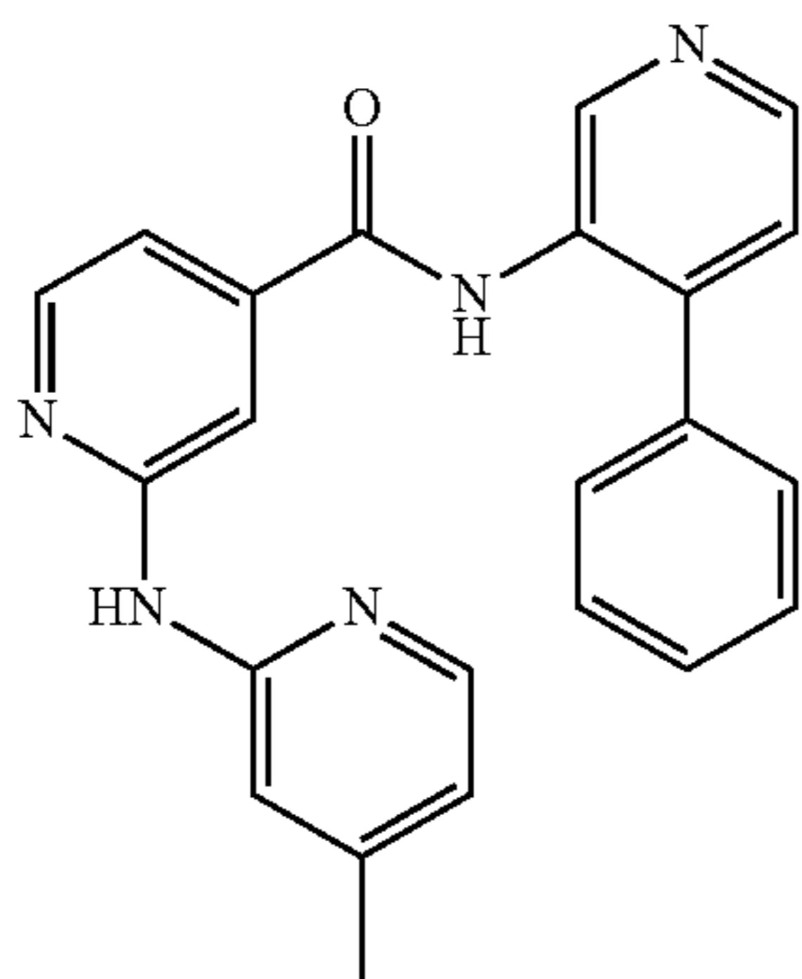
2-((4-Methylpyridin-2-yl)amino)-N-(4-phenylpyridin-3-yl)isonicotinamide
