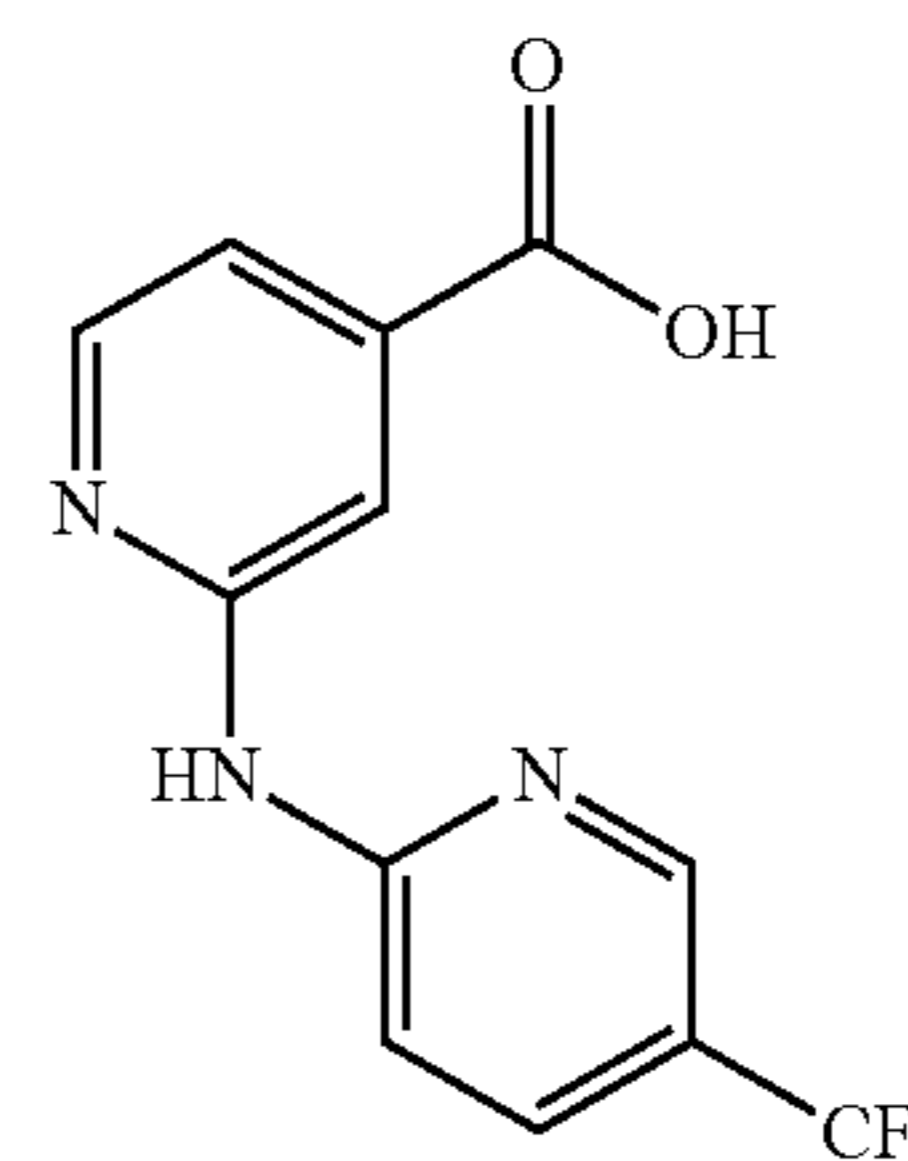
2-((5-(Trifluoromethyl)pyridin-2-yl)amino)isonicotinic acid
