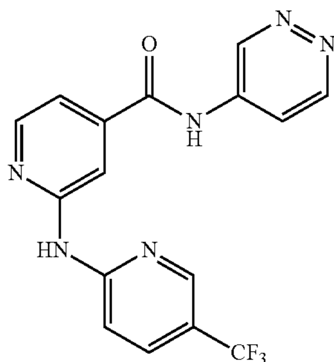
N-(Pyridazin-4-yl)-2-((5-(trifluoromethyl)pyridin-2-yl)amino)isonicotinamide
