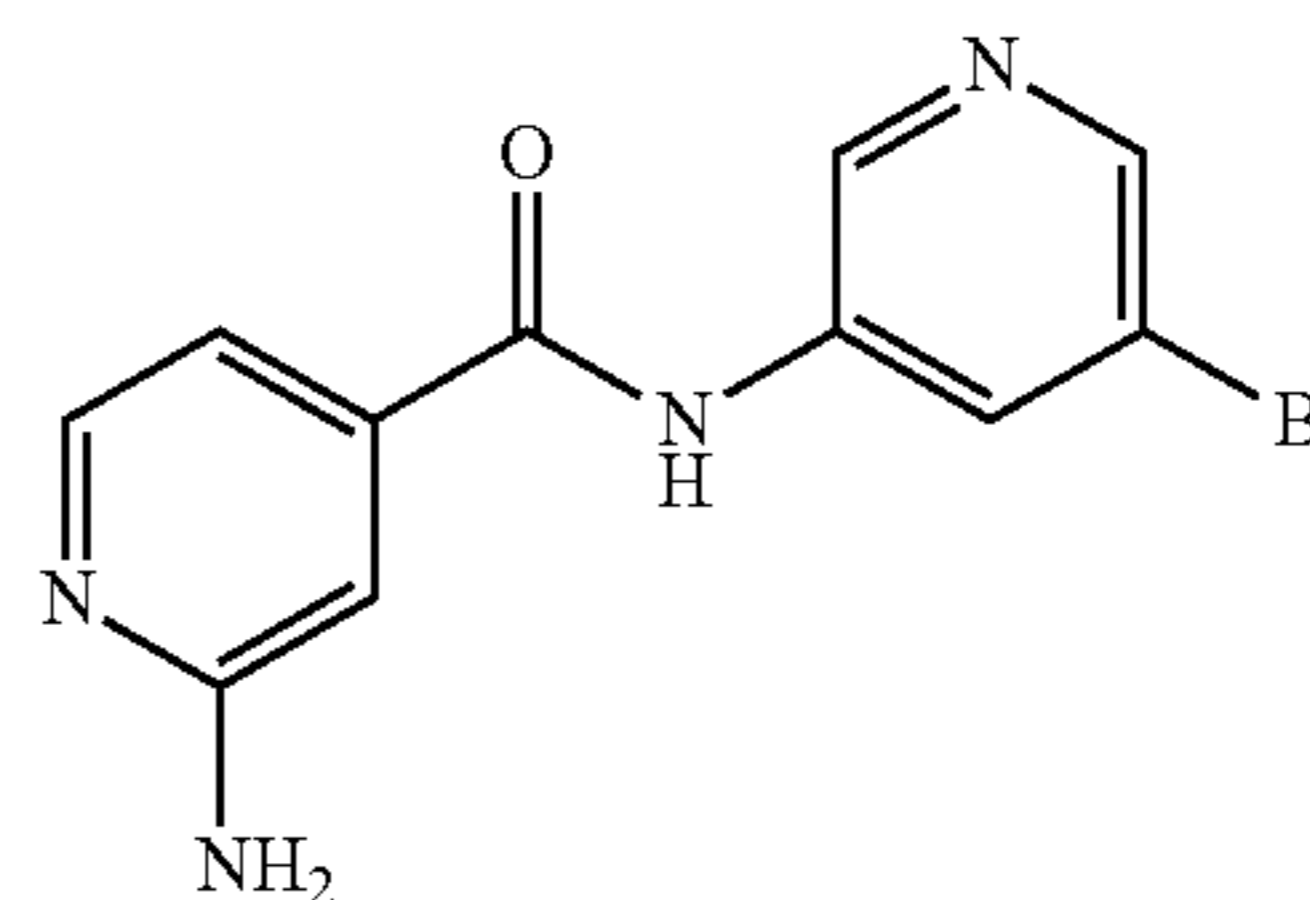
2-Amino-N-(5-bromopyridin-3-yl)isonicotinamide
