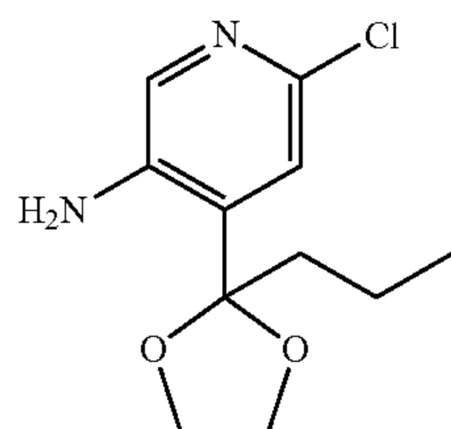
6-Chloro-4-(2-propyl-1,3-dioxolan-2-yl)pyridin-3-amine
