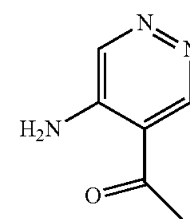
1-(5-Aminopyridazin-4-yl)ethanone
