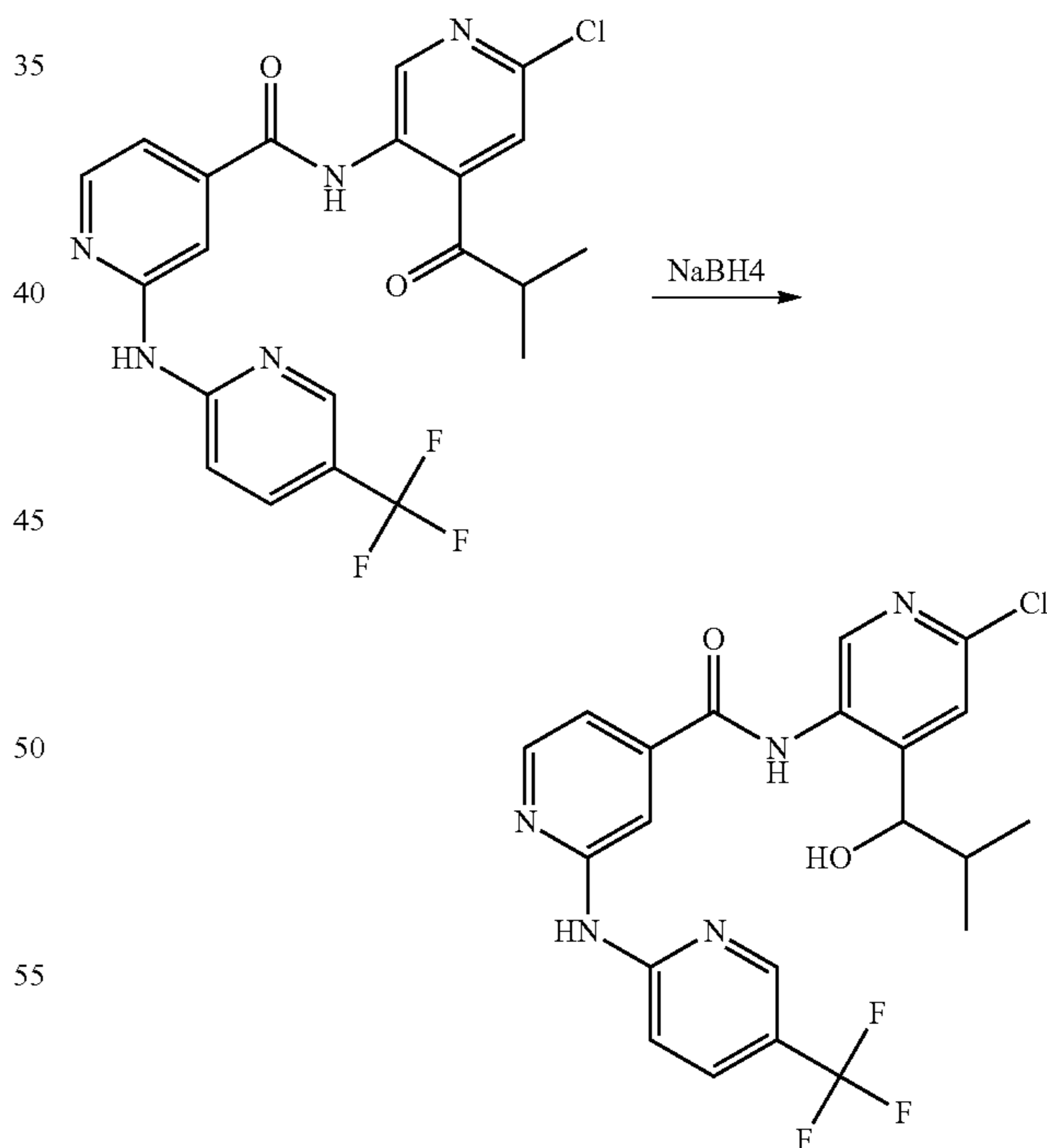
N-(6-Chloro-4-(1-hydroxy-2-methylpropyl)pyridin-3-yl)-2-((5-(trifluoromethyl)pyridin-2-yl)amino)isonicotinamide
