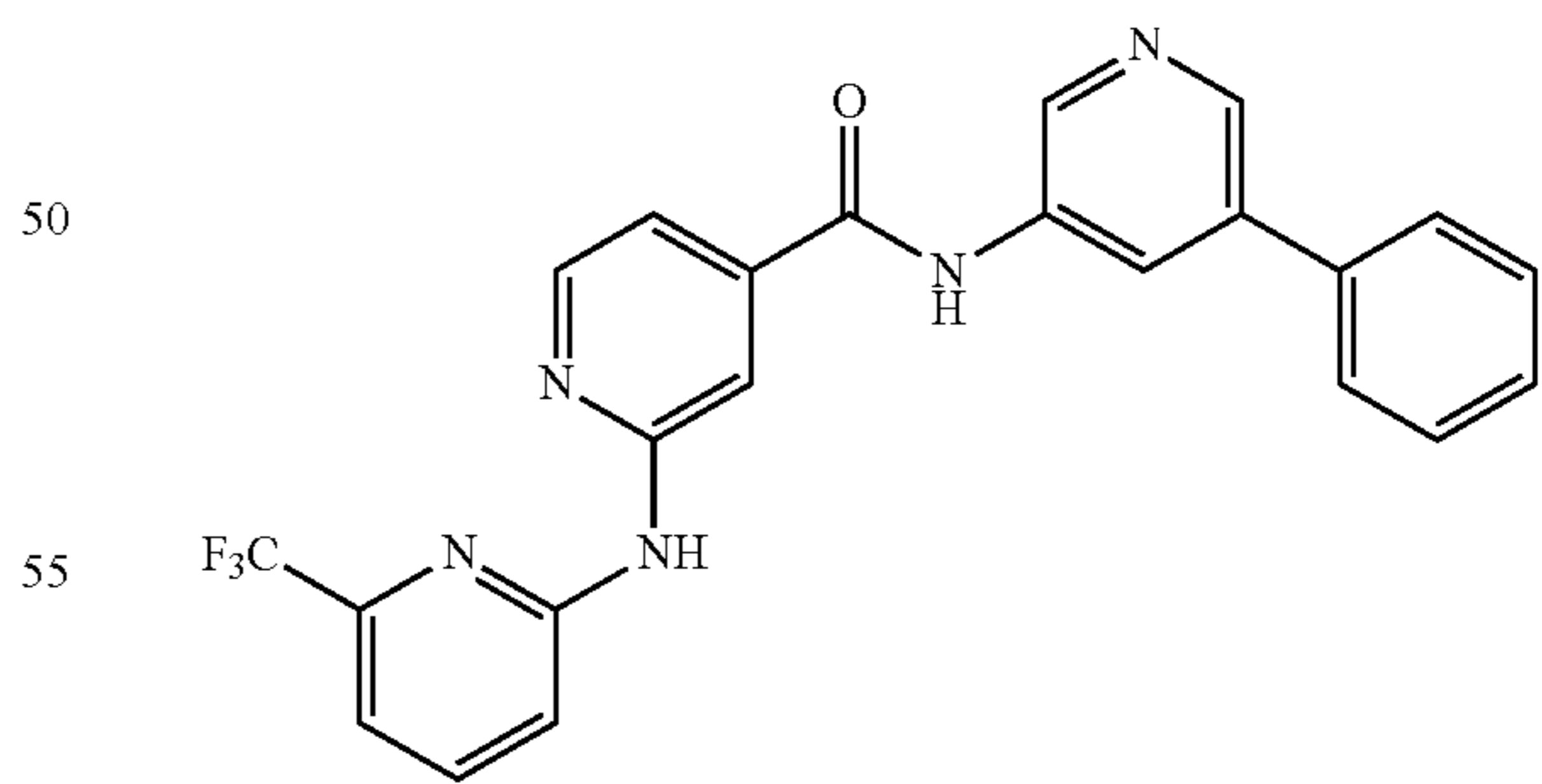
N-(5-Phenylpyridin-3-yl)-2-((6-(trifluoromethyl)pyridin-2-yl)amino)isonicotinamide
