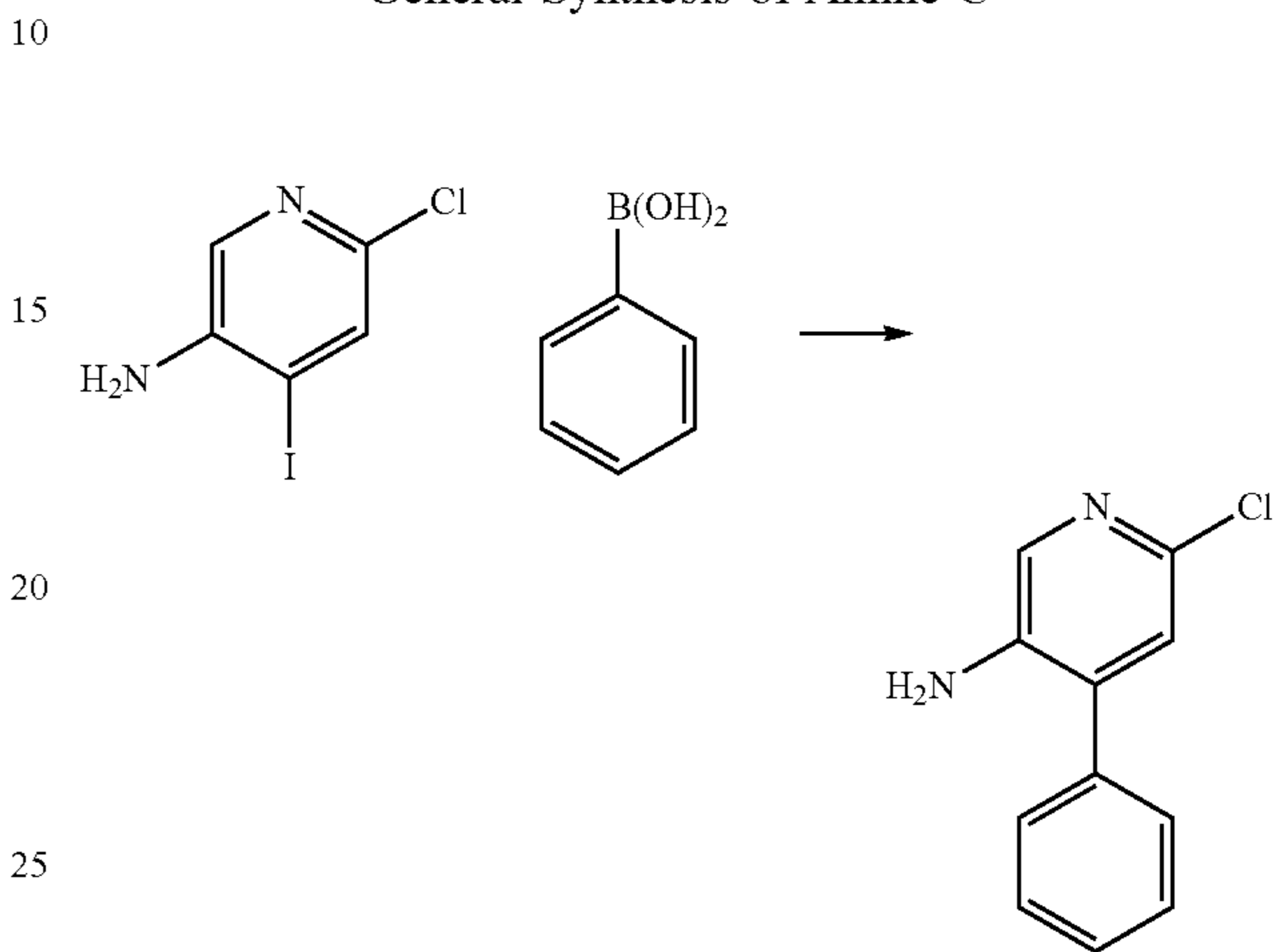
6-Chloro-4-phenylpyridin-3-amine
