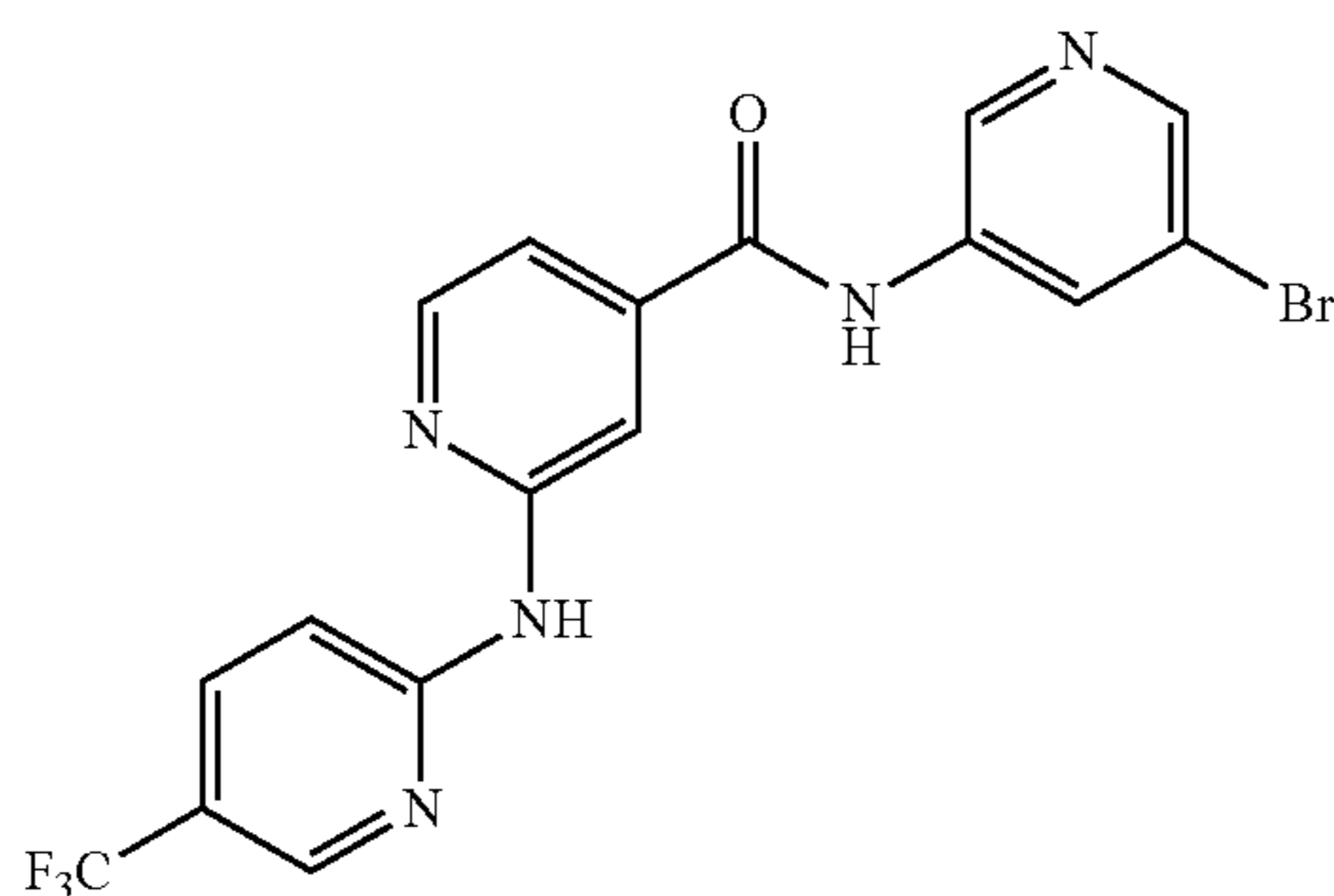
N-(5-Bromopyridin-3-yl)-2-((5-(trifluoromethyl)pyridin-2-yl)amino)isonicotinamide
