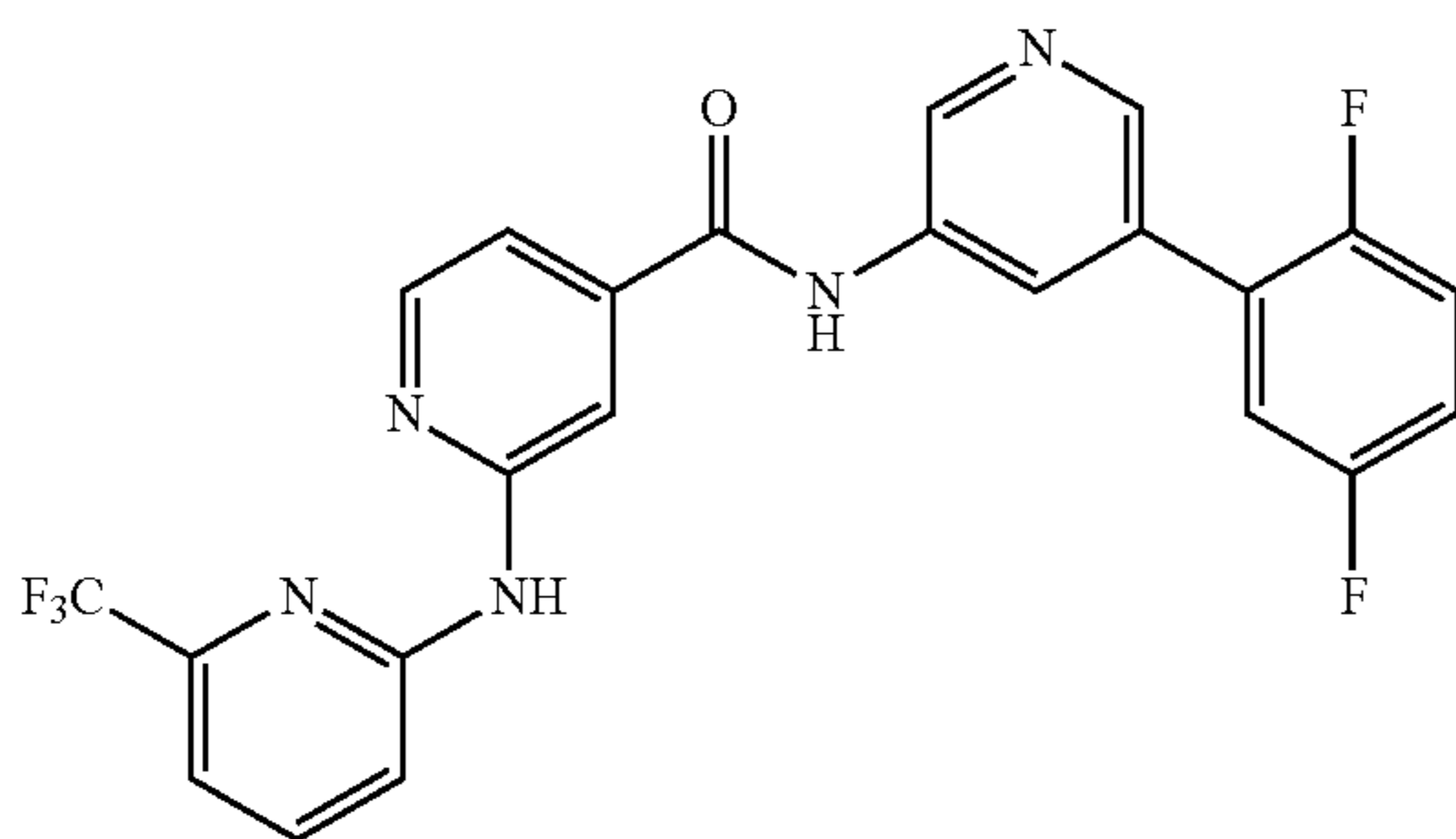
N-(5-(2,5-Difluorophenyl)pyridin-3-yl)-2-((6-(trifluoromethyl)pyridin-2-yl)amino)isonicotinamide
