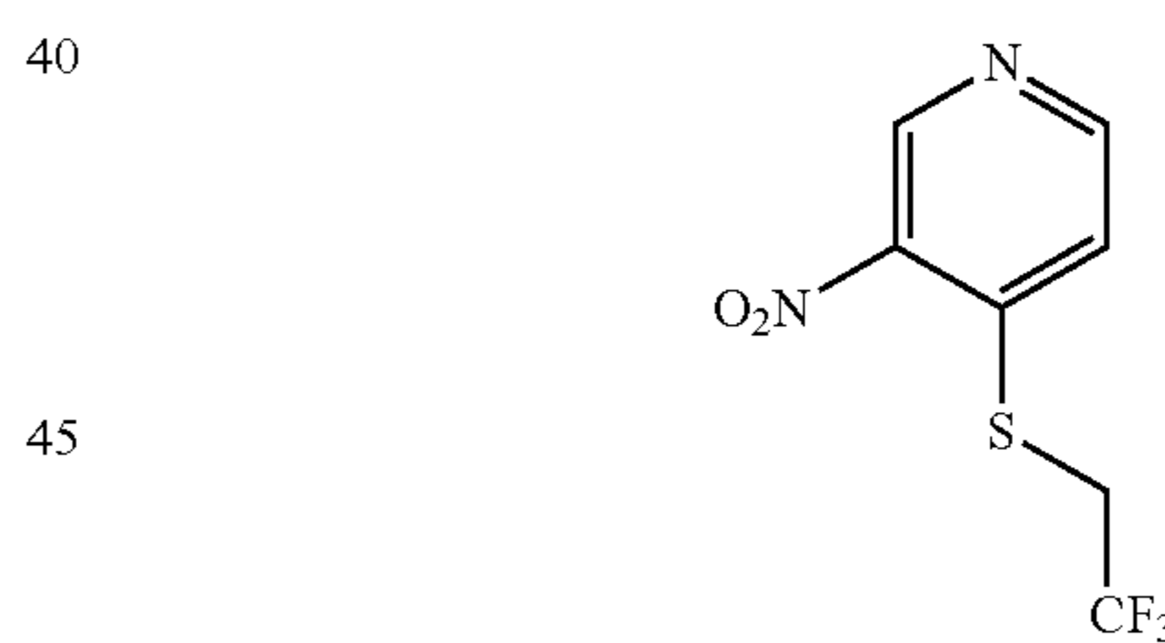
3-Nitro-4-((2,2,2-trifluoroethyl)thio)pyridine
