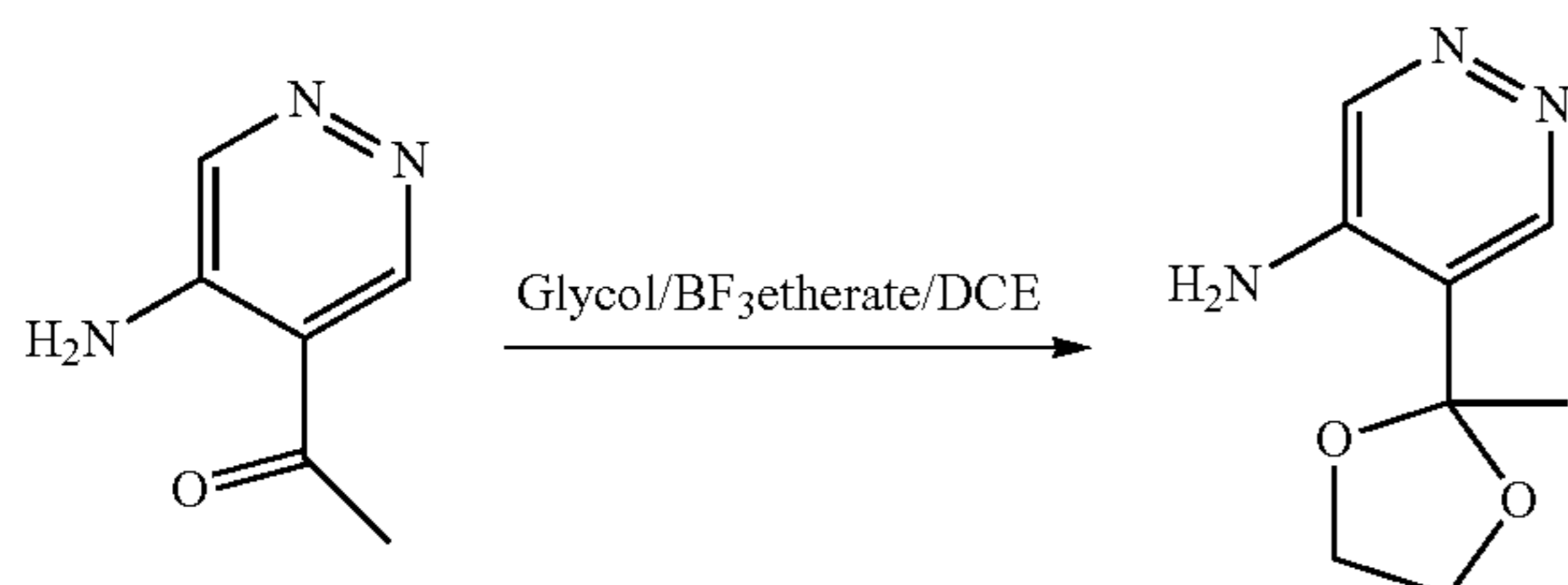
5-(2-Methyl-1,3-dioxolan-2-yl)pyridazin-4-amine
