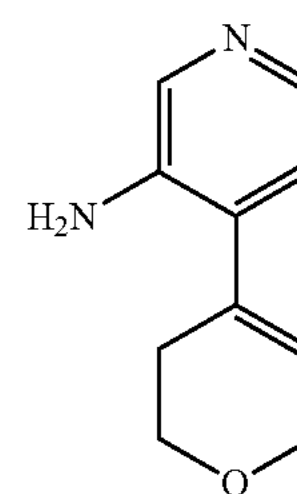
4-(3,6-Dihydro-2H-pyran-4-yl)pyridin-3-amine
