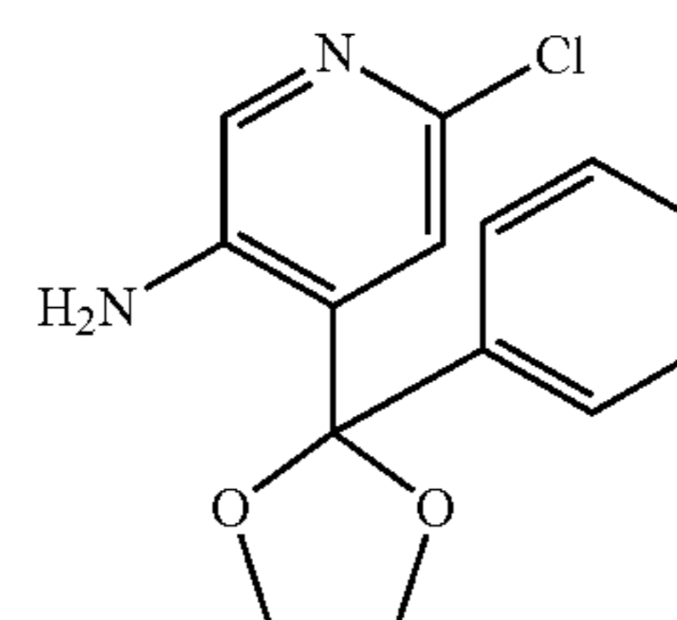
6-Chloro-4-(2-phenyl-1,3-dioxolan-2-yl)pyridin-3-amine
