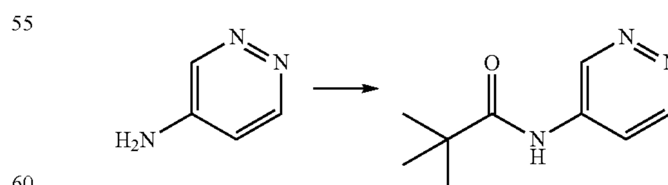
N-(Pyridazin-4-yl)pivalamide
