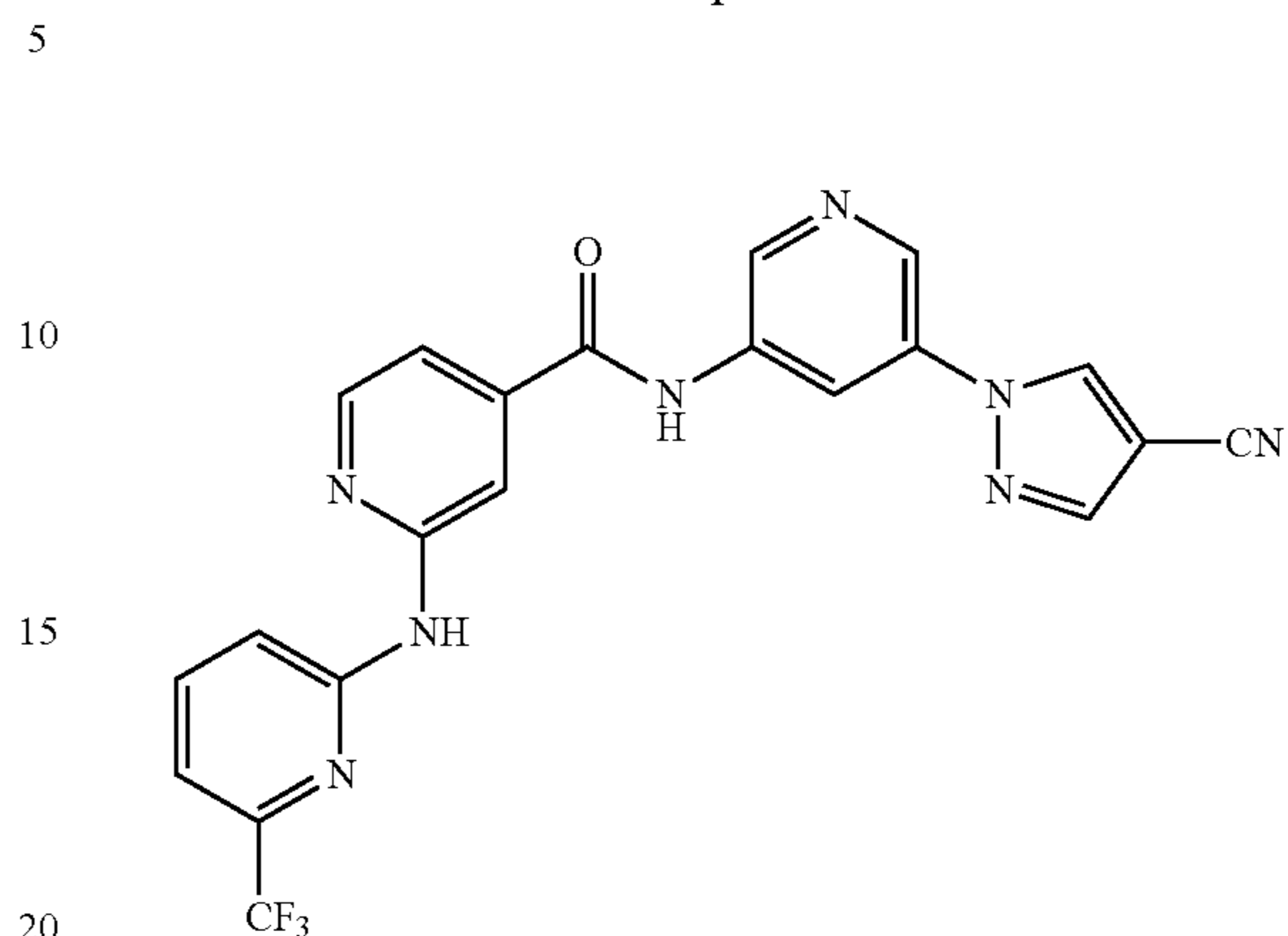
N-(5-(4-Cyano-1H-pyrazol-1-yl)pyridin-3-yl)-2-((6-(trifluoromethyl)pyridin-2-yl)amino)isonicotinamide
