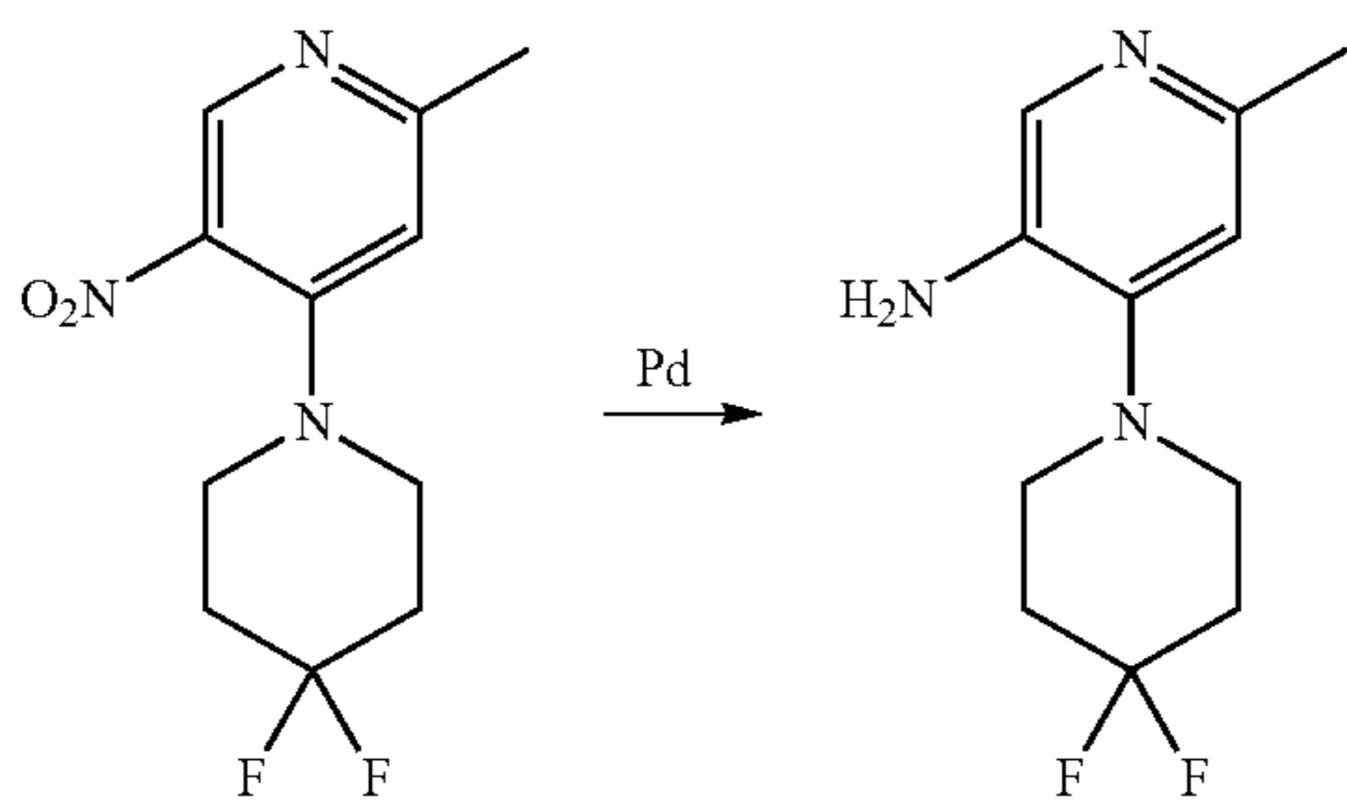
4-(4,4-Difluoropiperidin-1-yl)-6-methylpyridin-3-amine
