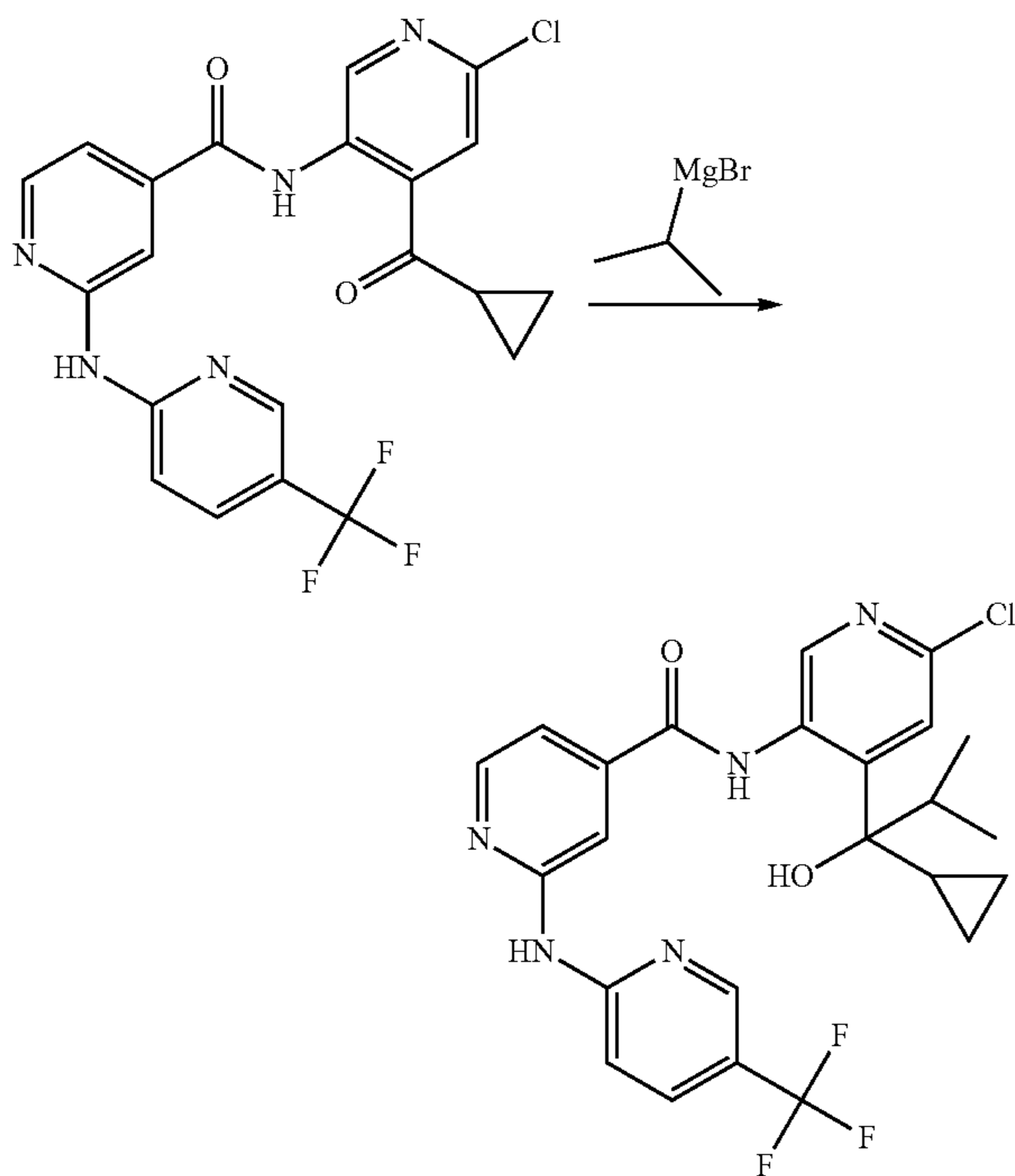
N-(6-Chloro-4-(1-cyclopropyl-1-hydroxy-2-methylpropyl)pyridin-3-yl)-2-((5-(trifluoromethyl)pyridin-2-yl)amino)isonicotinamide
