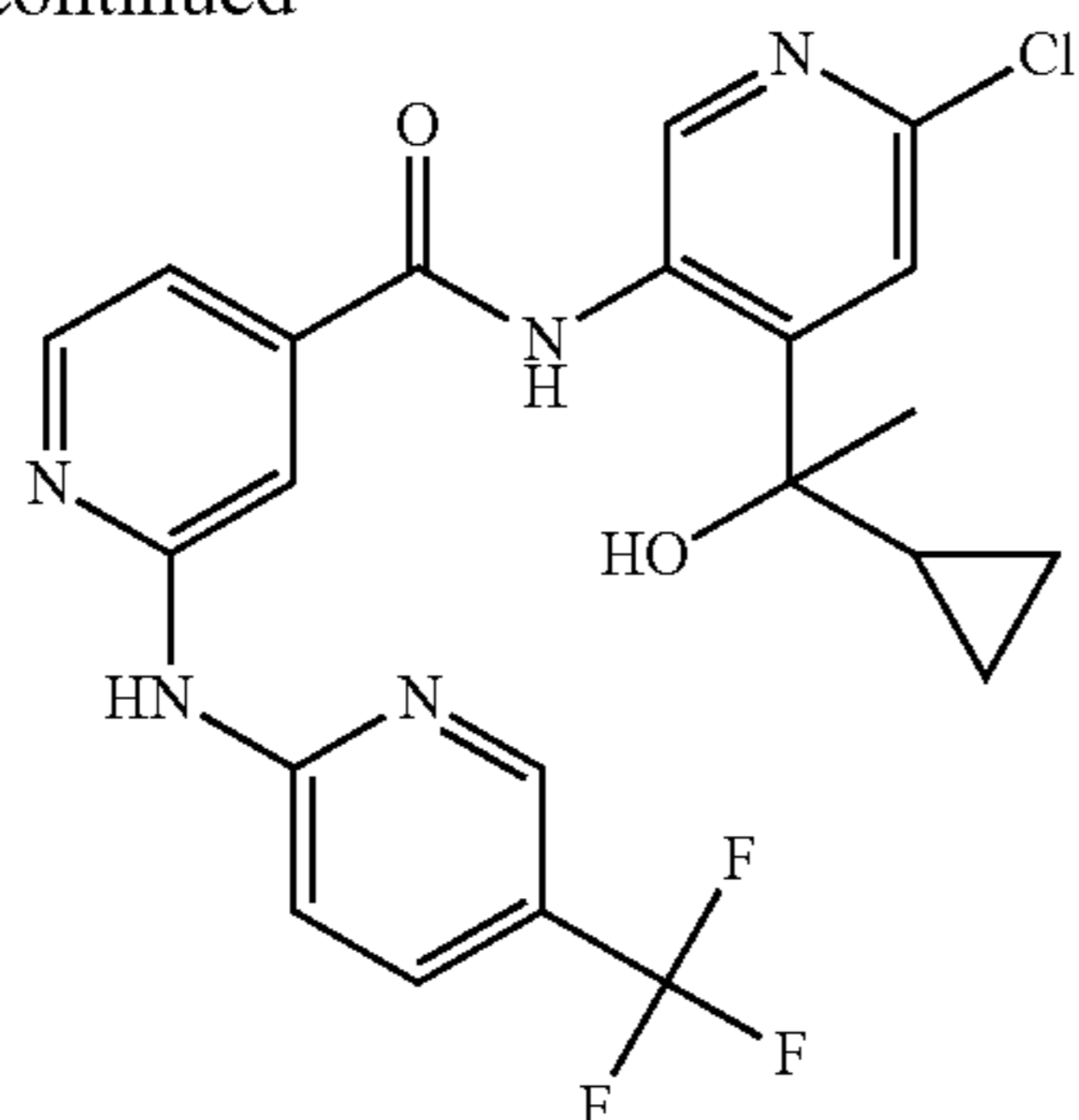
N-(6-Chloro-4-(1-cyclopropyl-1-hydroxyethyl)pyridin-3-yl)-2-((5-(trifluoromethyl)pyridin-2-yl)amino)isonicotinamide
