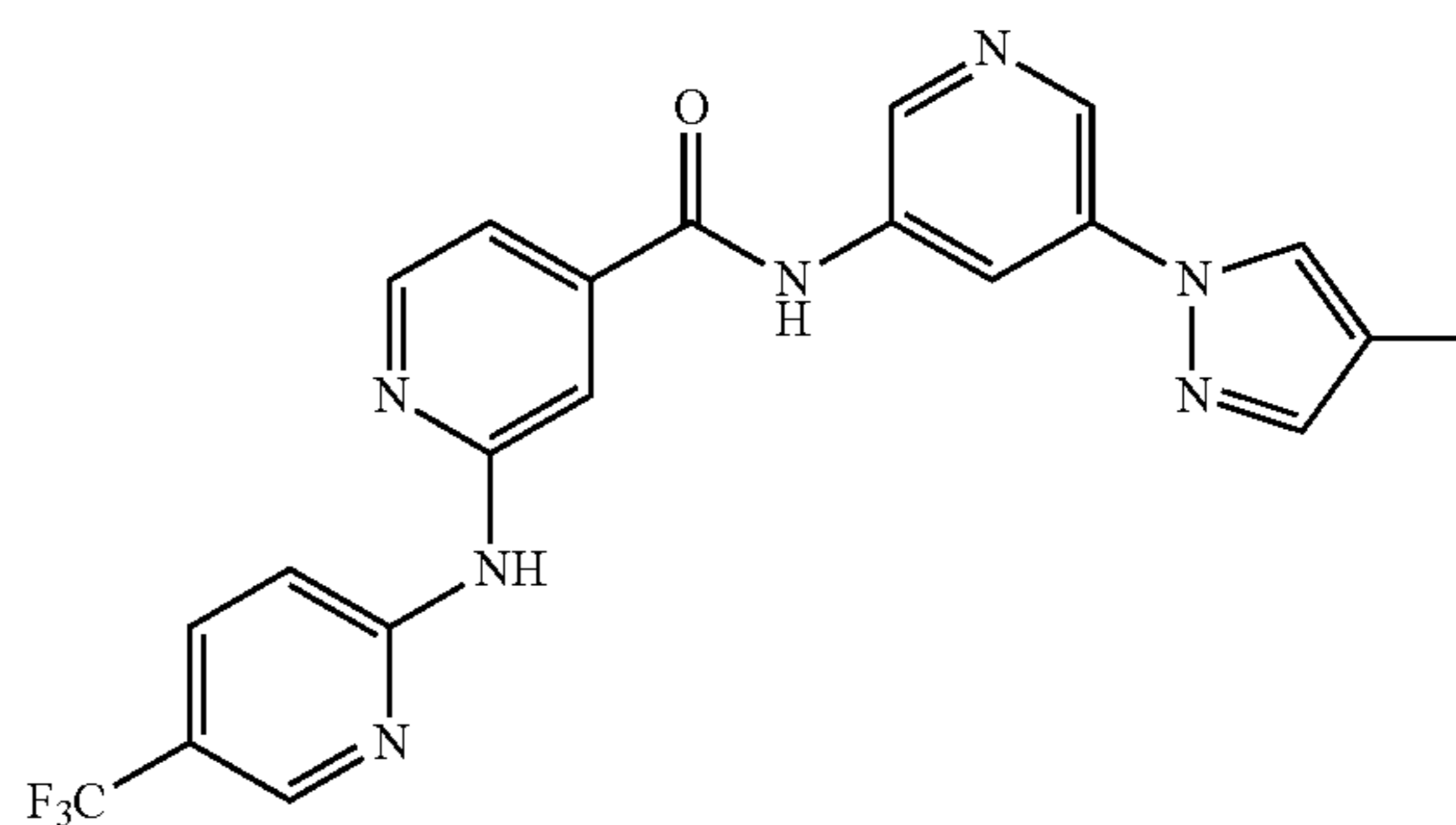
N-(5-(4-Methyl-1H-pyrazol-1-yl)pyridin-3-yl)-2-((5-(trifluoromethyl)pyridin-2-yl)amino)isonicotinamide
