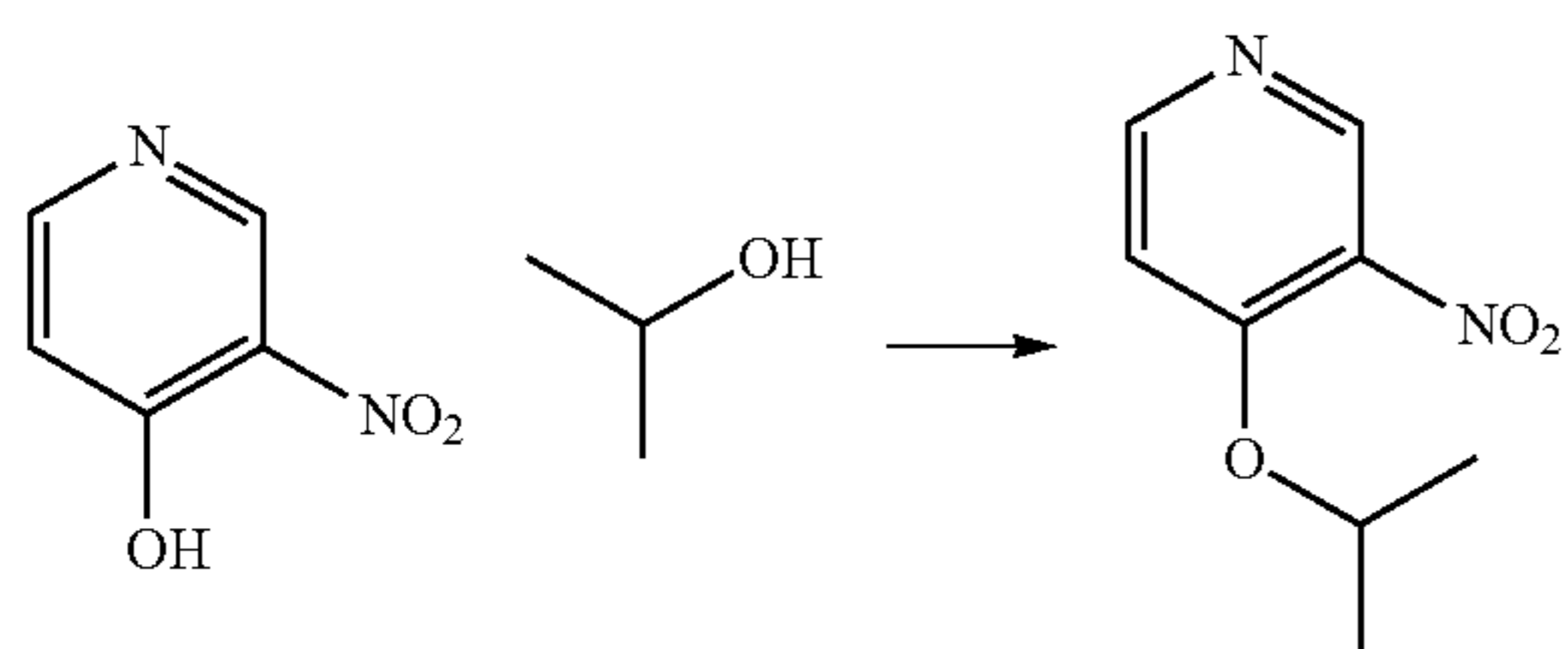
4-Isopropoxy-3-nitropyridine
