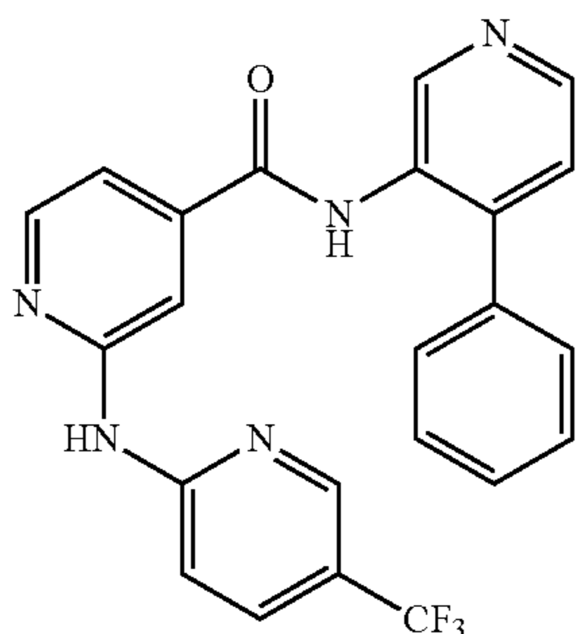
N-(4-Phenylpyridin-3-yl)-2-((5-(trifluoromethyl)pyridin-2-yl)amino)isonicotinamide
