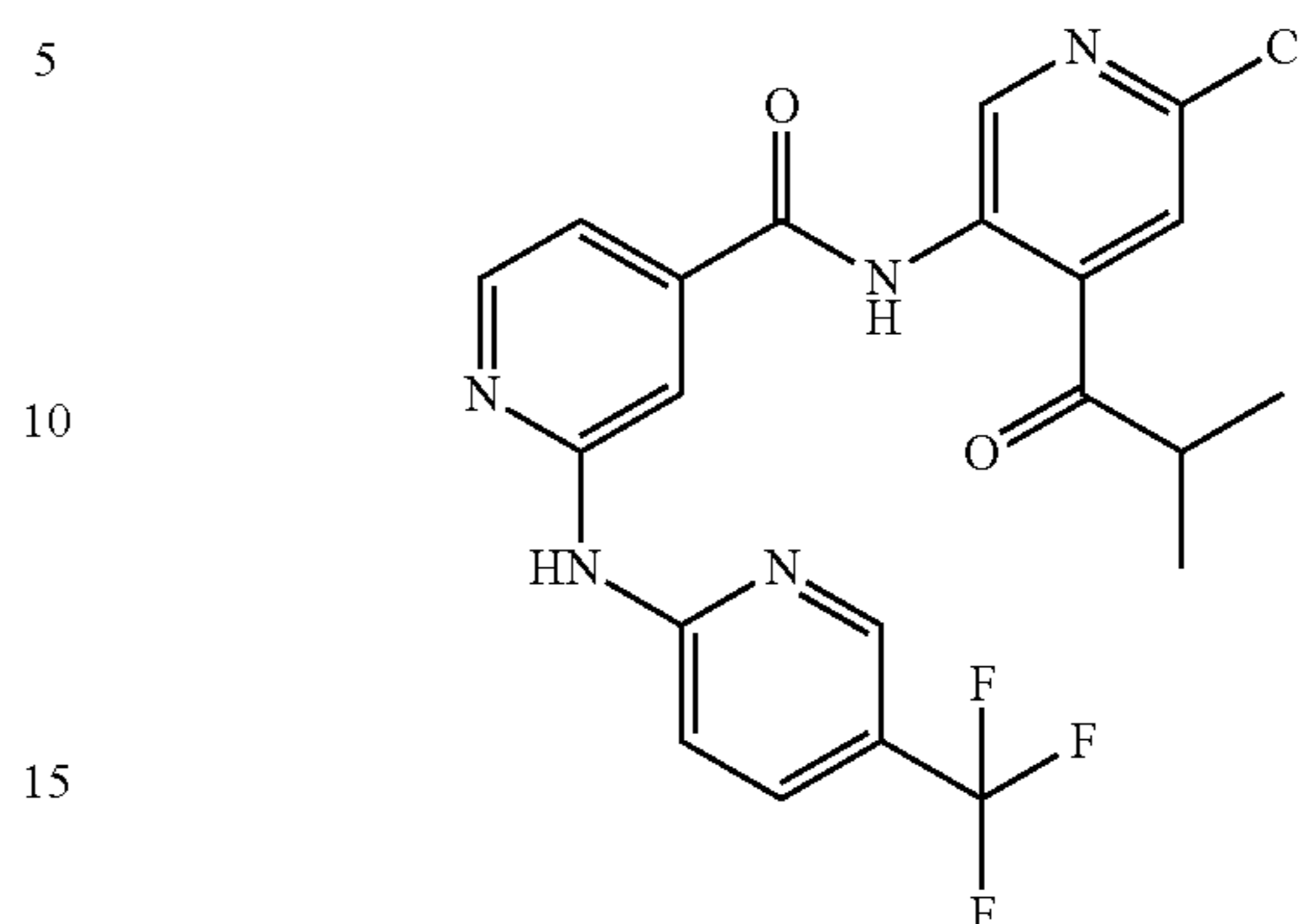
N-(6-Chloro-4-isobutyrylpyridin-3-yl)-2-((5-(trifluoromethyl)pyridin-2-yl)amino)isonicotinamide
