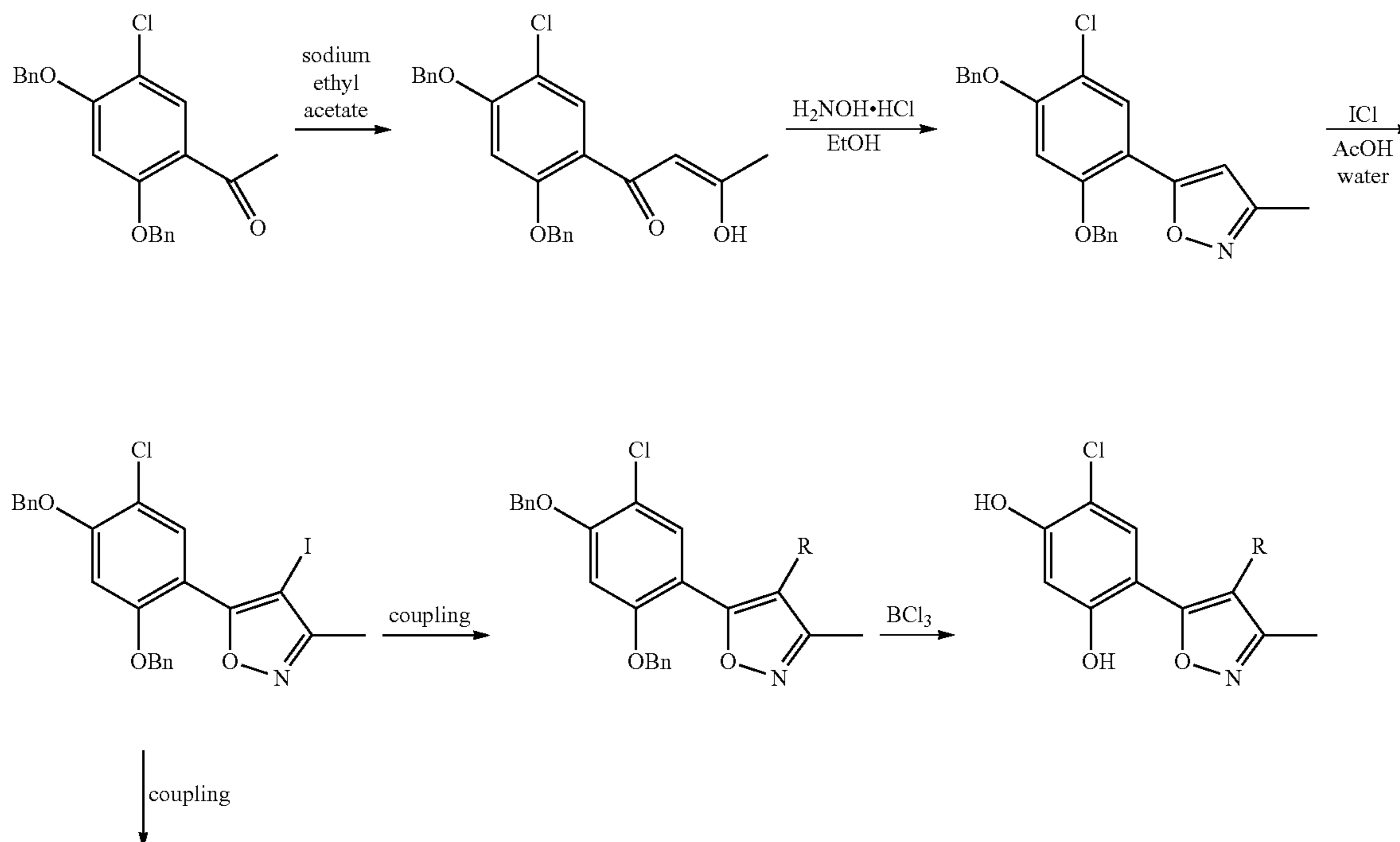
Scheme 7: Preparation of 5-(2,4-bis-benzyloxy-5-chloro-phenyl)-4-iodo-3-methyl-isoxazole intermediate
