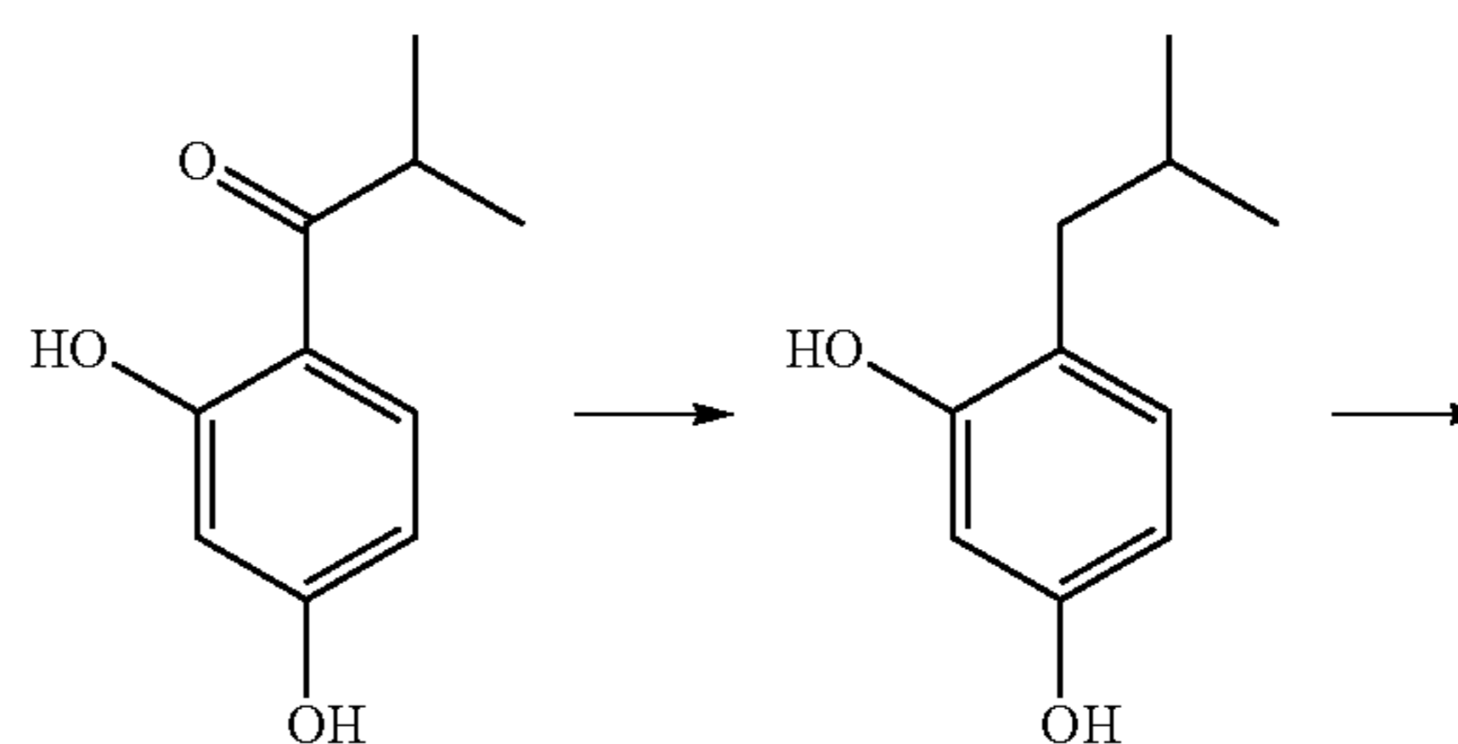
Reaction Scheme
