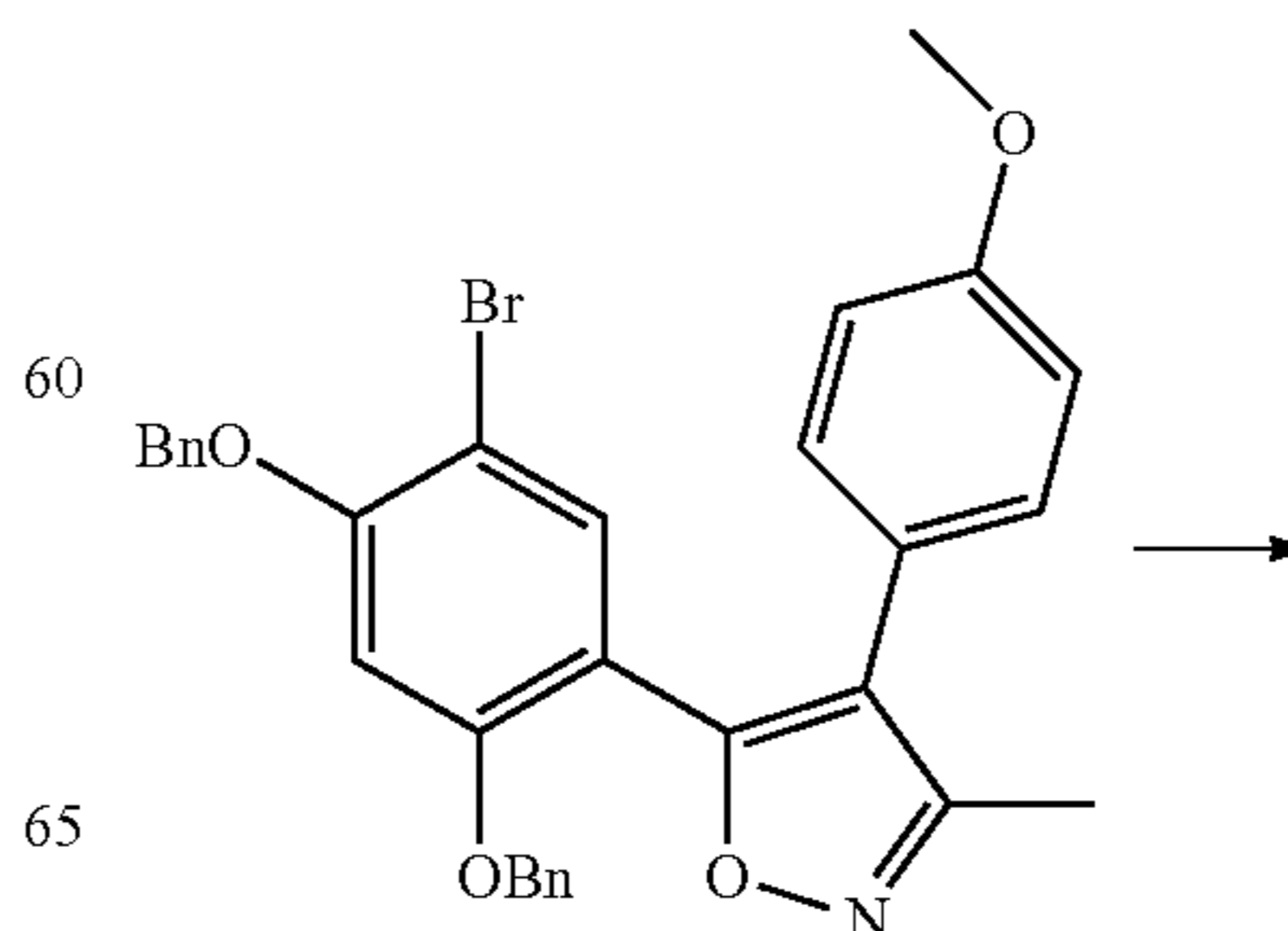
Scheme 5: Heck reaction and boron trichloride deprotection
