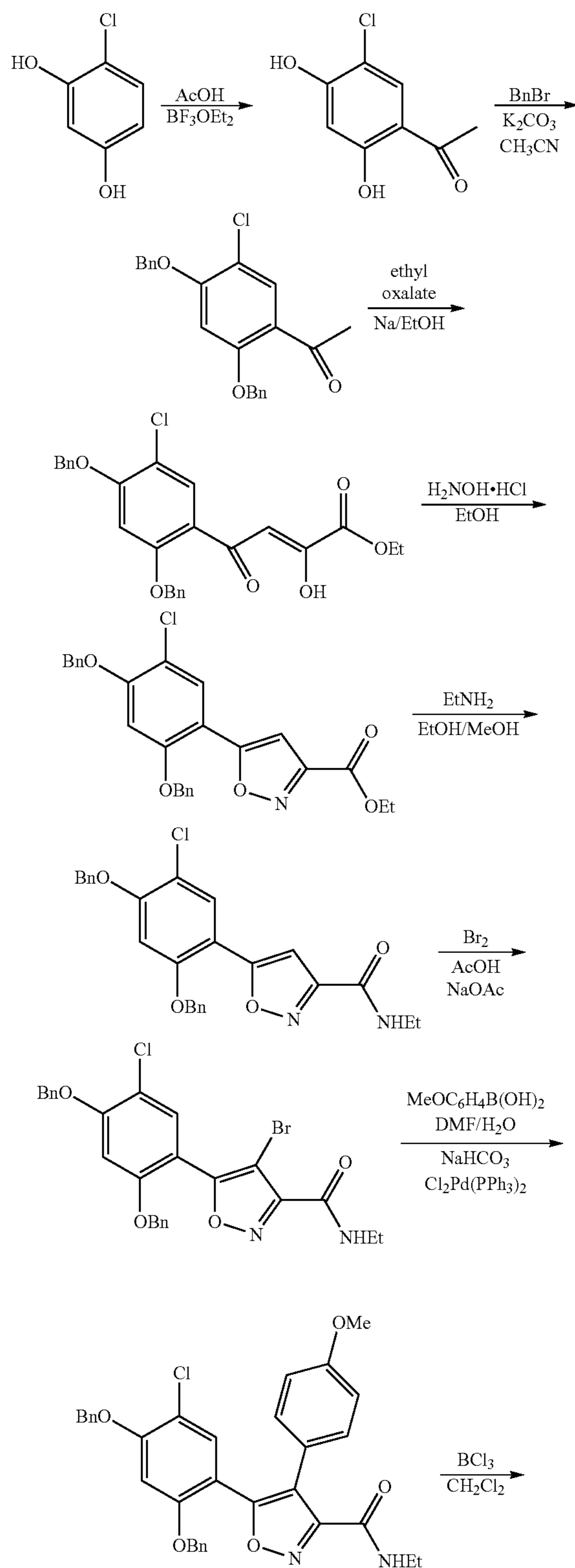
Scheme 6: Synthesis of 5-carboxamido isoxazoles
