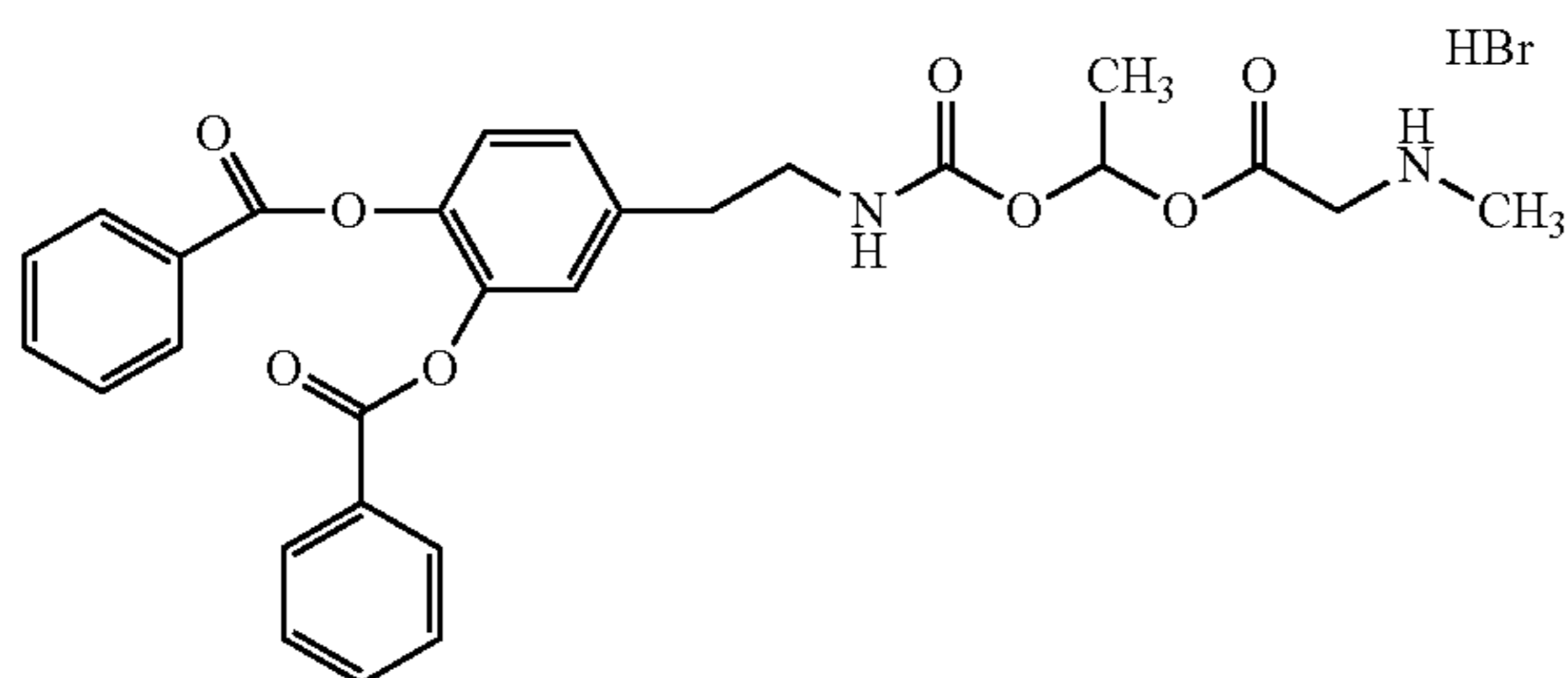
4-(6-methyl-4,8-dioxo-5,7-dioxa-2,9-diazadecan-11-yl)-1,2-phenylene dibenzoate hydrobromide
