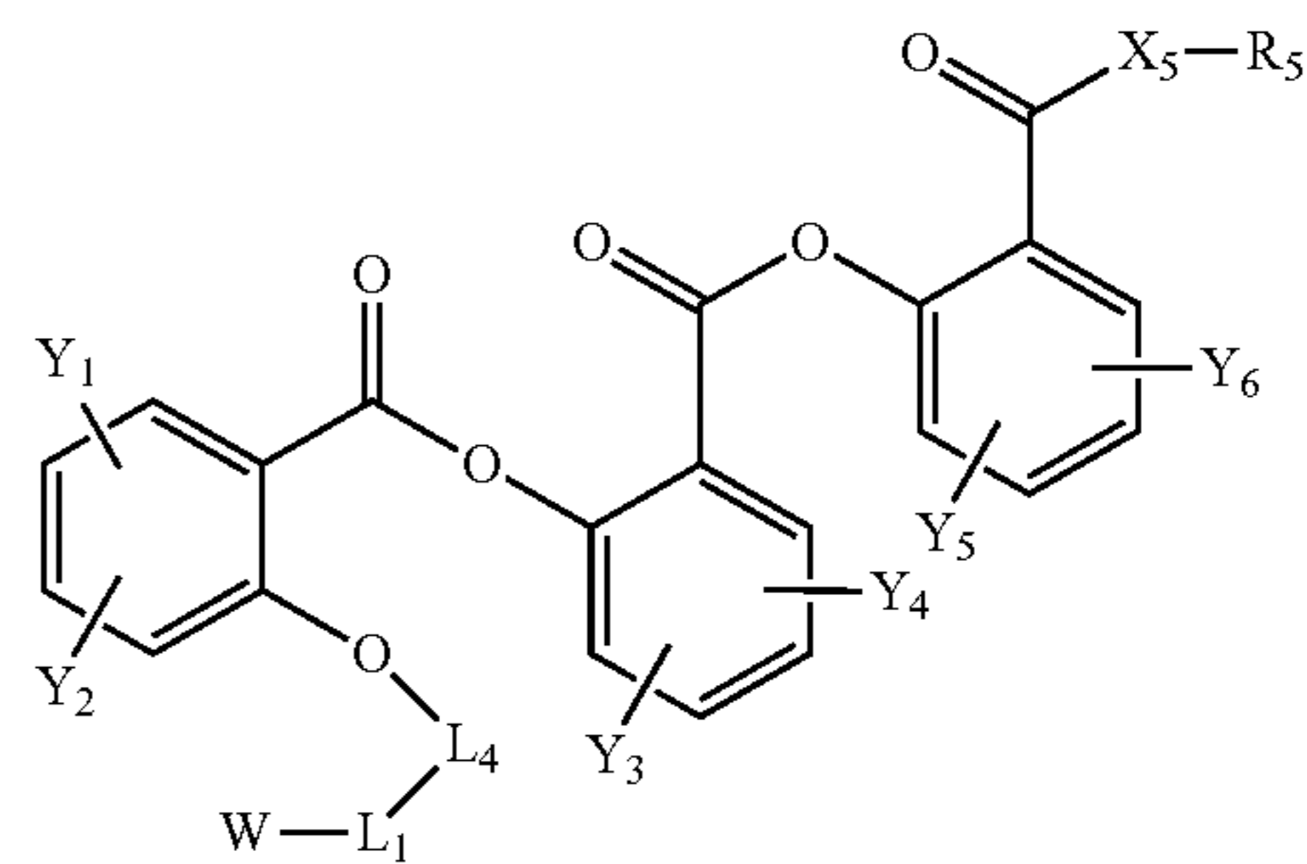
Structure NSAID-11
