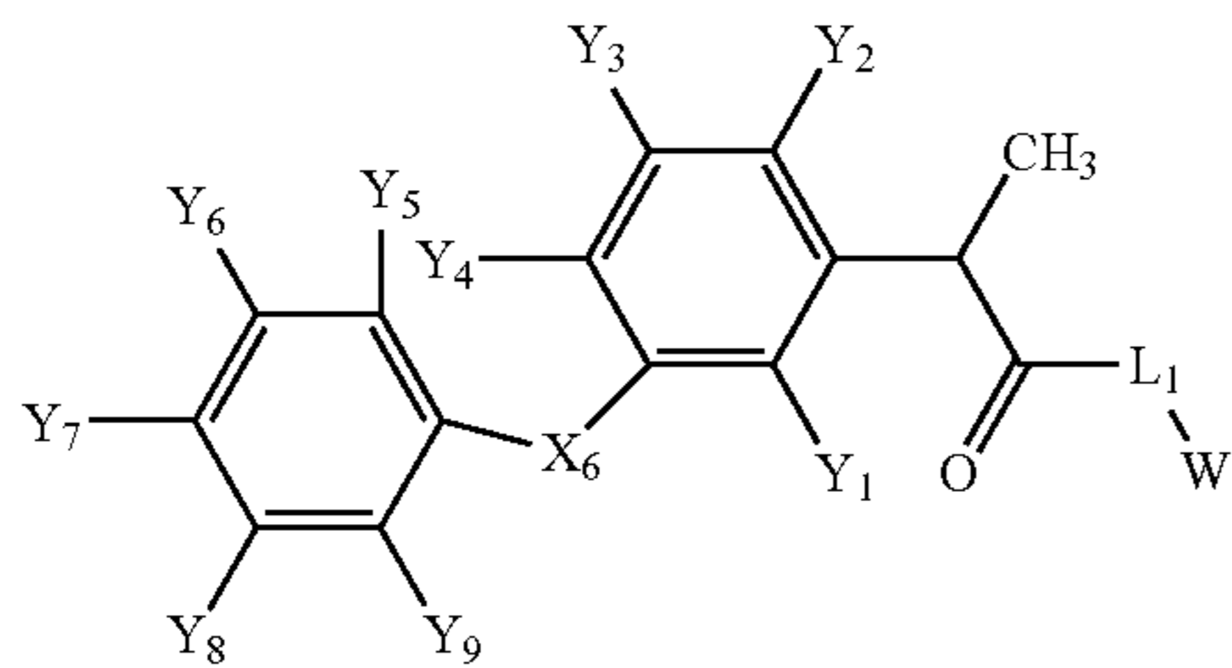
Structure NSAID-6
