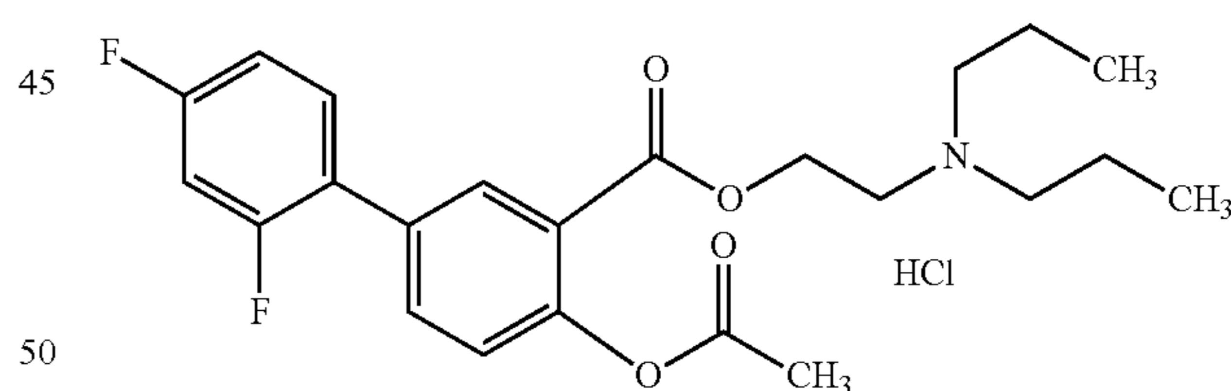
2-(dipropylamino)ethyl 4-acetoxy-2',4'-difluoro-[1,1'-biphenyl]-3-carboxylate hydrochloride
