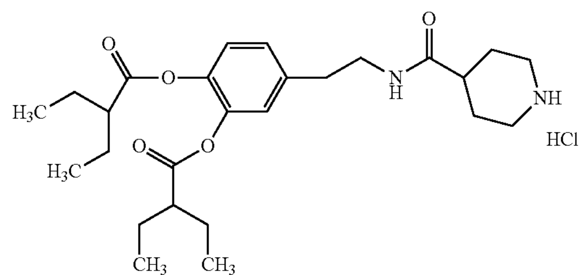
4-(2-(piperidine-4-carboxamido)ethyl)-1,2-phenylene bis(2-ethylbutanoate) hydrochloride
