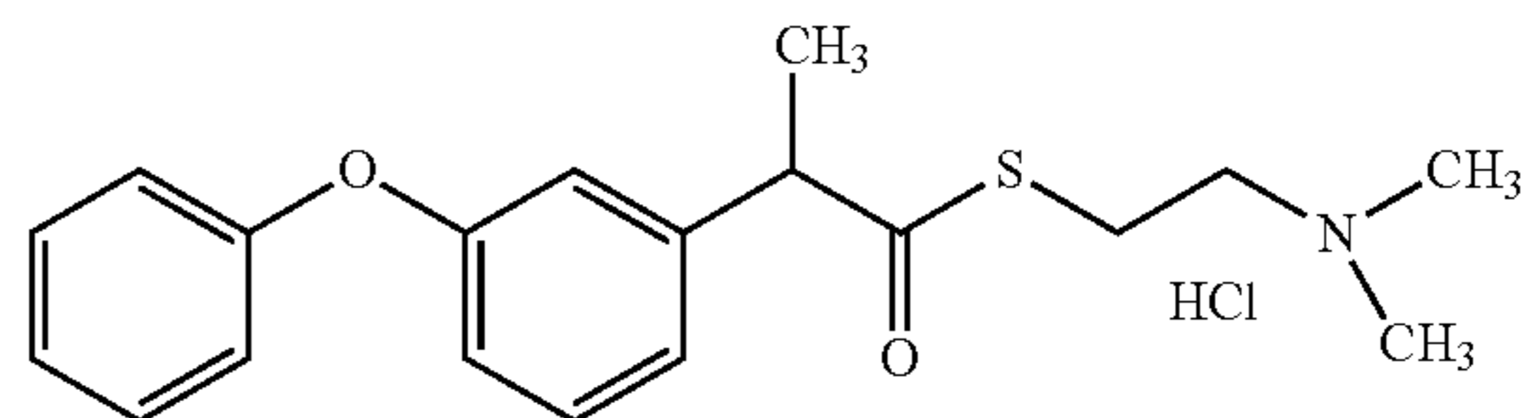
S-(2-(dimethylamino)ethyl 2-(3-phenoxyphenyl)propanethioate hydrochloride
