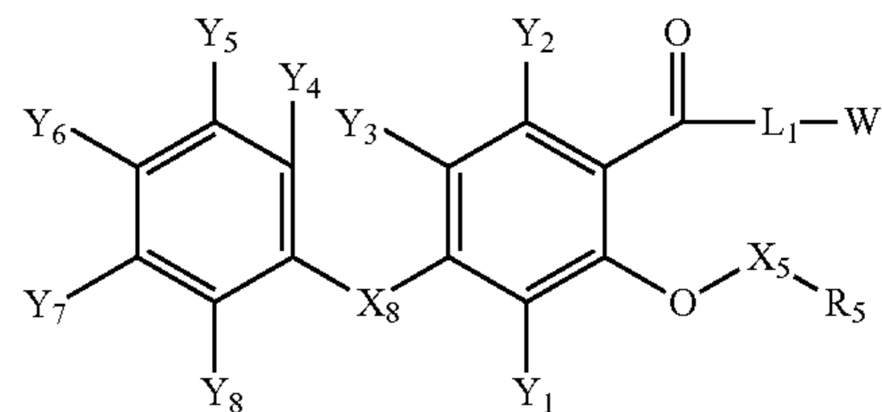
Structure NSAID-12
