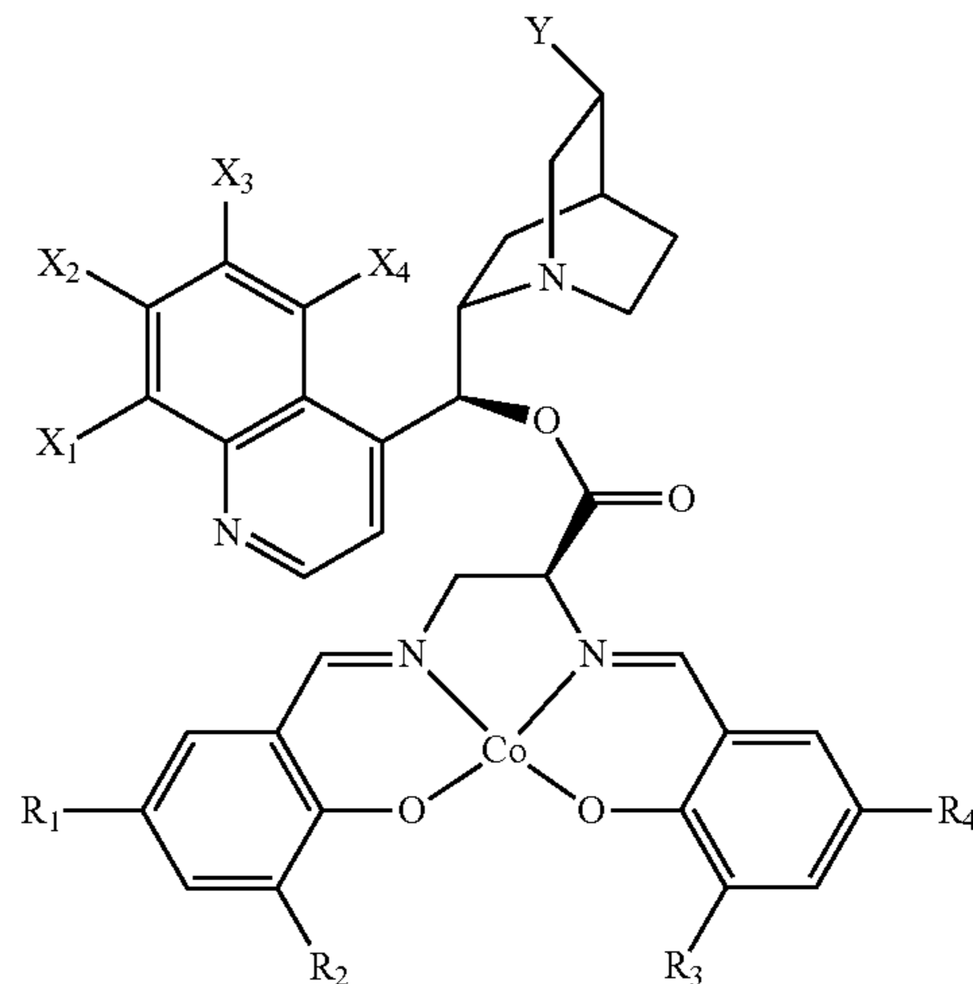
Formula II(E)
