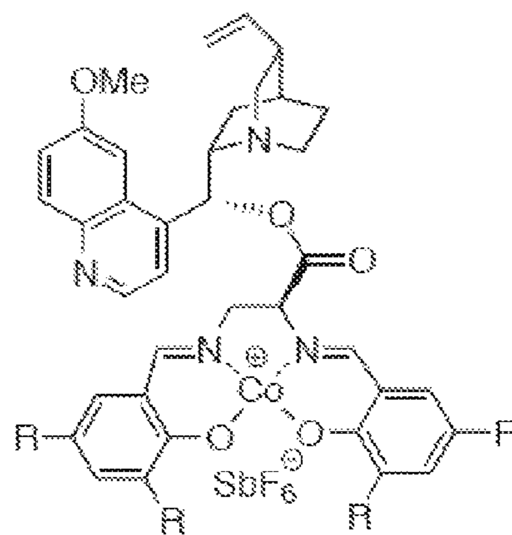
(S)-Co(III)-LB* (10A)
