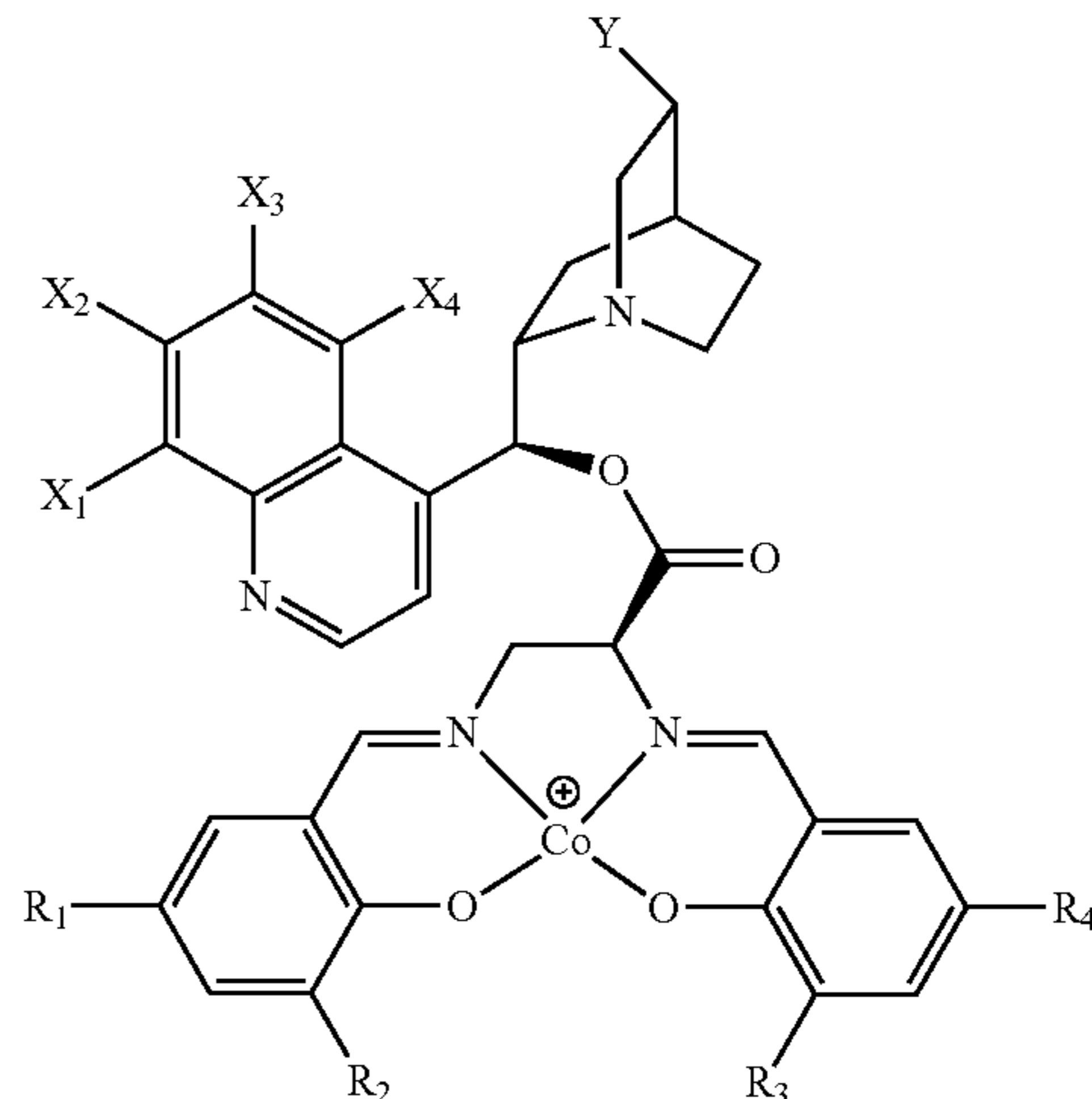
Formula I(E)
