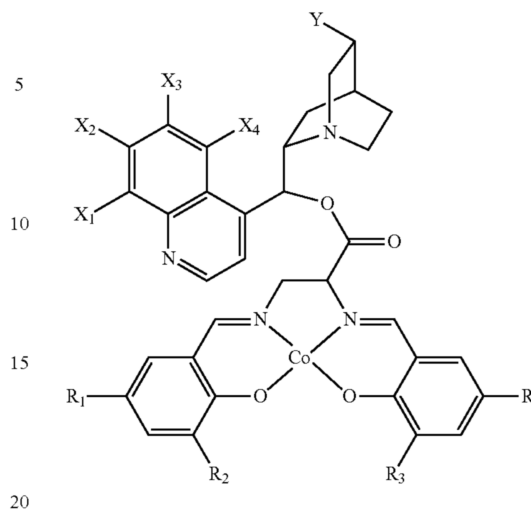
Formula II(H)
