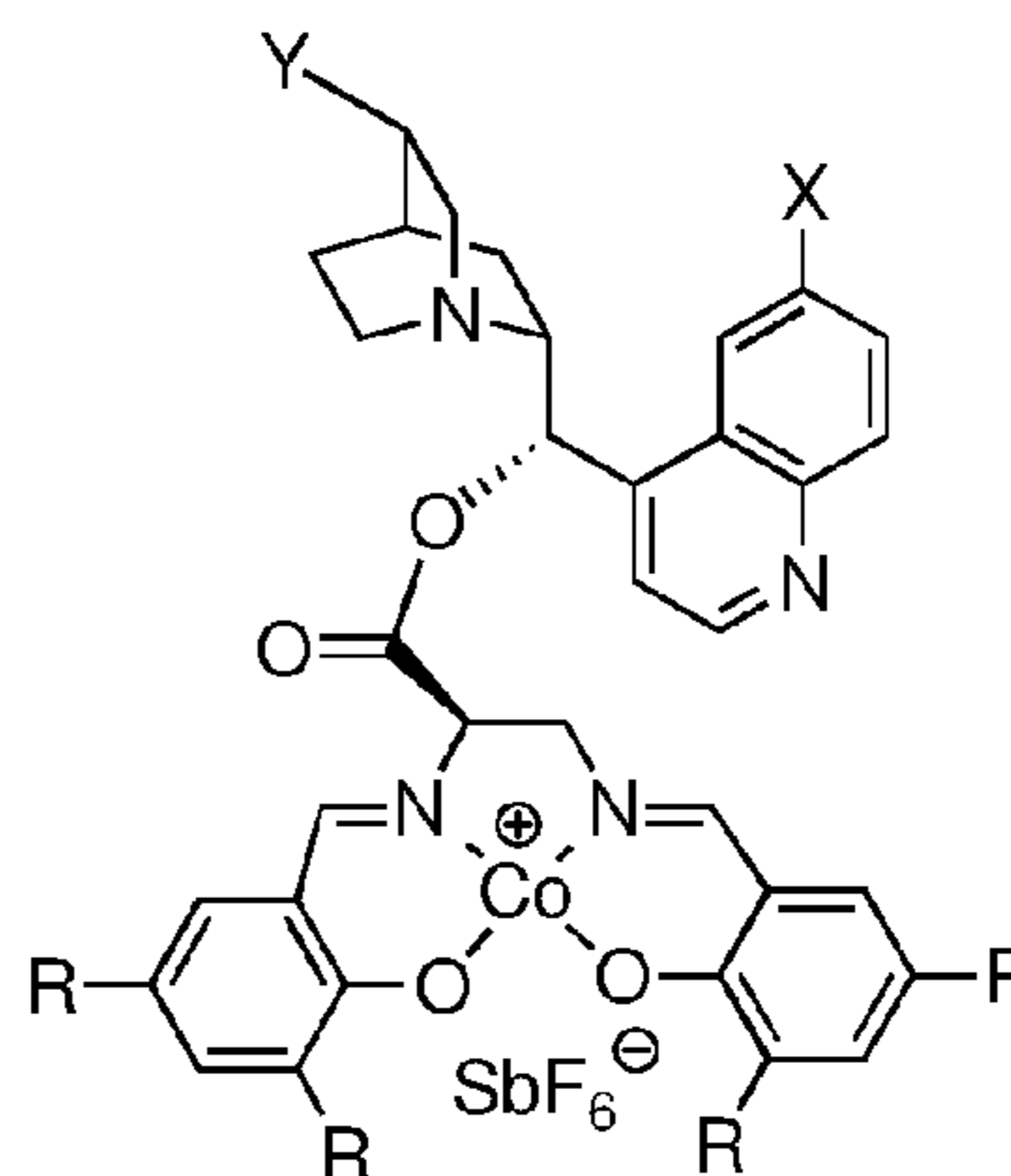
(R)-Co(III)-LB* 10A2
