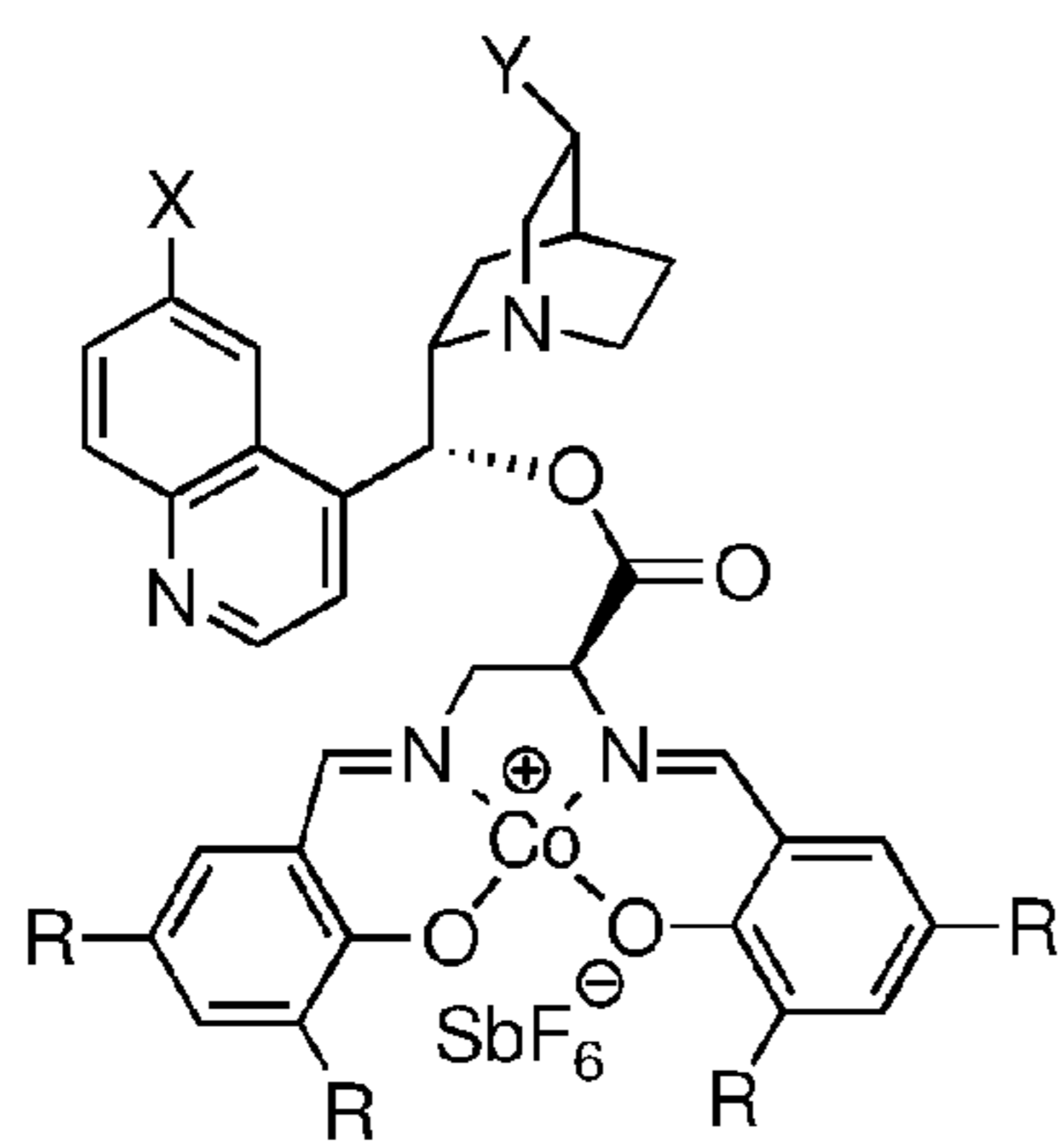
(S)-Co(III)-LB* 10A1
