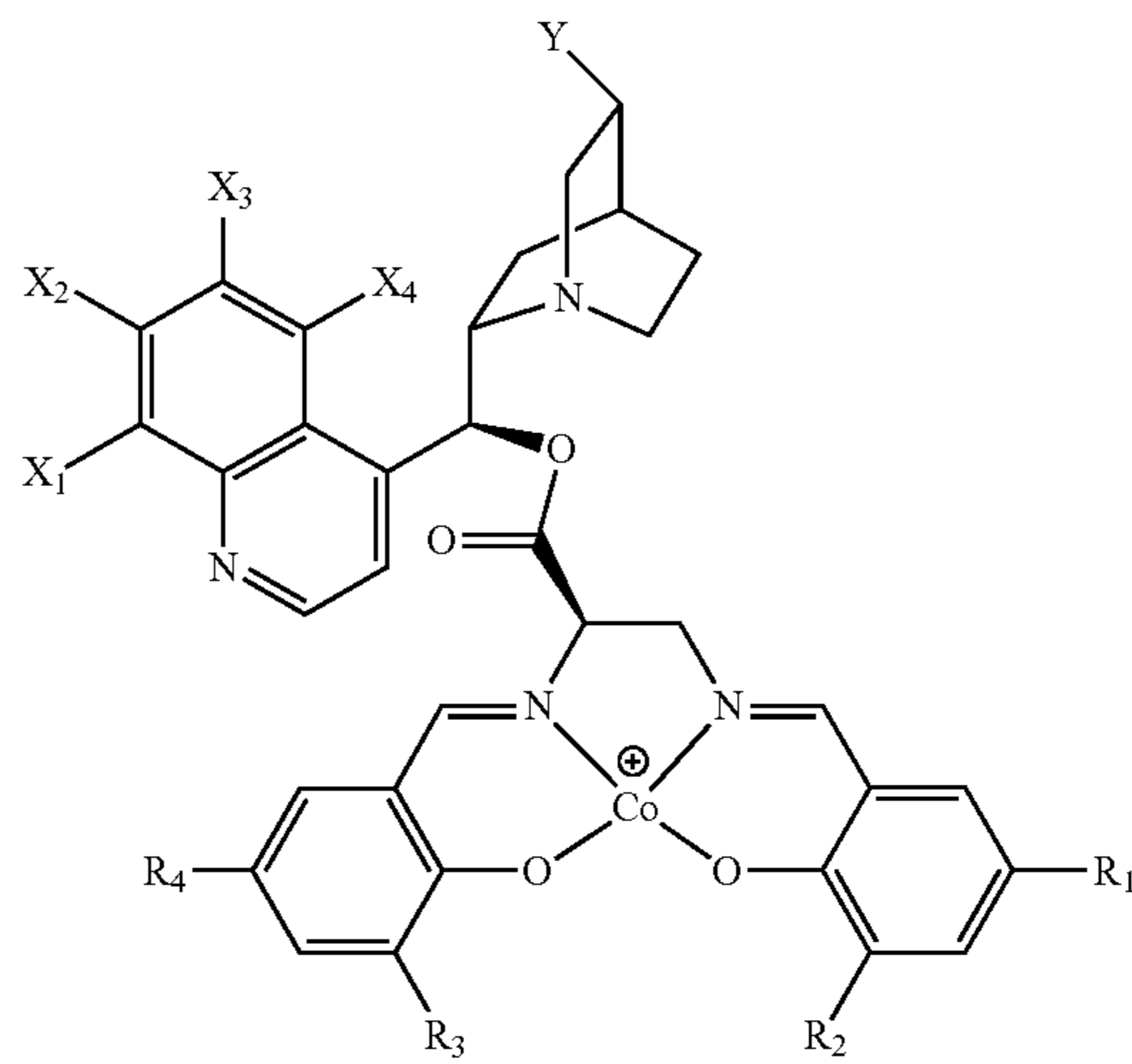
Formula I(G)
