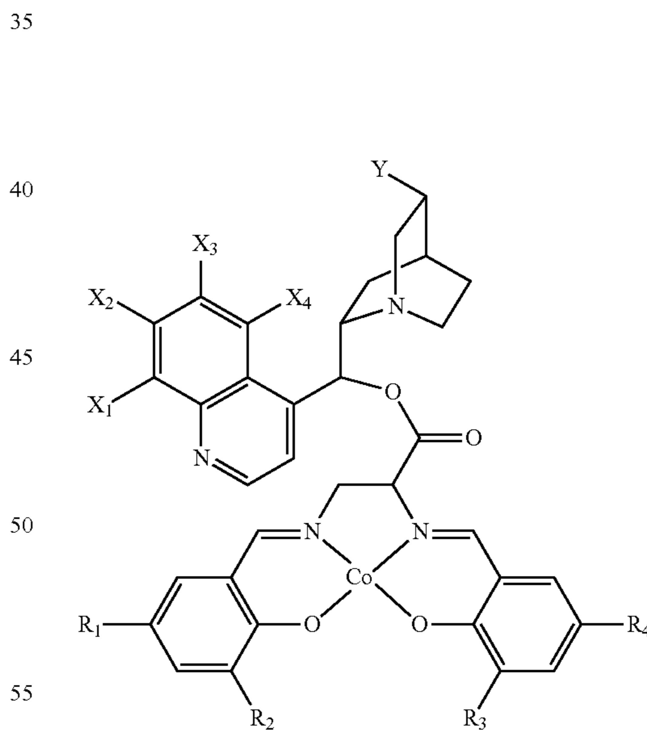
Formula II
