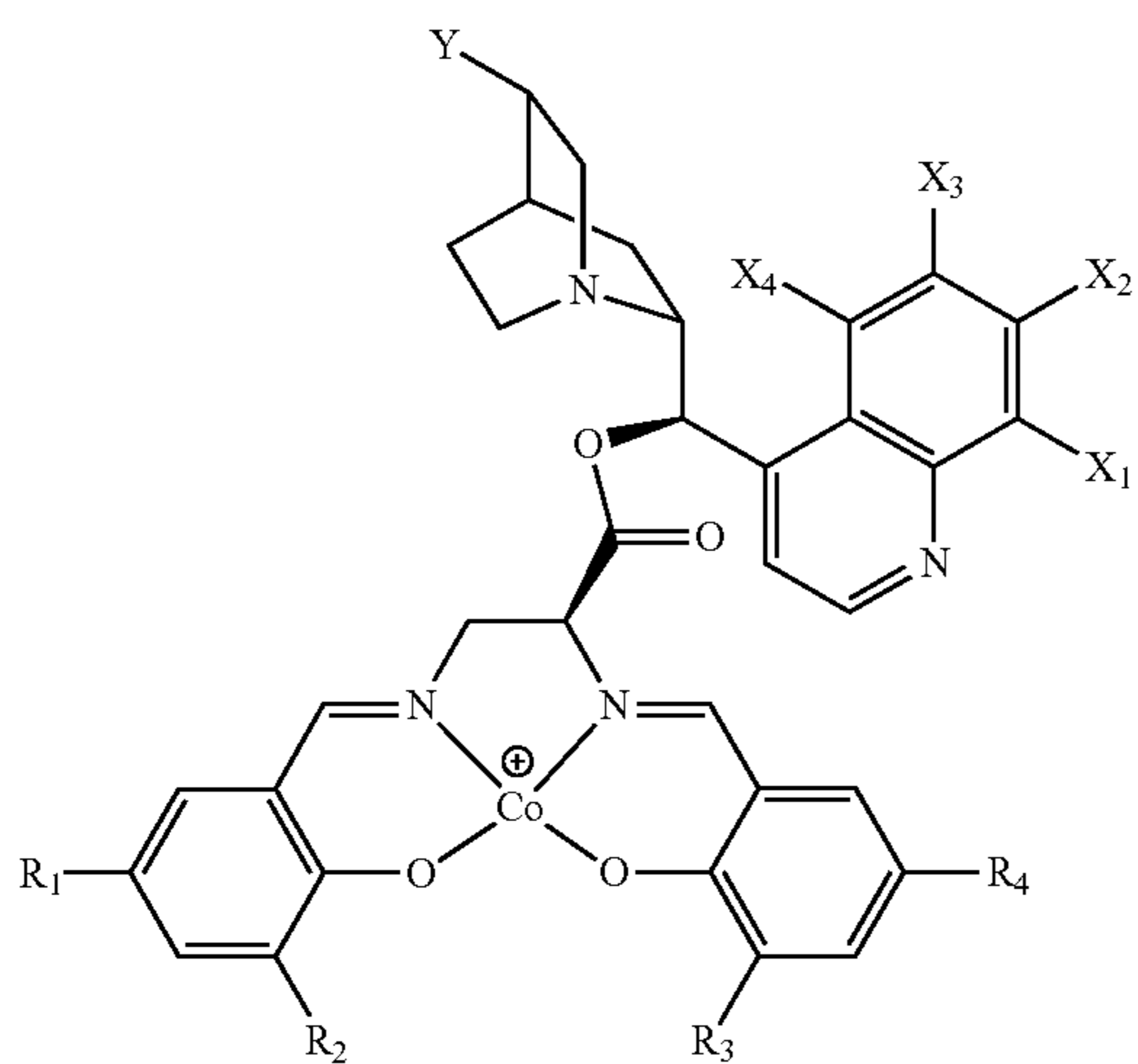
Formula I(H)
