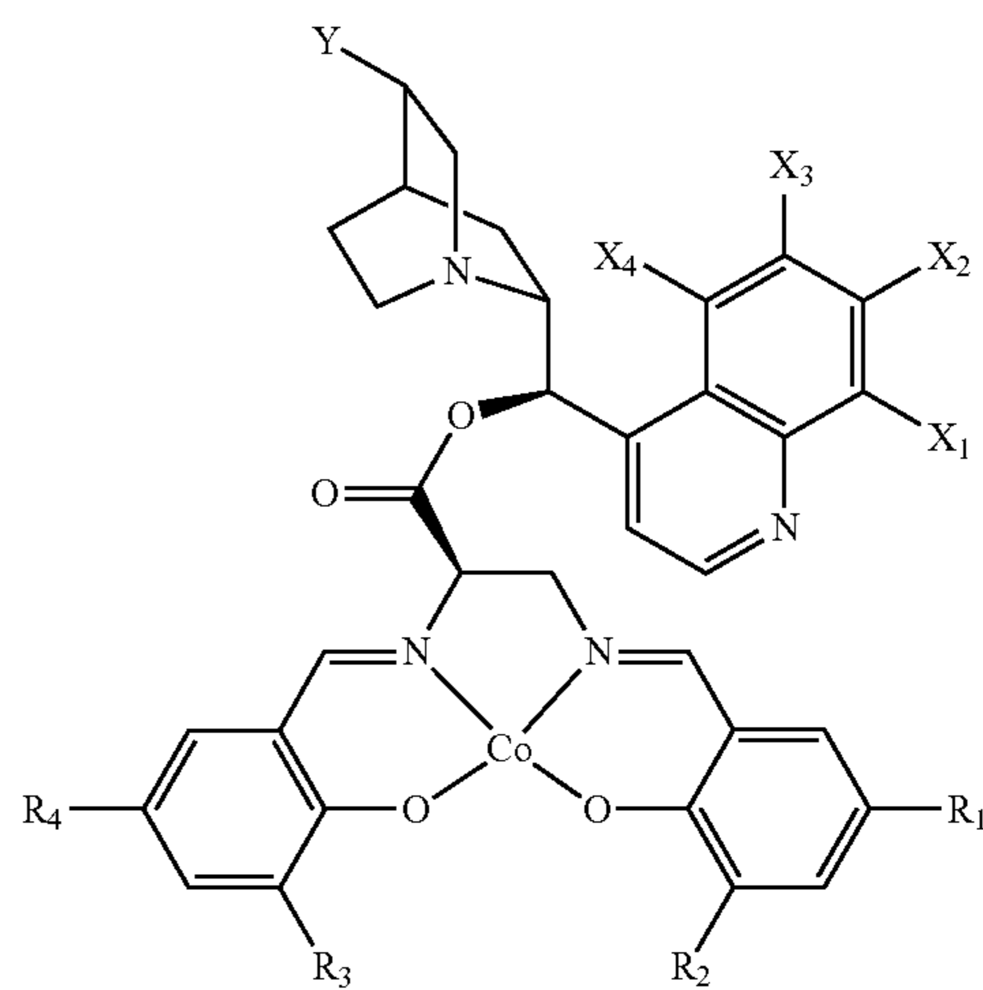
Formula II(F)
