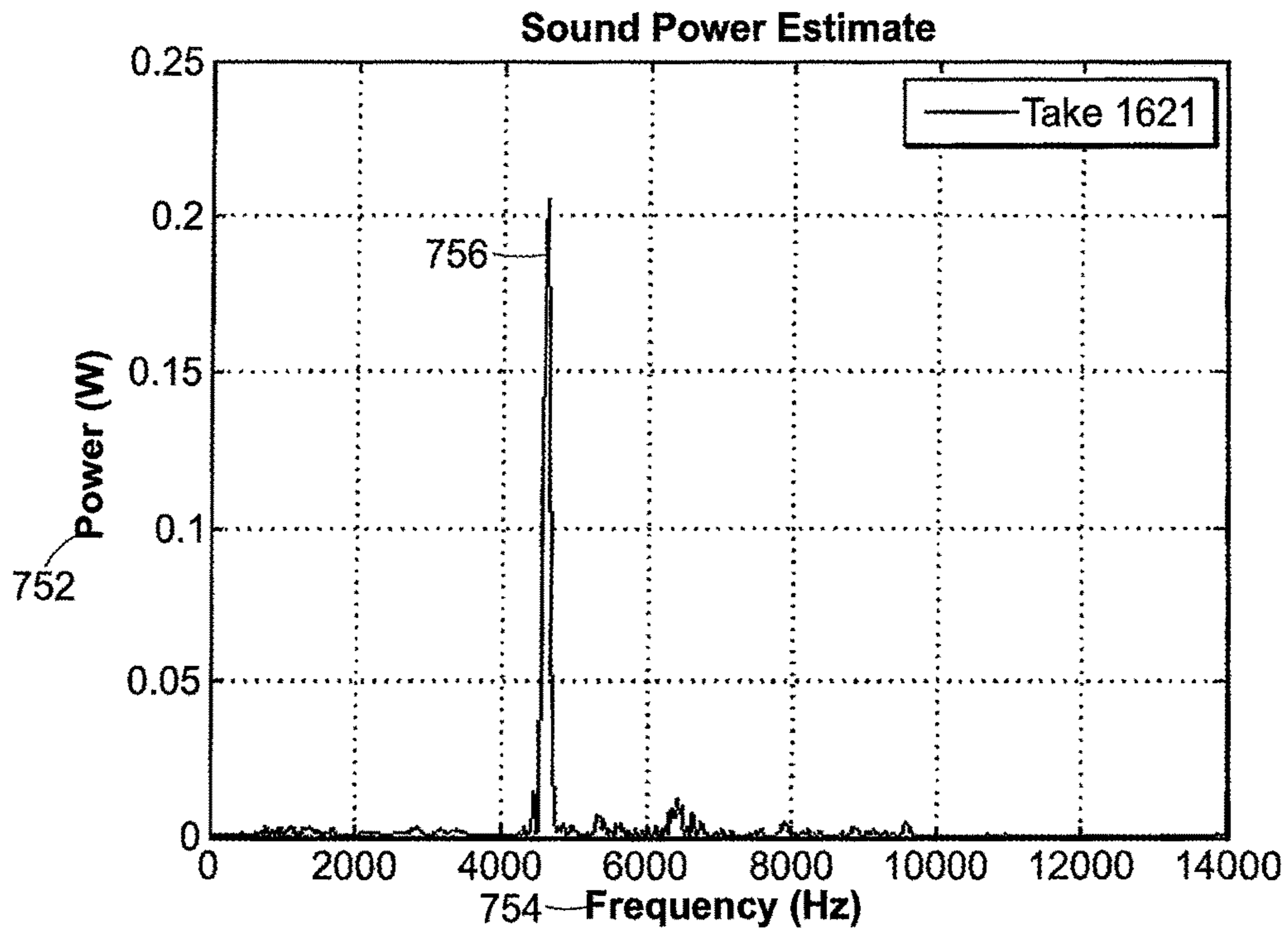
FIG. 7 (Prior Art)
