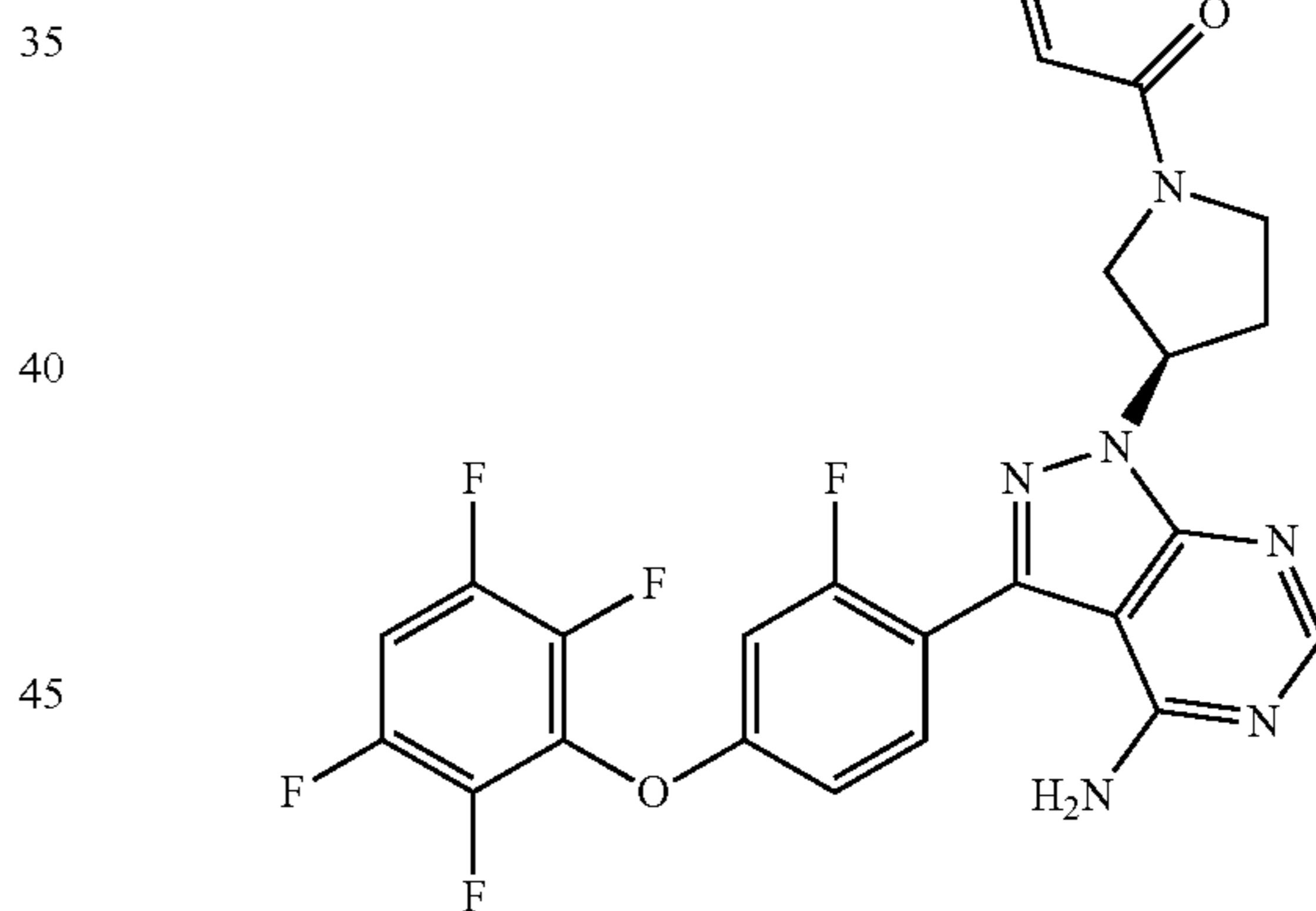
1-((R)-3-(4-amino-3-(2-fluoro-4-(2,3,5,6-tetrafluorophenoxy)phenyl)-1H-pyrazolo[3,4-d]pyrimidin-1-yl)piperidin-1-yl)prop-2-en-1-one
