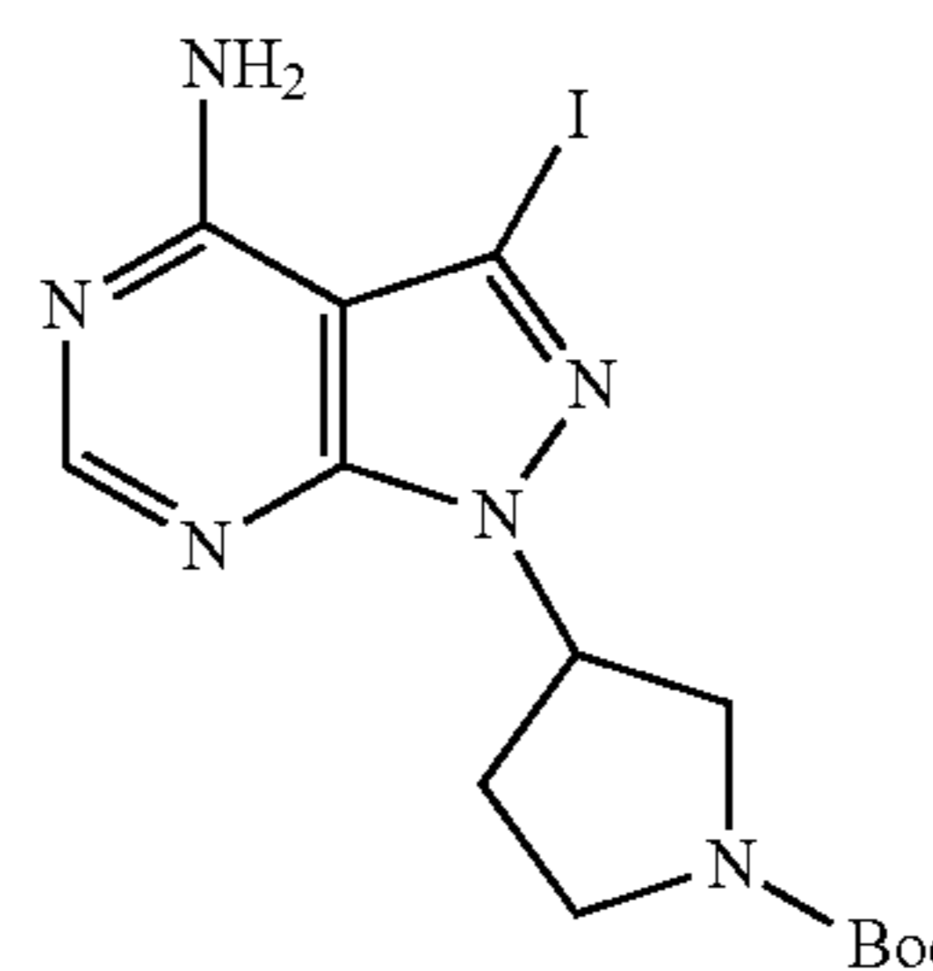
tert-butyl 3-(4-amino-3-iodo-1H-pyrazolo[3,4-d]pyrimidin-1-yl)pyrrolidine-1-carboxylate
