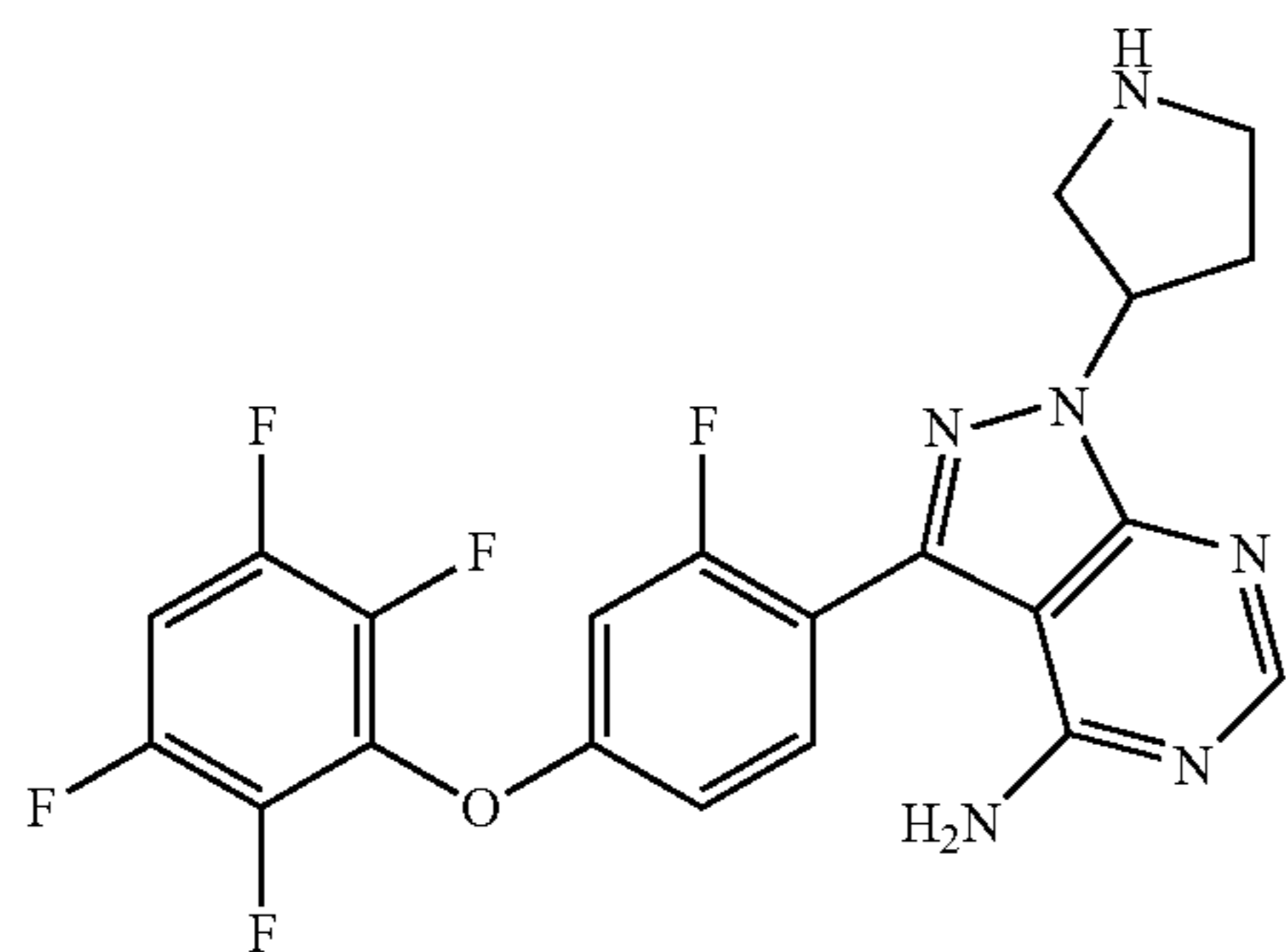
3-(2-fluoro-4-(2,3,5,6-tetrafluorophenoxy)phenyl)-1-(pyrrolidin-3-yl)-1H-pyrazolo[3,4-d]pyrimidin-4-amine
