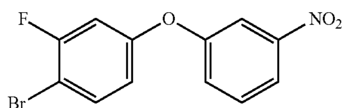
1-bromo-2-fluoro-4-(3-nitrophenoxy)benzene
