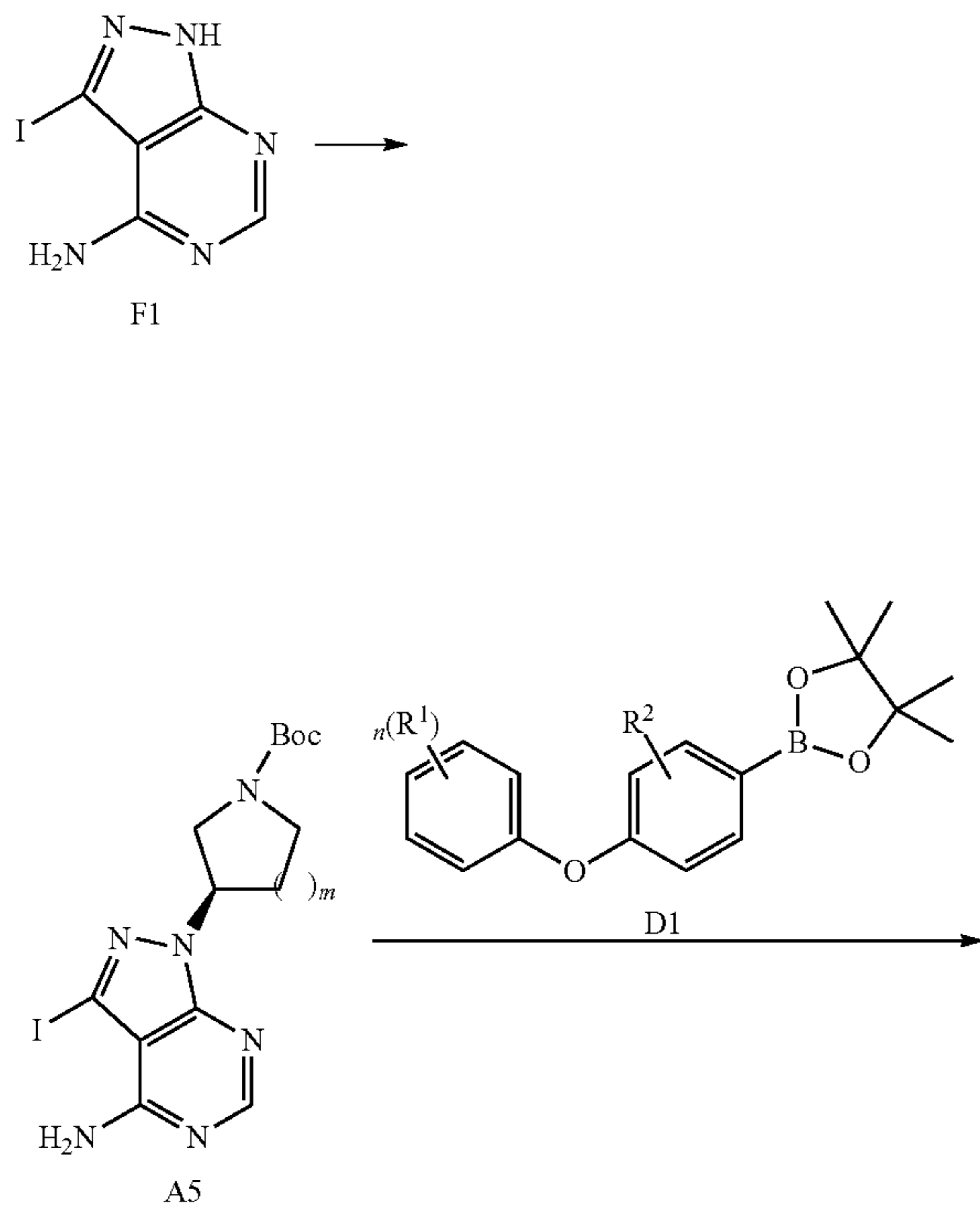
Scheme 5
