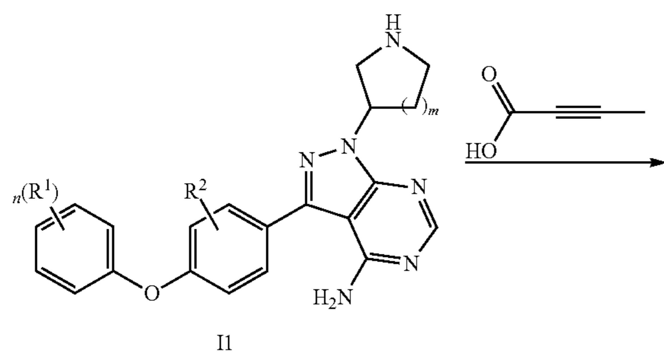
Scheme 4
