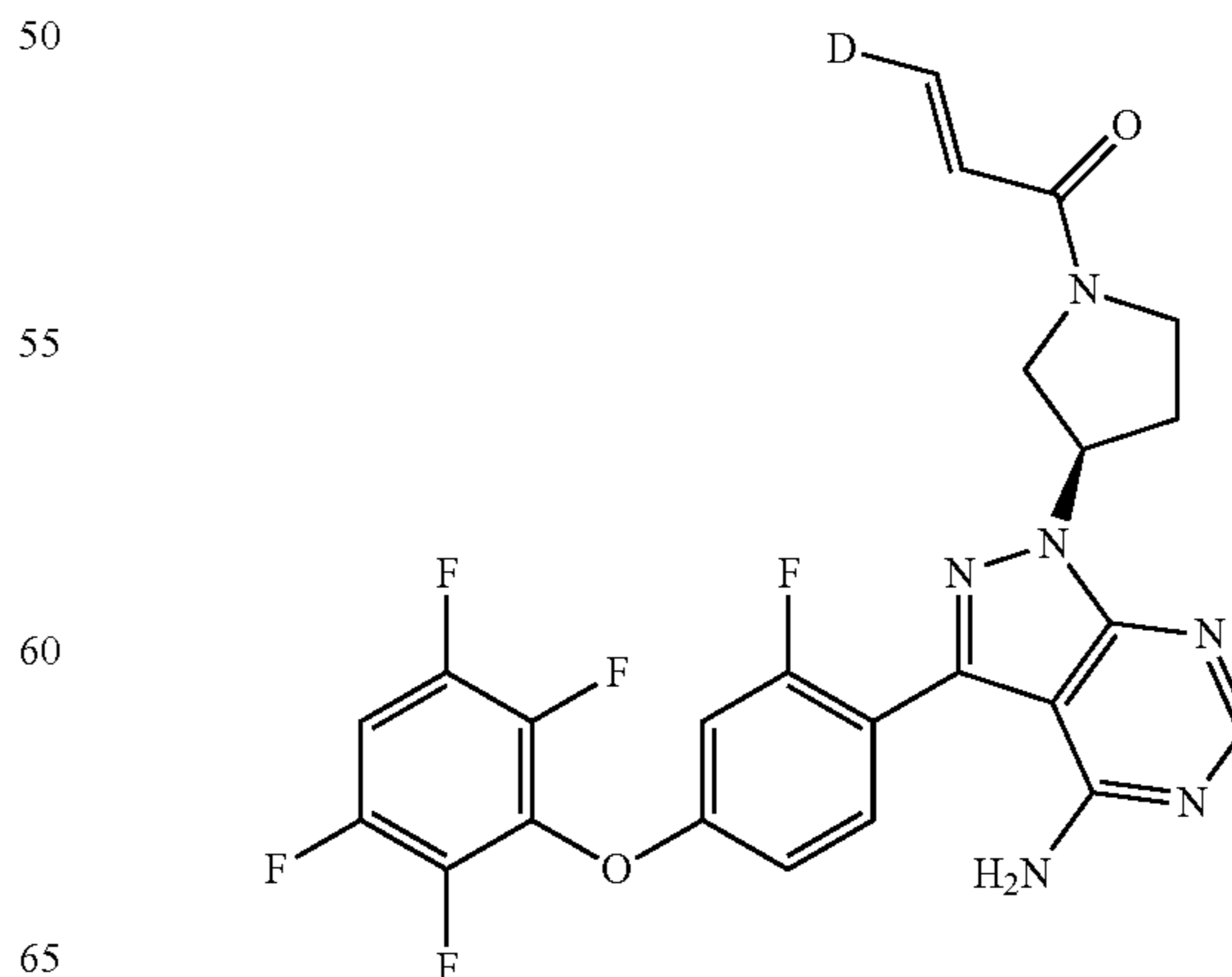
3-(2-fluoro-4-(3-fluorophenoxy)phenyl)-1-((R)-pyrrolidin-3-yl)-1H-pyrazolo[3,4-d]pyrimidin-4-amine
