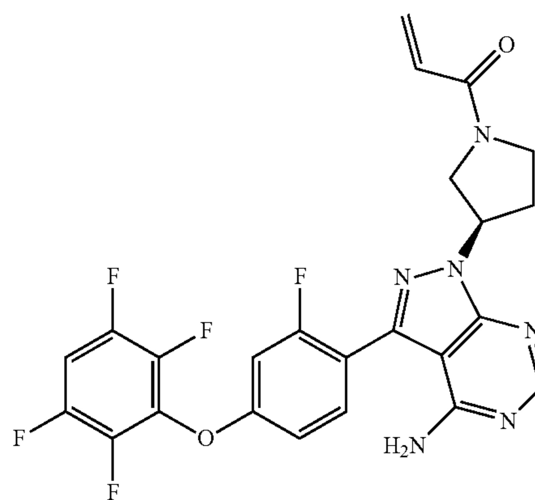
1-((R)-3-(4-amino-3-(2-fluoro-4-(2,3,5,6-tetrafluorophenoxy)phenyl)-1H-pyrazolo[3,4-d]pyrimidin-1-yl)pyrrolidin-1-yl)prop-2-en-1-one
