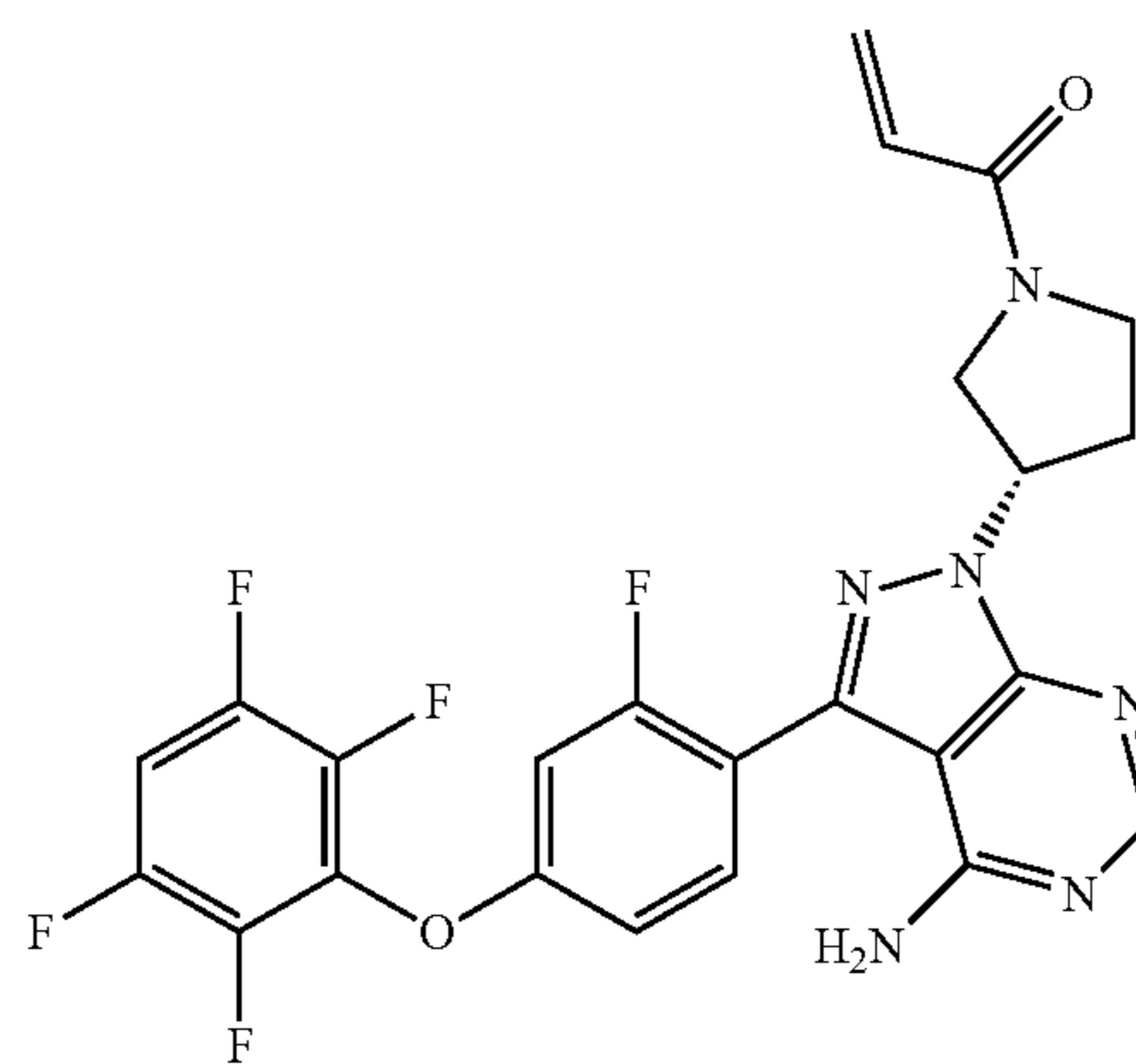
1-((S)-3-(4-amino-3-(2-fluoro-4-(2,3,5,6-tetrafluorophenoxy)phenyl)-1H-pyrazolo[3,4-d]pyrimidin-1-yl)pyrrolidin-1-yl)prop-2-en-1-one
