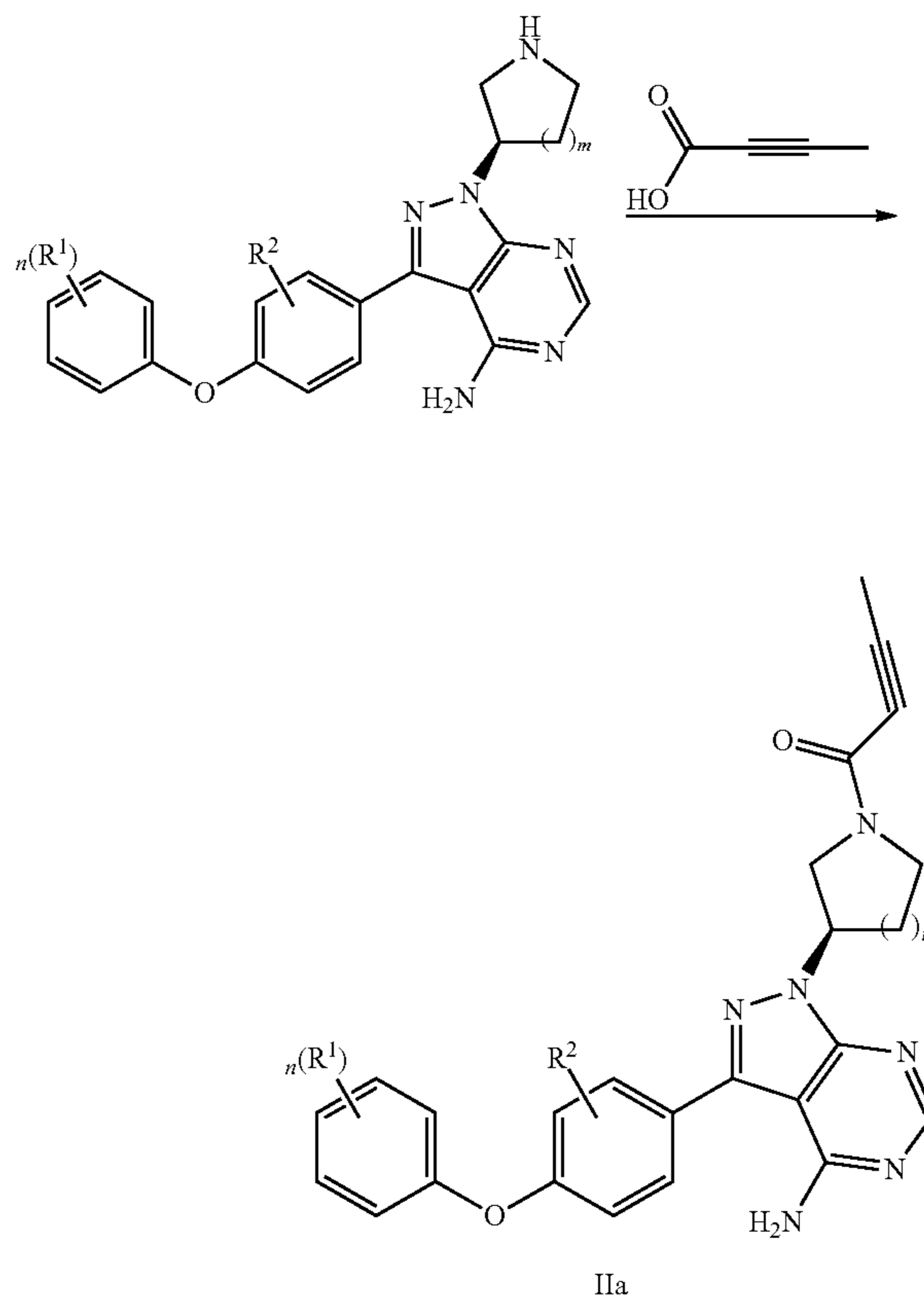
Scheme 6
