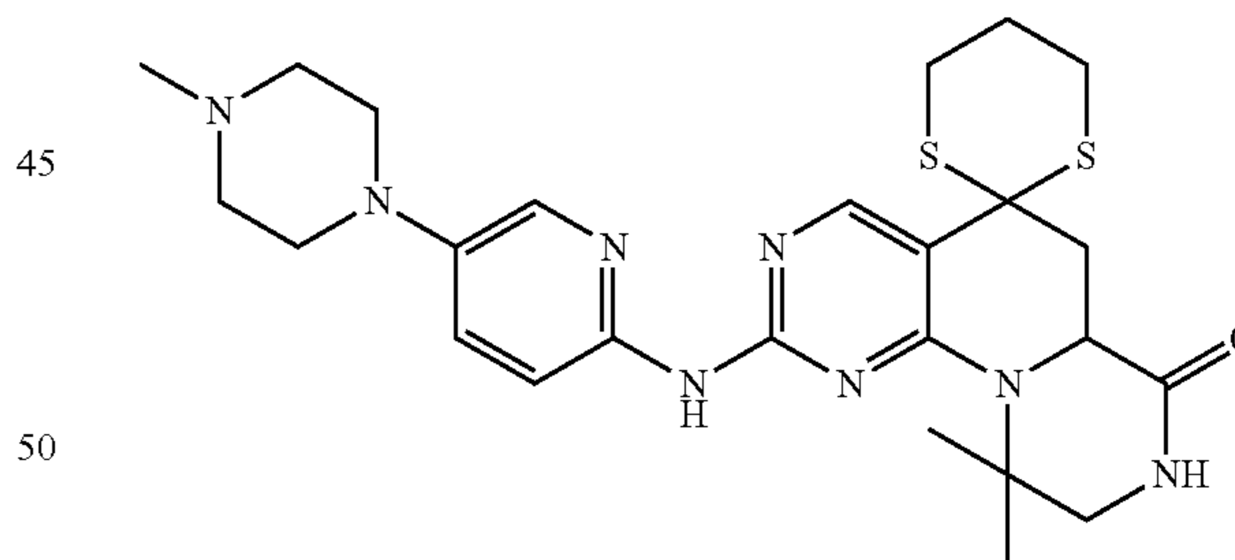
10',10'-Dimethyl-2'-([5-(4-methylpiperazin-1-yl)pyridin-2-yl]amino)-6',6a',9',10'-tetrahydrodispiro[1,3-dithiane-2,5'-pyrazino[1',2':1,6]pyrido[2,3-d]pyrimidine]-7'(8'H)-one
