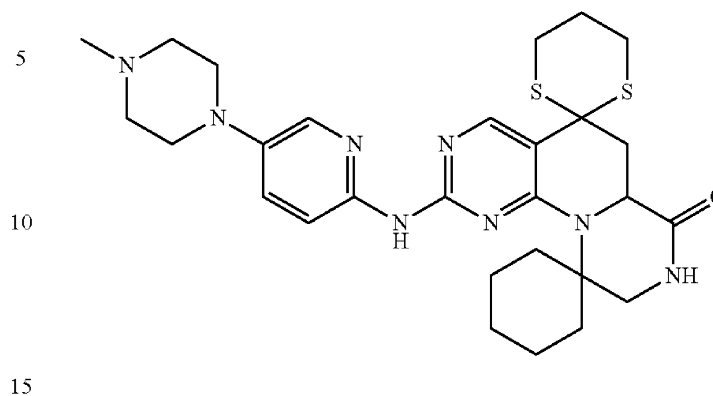
2'-([5-(4-Methylpiperazin-1-yl)pyridin-2-yl]amino)-6',6a',8',9'-tetrahydro-7'H-dispiro[cyclohexane-1,10'-pyrazino[1',2':1,6]pyrido[2,3-d]pyrimidine-5',2''-[1,3]dithian]-7'-one
