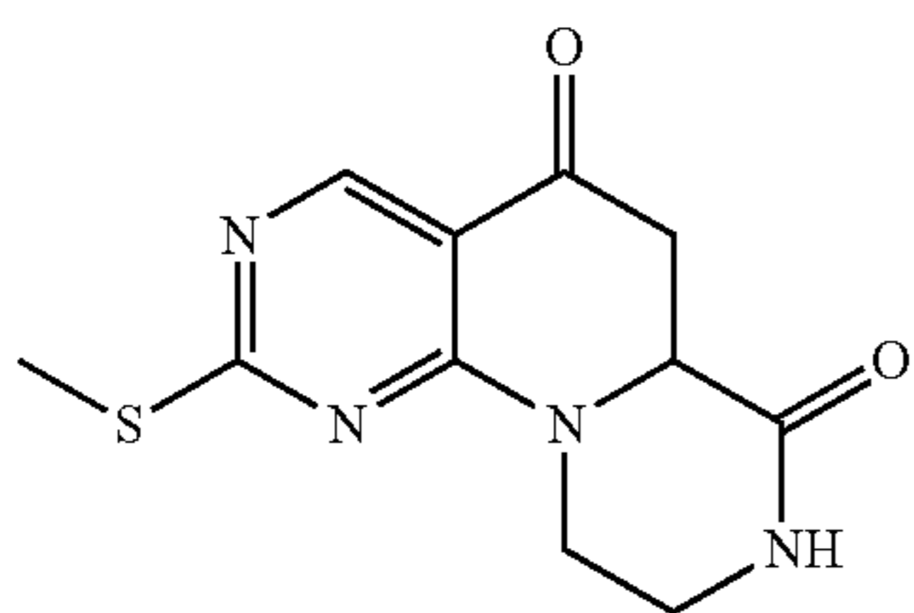
2-(Methylthio)-6,6a,9,10-tetrahydro-5H-pyrazino[1',2':1,6]pyrido[2,3-d]pyrimidine-5,7(8H)-dione
