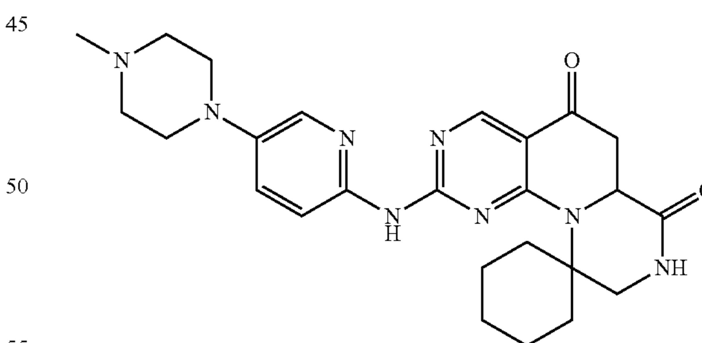
2'-{[5-(4-Methylpiperazin-1-yl)pyridin-2-yl]amino}-6',6a',8',9'-tetrahydrospiro[cyclohexane-1,10'-pyrazino[1',2':1,6]pyrido[2,3-d]pyrimidine]-5',7'-dione
