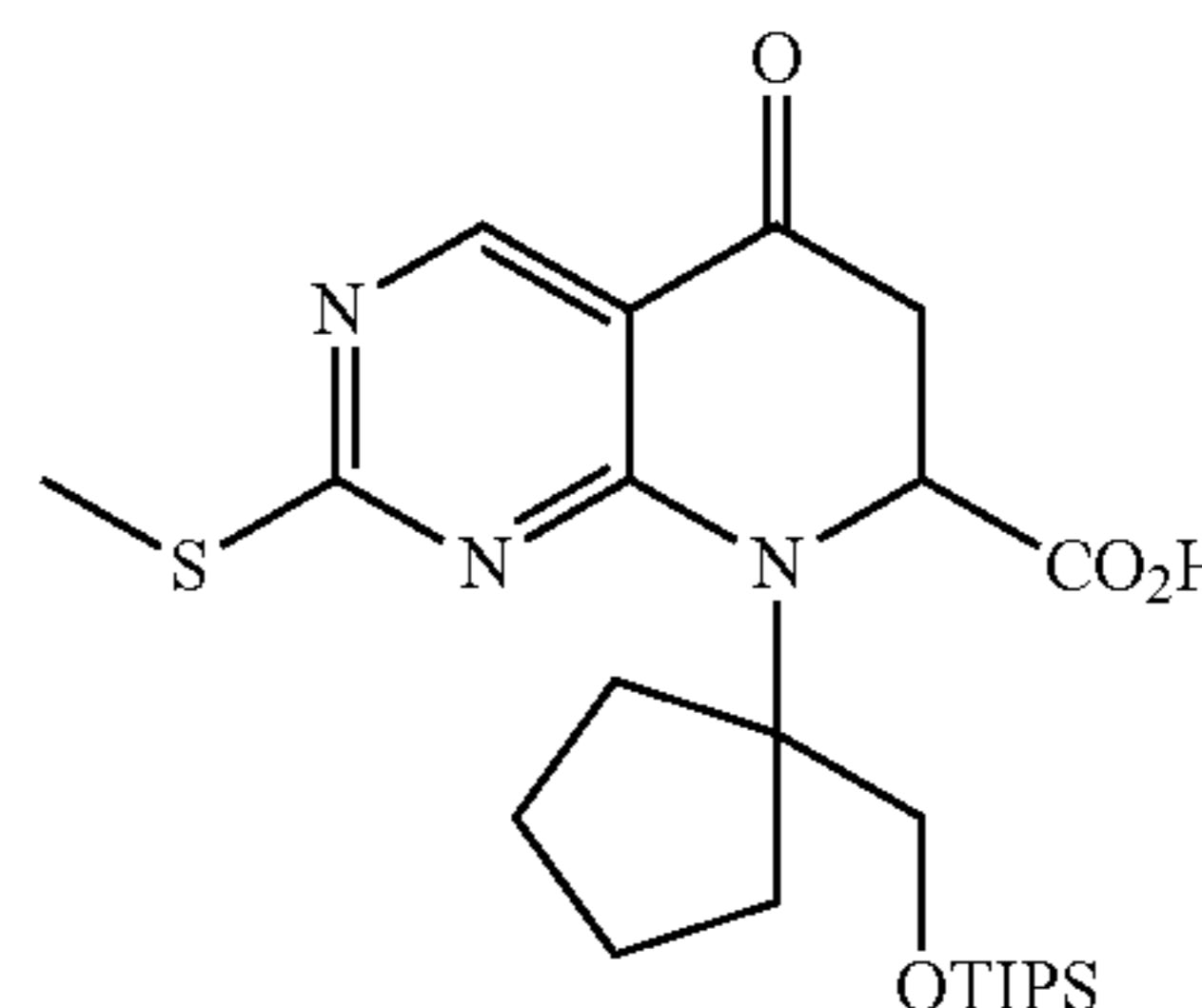
2-(Methylthio)-5-oxo-8-(1-[(triisopropylsilyloxy)methyl]cyclopentyl)-5,6,7,8-tetrahydropyrido[2,3-d]pyrimidine-7-carboxylic acid
