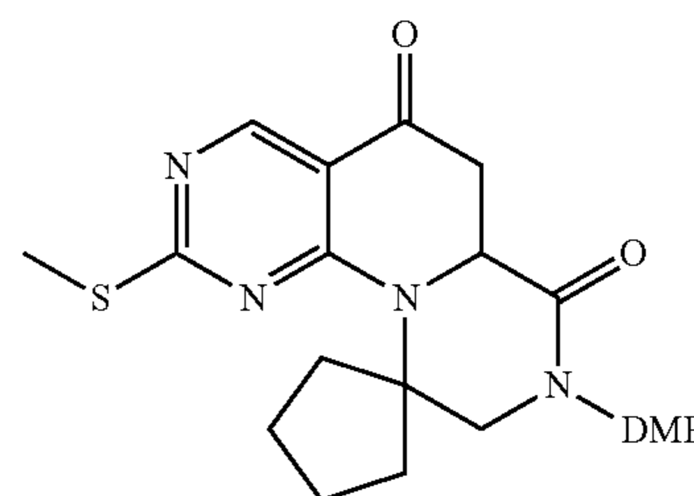
8'-(2,4-Dimethoxybenzyl)-2'-(methylthio)-6',6a',8',9'-tetrahydrospiro[cyclopentane-1,10'-pyrazino[1',2':1,6]pyrido[2,3-d]pyrimidine]-5',7'-dione
