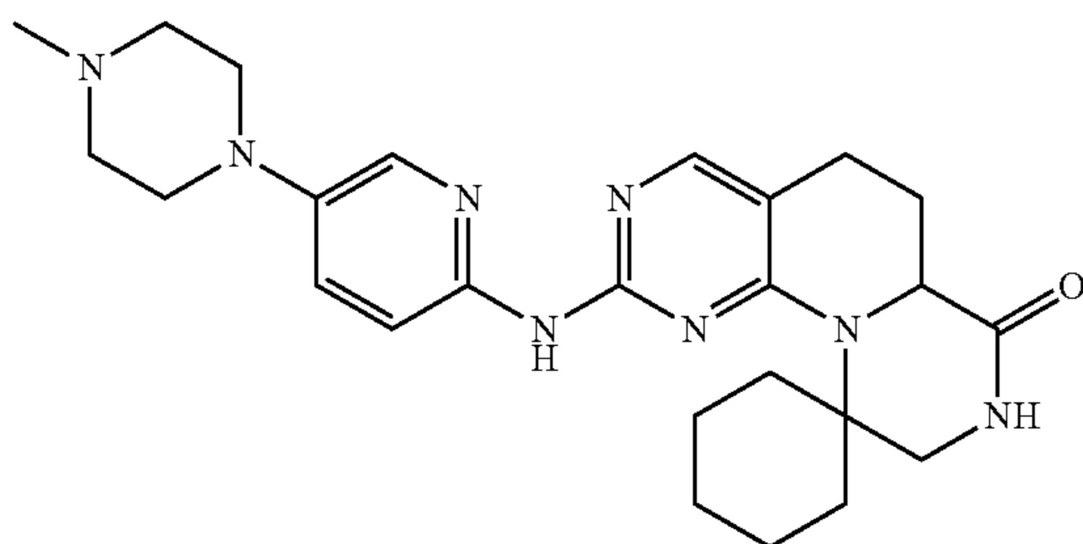
2'--[5-(4-Methylpiperazin-1-yl)pyridin-2-yl]amino}-6',6a',8',9'-tetrahydrospiro[cyclohexane-1,10'-pyrazino[1',2':1,6]pyrido[2,3-d]pyrimidin]-7'(5'H)-one
