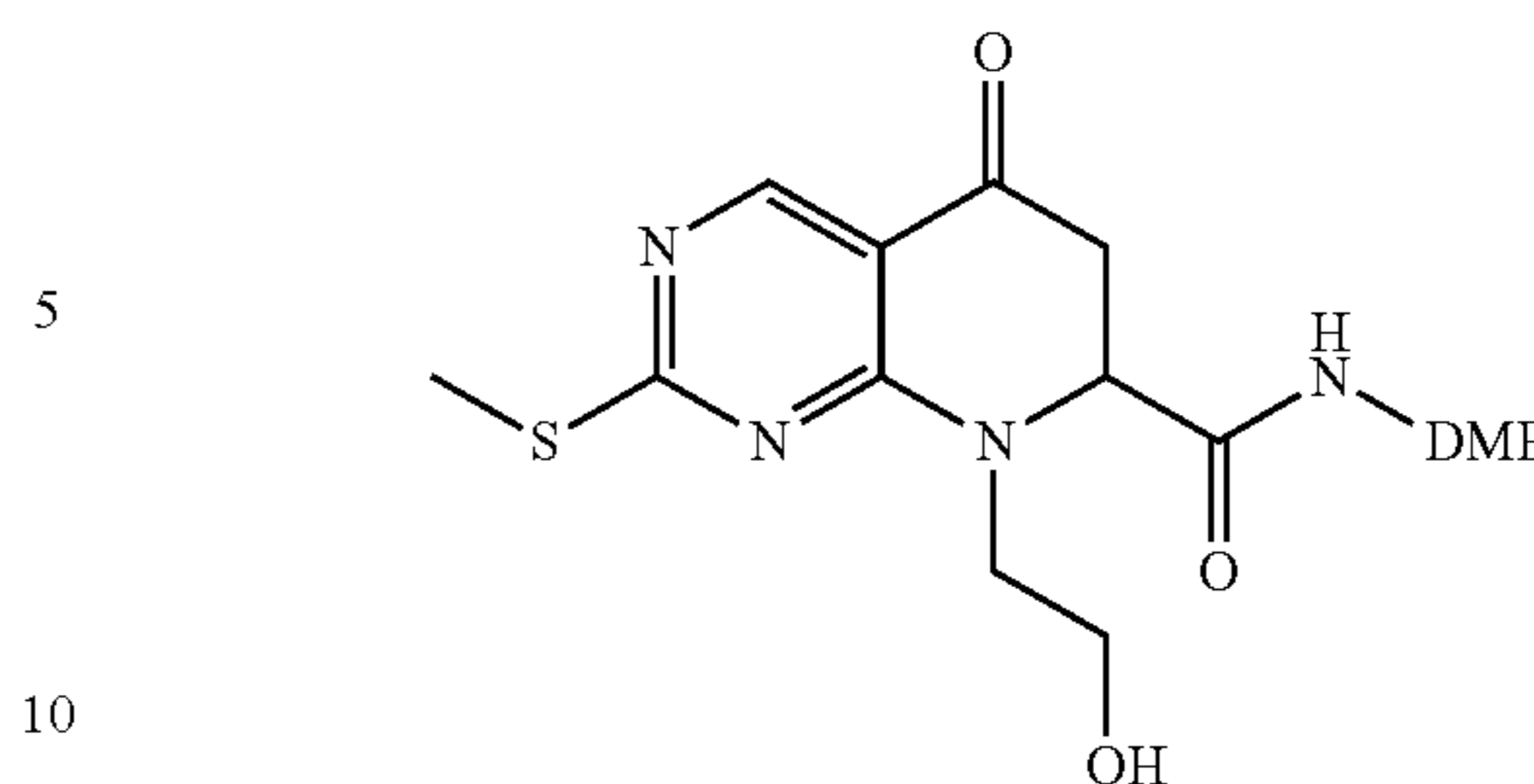
N-(2,4-Dimethoxybenzyl)-8-(2-hydroxyethyl)-2-(methylthio)-5-oxo-5,6,7,8-tetrahydropyrido[2,3-d]pyrimidine-7-carboxamide
