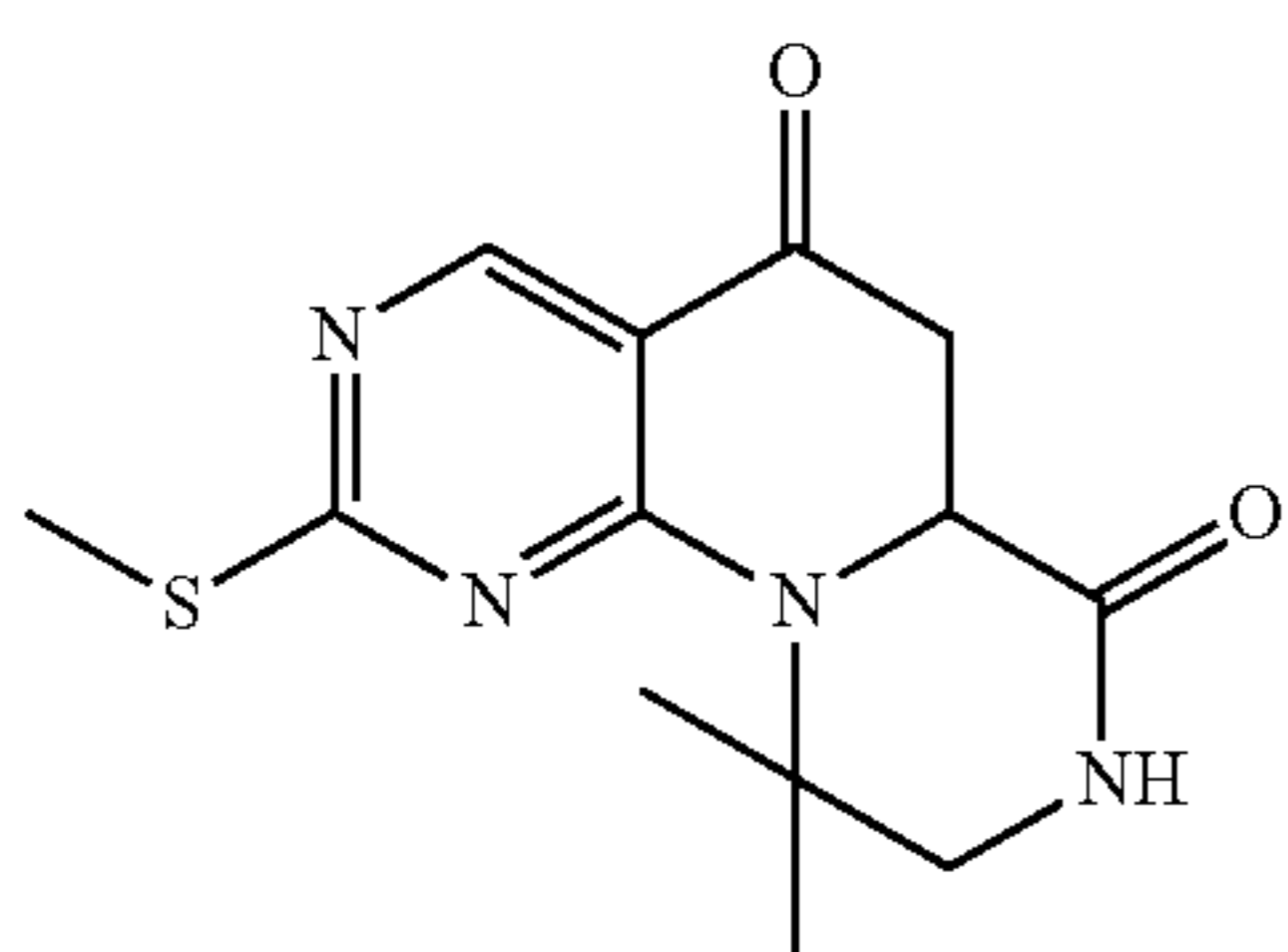
10,10-Dimethyl-2-(methylthio)-6,6a,9,10-tetrahydro-5H-pyrazino[1',2':1,6]pyrido[2,3-d]pyrimidine-5,7(8H)-dione
