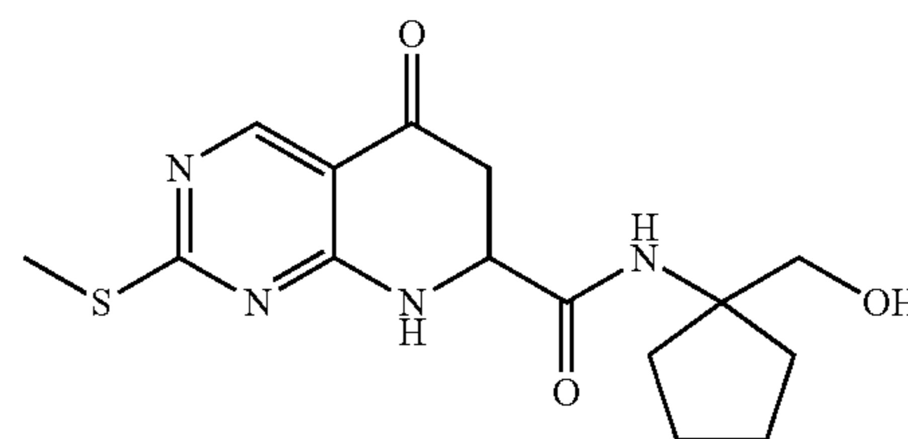
N-[1-(Hydroxymethyl)cyclopentyl]-2-(methylthio)-5-oxo-5,6,7,8-tetrahydropyrido[2,3-d]pyrimidine-7-carboxamide
