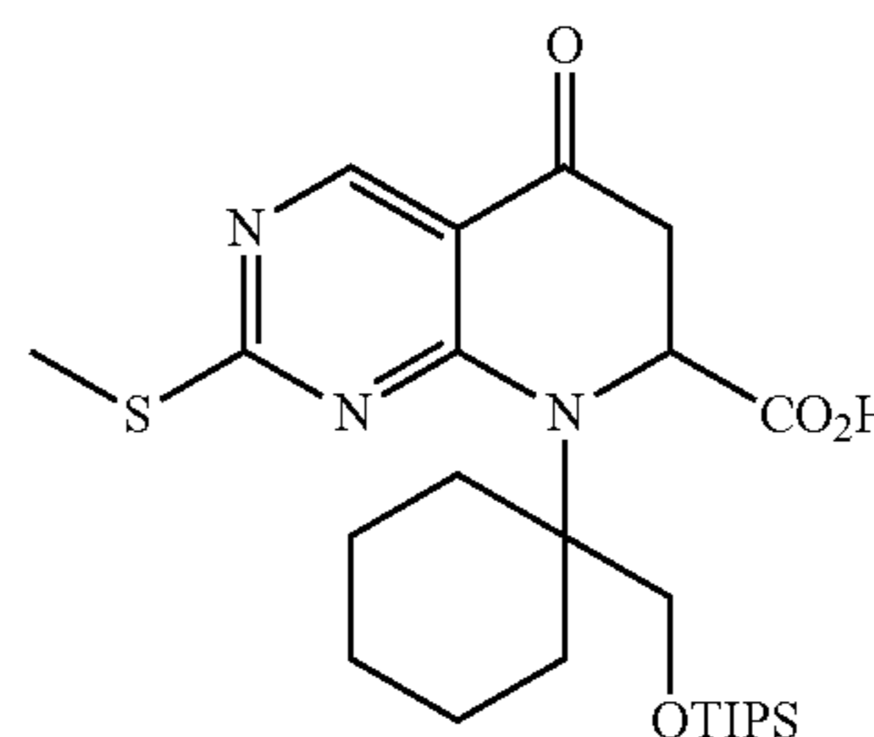
2-(Methylthio)-5-oxo-8-(1-[(triisopropylsilyloxy)methyl]cyclohexyl)-5,6,7,8-tetrahydropyrido[2,3-d]pyrimidine-7-carboxylic acid
