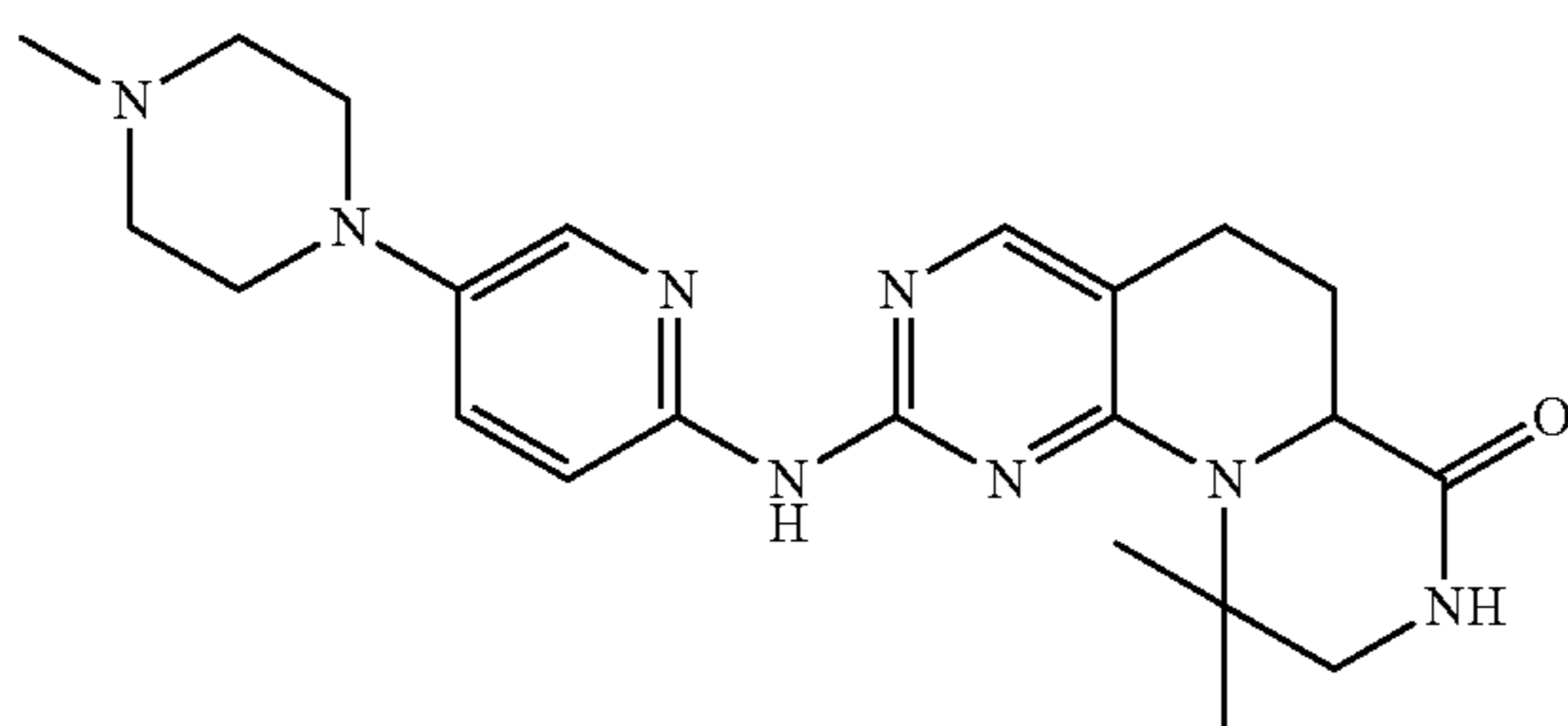
10,10-Dimethyl-2'--[5-(4-methylpiperazin-1-yl)pyridin-2-yl]amino}-6',6a',9,10-tetrahydro-5H-pyrazino[1',2':1,6]pyrido[2,3-d]pyrimidin-7'(8'H)-one
