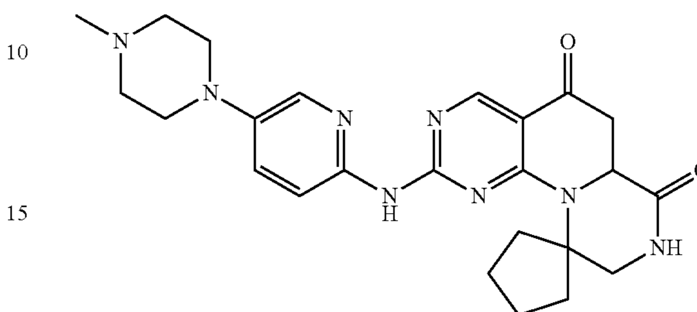
2'-{[5-(4-Methylpiperazin-1-yl)pyridin-2-yl]amino}-6',6a',8',9'-tetrahydrospiro[cyclopentane-1,10'-pyrazino[1',2':1,6]pyrido[2,3-d]pyrimidine]-5',7'-dione
