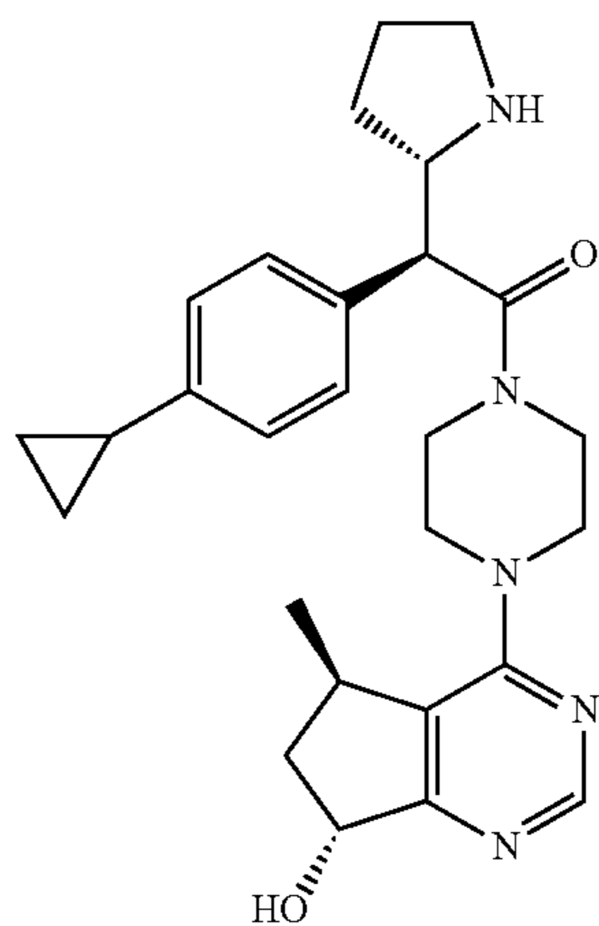
(S)-2-(4-cyclopropylphenyl)-1-(4-((5R,7R)-7-hydroxy-5-methyl-6,7-dihydro-5H-cyclopenta[d]pyrimidin-4-yl)piperazin-1-yl)-2-((S)-pyrrolidin-2-yl)ethanone
