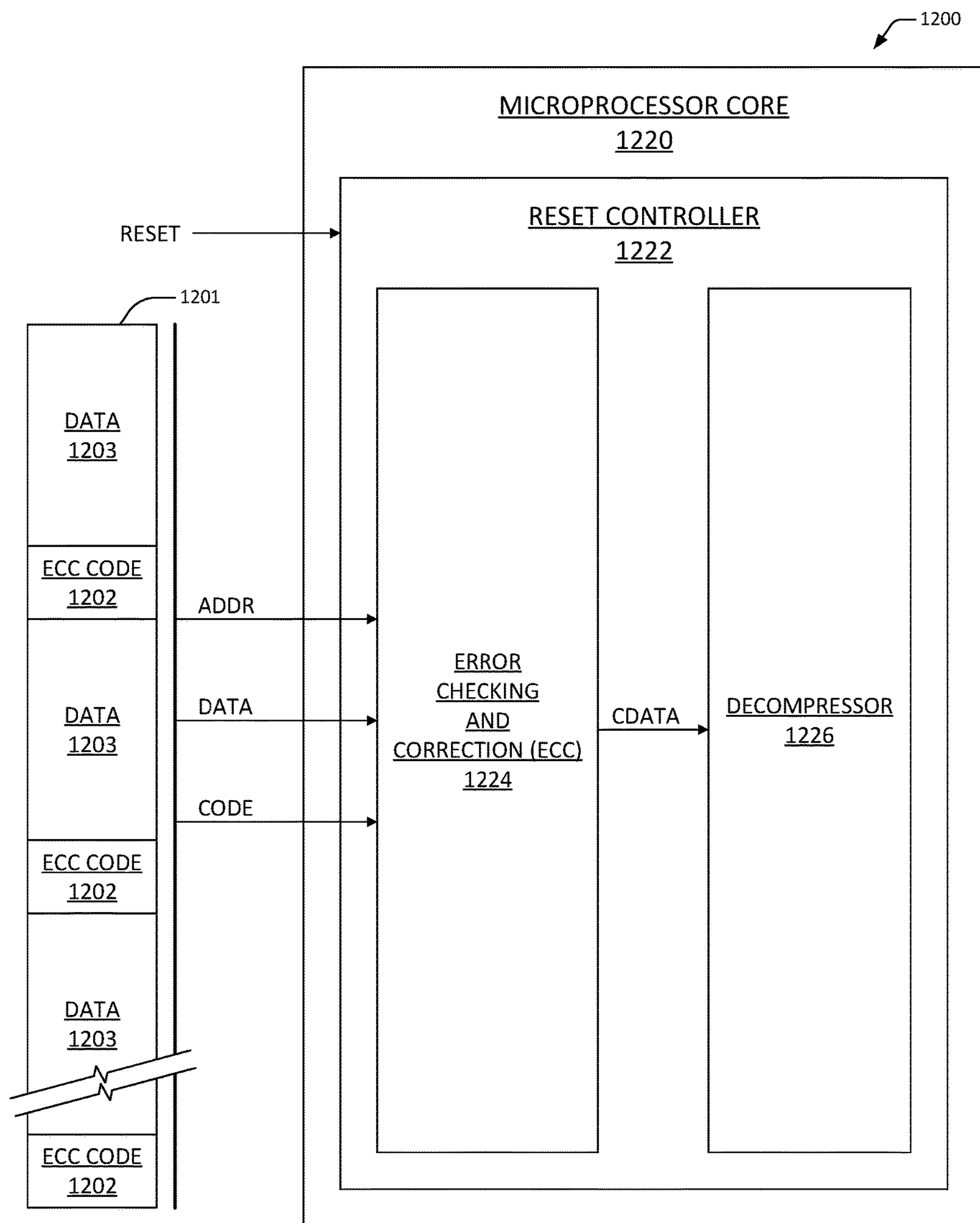
ERROR CHECKING AND CORRECTION (ECC) MECHANISM
