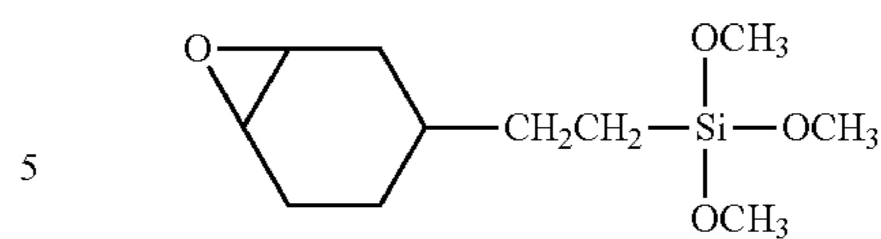
Beta-(3,4-Epoxy)cyclohexyl ethyltrimethoxysilane
