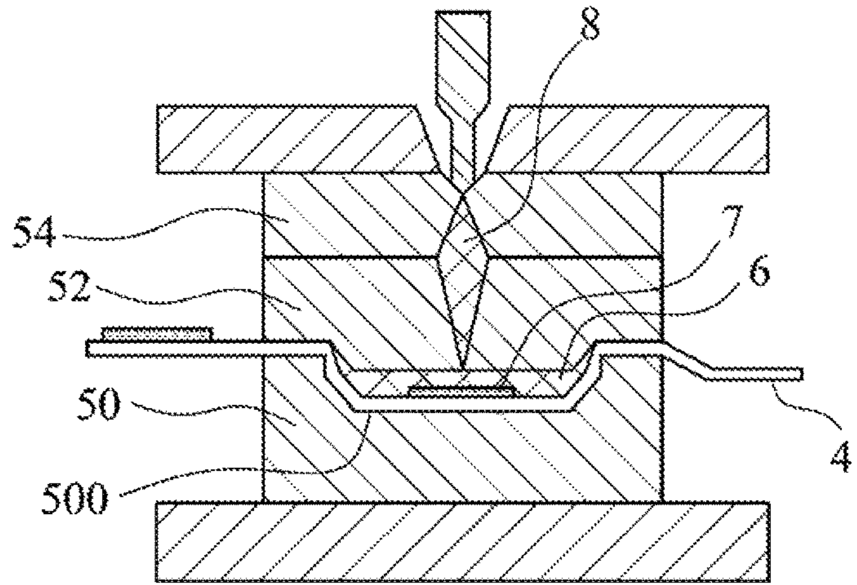
Fig. 5C (PRIOR ART)
