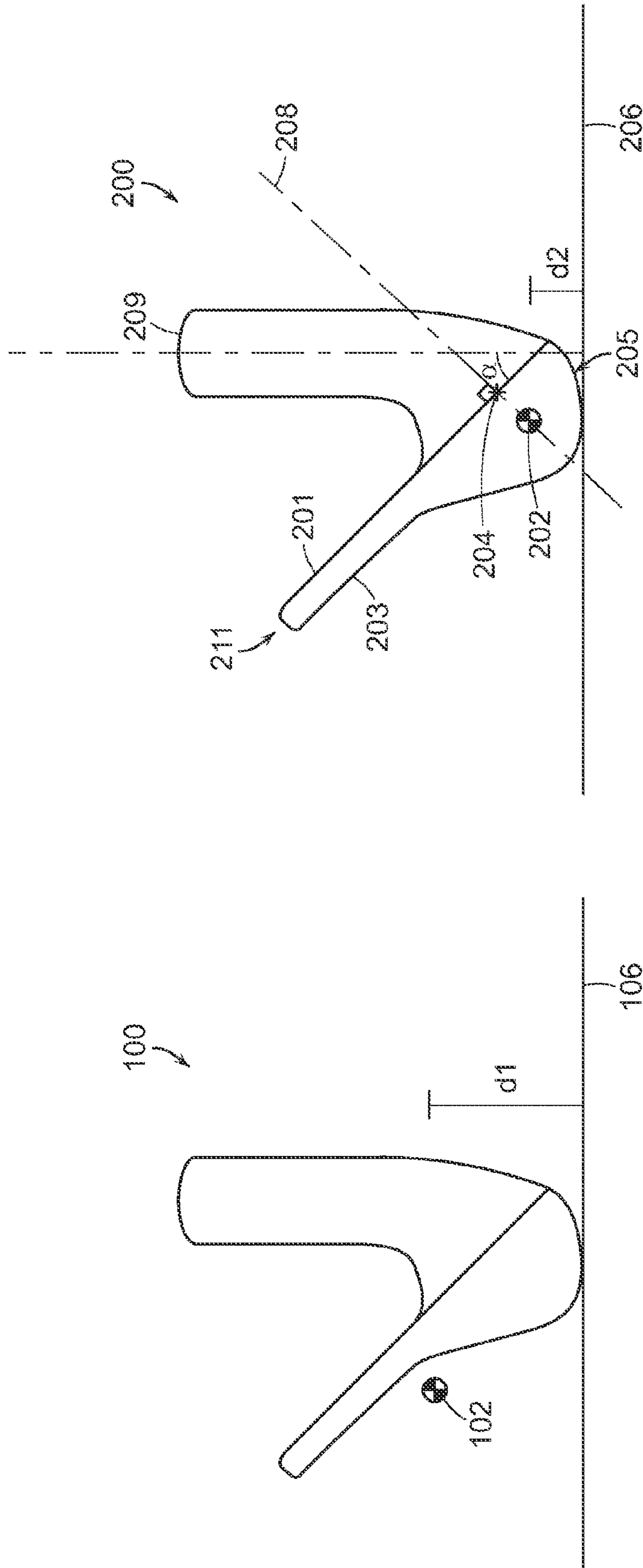
FIG. 1 (Prior Art)
