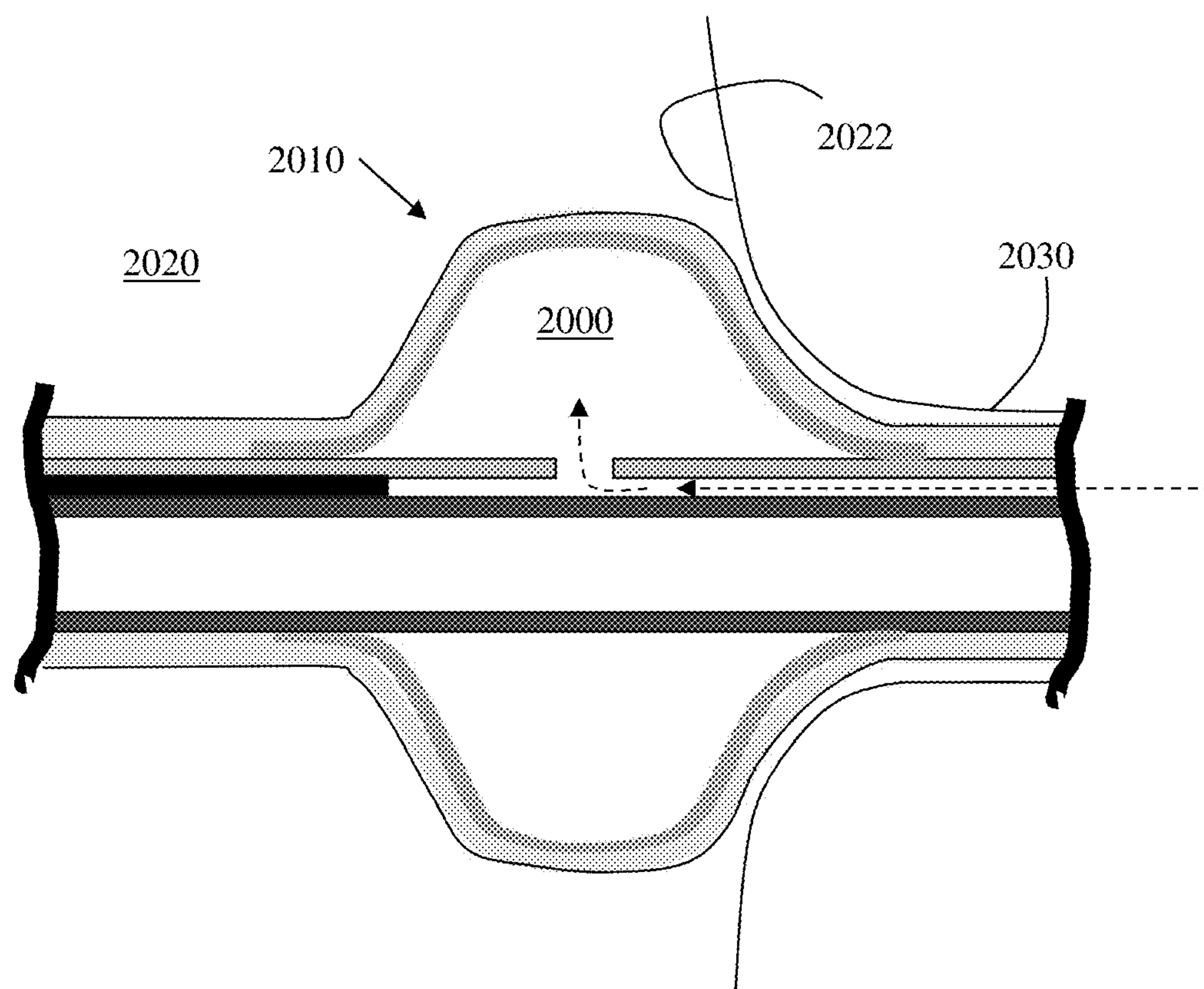
FIG. 20 Prior Art
