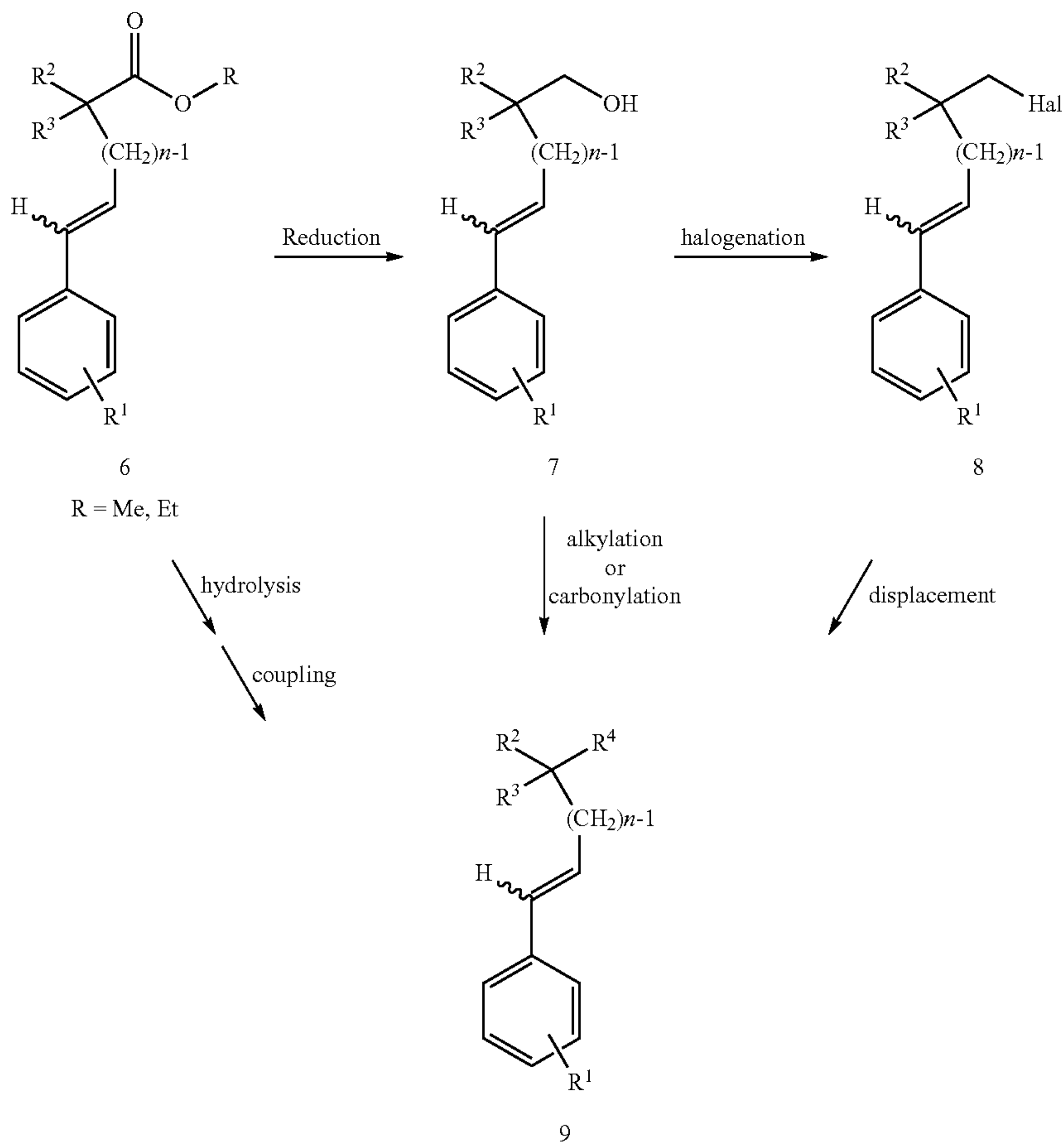
Scheme 2:
