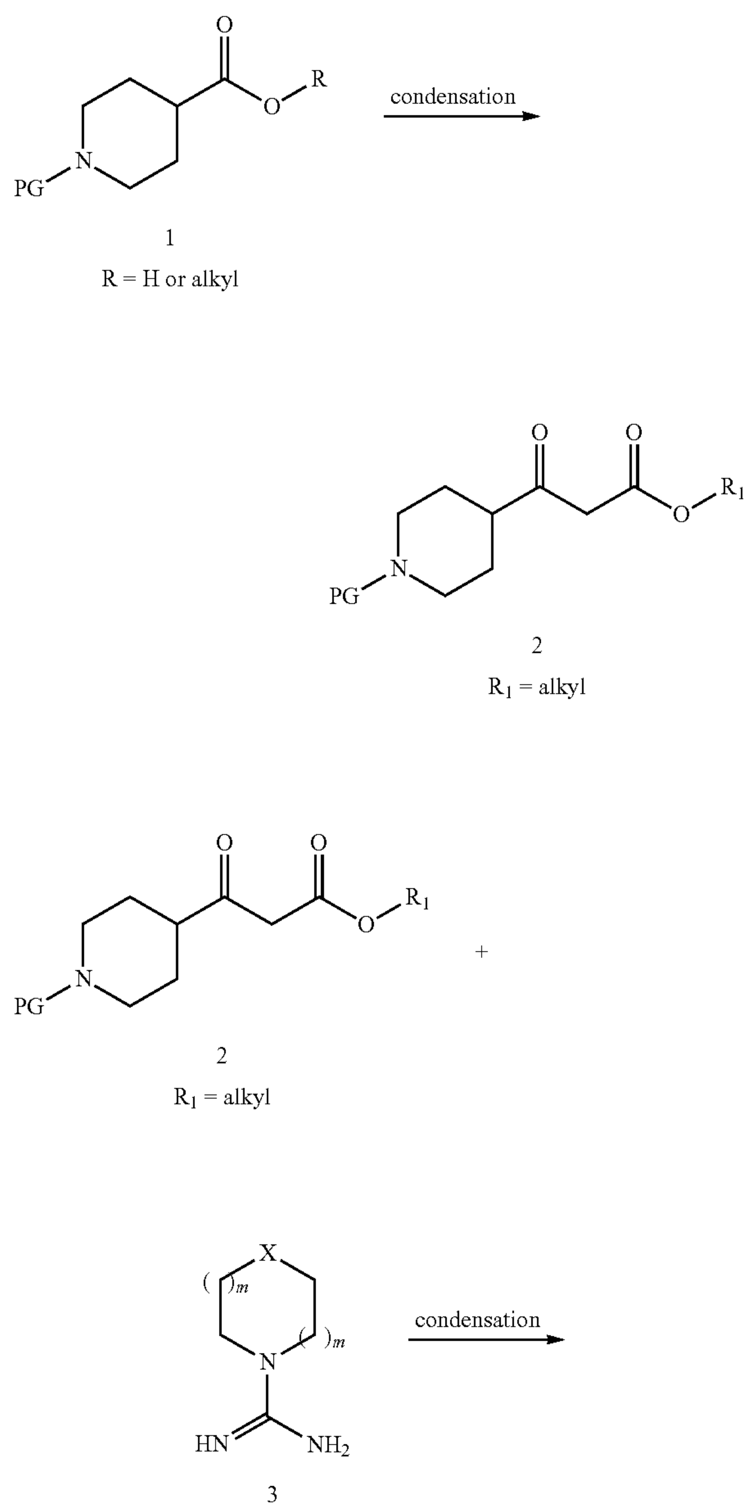
Scheme 1:
