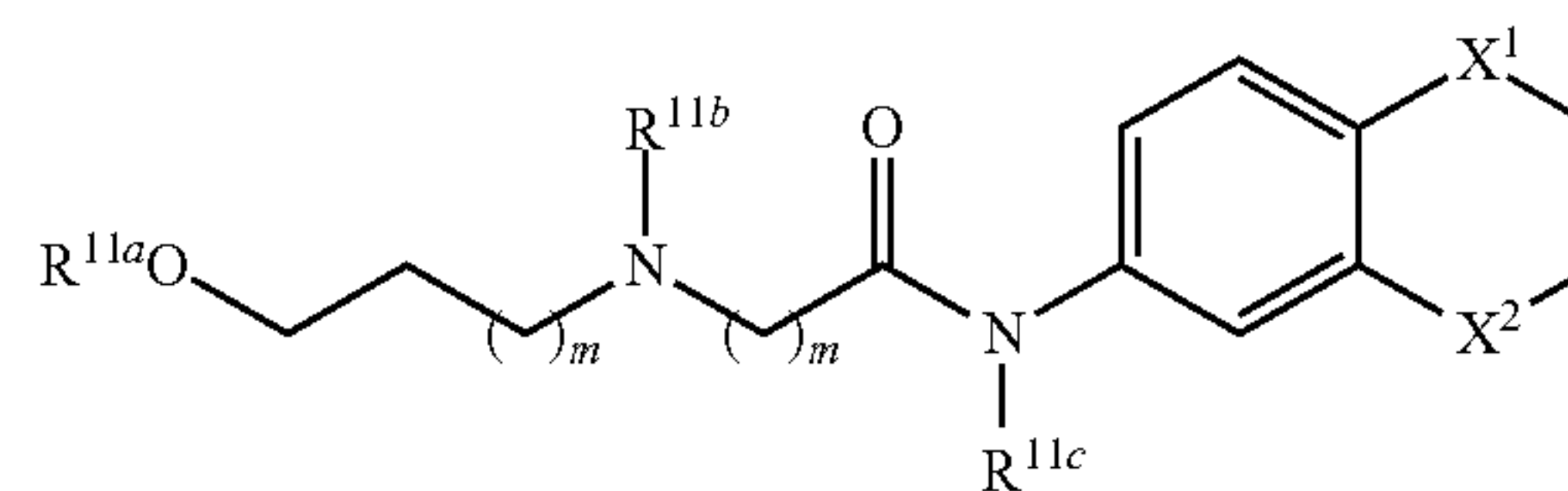
Formula IX
