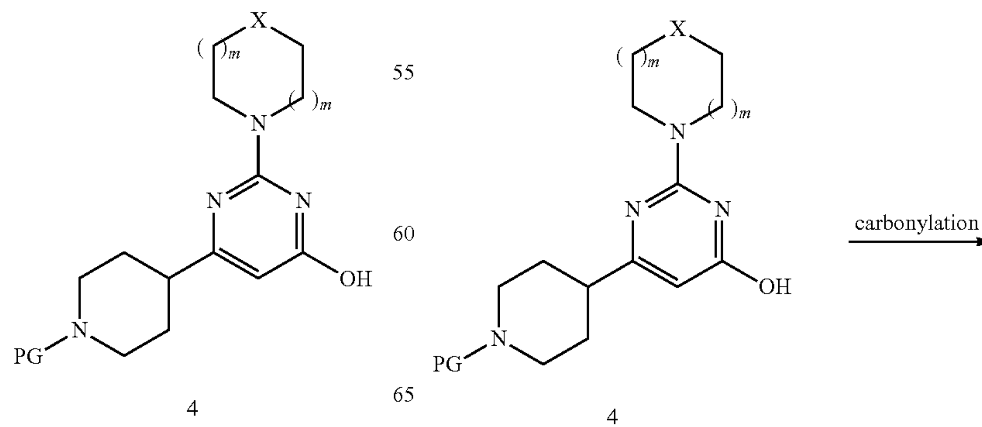
Scheme 3:
