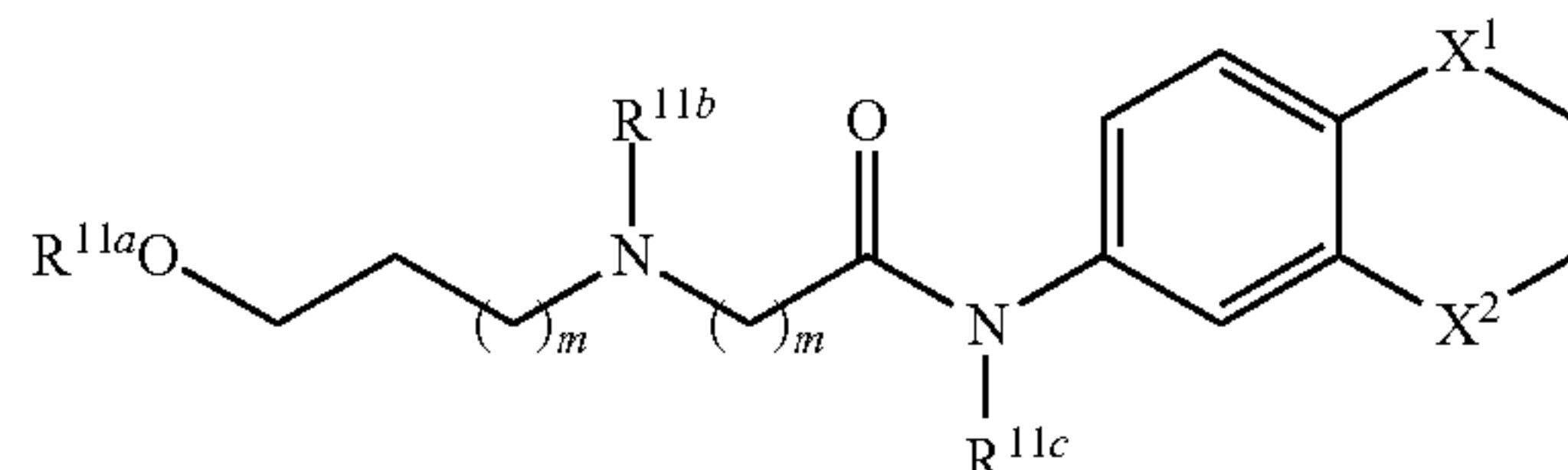
Formula IX
