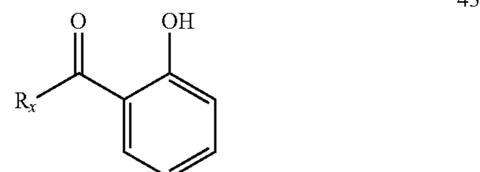
(salicylaldehyde)
