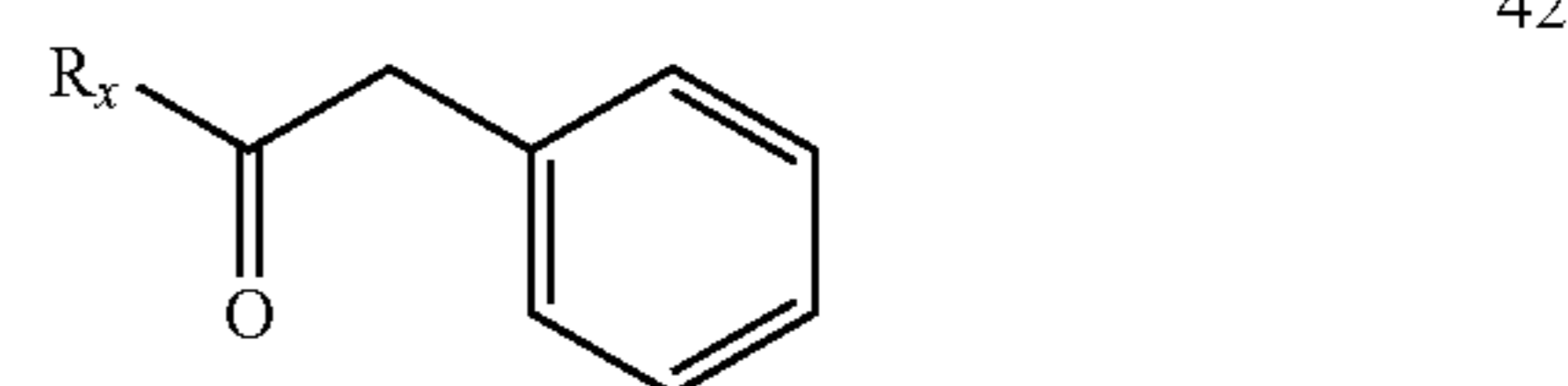
(2-phenylacetaldehyde)
