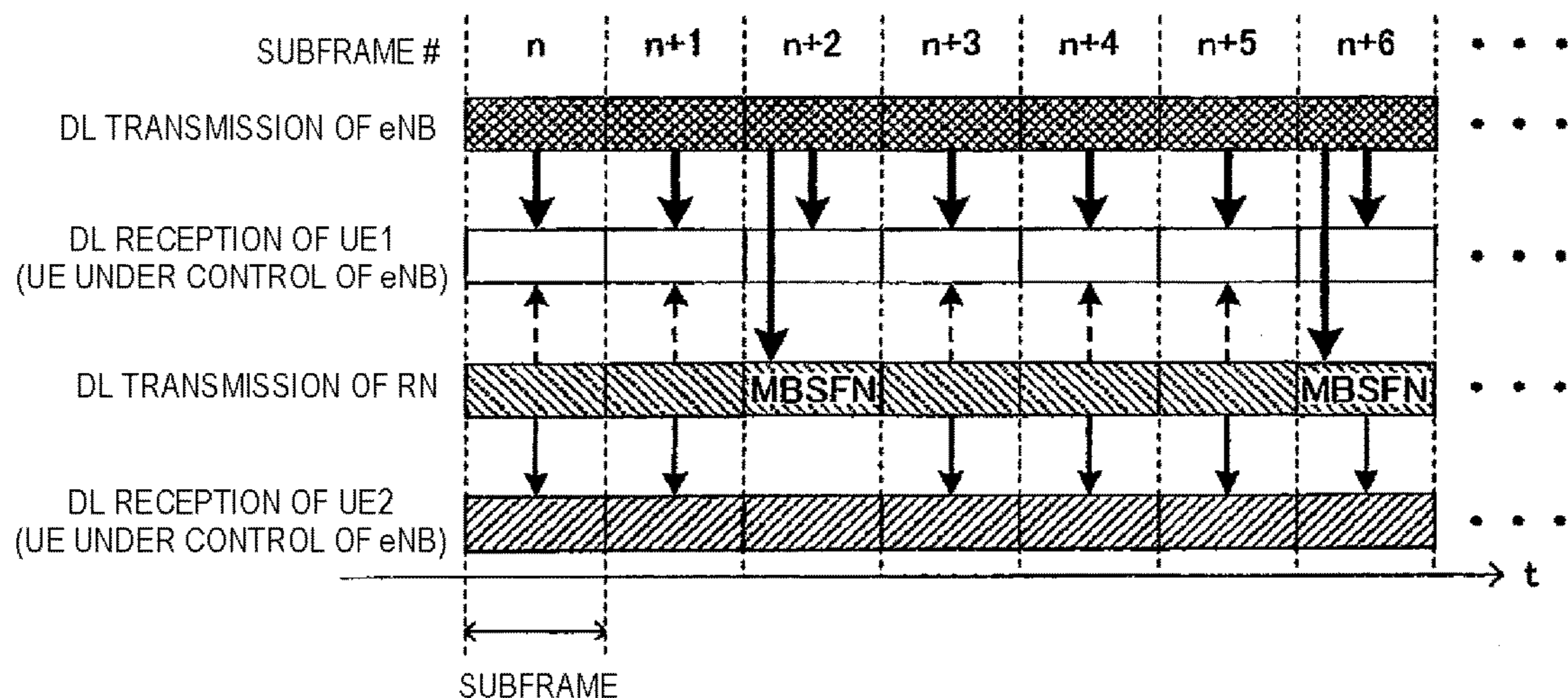
FIG. 21 (PRIOR ART)
