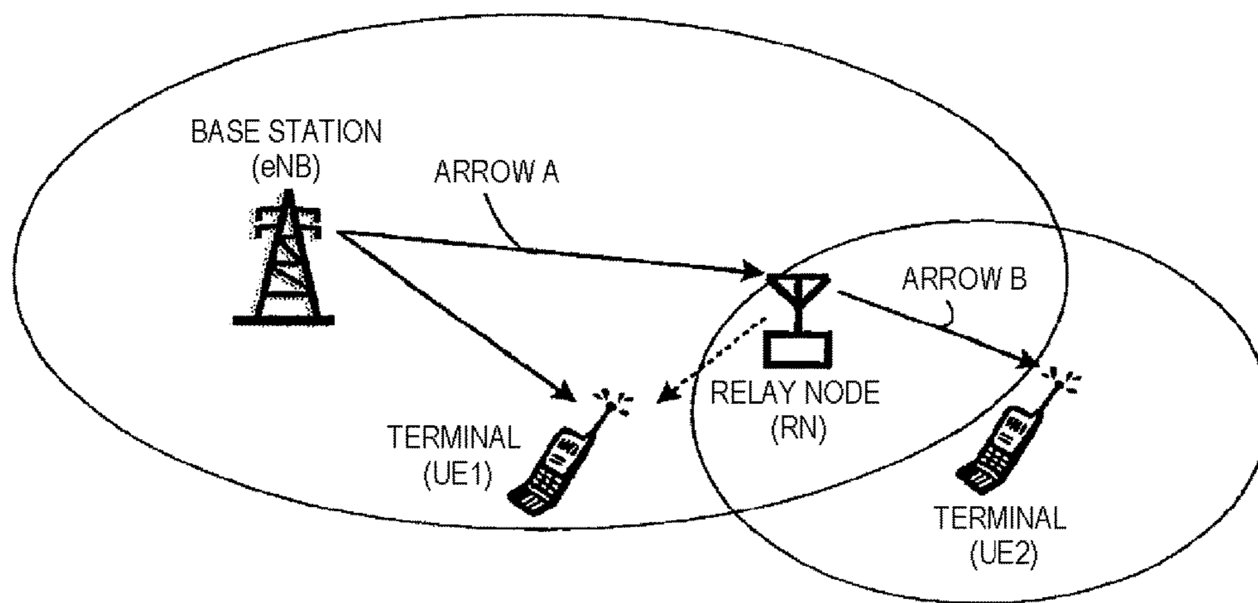
FIG. 21 (PRIOR ART)
