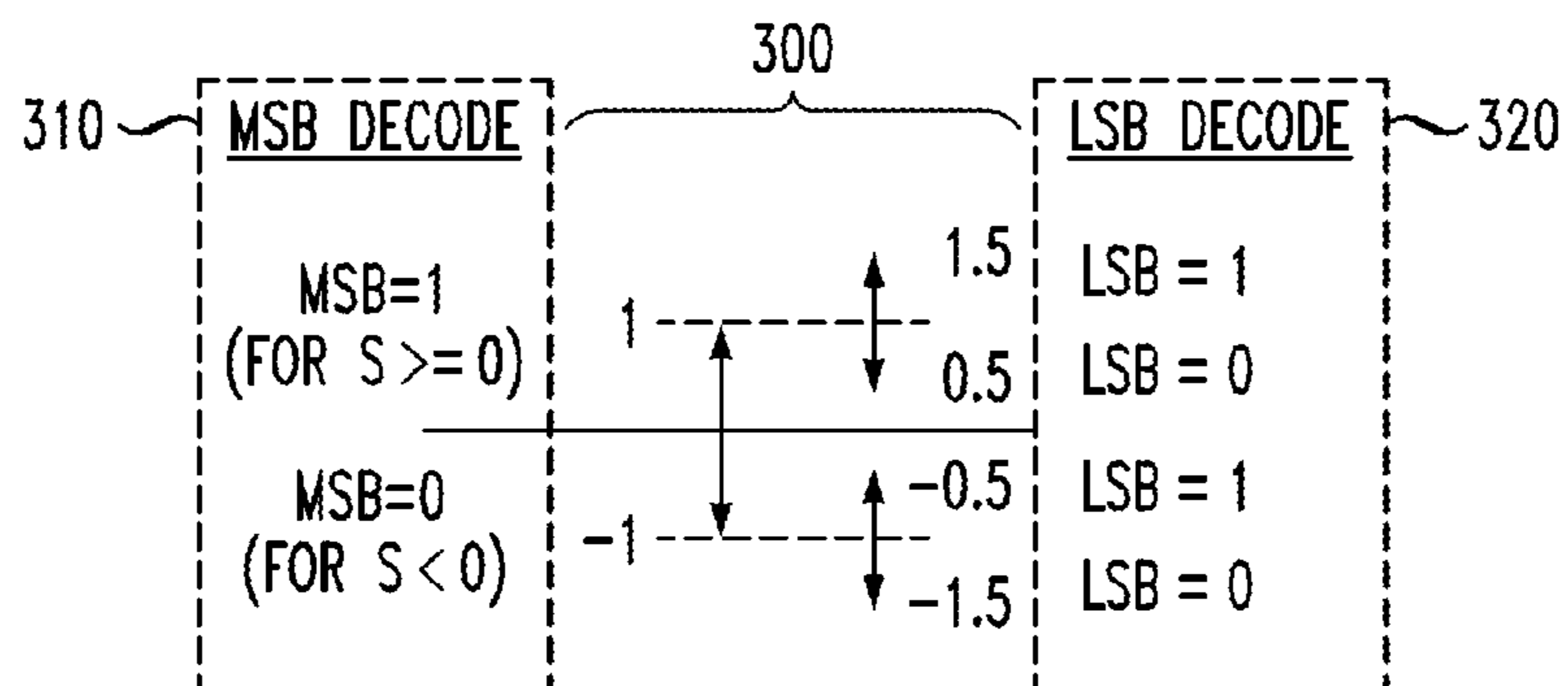
4-LEVEL SIGNAL MSB AND LSB COMPONENTS AND MSB DECODE/LSB DECODE FUNCTION
