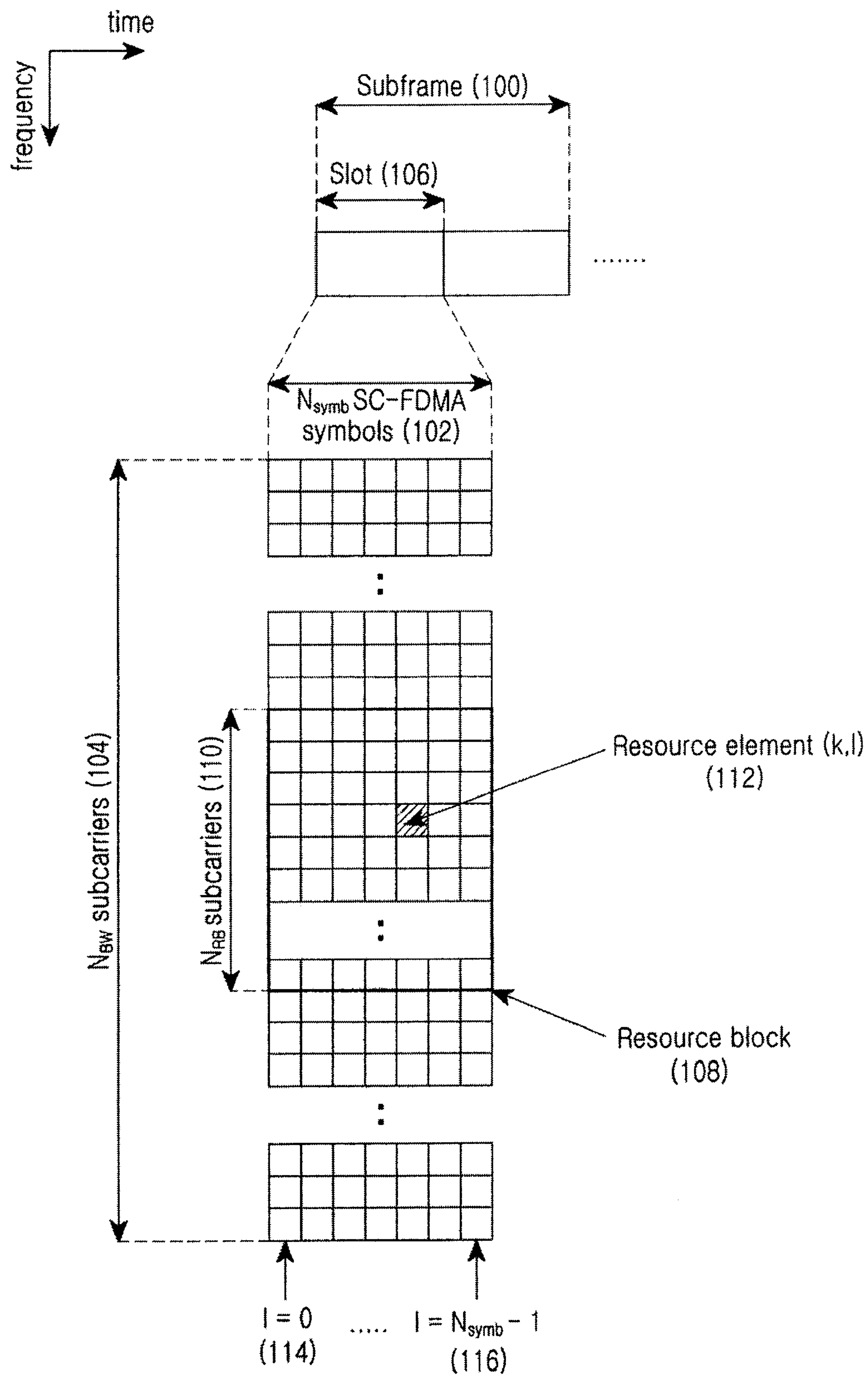
FIG.1 (CONVENTIONAL ART)
