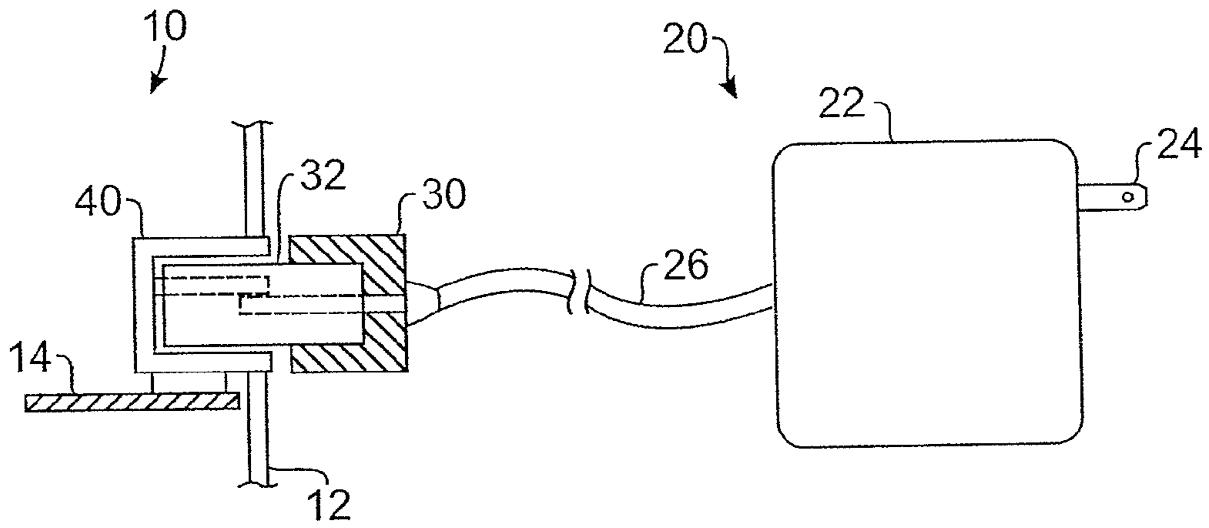
FIG. 1 (Prior Art)
