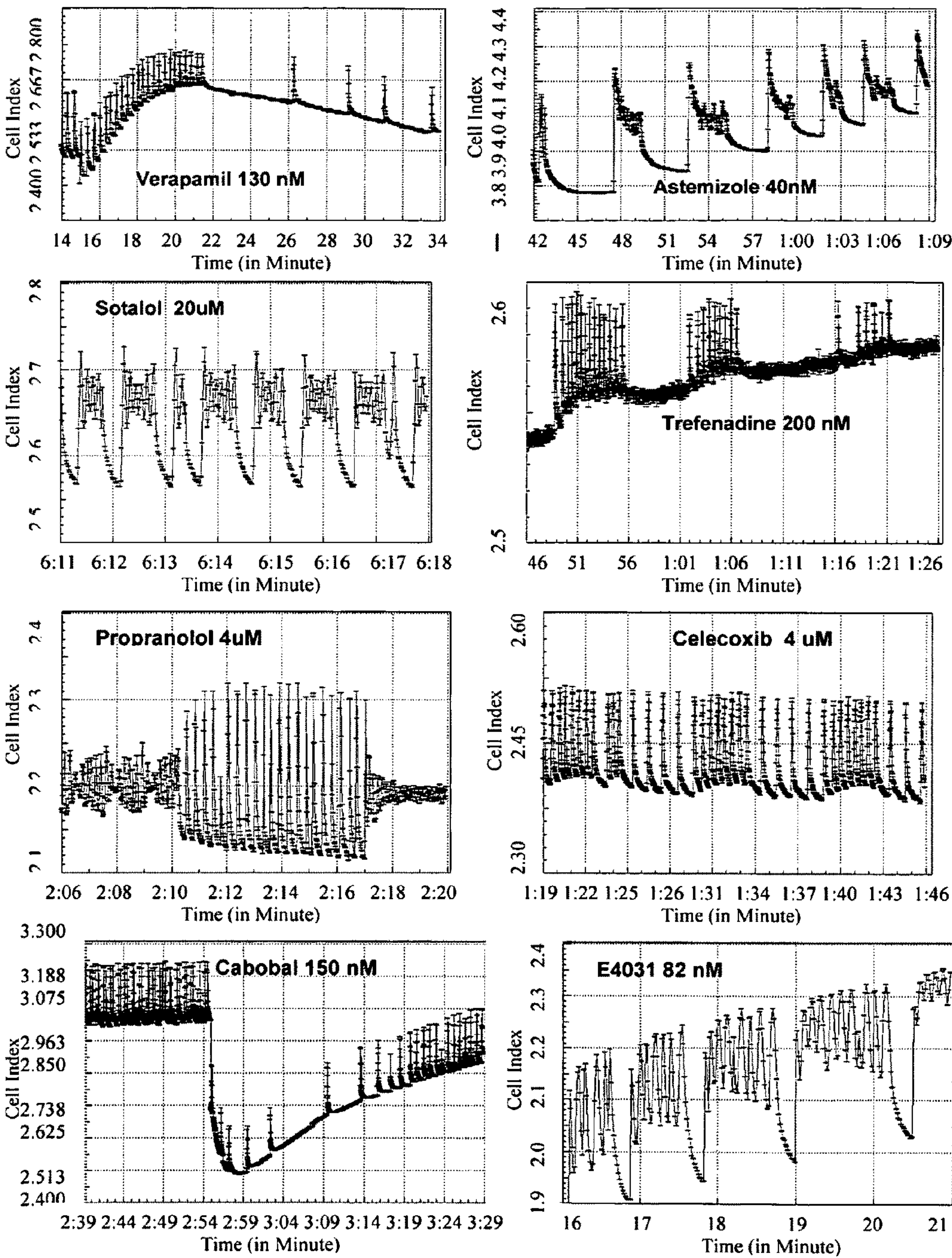
FIG. 12 Cardiotoxic Patterns
