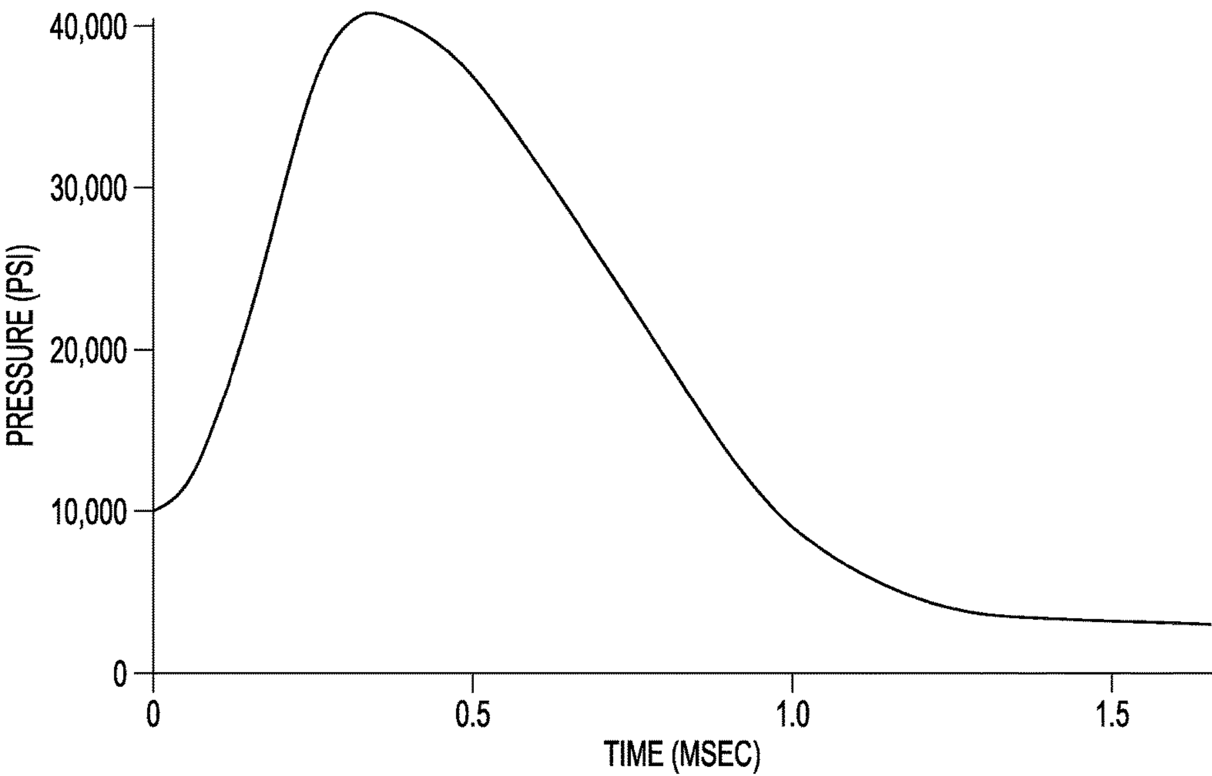
FIG. 15 PRIOR ART
