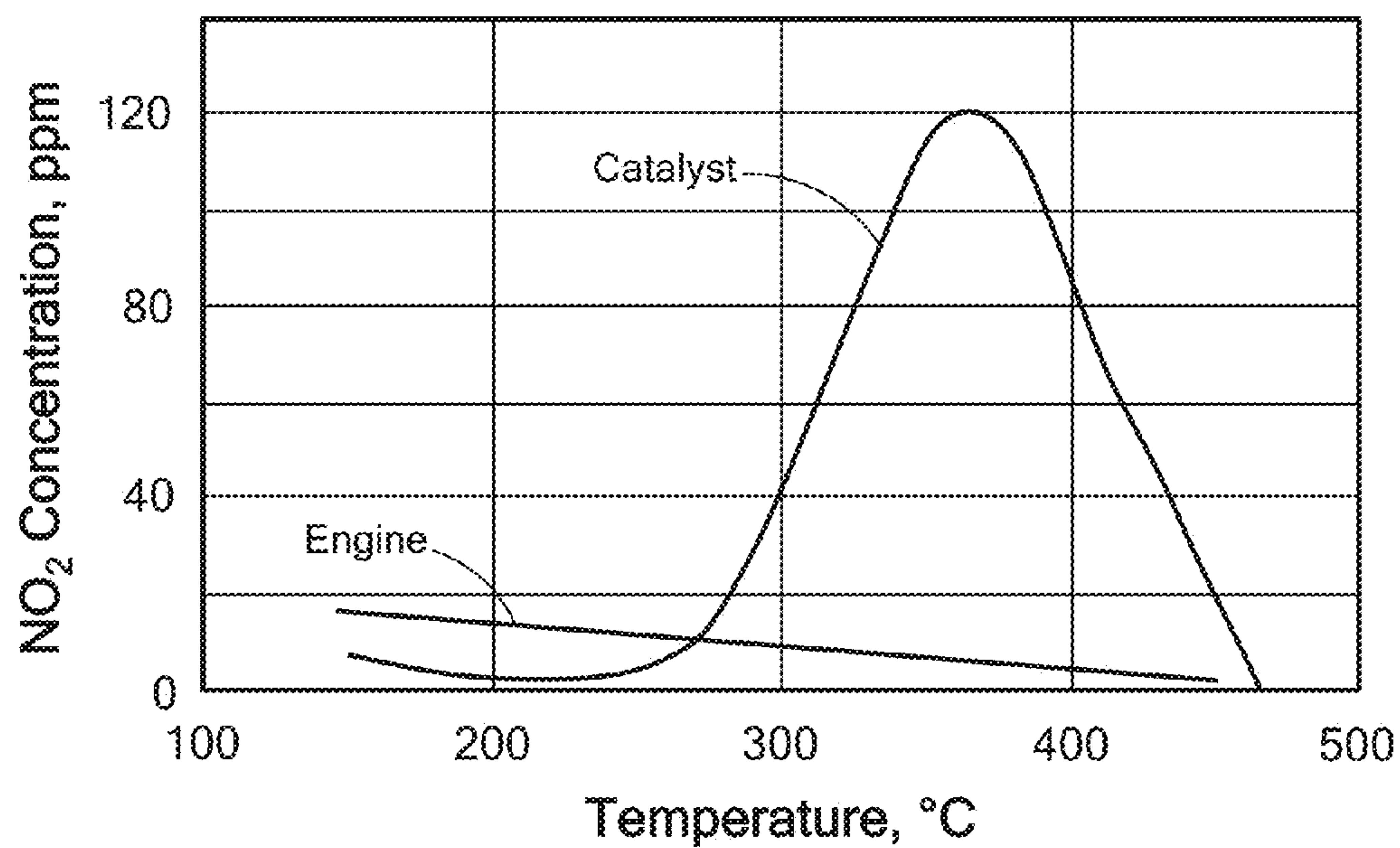
Concentration of NO 2 with Diesel Oxidation Catalyst
