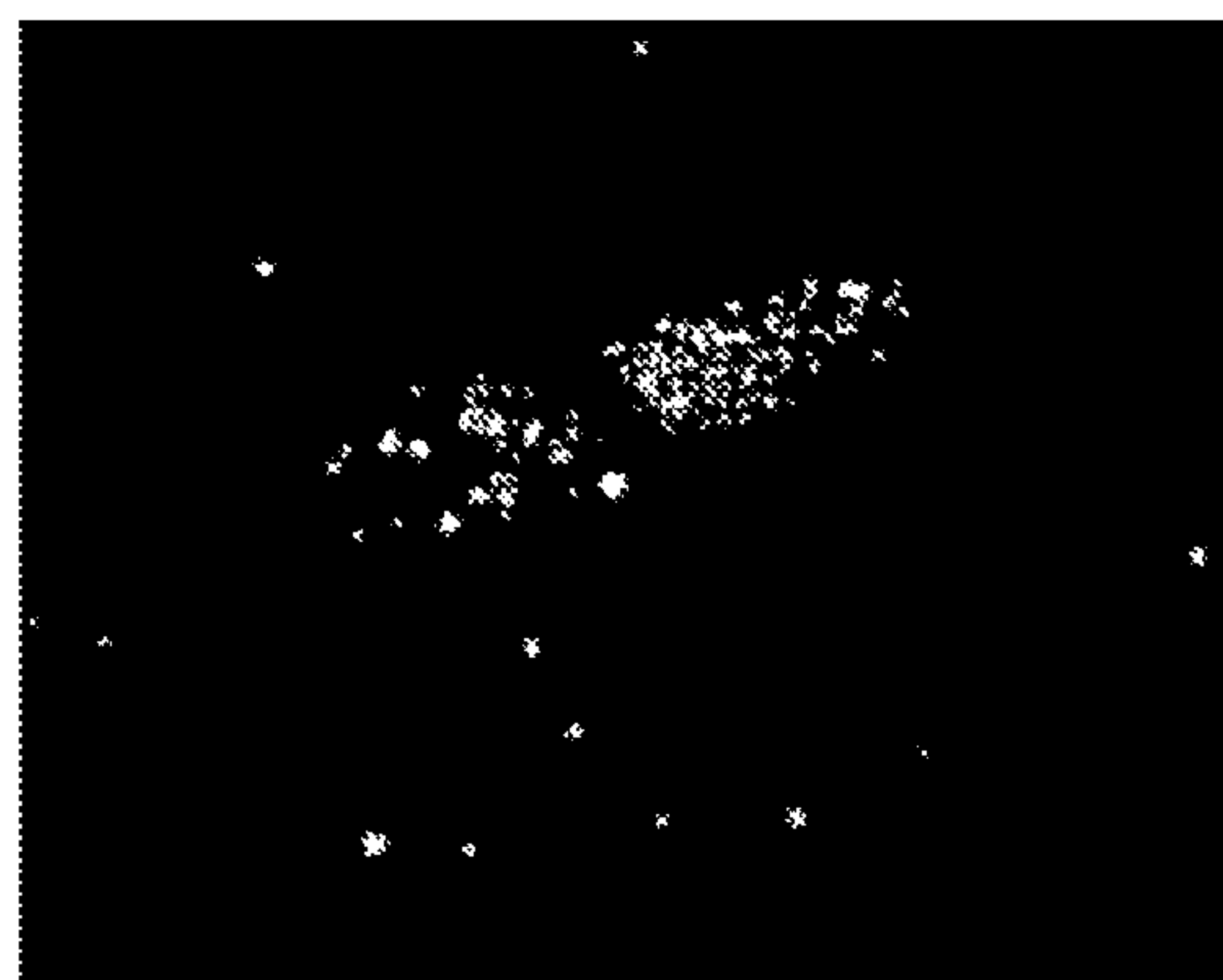
alpha-L-oxy-LNA; 2774
