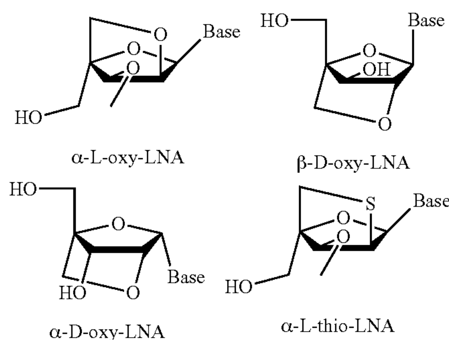
LNA diastereoisomers:
