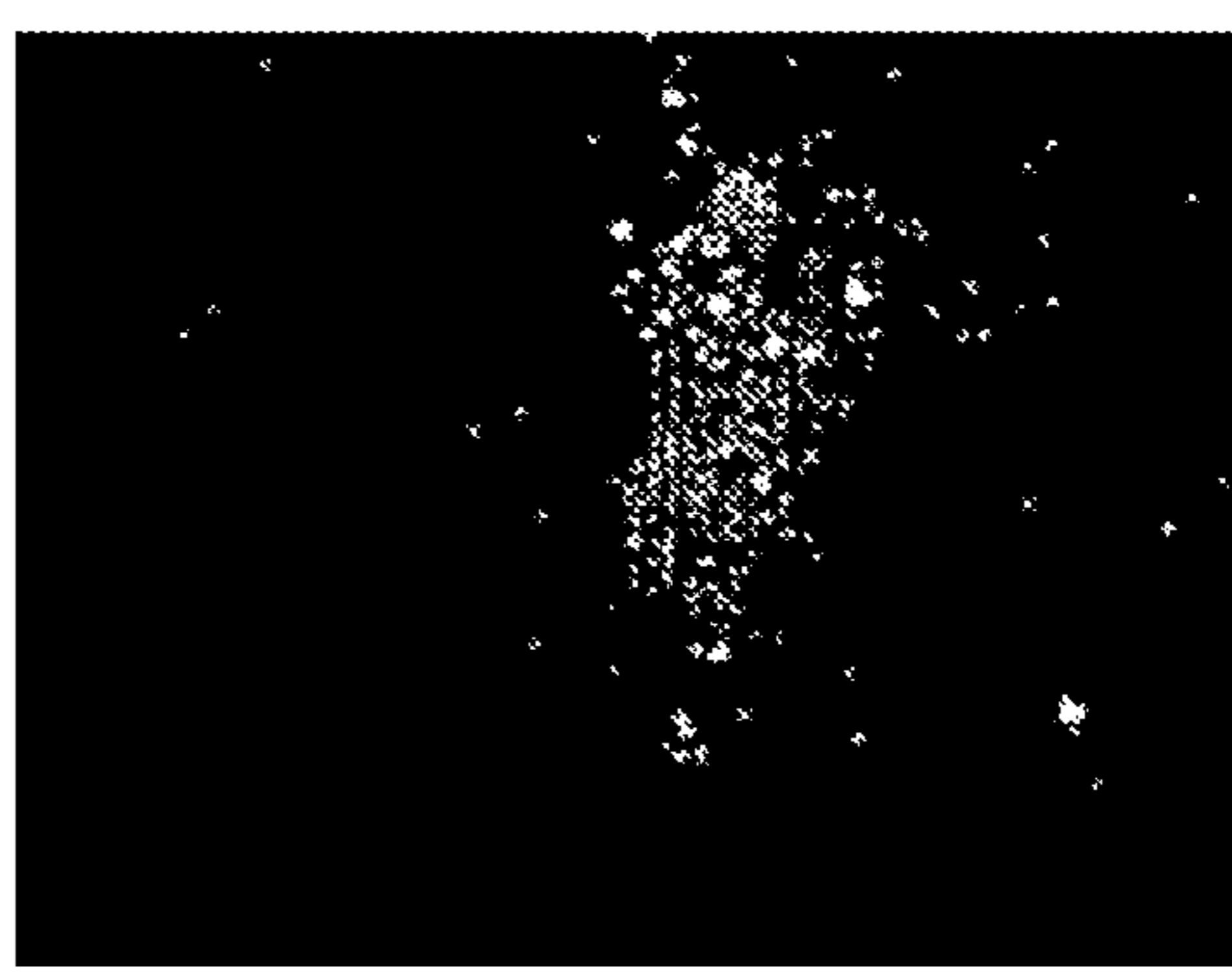
beta-D-thio-LNA; 2746
