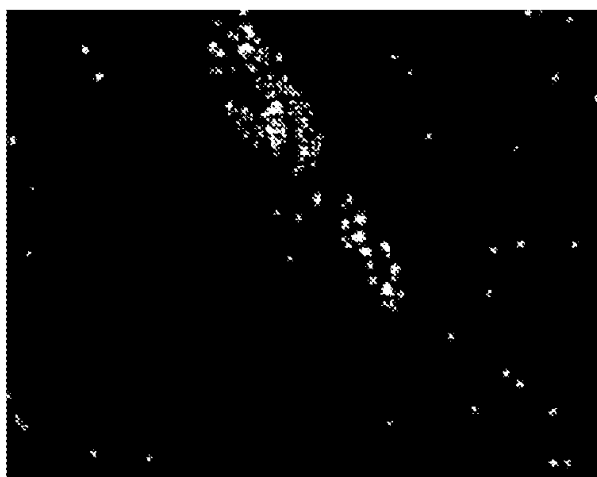
beta-D-oxy-LNA; 2740
