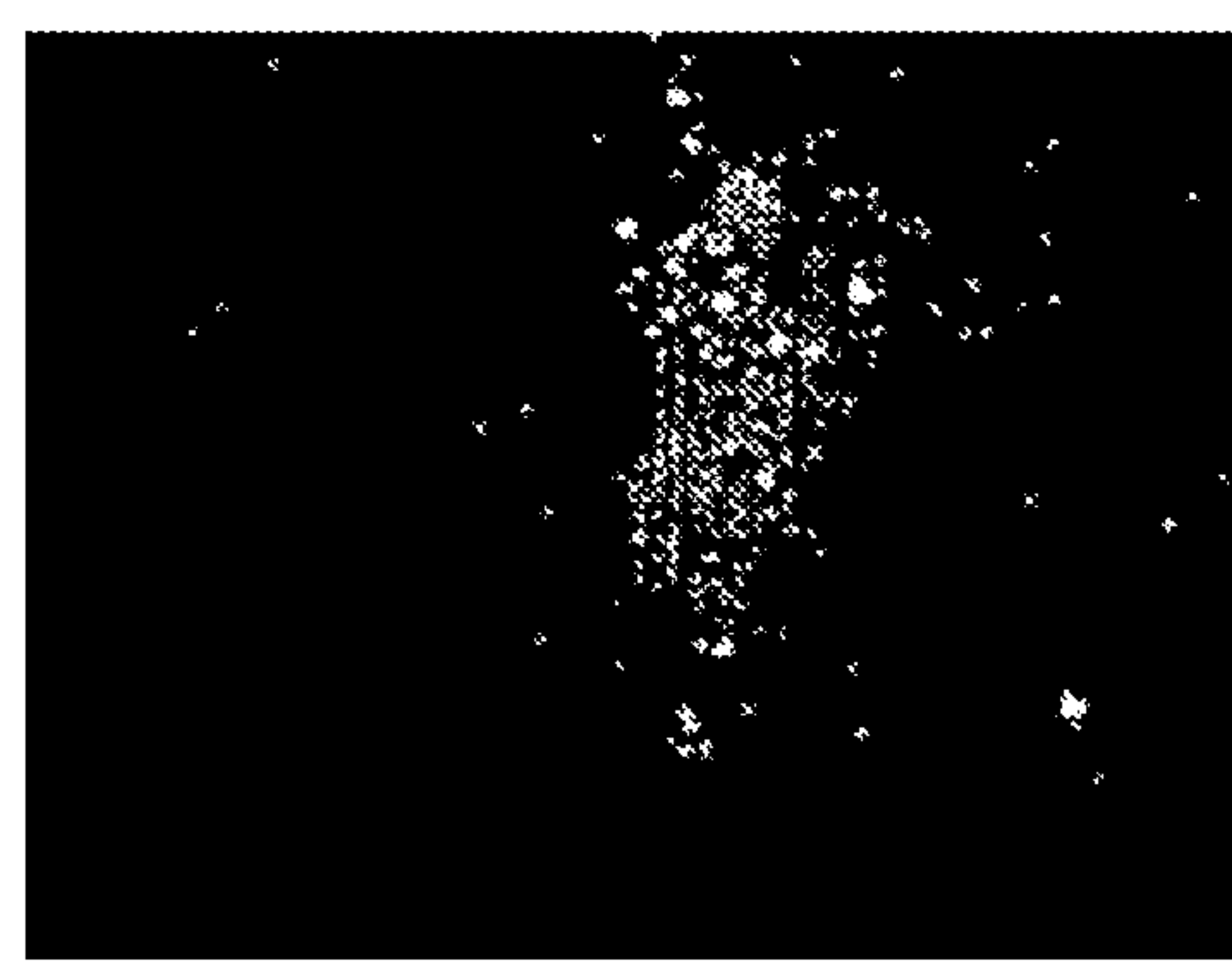
beta-D-thio-LNA; 2746
