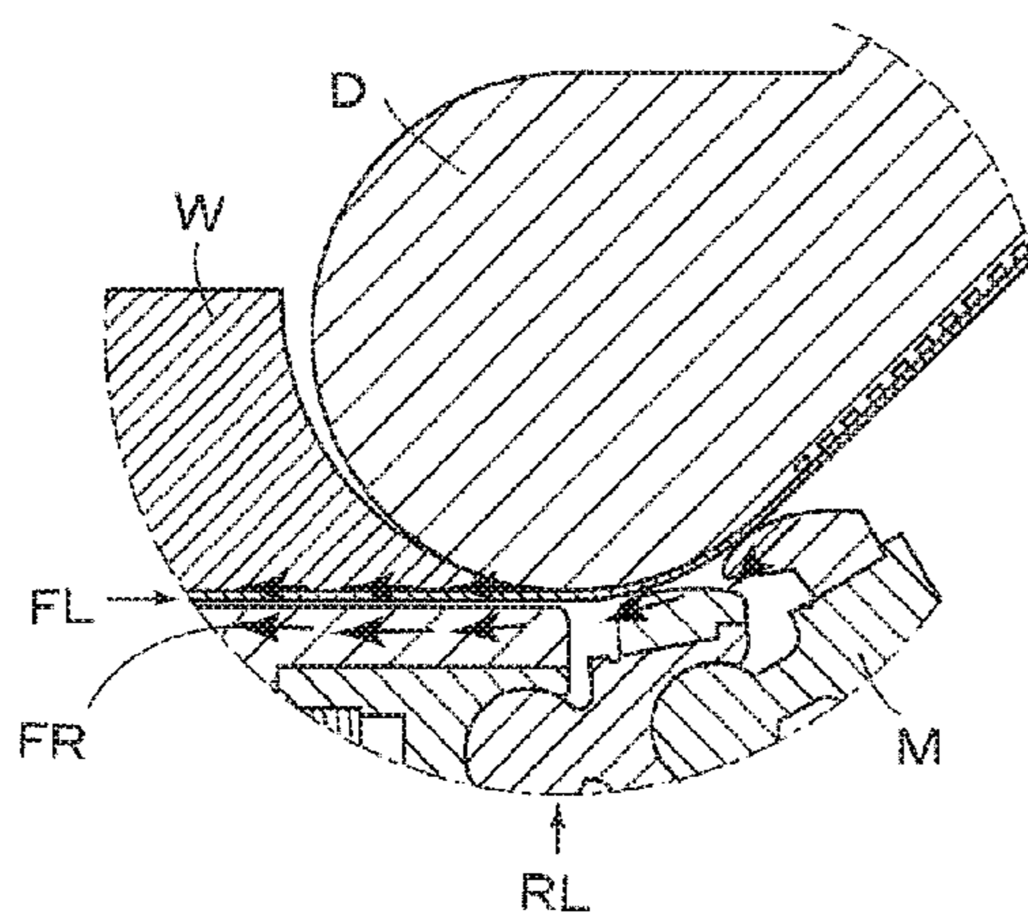
FIG. 31 PRIOR ART
