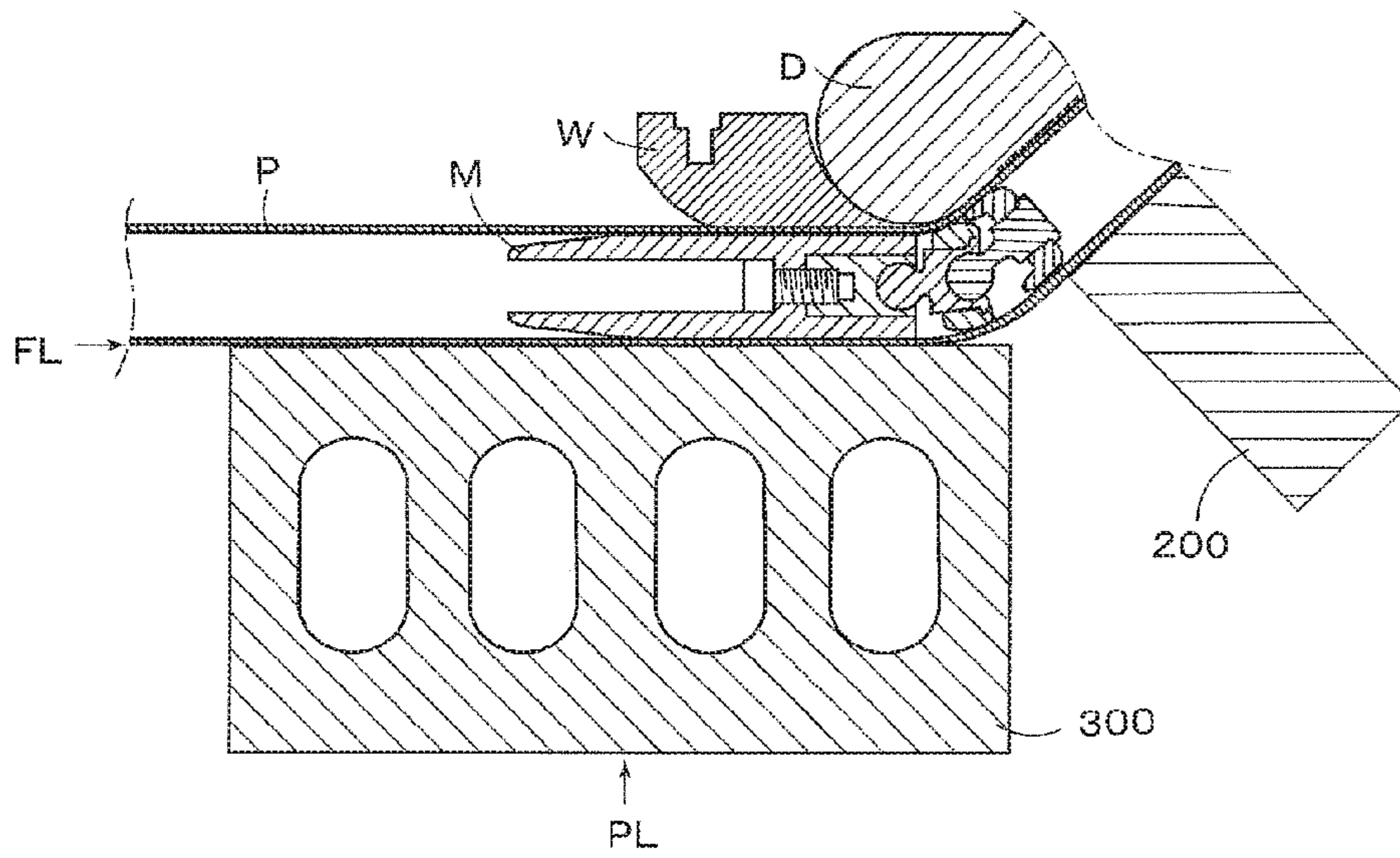
FIG. 30 PRIOR ART
