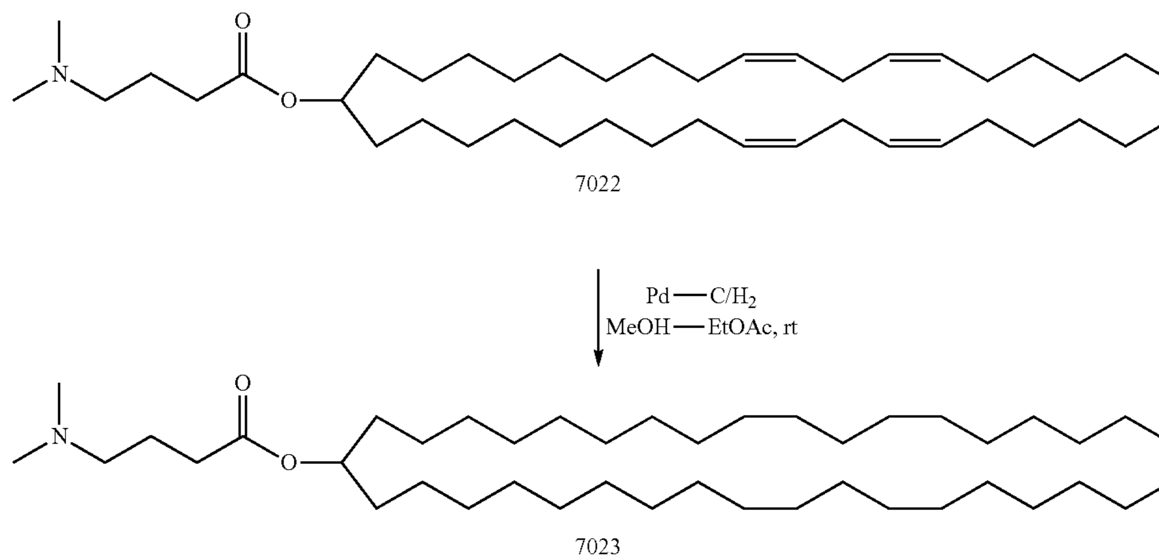
Scheme 6
