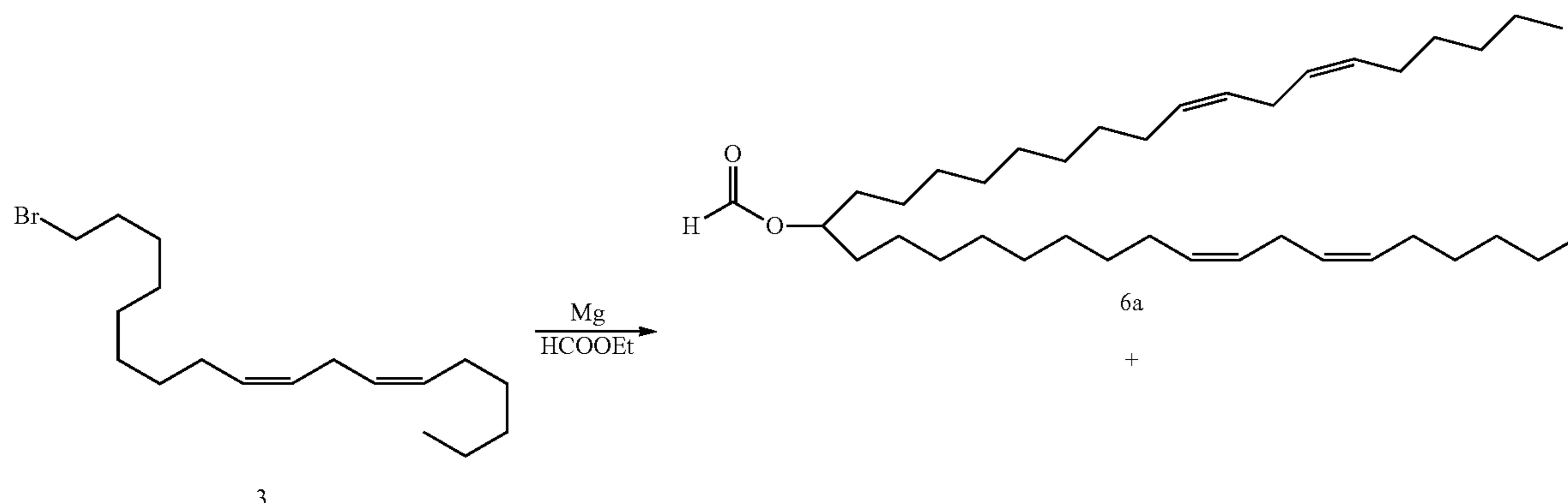
Scheme 2
