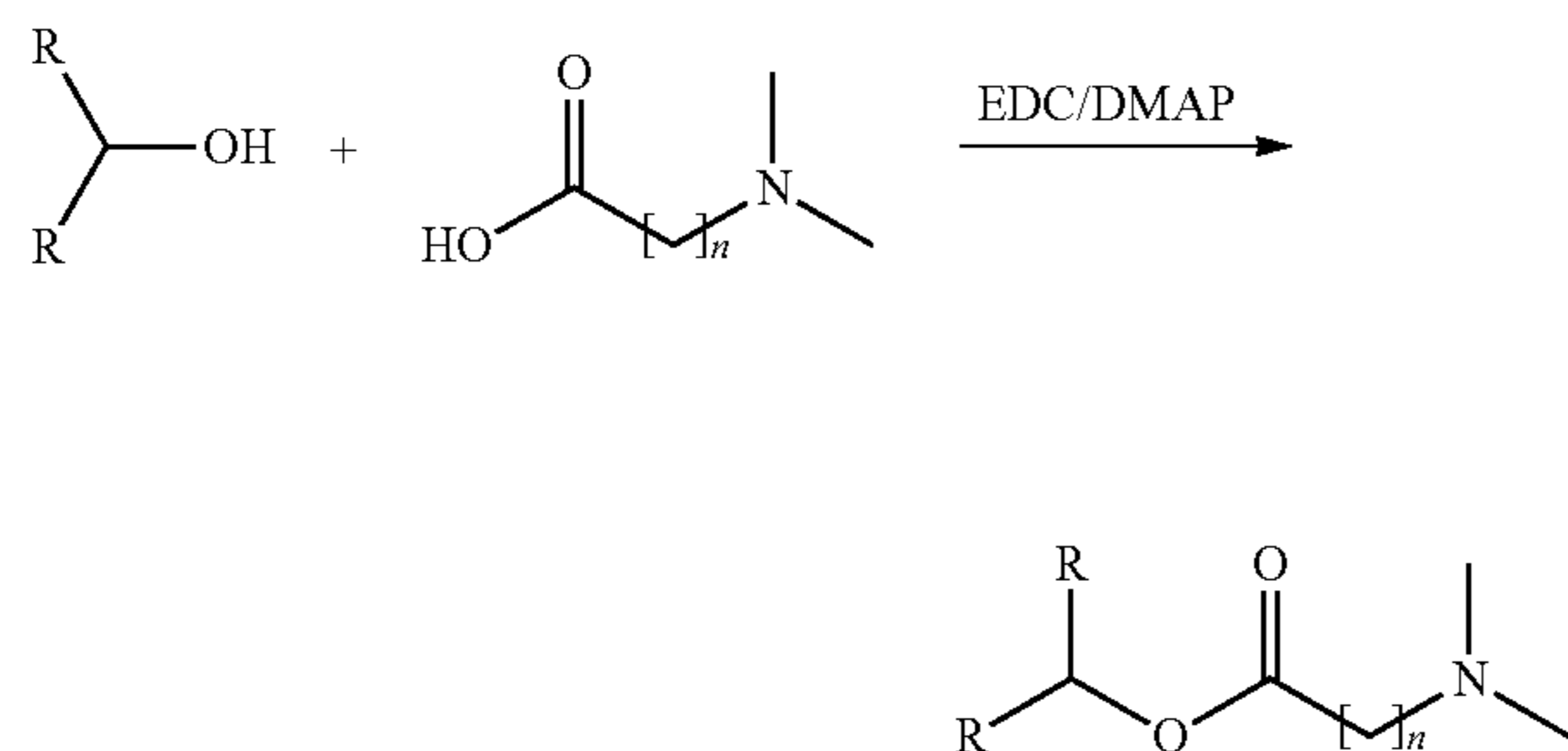
Scheme 1: M series (esters) synthesis
