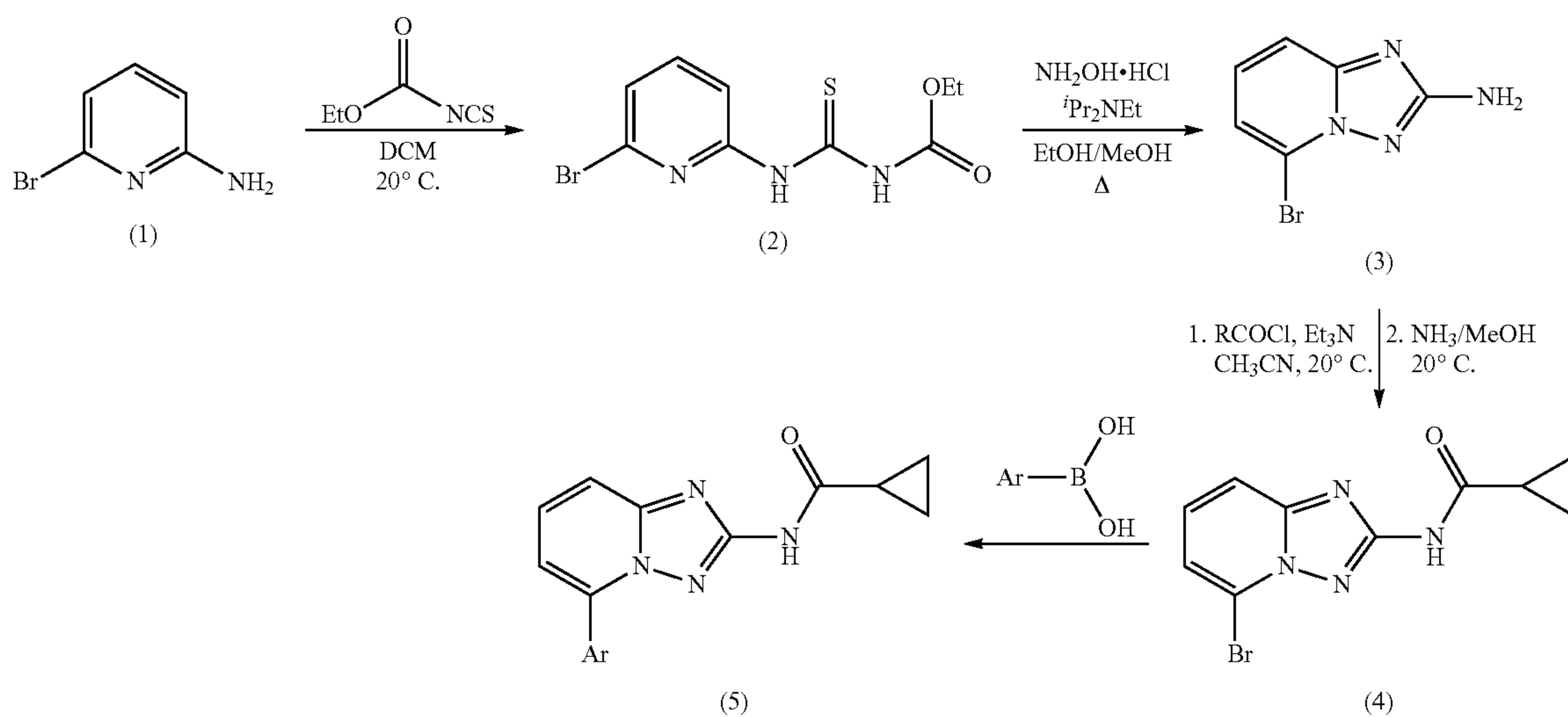
General Synthetic Method Scheme 1
