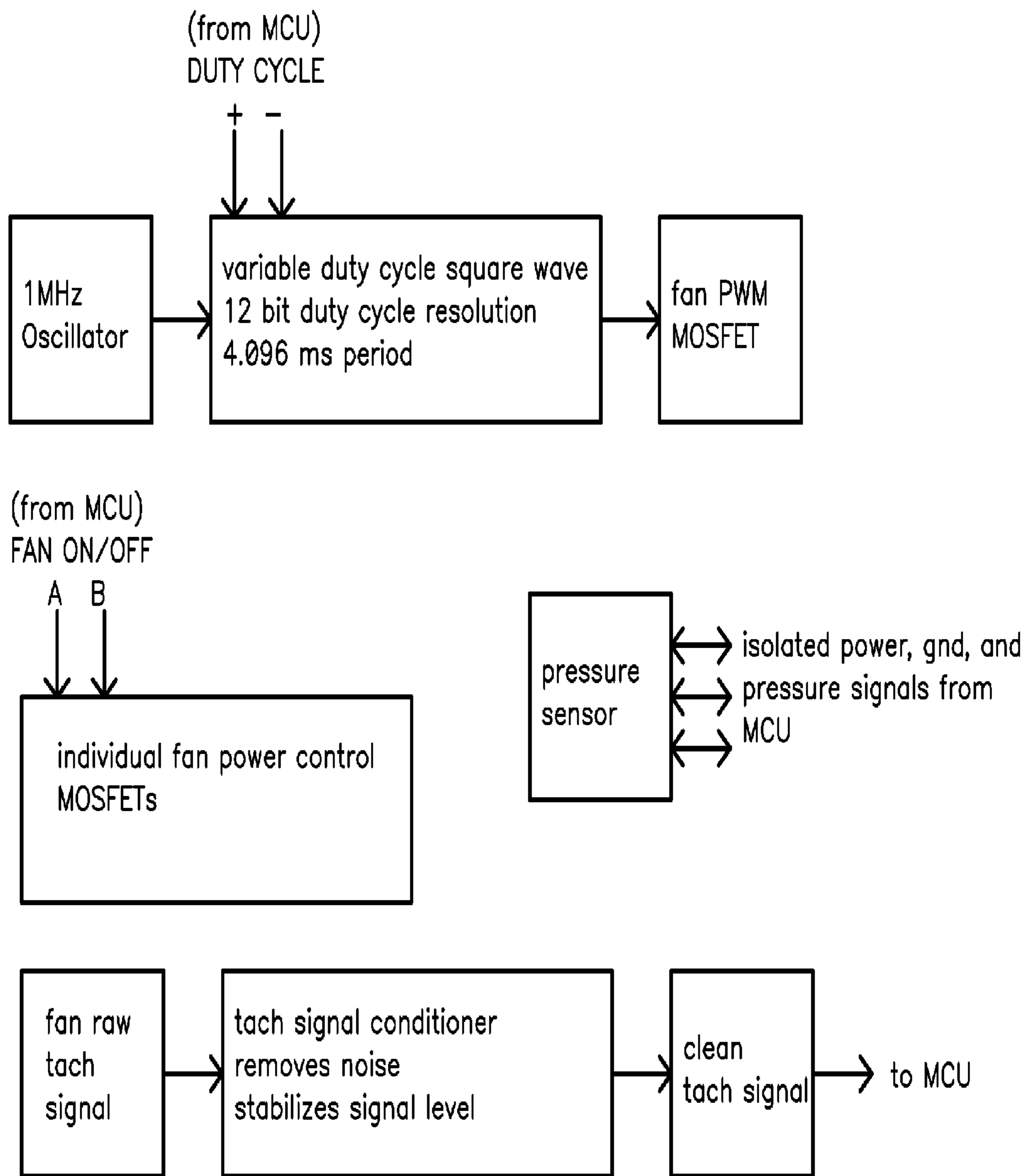
BLOWER CONTROL SYSTEM PWM PCB FUNCTIONAL DIAGRAM
