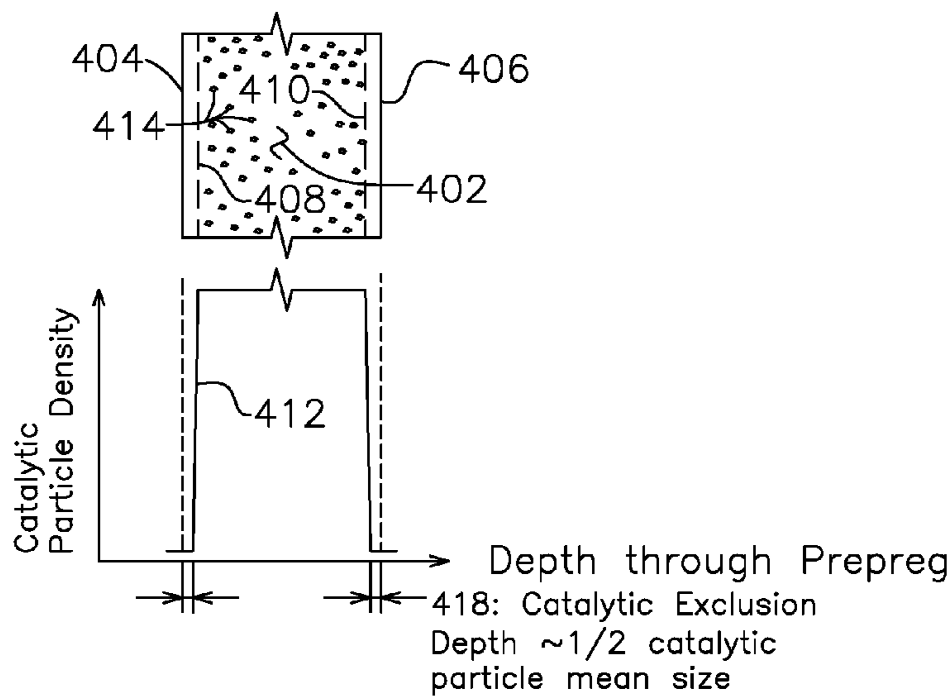
Figure 4 Catalytic Particle Distribution through Prepreg
