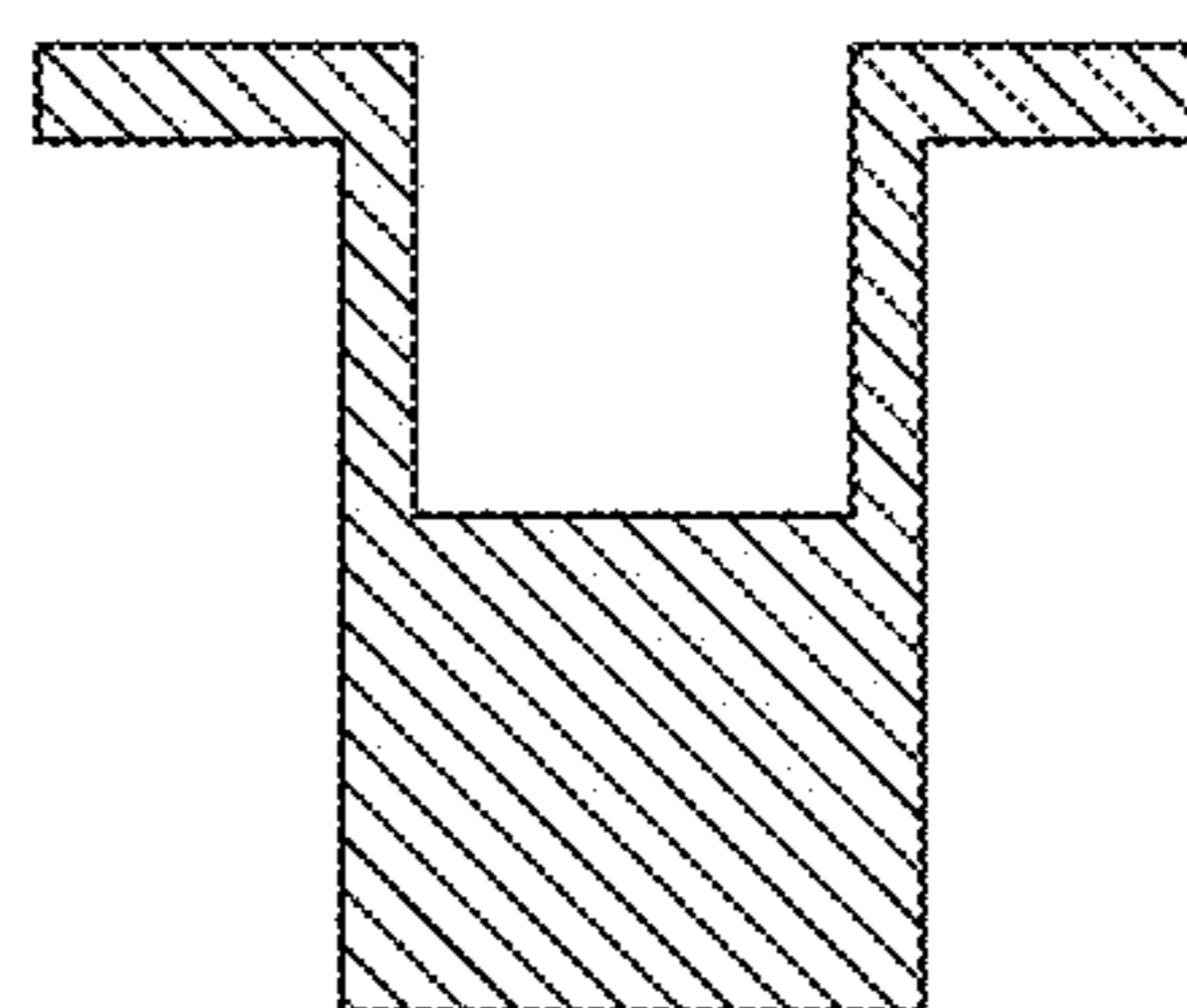
Partial fill with Super conformal ECD
