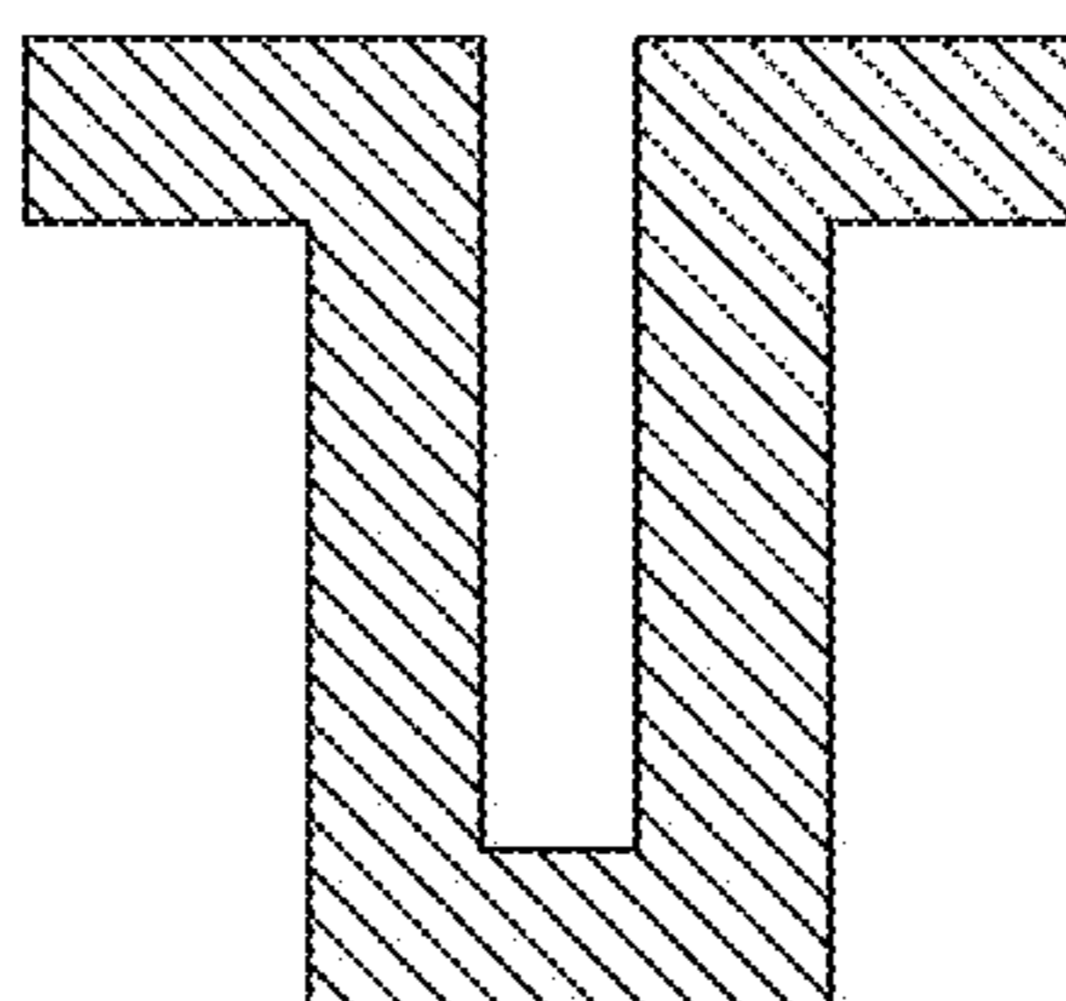
Partial fill with conformal ECD
