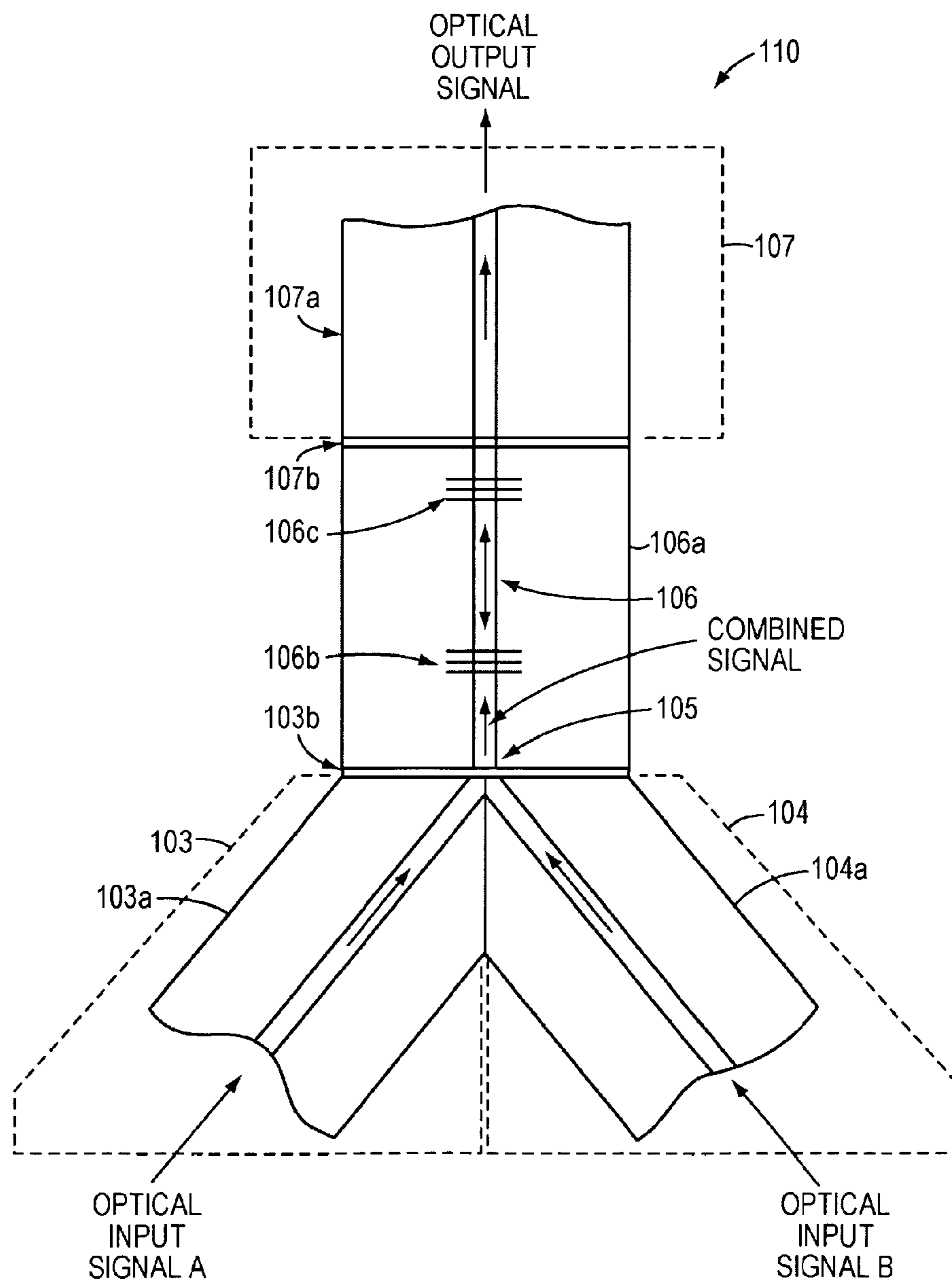
ALL-OPTICAL LOGICAL GATE IMPLEMENTED WITH OPTICAL FIBERS
