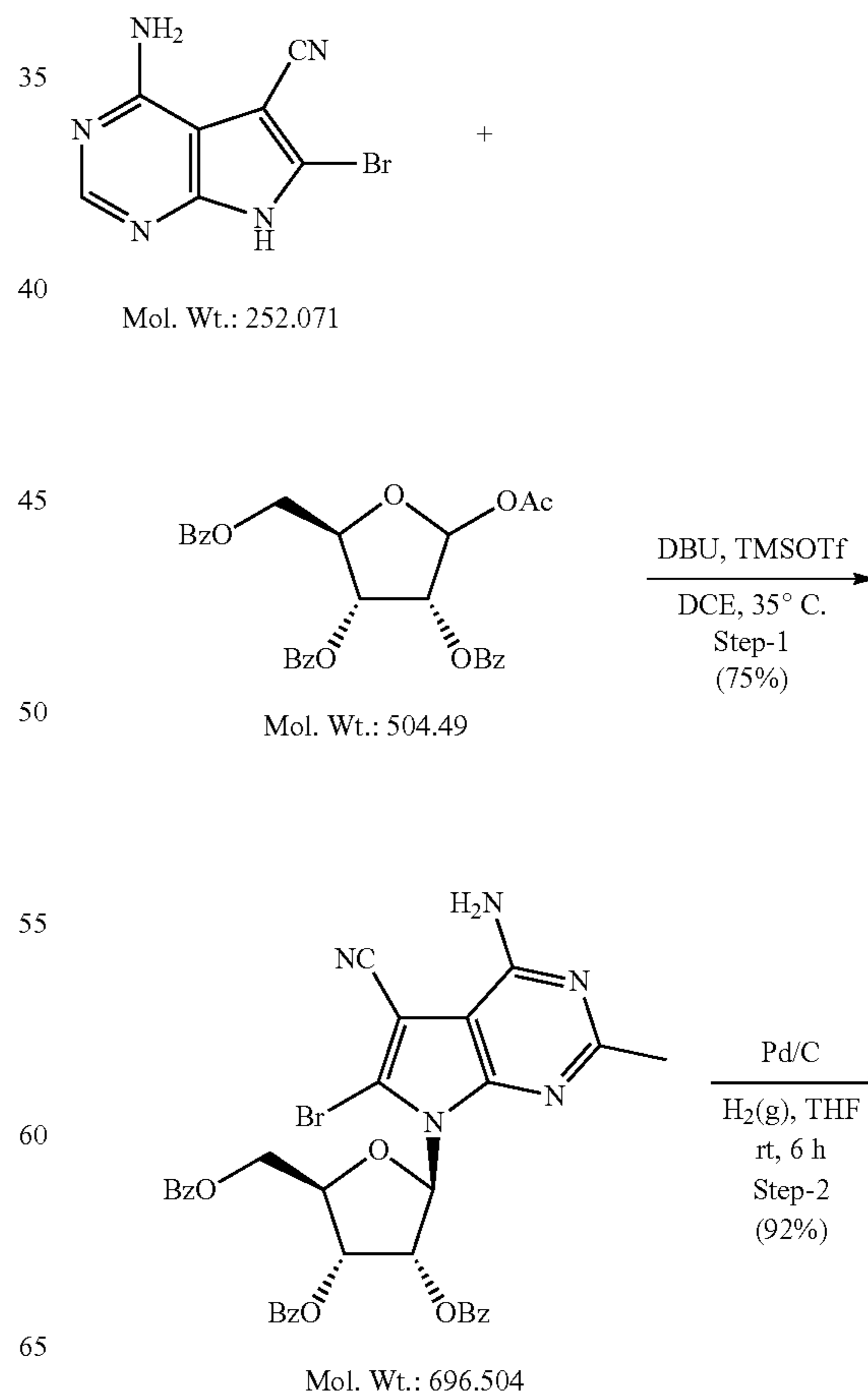
Scheme 2: General Synthesis of Compounds of the Invention
