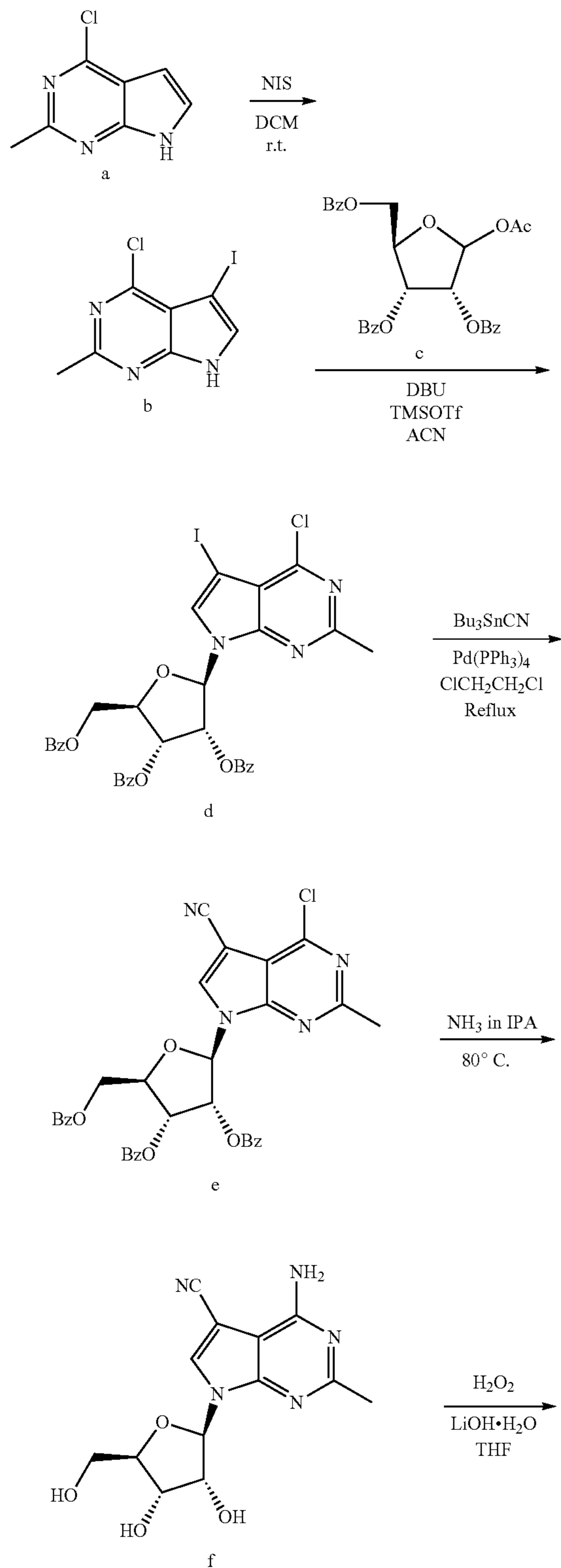
Scheme 1: General Synthesis of Compounds of the Inventions
