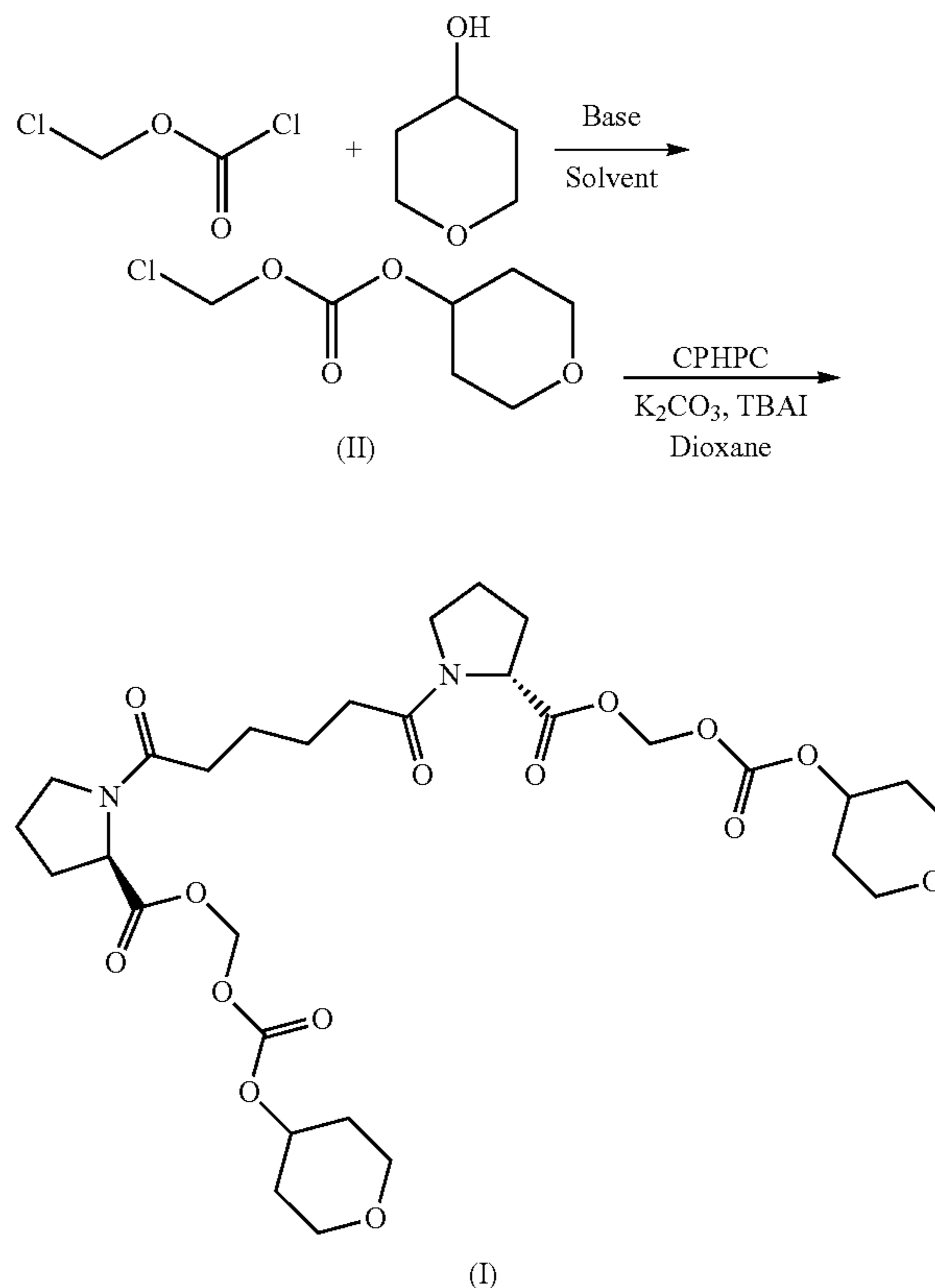
Reaction Scheme 1
